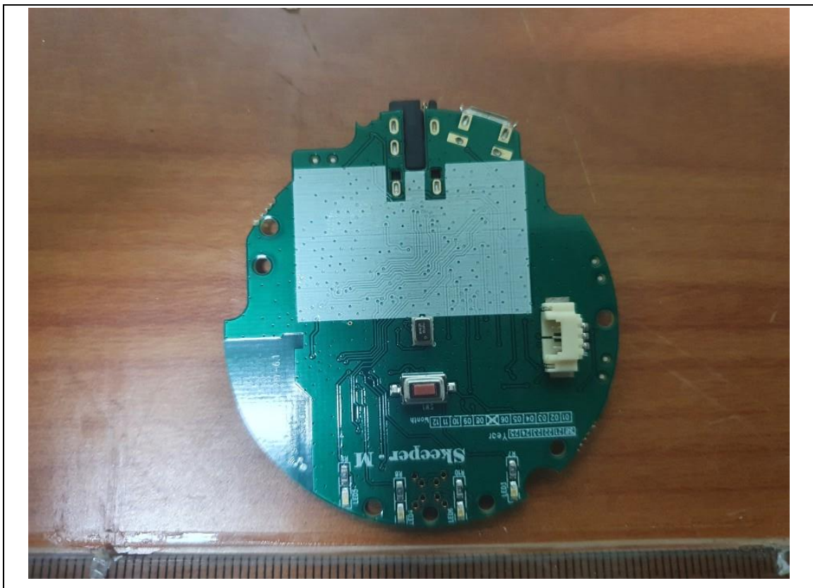
MainBoard-Rear
