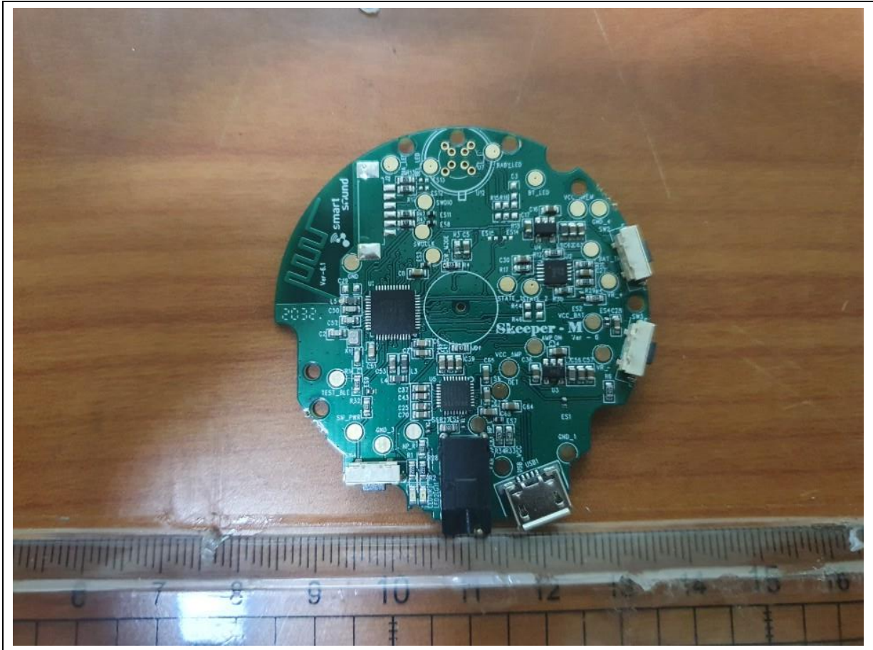
MainBoard-Rear
