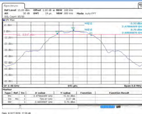
GFSK (BLE) HIGH CHANNEL
