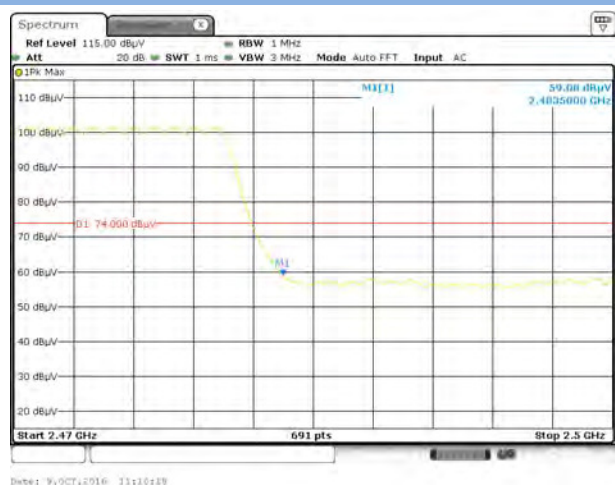
GFSK HIGH FREQUENCY BAND, PEAK
