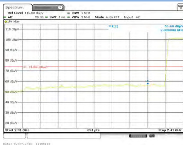
GFSK LOW FREQUENCY BAND, PEAK
