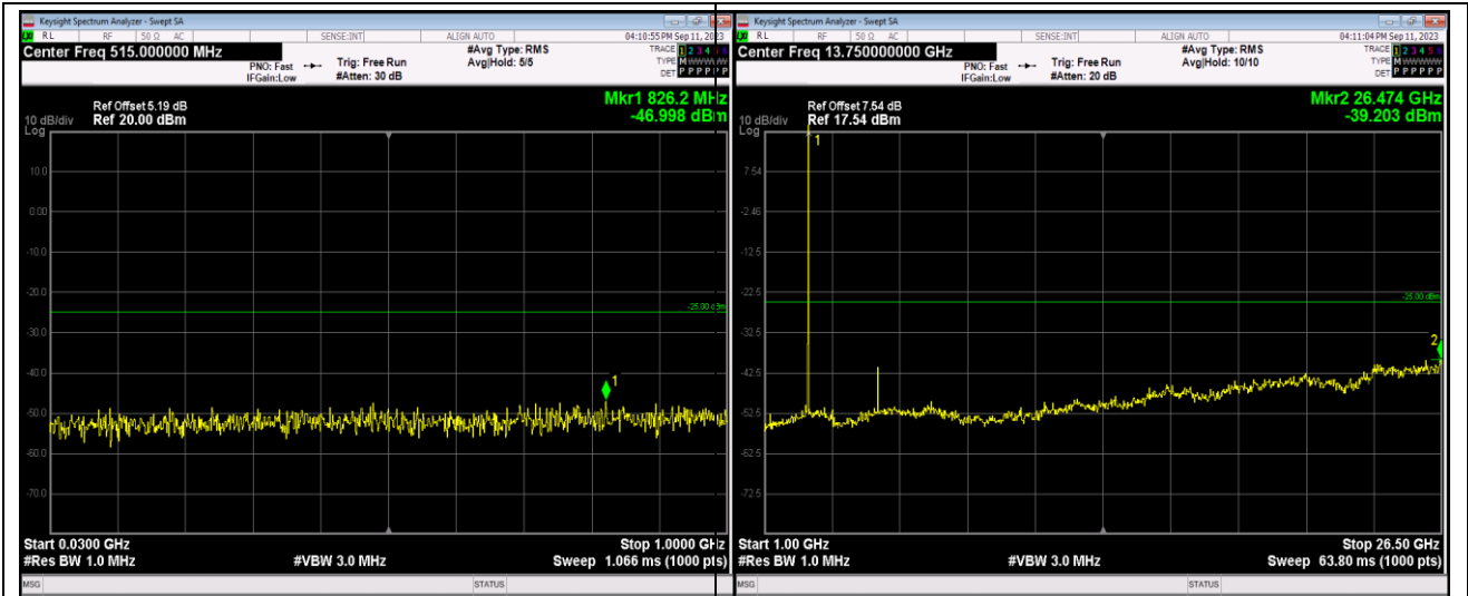
Band41-5MHz-64QAM-40265-1RB#0-Range1:30~1000MHz
