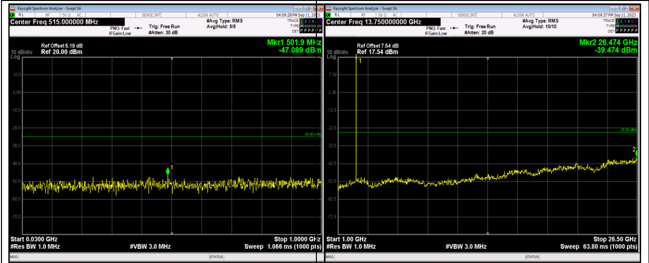
Band41-5MHz-64QAM-40740-1RB#0-Range1:30~1000MHz
