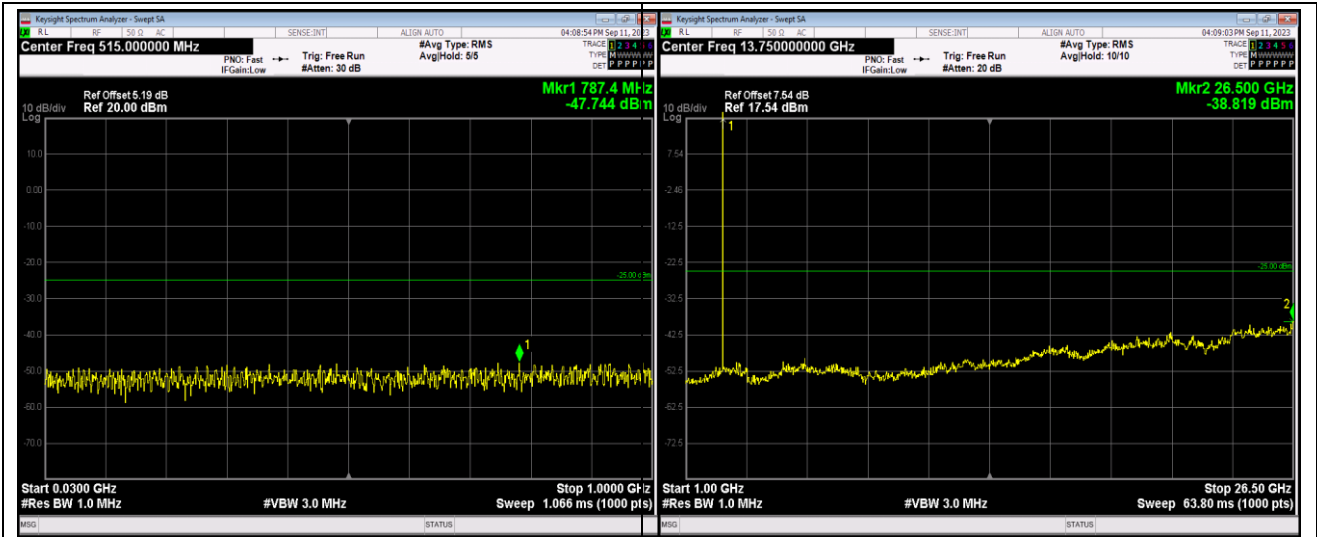
Band41-5MHz-QPSK-40740-1RB#0-Range1:30~1000MHz
