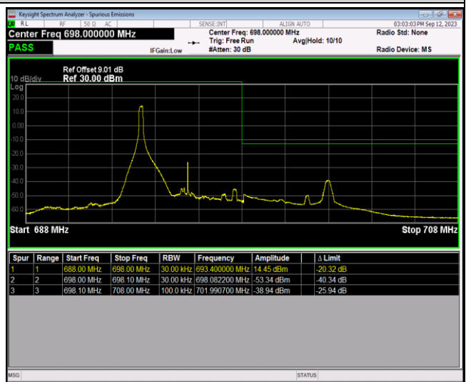
Band71-5MHz-64QAM-133447-25RB#0
