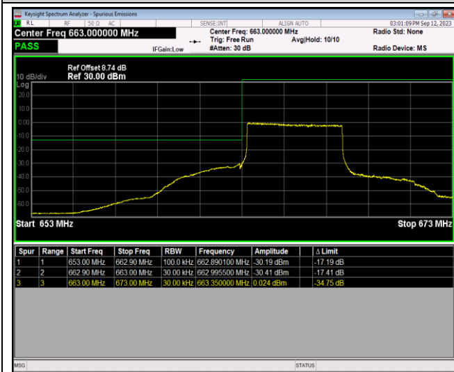
Band71-5MHz-64QAM-133447-1RB#24
