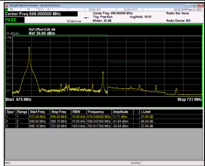
Band71-20MHz-16QAM-133372-100RB#0
