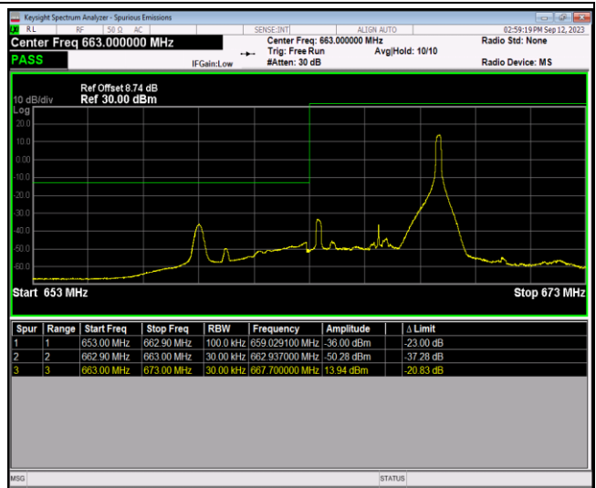
Band71-5MHz-64QAM-133447-1RB#0
