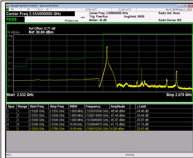
Band41-20MHz-64QAM-40340-100RB#0
