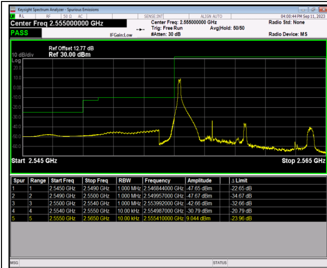
Band41-5MHz-64QAM-40265-25RB#0
