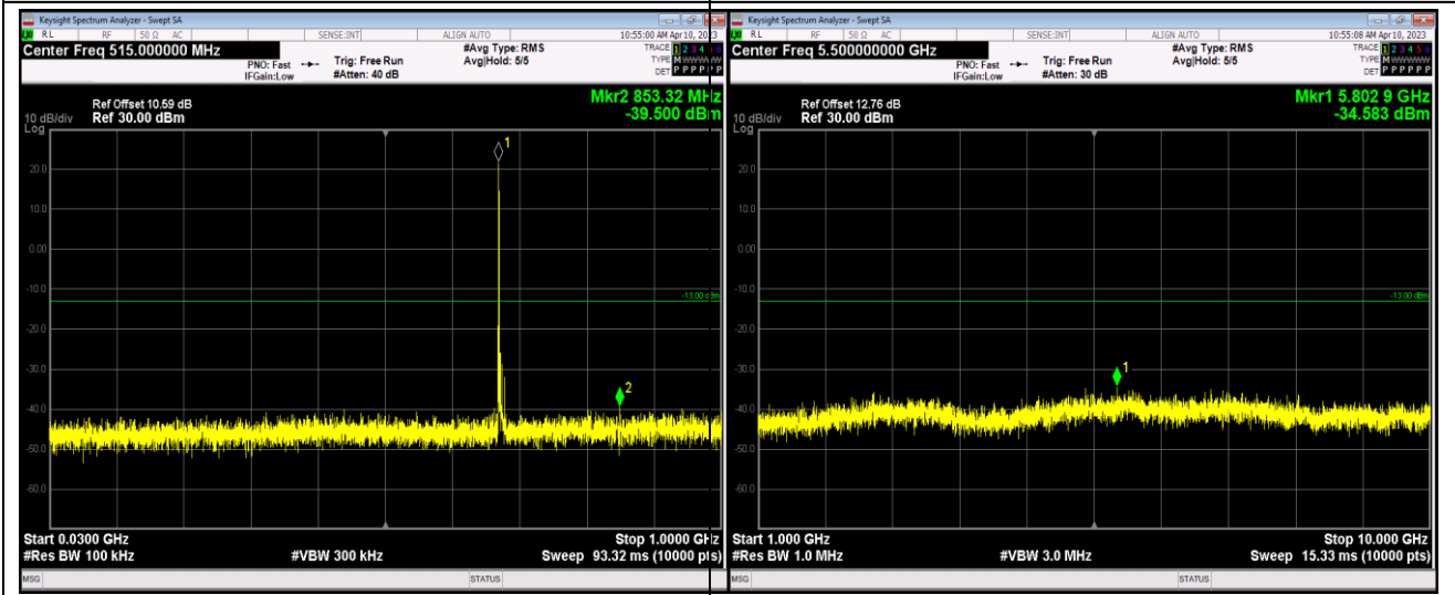
Band71-5MHz-16QAM-133297-1RB#0-Range1:30 ~1000MHz
