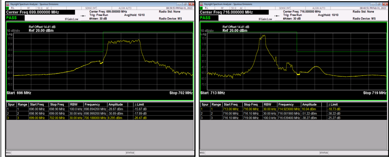
Band12-1.4MHz-16QAM-23173-1RB#5
