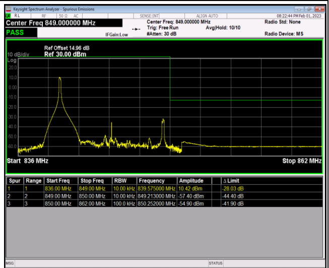
Band5-10MHz-QPSK-20600-50RB#0
