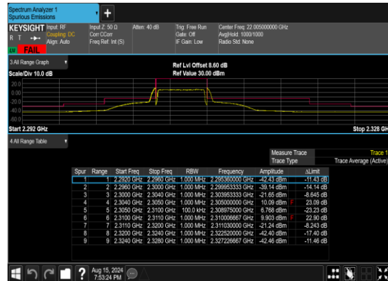
N30(5M)_DFT-s- OFDM_QPSK_Outer_Full_Low_CH
