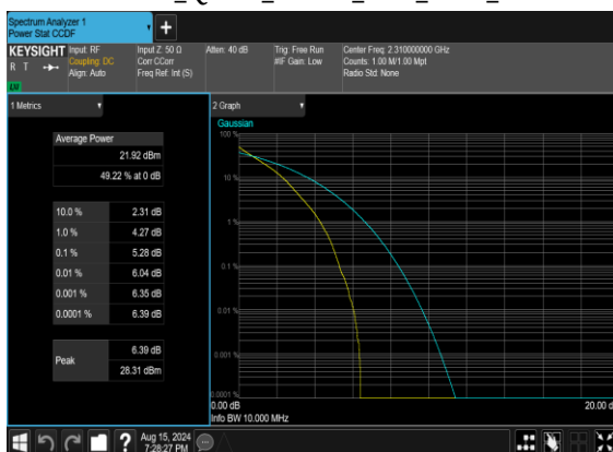
N30(10M)_DFT-s- OFDM_QPSK_Outer_Full_Low_CH
