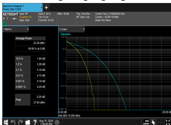
N30(10M)_DFT-s-OFDM_PI_2- BPSK_Outer_Full_Low_CH
