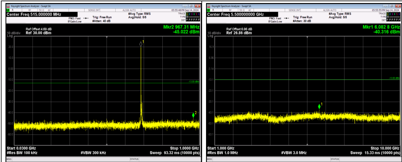
Band71-20MHz-QPSK-133222-1RB#0-Range1:30~1000MHz
