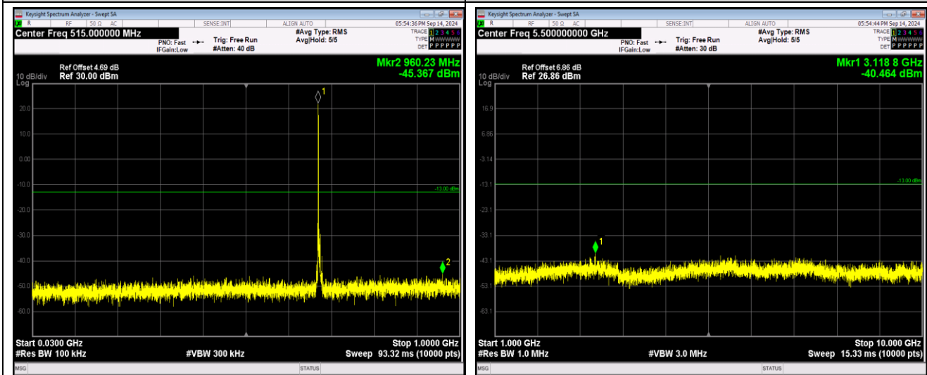
Band71-5MHz-16QAM-133447-1RB#0-Range1:30~1000MHz
