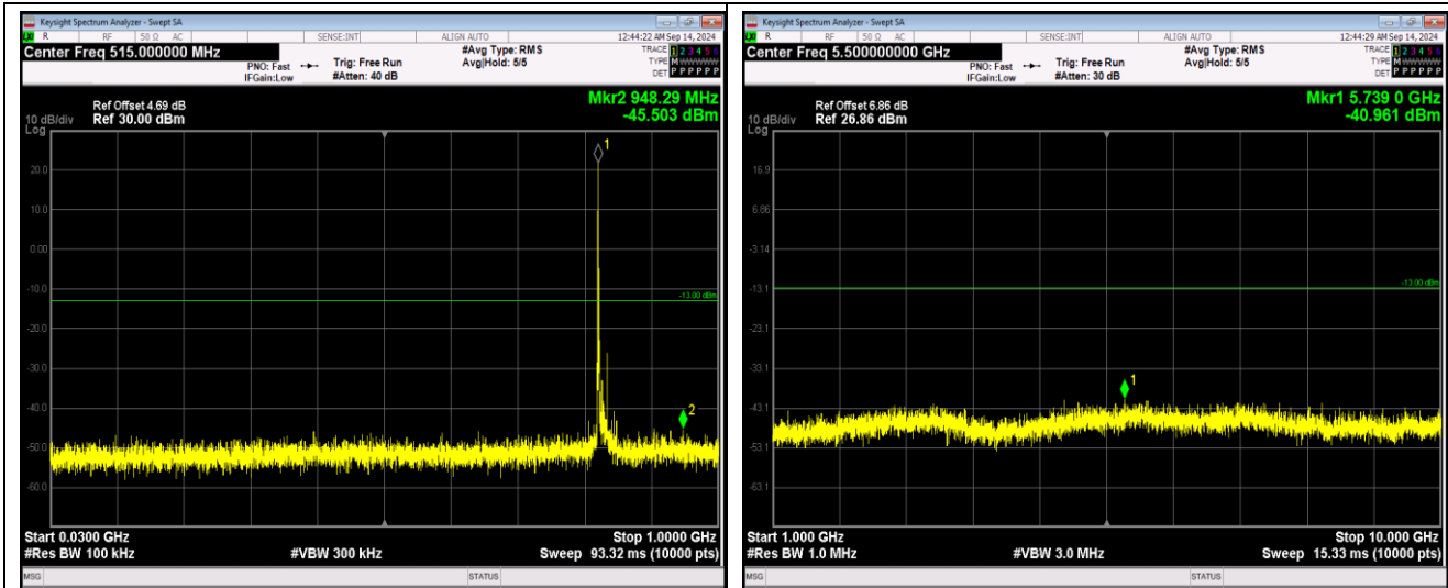
Band26-15MHz-QPSK-26915-1RB#0-Range1:30~1000MHz
