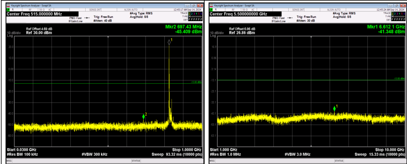
Band26-15MHz-QPSK-26965-1RB#0-Range1:30~1000MHz
