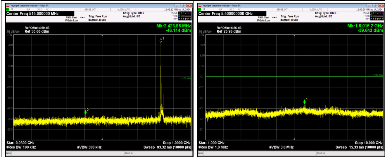
Band26-15MHz-QPSK-26965-1RB#0-Range1:30~1000MHz
