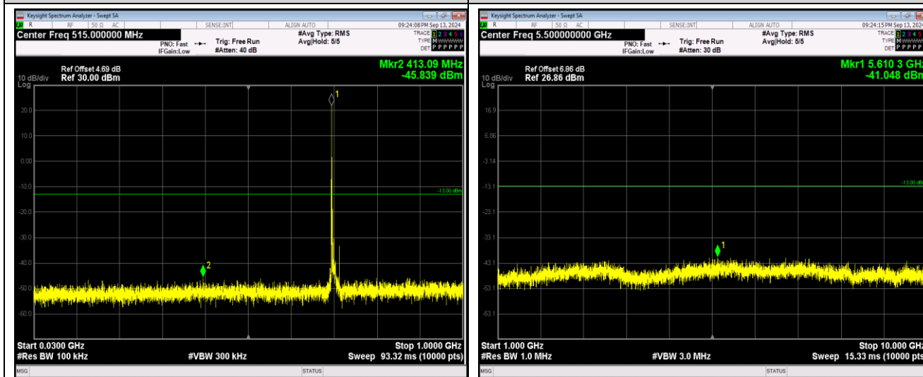
Band12-10MHz-QPSK-23130-1RB#0-Range1:30~1000MHz
