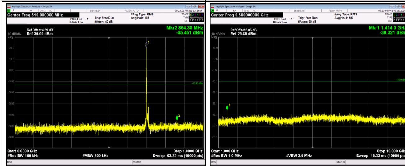
Band12-10MHz-QPSK-23130-1RB#0-Range1:30~1000MHz
