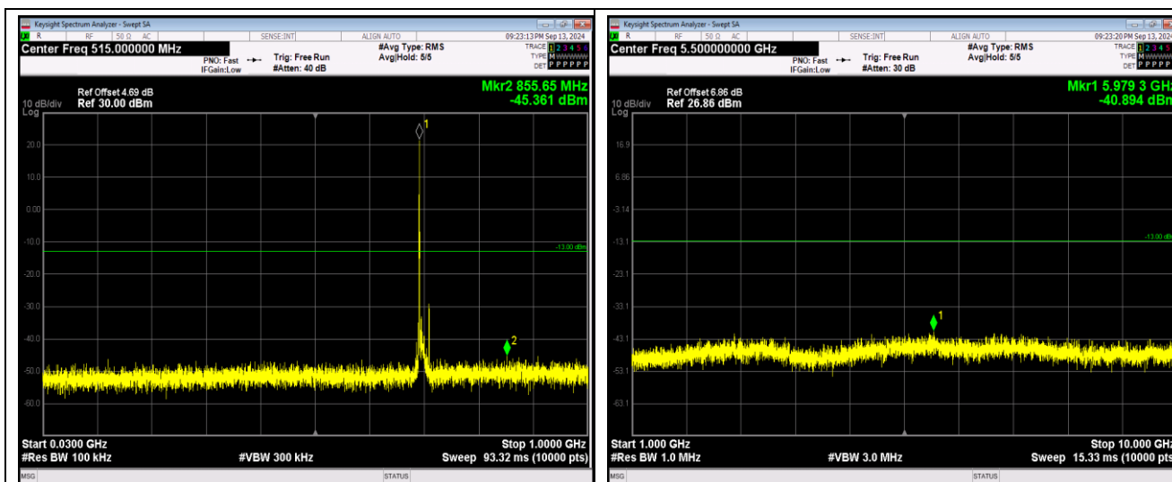
Band12-10MHz-QPSK-23095-1RB#0-Range1:30~1000MHz
