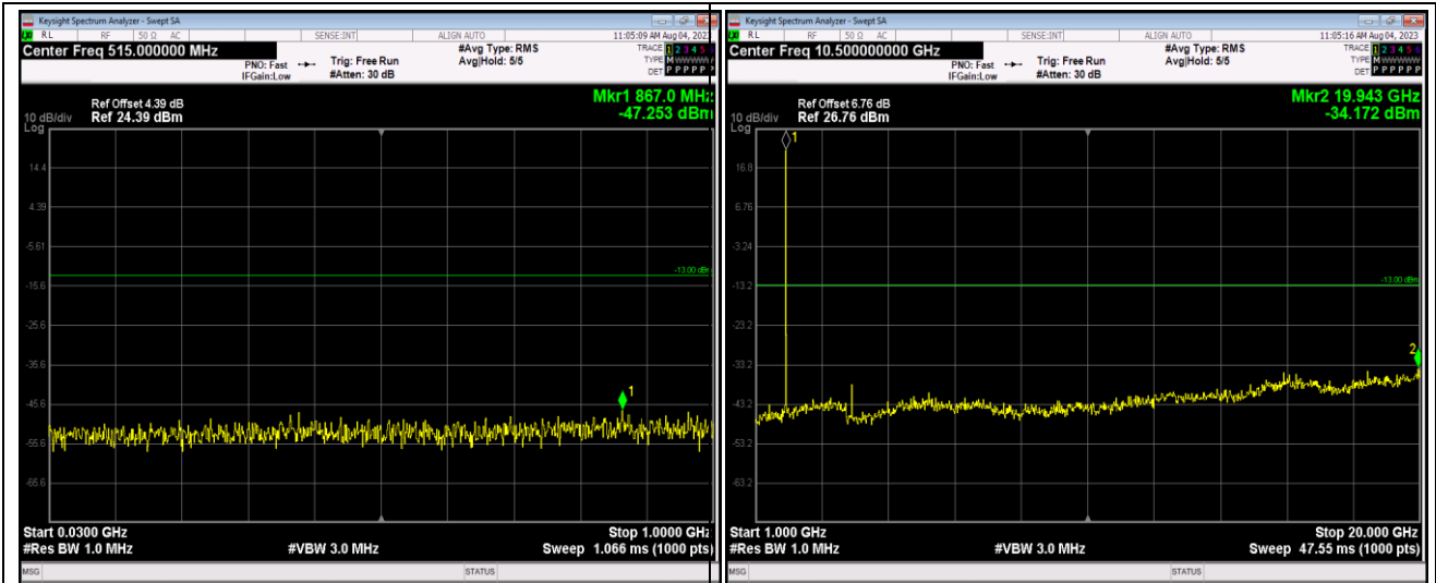
Band25-1.4MHz-QPSK-26683-1RB#0-Range1:30~1000MHz
