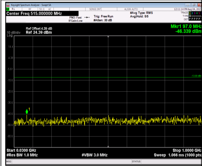
Band25-20MHz-16QAM-26365-1RB#0-Range1:30~1000MHz
