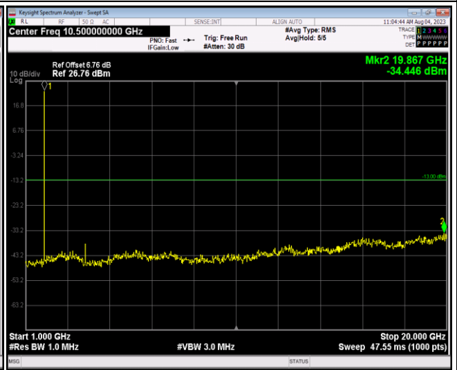
Band25-1.4MHz-16QAM-26047-1RB#0-Range2:1000~20000MHz
