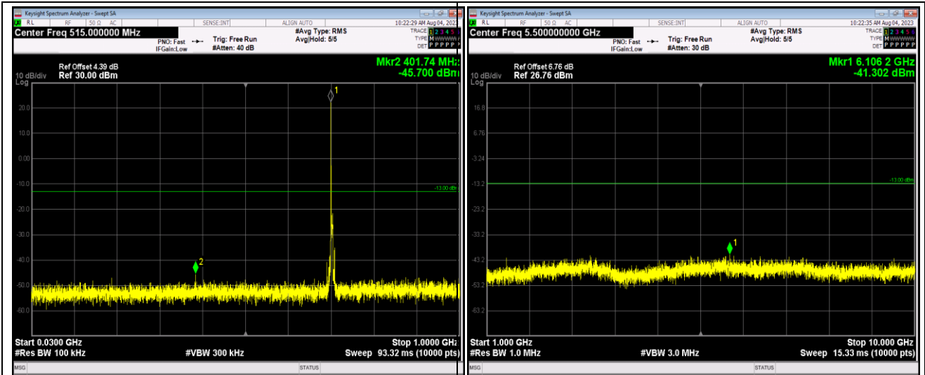
Band17-5MHz-16QAM-23825-1RB#0-Range1:30~1000MHz
