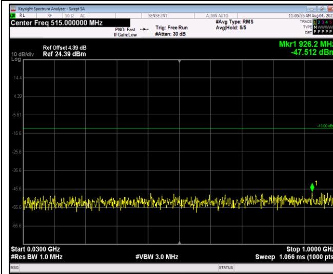
Band25-1.4MHz-16QAM-26047-1RB#0-Range1:30~1000MHz
