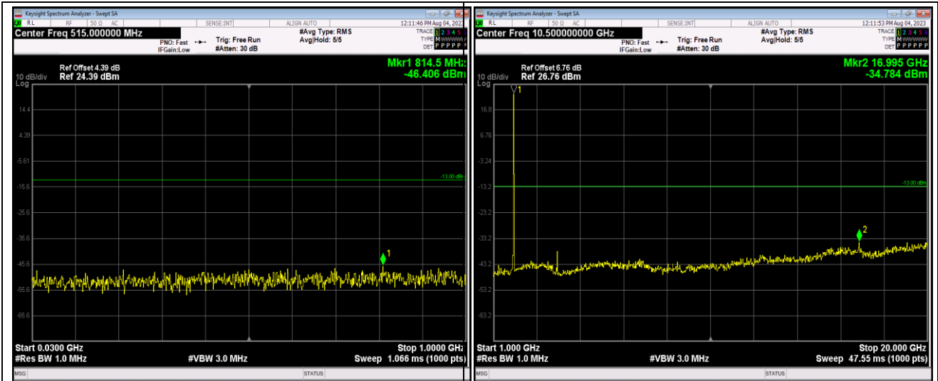
Band25-20MHz-16QAM-26140-1RB#0-Range1:30~1000MHz
