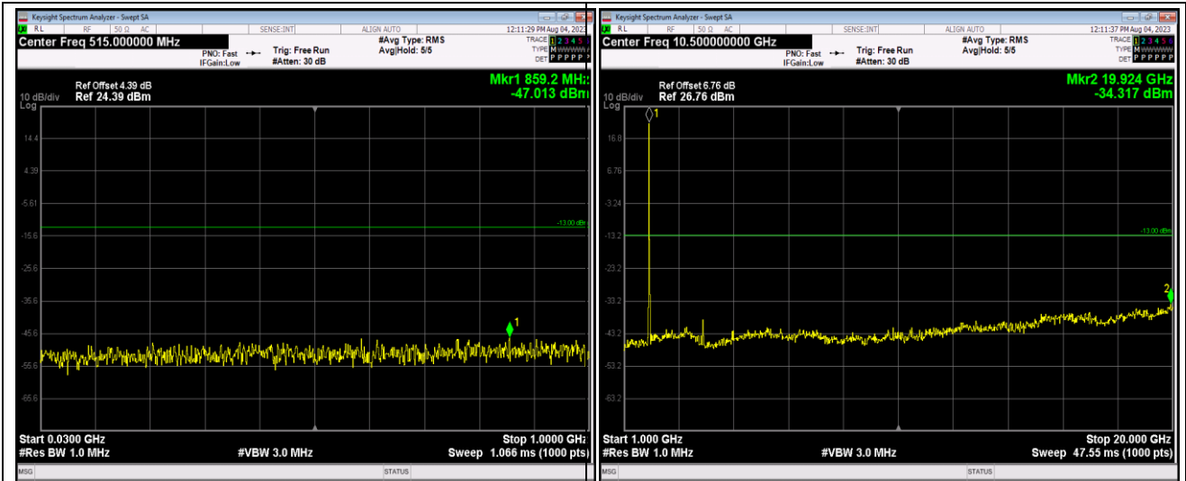
Band25-20MHz-64QAM-26590-1RB#0-Range1:30~1000MHz
