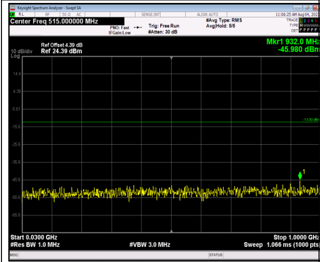
Band25-1.4MHz-64QAM-26683-1RB#0-Range1:30 ~1000MHz
