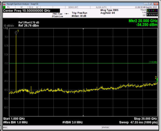
Band25-1.4MHz-64QAM-26683-1RB#0-Range2:1000 ~20000MHz
