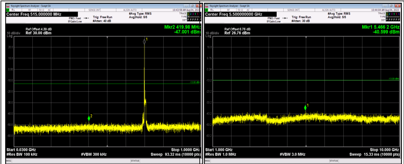
Band17-10MHz-64QAM-23780-1RB#0-Range1:30~1000MHz
