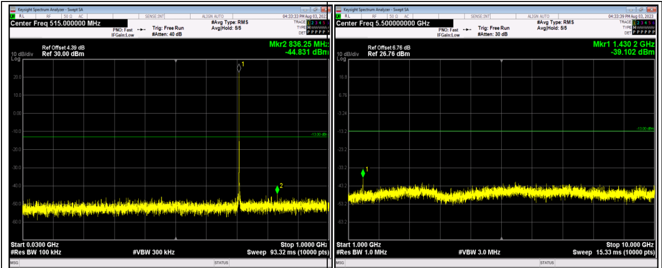
Band12-1.4MHz-64QAM-23017-1RB#0-Range1:30 ~1000MHz
