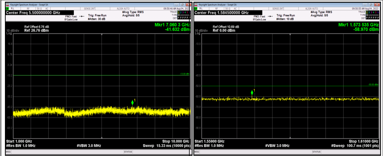
Band13-10MHz-QPSK-23230-1RB#0-Range2:1000~10000MHz
