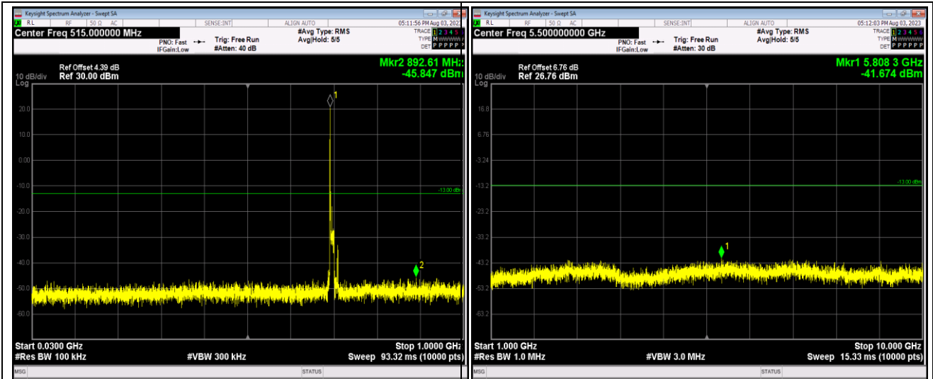
Band12-10MHz-64QAM-23095-1RB#0-Range1:30~1000MHz
