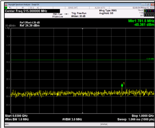
Band4-20MHz-QPSK-20175-1RB#0-Range1:30~1000MHz
