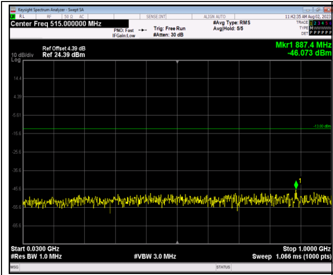
Band2-1.4MHz-16QAM-18607-1RB#0-Range1:30~1000MHz
