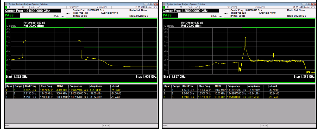
Band25-20MHz-16QAM-26140-1RB#99
