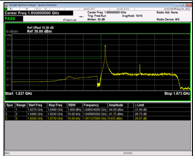
Band25-20MHz-QPSK-26140-100RB#0
