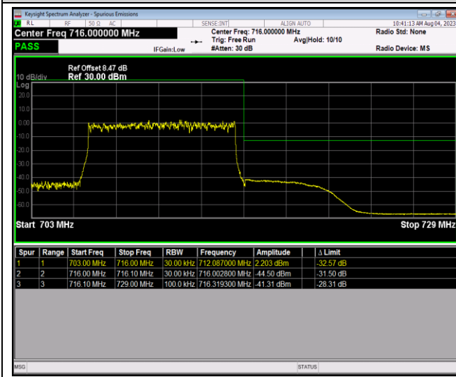
Band17-10MHz-64QAM-23780-1RB#49
