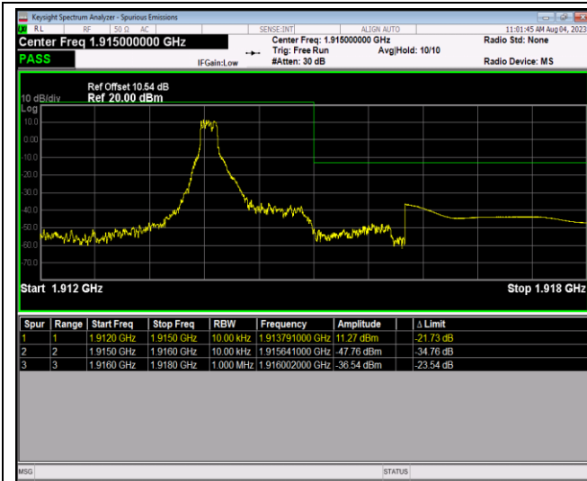
Band25-1.4MHz-64QAM-26683-6RB#0
