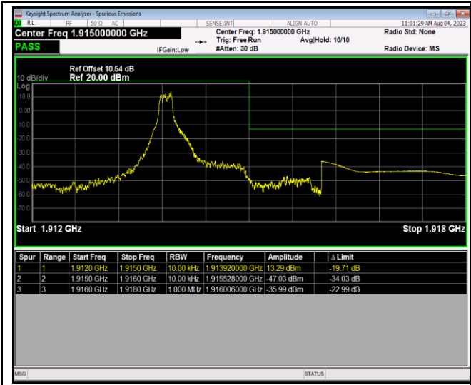
Band25-1.4MHz-16QAM-26683-6RB#0
