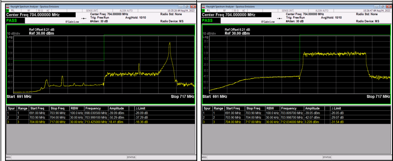
Band17-10MHz-QPSK-23800-1RB#0
