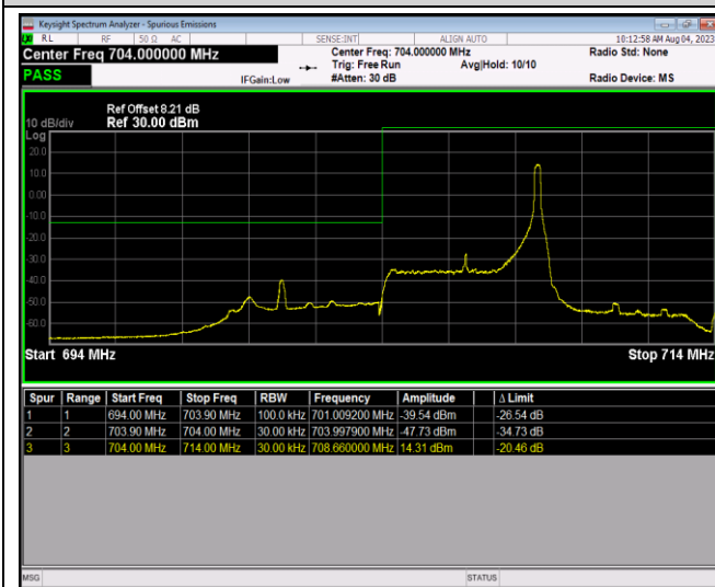
Band17-5MHz-16QAM-23825-1RB#0
