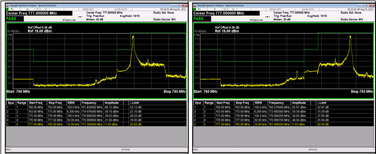
Band13-5MHz-64QAM-23205-25RB#0
