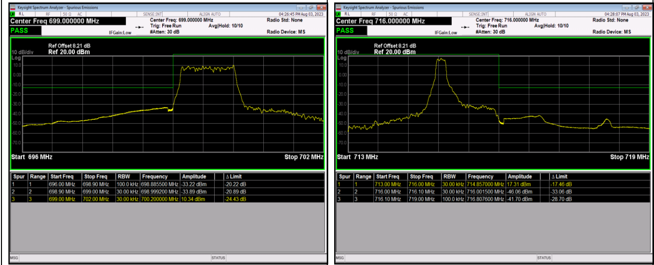
Band12-1.4MHz-16QAM-23173-1RB#5
