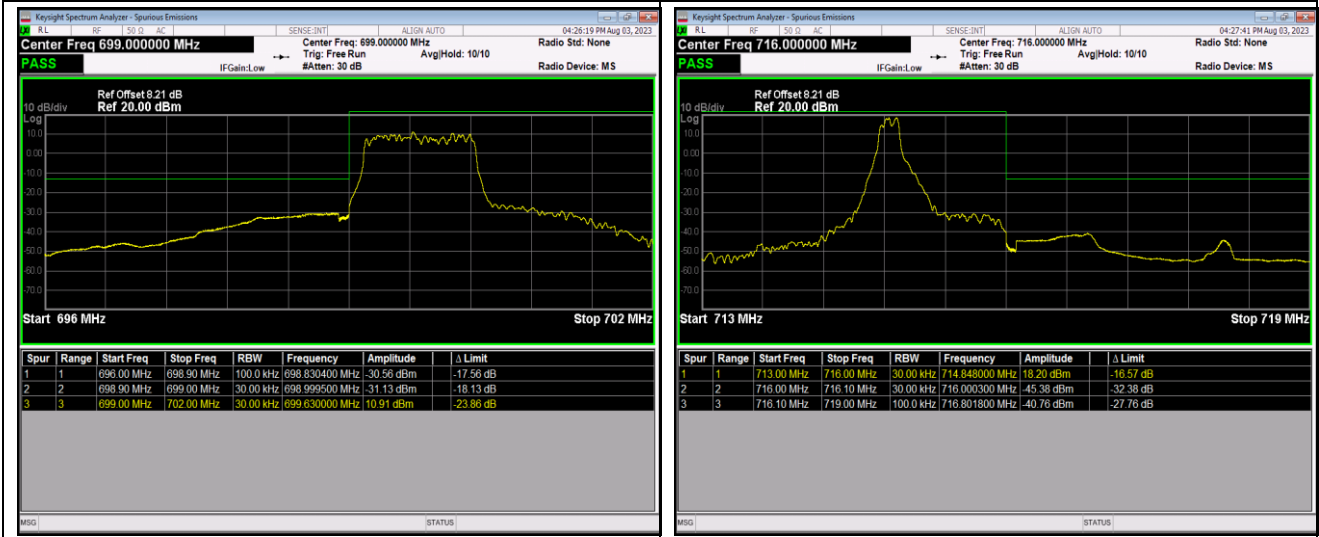
Band12-1.4MHz-QPSK-23173-1RB#5
