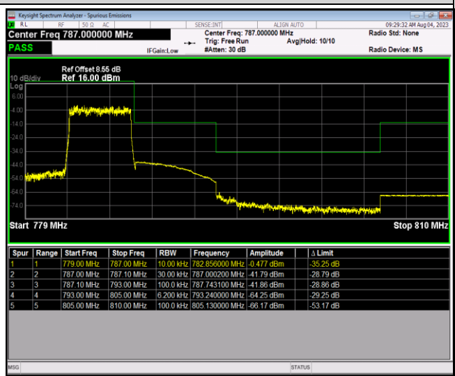
Band13-5MHz-64QAM-23205-1RB#24
