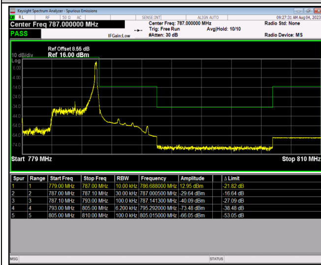
Band13-5MHz-64QAM-23205-1RB#0
