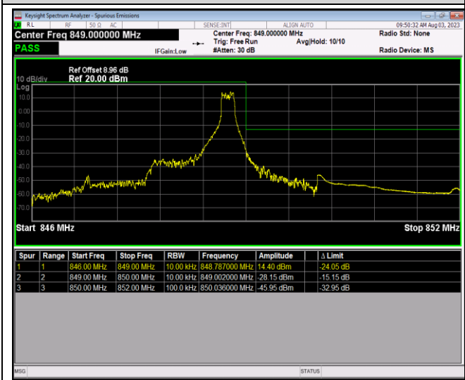
Band5-1.4MHz-16QAM-20407-1RB#0
