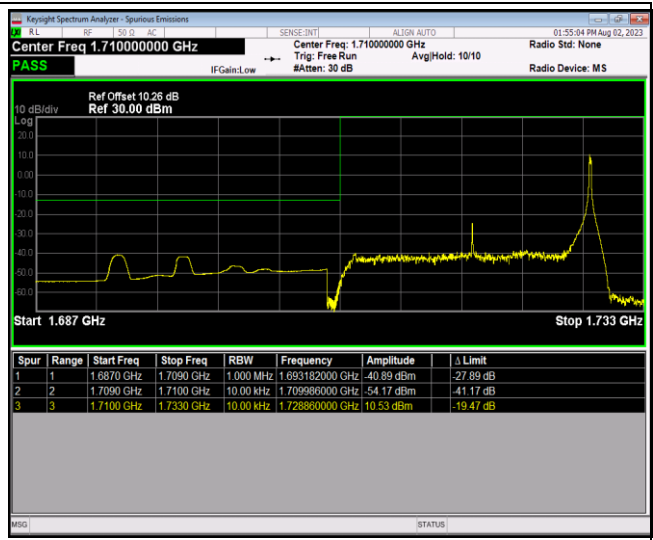
Band4-20MHz-64QAM-20300-1RB#0
