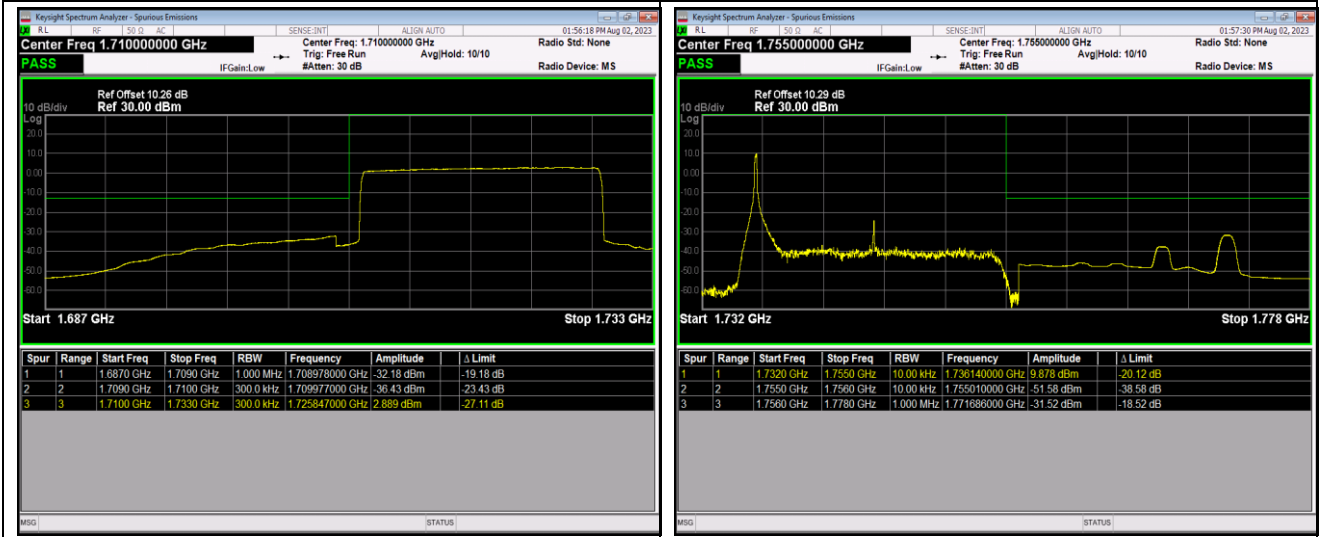
Band4-20MHz-16QAM-20300-1RB#99
