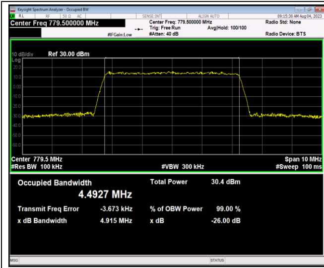
Band13-5MHz-64QAM-23255-25RB#0
