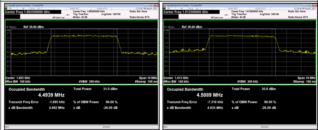
Band25-5MHz-64QAM-26065-25RB#0
