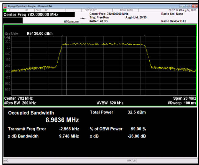
Band13-10MHz-64QAM-23230-50RB#0
