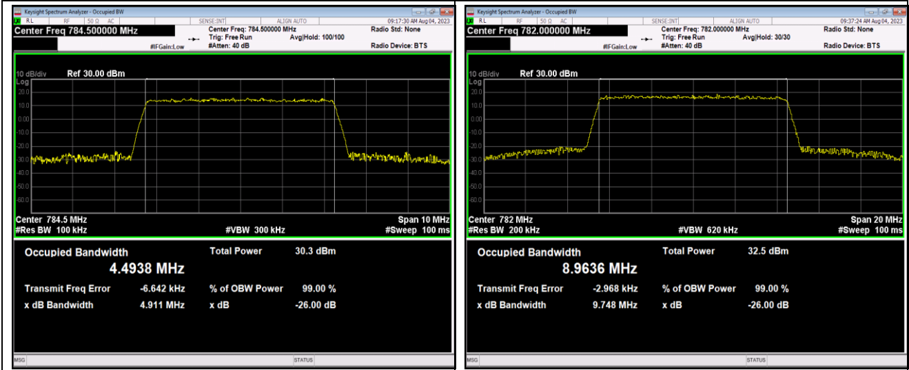
Band13-10MHz-16QAM-23230-50RB#0
