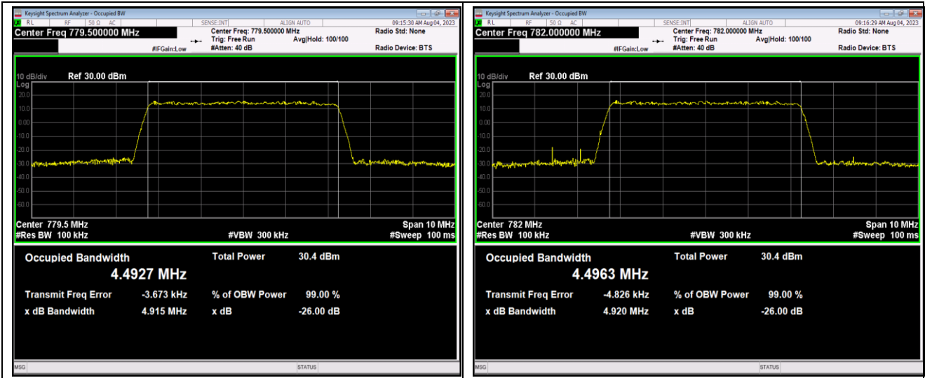
Band13-5MHz-64QAM-23255-25RB#0
