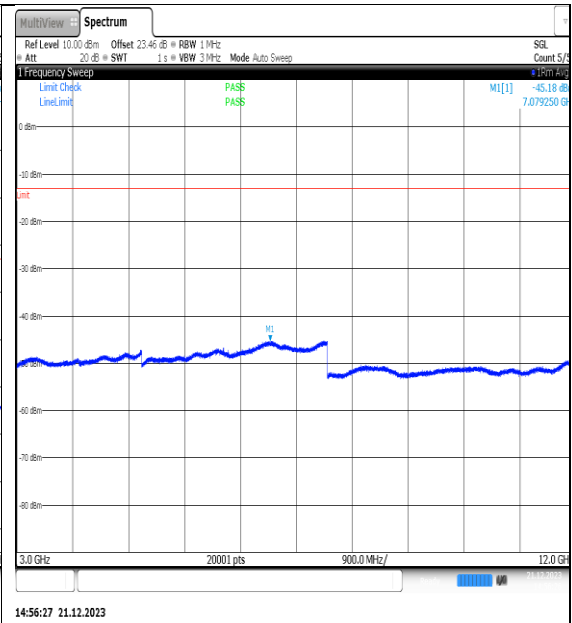
NTVN_N66_PC3_15_40_L_TID4_NS_01_3000_12000_#1
