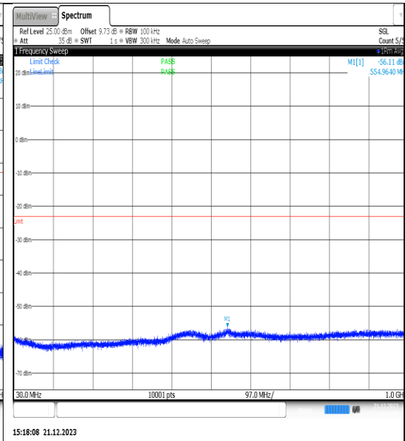
NTVN_N66_PC3_15_40_L_TID11_NS_01_30_10_00_#1
