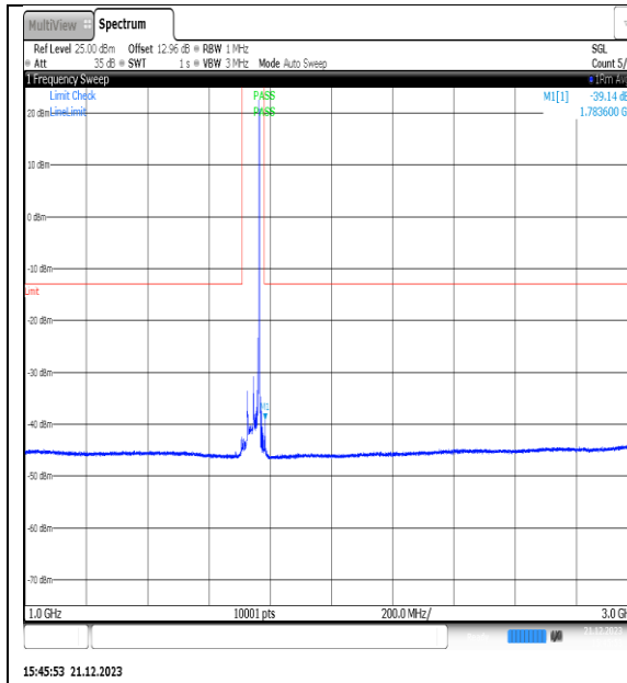
NTNV_N66_PC3_15_40_M_TID3_NS_01_1000_3000_#1
