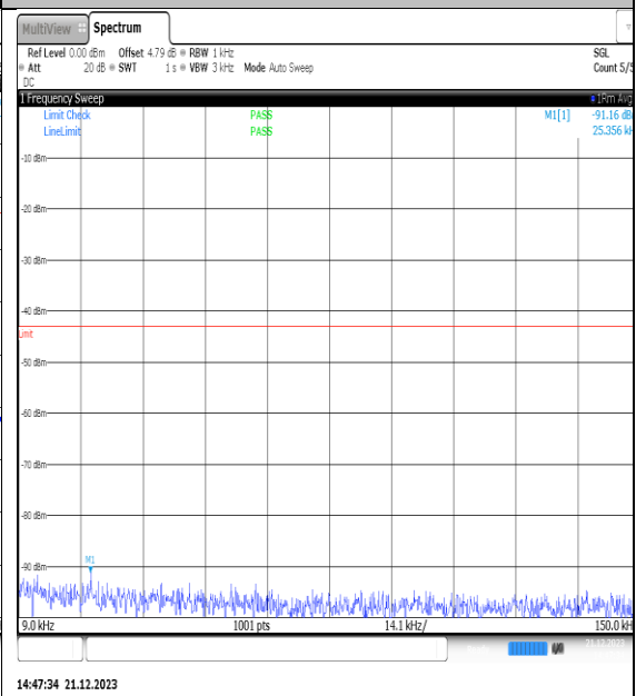
NTVN_N66_PC3_15_40_L_TID1_NS_01_0.009_0.15_#1
