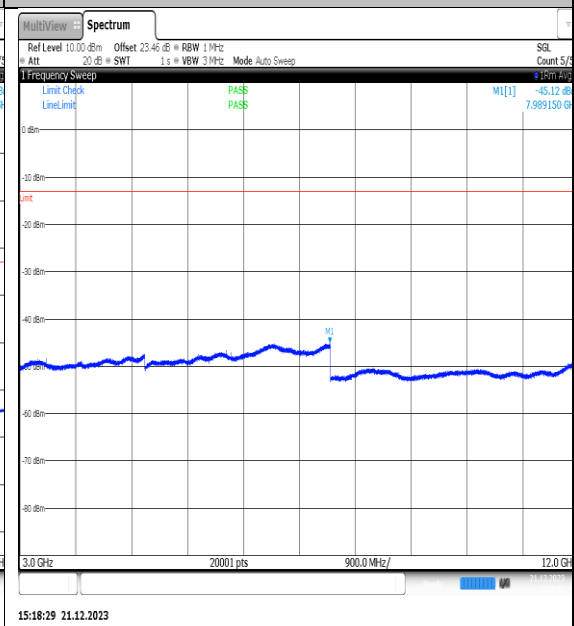
NTVN_N66_PC3_15_40_L_TID11_NS_01_3000_12000_#1
