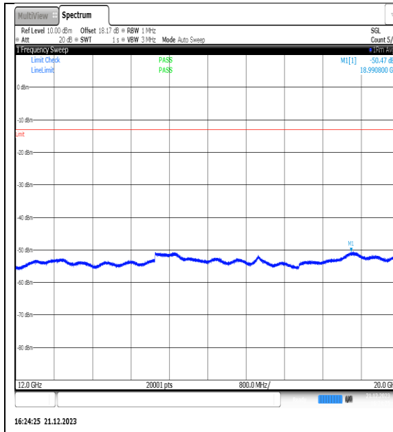
NTVN_N66_PC3_15_40_M_TID8_NS_01_12000_20000_#1
