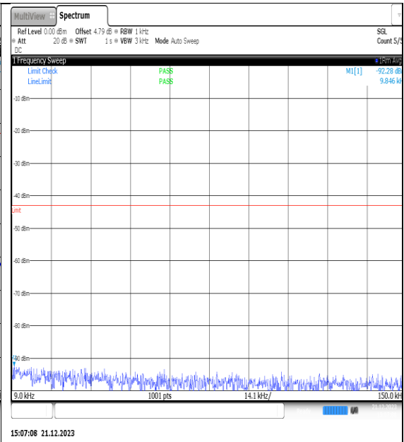
NTVN_N66_PC3_15_40_L_TID8_NS_01_0.009_0.15_#1
