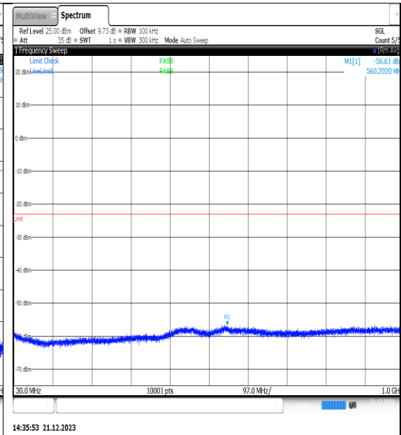
NTNV_N66_PC3_15_30_H_TID12_NS_01_30_1000_#1
