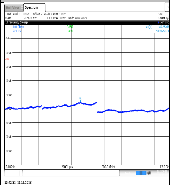
NTNV_N66_PC3_15_40_M_TID2_NS_01_3000_12000_#1
