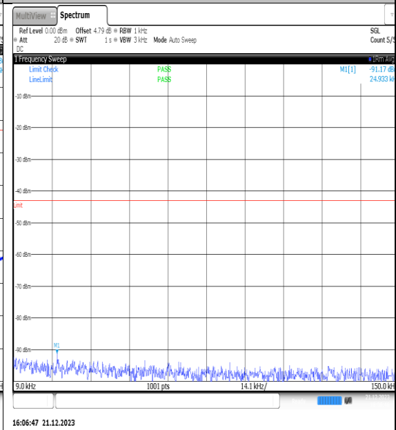
NTVN_N66_PC3_15_40_M_TID6_NS_01_0.009_0.15_#1
