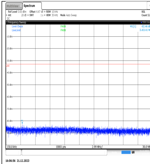
NTVN_N66_PC3_15_40_M_TID6_NS_01_0.15_3_0_#1
