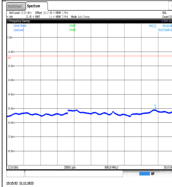
NTVN_N66_PC3_15_40_L_TID10_NS_01_12000_20000_#1
