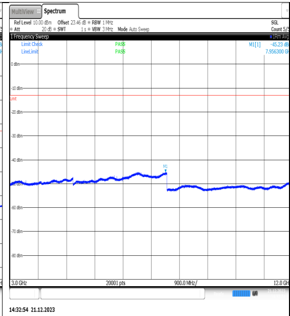
NTVN_N66_PC3_15_30_H_TID11_NS_01_3000_12000_#1
