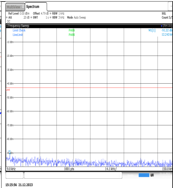
NTNV_N66_PC3_15_40_L_TID14_NS_01_0.009_0.15_#1
