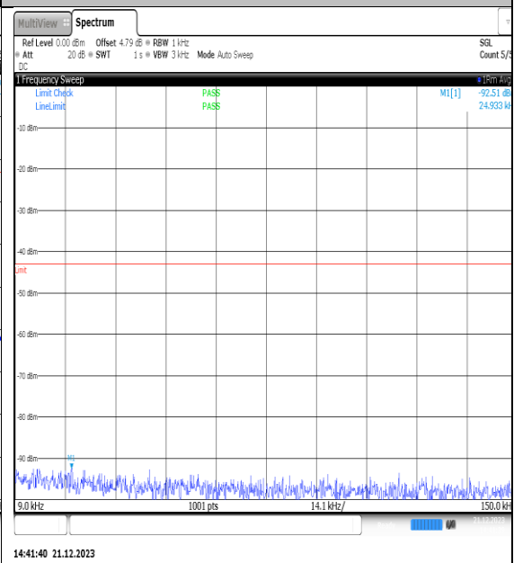
NTVN_N66_PC3_15_30_H_TID14_NS_01_0.009_0.15_#1
