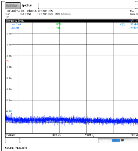
NTVN_N66_PC3_15_40_L_TID5_NS_01_0.15_3_0_#1
