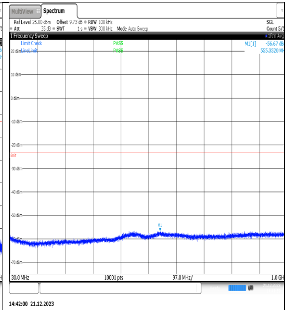
NTVN_N66_PC3_15_30_H_TID14_NS_01_30_1000_3000_#1
