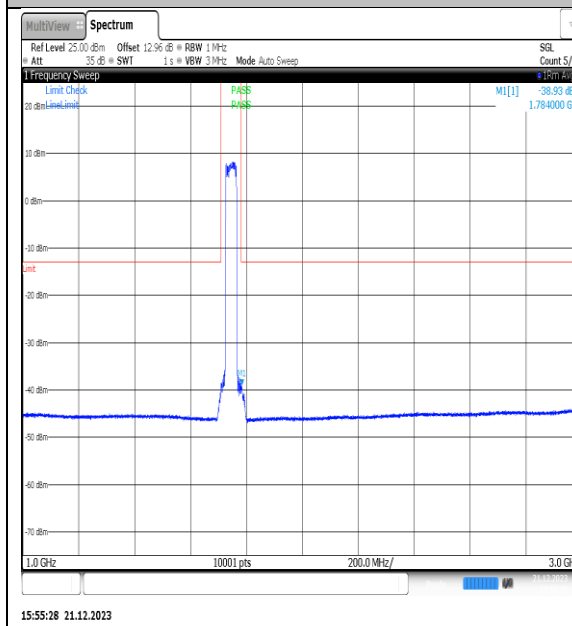
NTNV_N66_PC3_15_40_M_TID4_NS_01_1000_3000_#1
