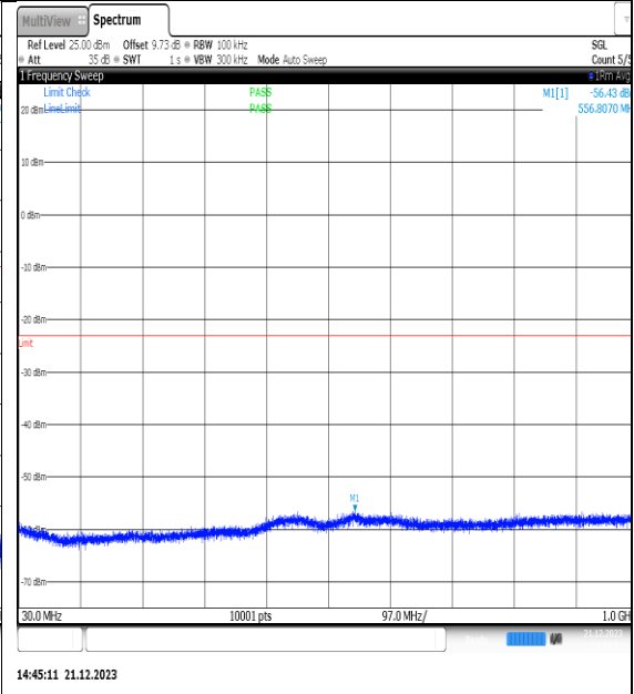
NTVN_N66_PC3_15_30_H_TID15_NS_01_30_1000_#1
