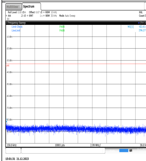
NTNV_N66_PC3_15_40_L_TID6_NS_01_0.15_30_#1
