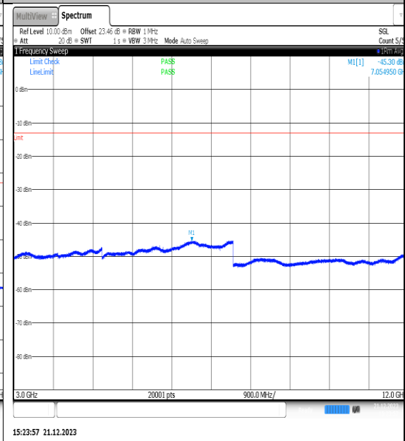
NTNV_N66_PC3_15_40_L_TID13_NS_01_3000_12000_#1
