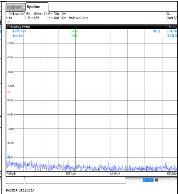
NTVN_N66_PC3_15_40_M_TID5_NS_01_0.009_0.15_#1
