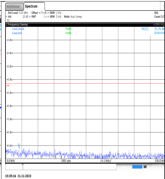
NTVN_N66_PC3_15_40_M_TID1_NS_01_0.009_0.15_#1
