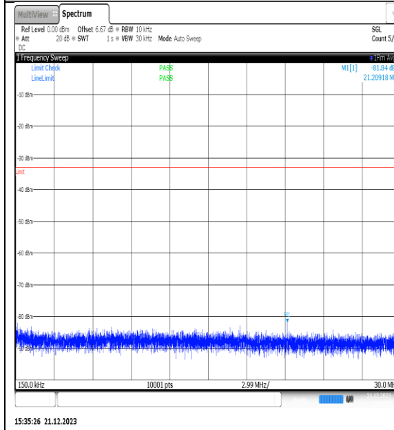
NTVN_N66_PC3_15_40_M_TID1_NS_01_0.15_30_#1
