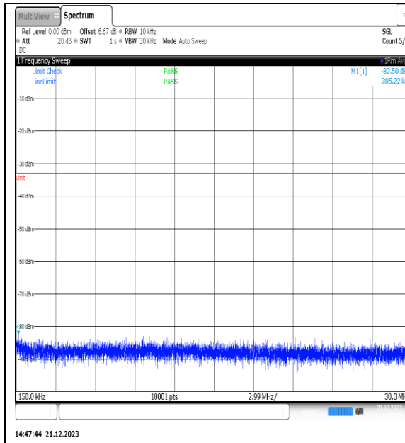
NTVN_N66_PC3_15_40_L_TID1_NS_01_0.15_3_0_#1
