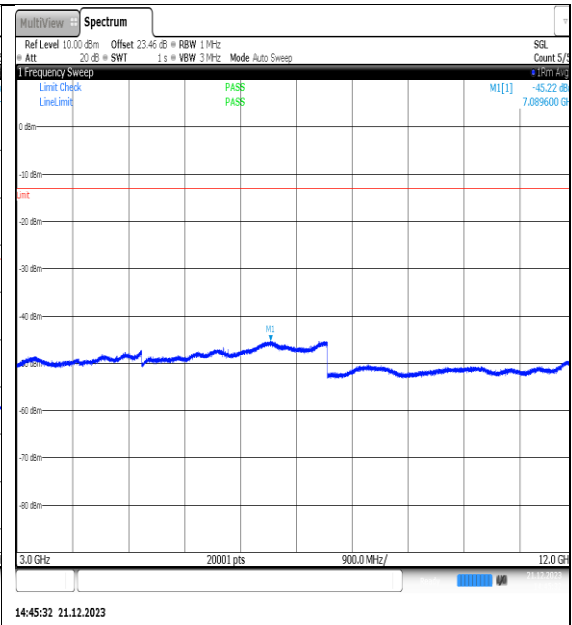
NTVN_N66_PC3_15_30_H_TID15_NS_01_3000_12000_#1
