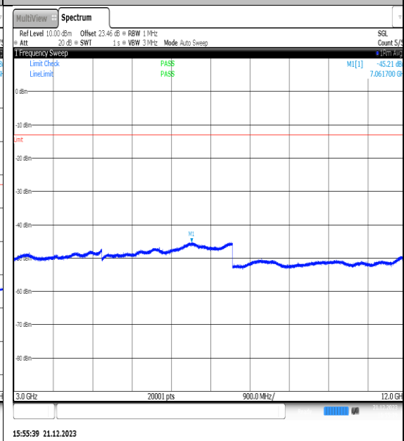
NTNV_N66_PC3_15_40_M_TID4_NS_01_3000_12000_#1
