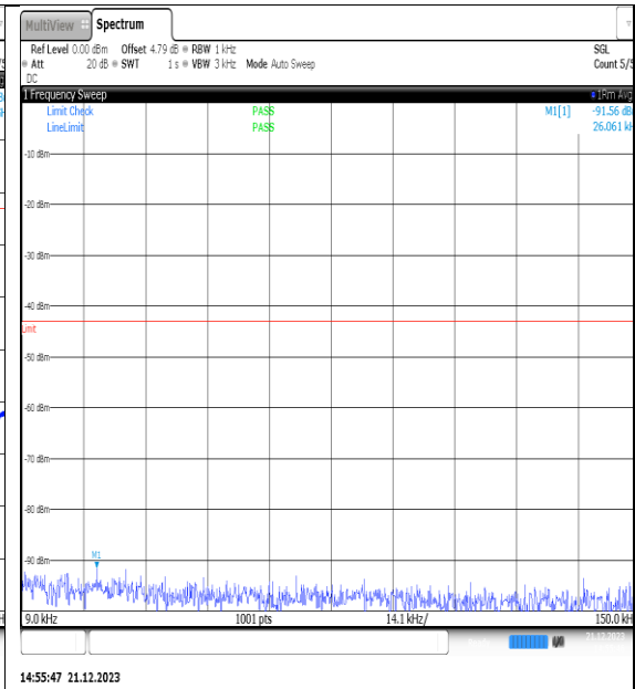
NTVN_N66_PC3_15_40_L_TID4_NS_01_0.009_0.15_#1
