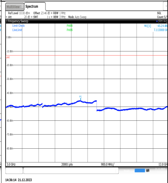
NTNV_N66_PC3_15_30_H_TID12_NS_01_3000_12000_#1
