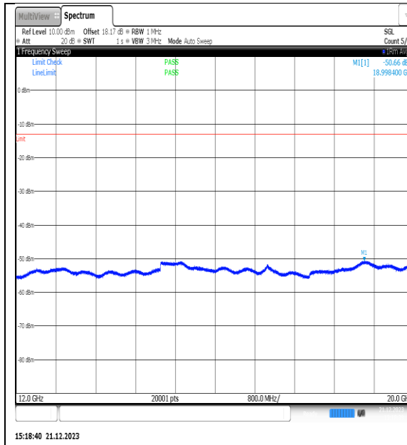
NTNV_N66_PC3_15_40_L_TID11_NS_01_12000_20000_#1
