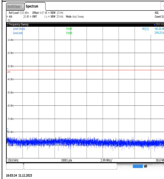
NTVN_N66_PC3_15_40_M_TID5_NS_01_0.15_30_#1
