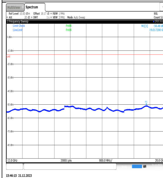
NTNV_N66_PC3_15_40_M_TID3_NS_01_12000_20000_#1
