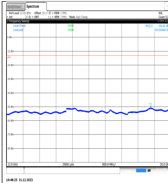
NTNV_N66_PC3_15_40_L_TID1_NS_01_12000_20000_#1
