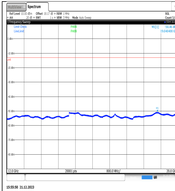
NTVN_N66_PC3_15_40_M_TID4_NS_01_12000_20000_#1
