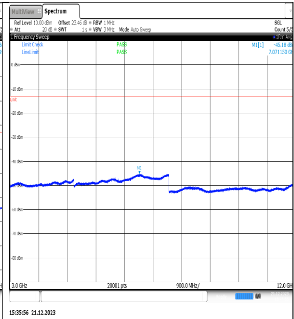
NTVN_N66_PC3_15_40_M_TID1_NS_01_3000_12000_#1
