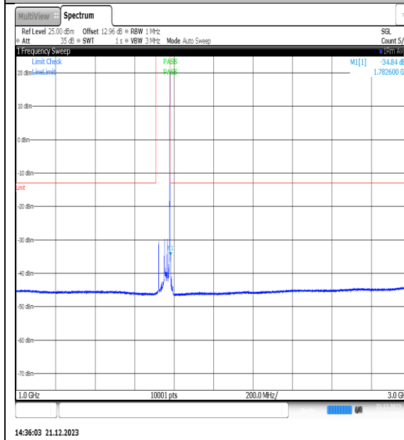
NTNV_N66_PC3_15_30_H_TID12_NS_01_1000_3000_#1
