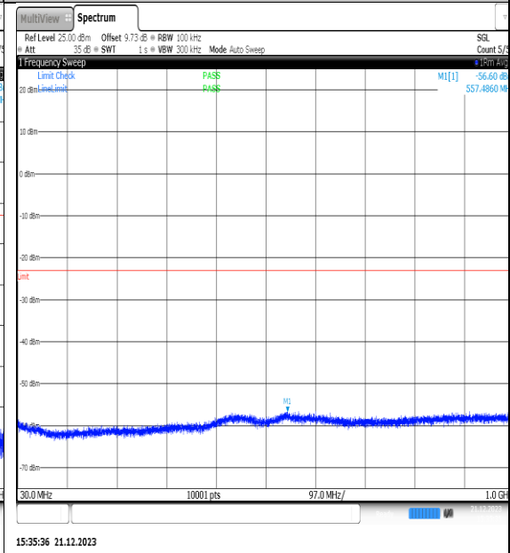
NTVN_N66_PC3_15_40_M_TID1_NS_01_30_100_#1
