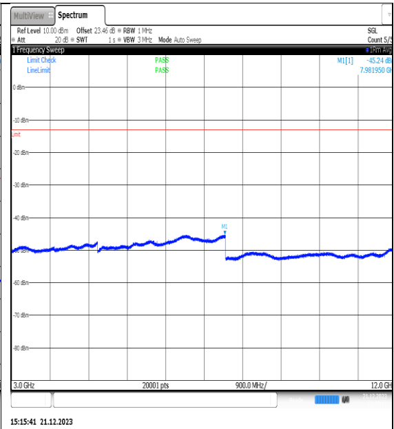
NTVN_N66_PC3_15_40_L_TID10_NS_01_3000_12000_#1
