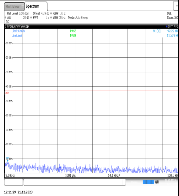
NTNV_N66_PC3_15_30_L_TID6_NS_01_0.009_0.15_#1
