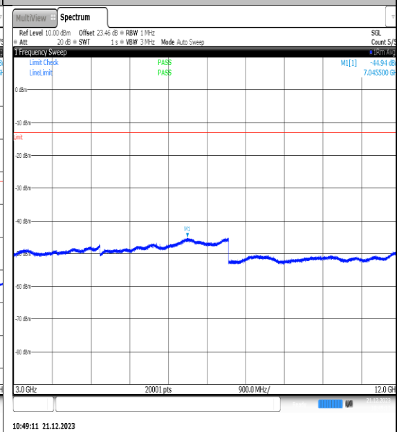
NTNV_N66_PC3_15_25_H_TID1_NS_01_3000_1 2000_#1
