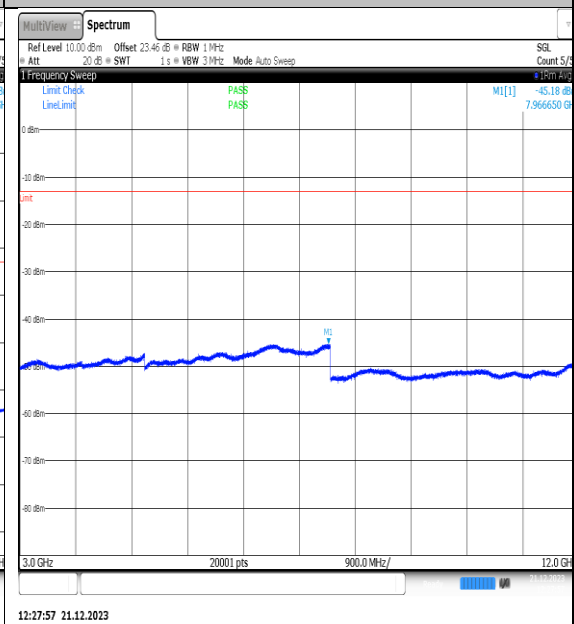
NTNV_N66_PC3_15_30_L_TID10_NS_01_3000_12000_#1
