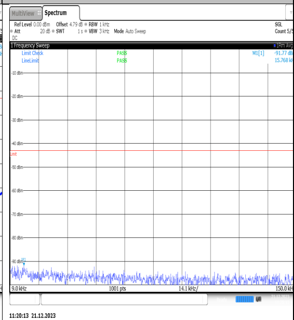
NTVN_N66_PC3_15_25_H_TID7_NS_01_0.009_0.15_#1
