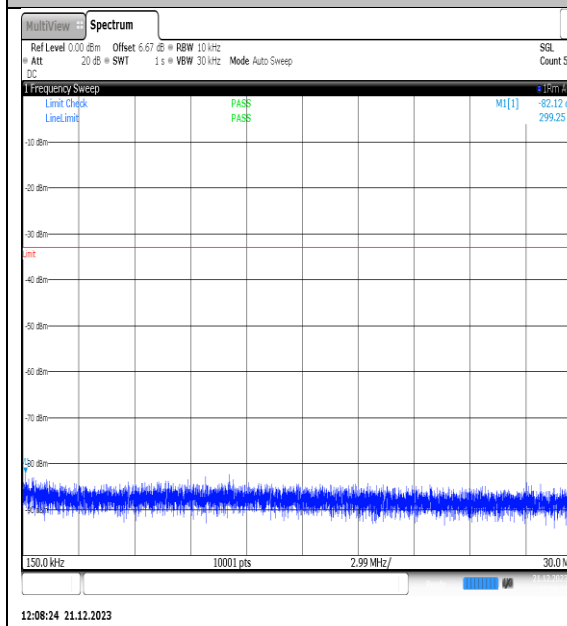
NTNV_N66_PC3_15_30_L_TID5_NS_01_0.15_3_0_#1
