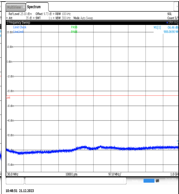
NTNV_N66_PC3_15_25_H_TID1_NS_01_30_100 0_#1
