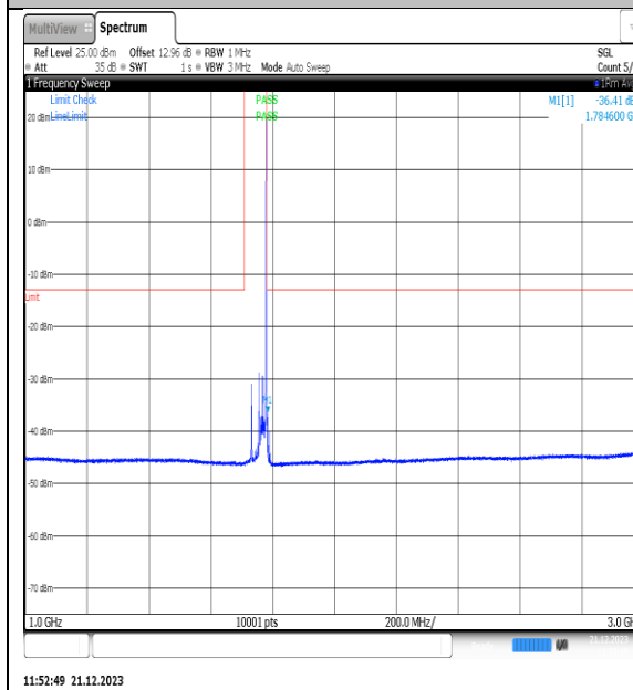
NTNV_N66_PC3_15_25_H_TID15_NS_01_1000_3000_#1
