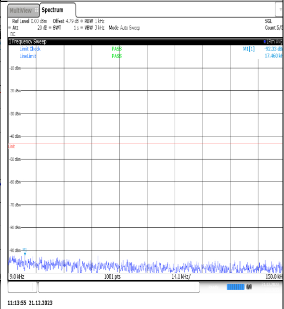
NTVN_N66_PC3_15_25_H_TID5_NS_01_0.009_0.15_#1
