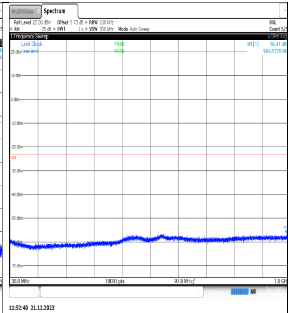
NTNV_N66_PC3_15_25_H_TID15_NS_01_30_10_00_#1
