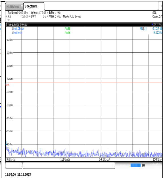
NTVN_N66_PC3_15_25_H_TID10_NS_01_0.009_0.15_#1
