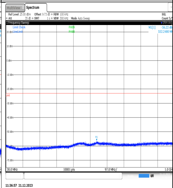
NTVN_N66_PC3_15_25_H_TID12_NS_01_30_1000_#1
