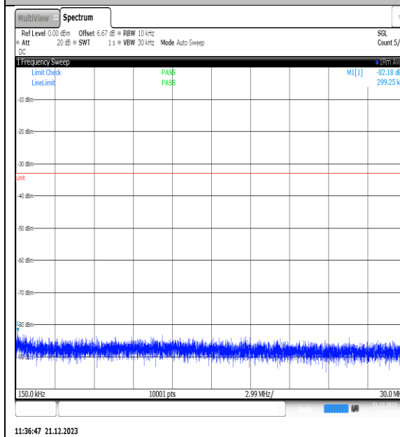
NTVN_N66_PC3_15_25_H_TID12_NS_01_0.15_30_#1
