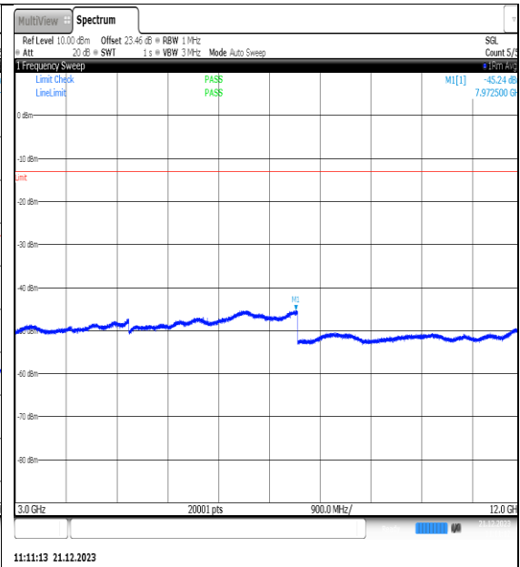
NTVN_N66_PC3_15_25_H_TID4_NS_01_3000_12000_#1
