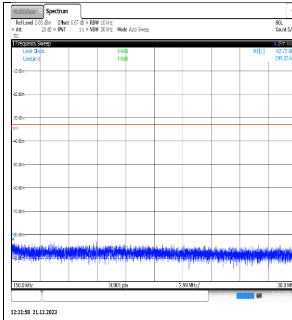
NTVN_N66_PC3_15_30_L_TID8_NS_01_0.15_3_0_#1
