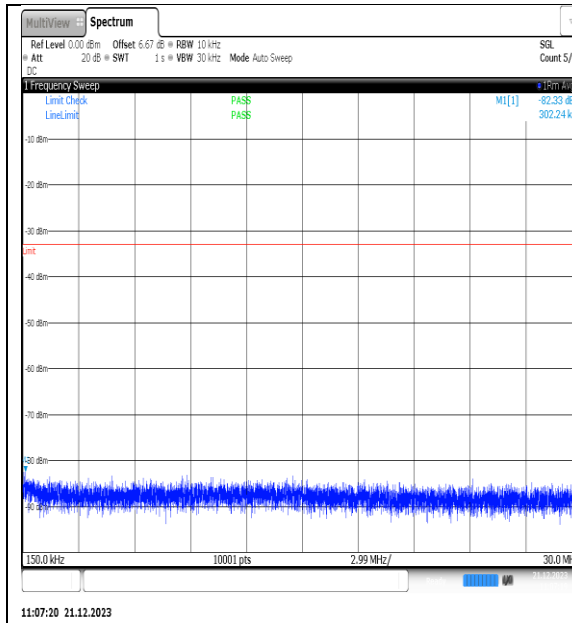
NTNV_N66_PC3_15_25_H_TID3_NS_01_0.15_3_0_#1
