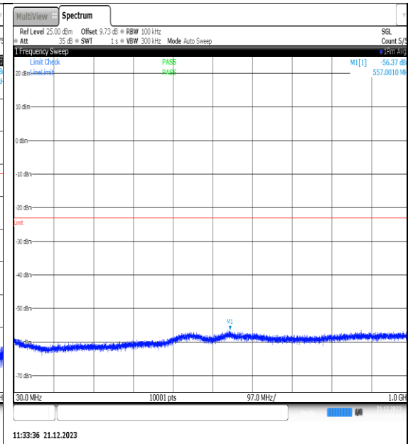
NTNV_N66_PC3_15_25_H_TID11_NS_01_30_10_00_#1
