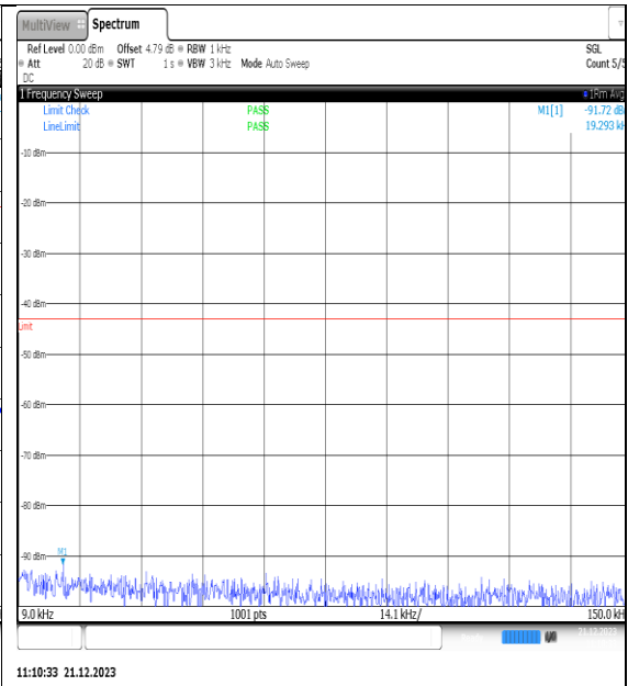
NTNV_N66_PC3_15_25_H_TID4_NS_01_0.009_0.15_#1
