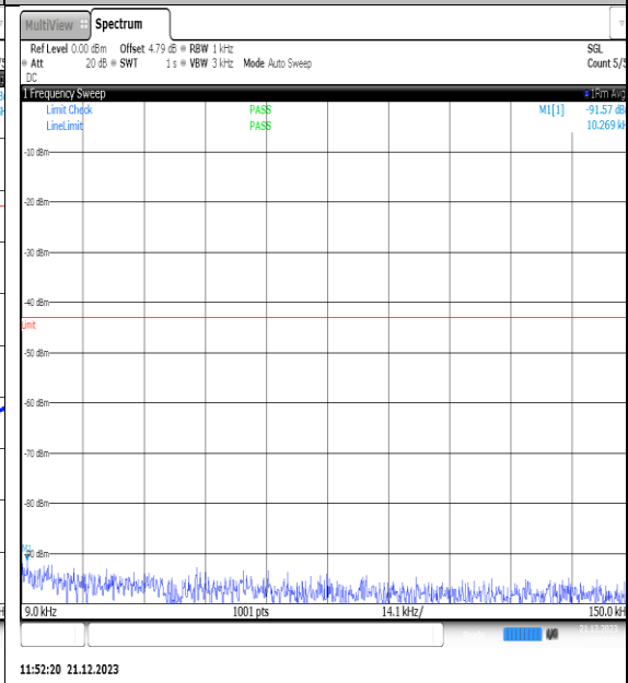
NTVN_N66_PC3_15_25_H_TID15_NS_01_0.009_0.15_#1
