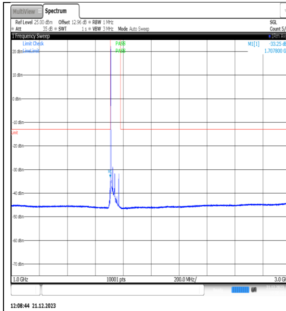
NTNV_N66_PC3_15_30_L_TID5_NS_01_1000_3000_#1
