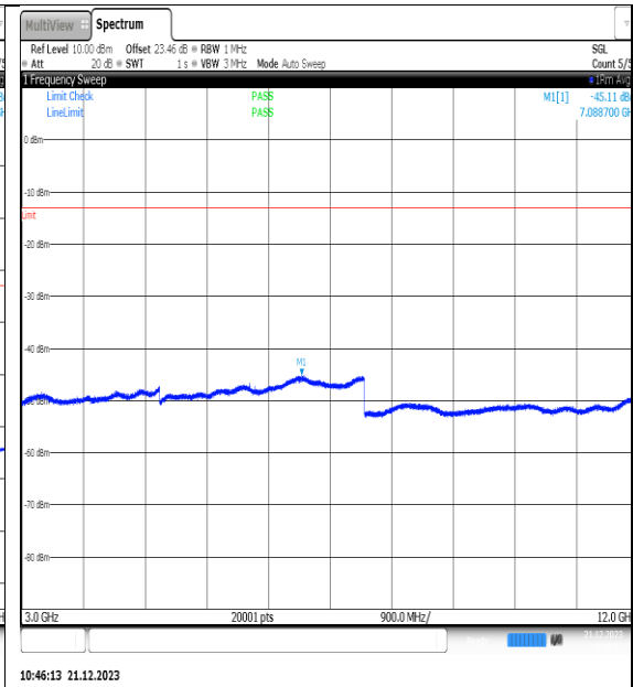
NTVN_N66_PC3_15_25_M_TID15_NS_01_3000_12000_#1
