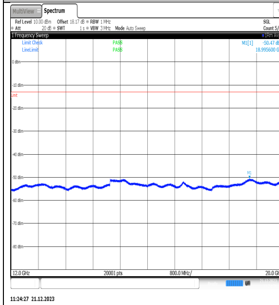
NTVN_N66_PC3_15_25_H_TID8_NS_01_12000_20000_#1
