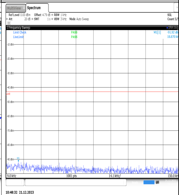
NTVN_N66_PC3_15_25_H_TID1_NS_01_0.009_0.15_#1
