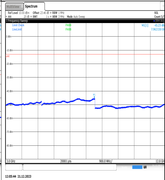
NTVN_N66_PC3_15_30_L_TID4_NS_01_3000_1_2000_#1
