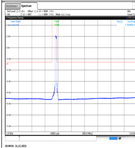
NTNV_N66_PC3_15_25_H_TID1_NS_01_1000_3 000_#1
