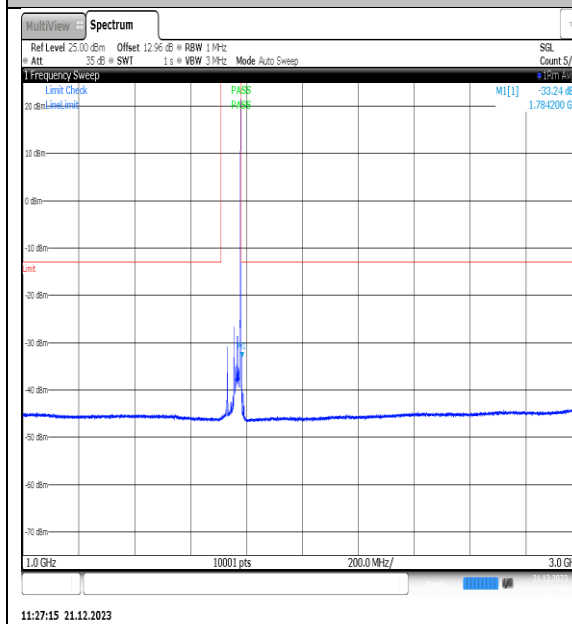
NTNV_N66_PC3_15_25_H_TID9_NS_01_1000_3_000_#1
