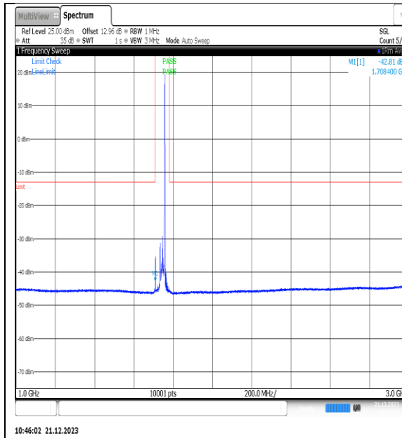
NTVN_N66_PC3_15_25_M_TID15_NS_01_1000_3000_#1
