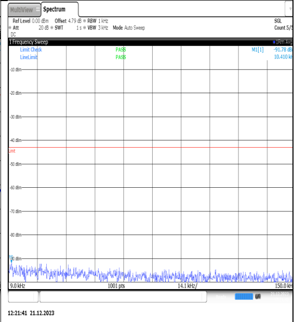
NTNV_N66_PC3_15_30_L_TID8_NS_01_0.009_0.15_#1
