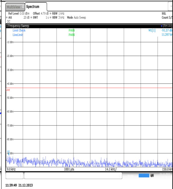
NTVN_N66_PC3_15_25_H_TID13_NS_01_0.009_0.15_#1
