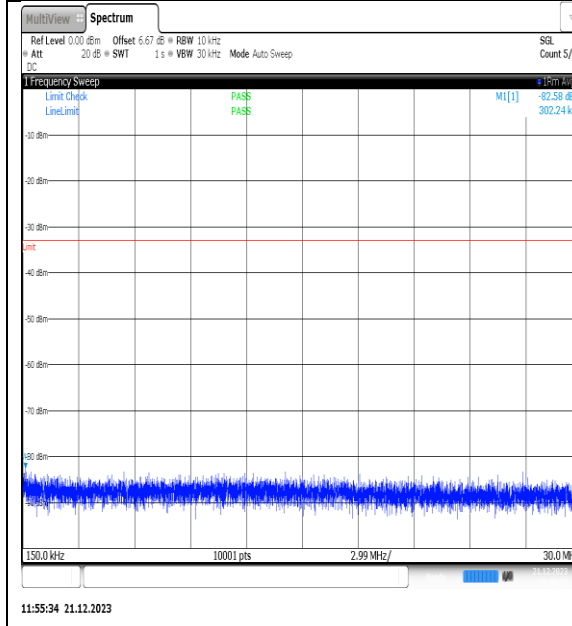
NTVN_N66_PC3_15_30_L_TID1_NS_01_0.15_3_0_#1
