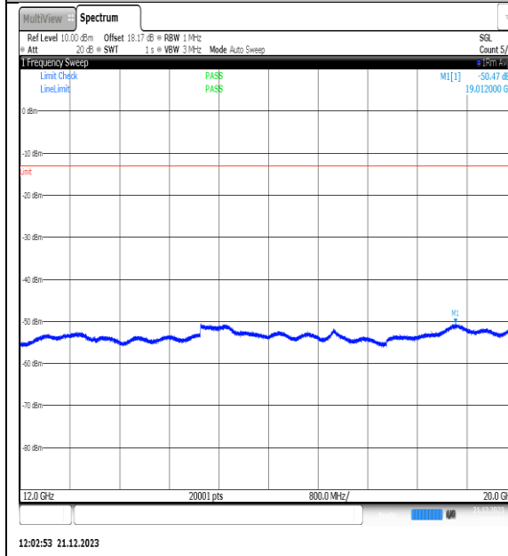
NTVN_N66_PC3_15_30_L_TID3_NS_01_12000_20000_#1
