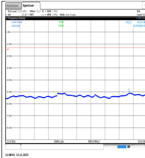
NTNV_N66_PC3_15_25_H_TID3_NS_01_12000_20000_#1
