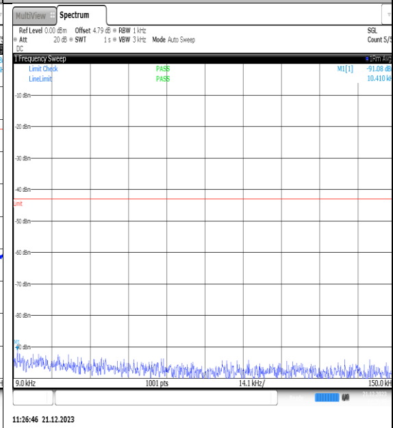
NTVN_N66_PC3_15_25_H_TID9_NS_01_0.009_0.15_#1
