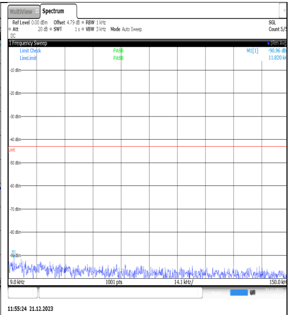
NTVN_N66_PC3_15_30_L_TID1_NS_01_0.009_0.15_#1
