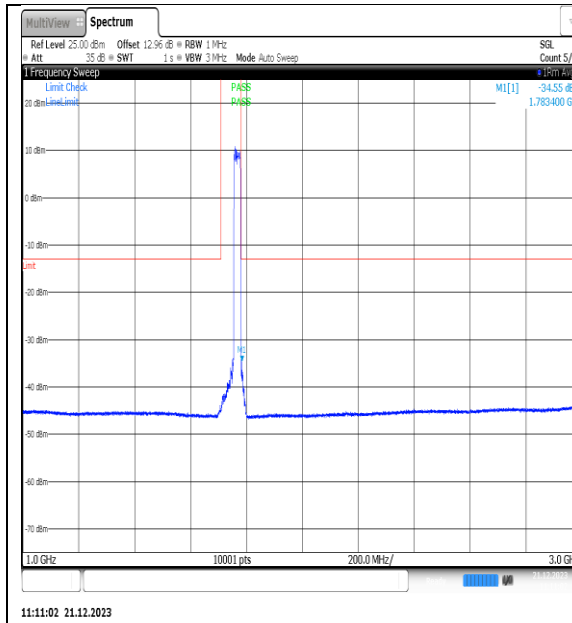
NTVN_N66_PC3_15_25_H_TID4_NS_01_1000_3000_#1
