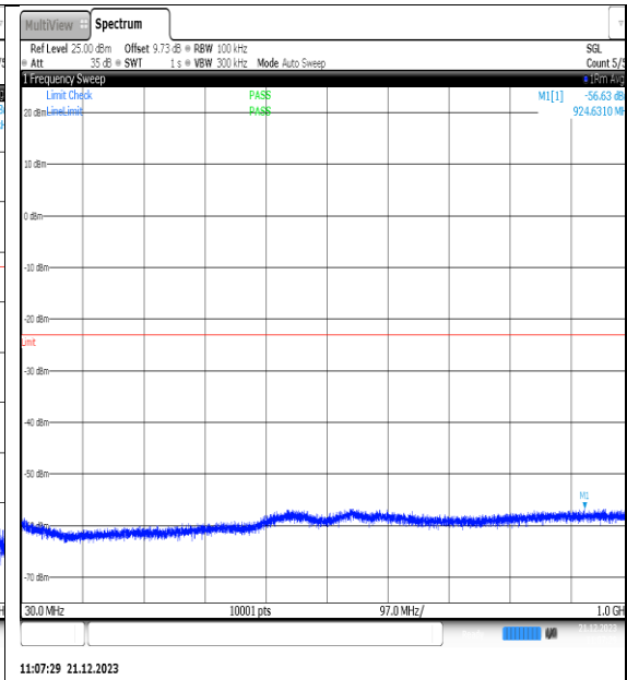
NTNV_N66_PC3_15_25_H_TID3_NS_01_30_100_0_#1
