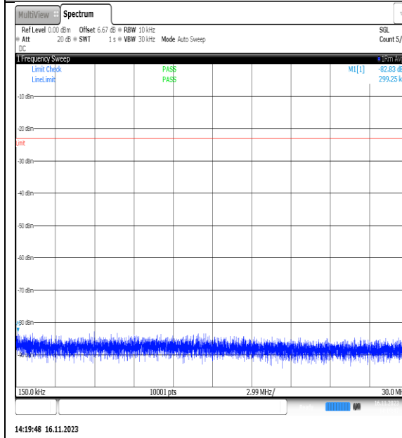
NTVN_N5_PC3_15_5_H_TID15_NS_01_0.15_30_#1
