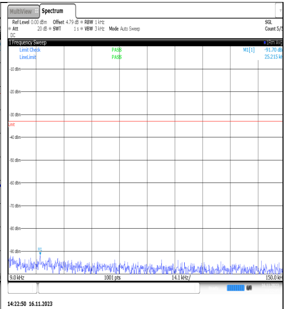
NTVN_N5_PC3_15_5_H_TID17_NS_01_0.009_0_15_#1
