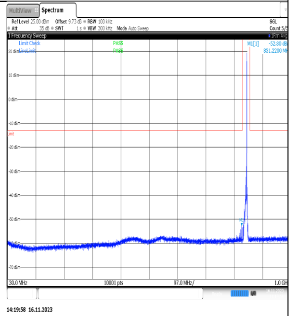
NTVN_N5_PC3_15_5_H_TID15_NS_01_30_1000_#1
