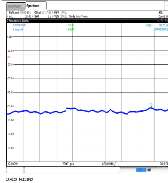
NTVN_N5_PC3_15_10_L_TID8_NS_01_12000_2_0000_#1
