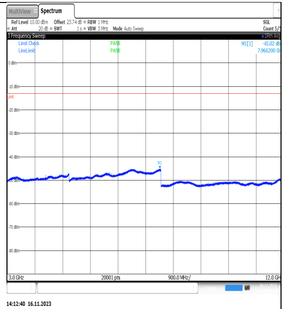
NTVN_N5_PC3_15_5_H_TID9_NS_01_3000_120_00_#1
