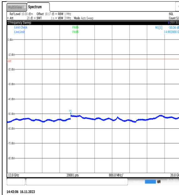
NTVN_N5_PC3_15_10_L_TID5_NS_01_12000_2_0000_#1
