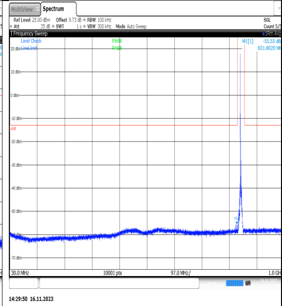
NTVN_N5_PC3_15_5_H_TID23_NS_01_30_1000_#1
