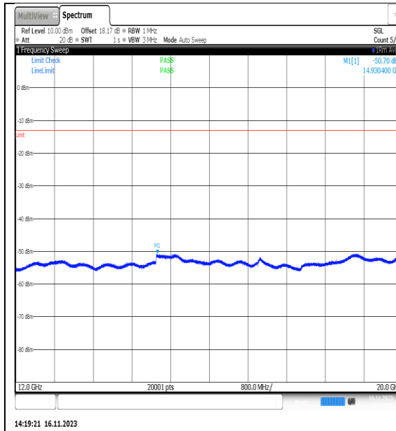
NTVN_N5_PC3_15_5_H_TID14_NS_01_12000_2_0000_#1
