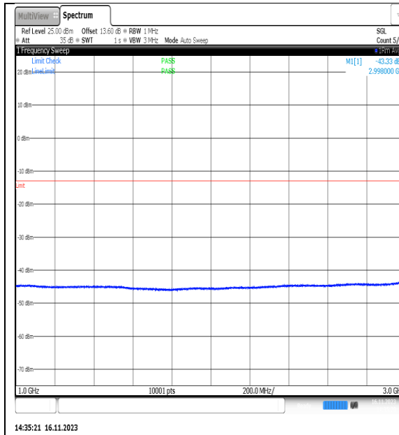
NTVN_N5_PC3_15_5_H_TID27_NS_01_1000_30_00_#1
