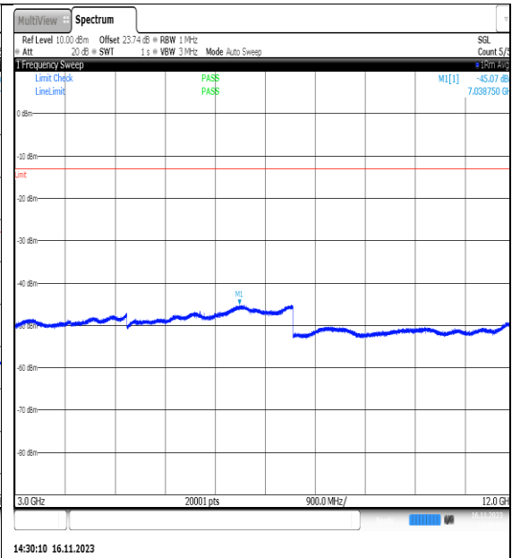
NTVN_N5_PC3_15_5_H_TID23_NS_01_3000_12 000_#1
