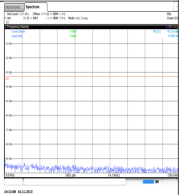
NTVN_N5_PC3_15_5_H_TID10_NS_01_0.009_0_15_#1
