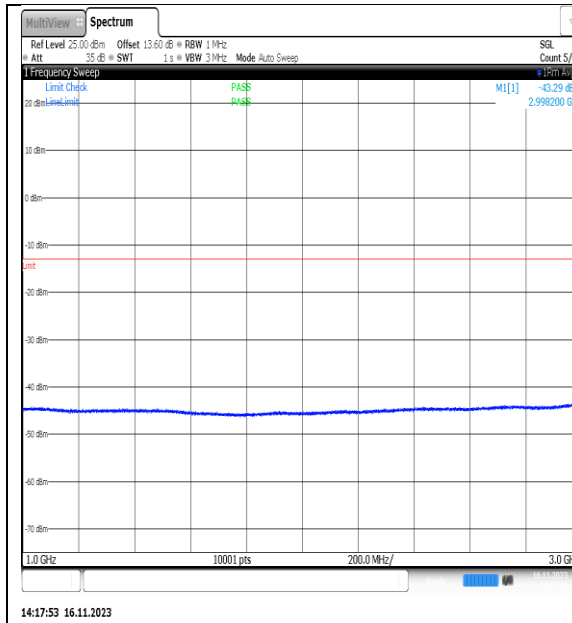
NTVN_N5_PC3_15_5_H_TID13_NS_01_1000_30_00_#1
