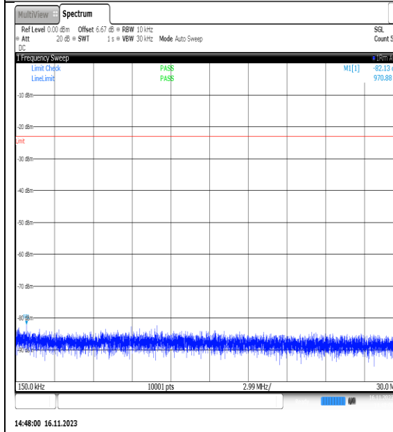
NTNV_N5_PC3_15_10_L_TID10_NS_01_0.15_3_0_#1
