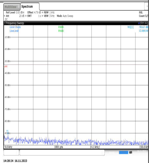
NTVN_N5_PC3_15_5_H_TID22_NS_01_0.009_0. 15_#1
