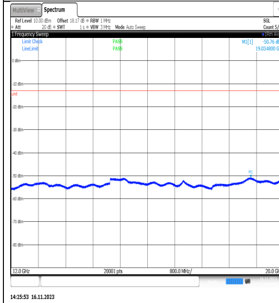
NTVN_N5_PC3_15_5_H_TID19_NS_01_12000_2_0000_#1
