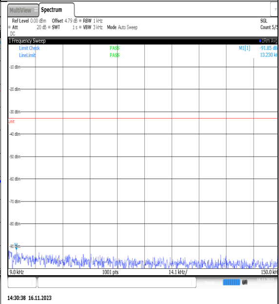
NTVN_N5_PC3_15_5_H_TID24_NS_01_0.009_0. 15_#1
