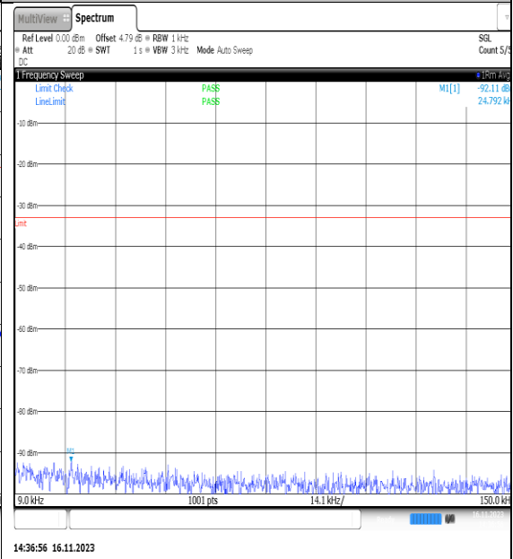
NTVN_N5_PC3_15_10_L_TID1_NS_01_0.009_0_15_#1
