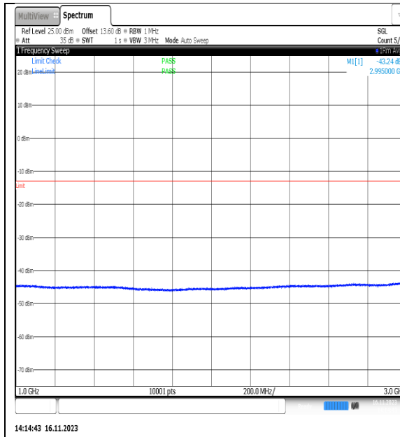
NTVN_N5_PC3_15_5_H_TID11_NS_01_1000_30_00_#1
