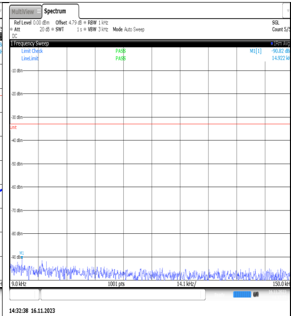
NTVN_N5_PC3_15_5_H_TID25_NS_01_0.009_0_15_#1
