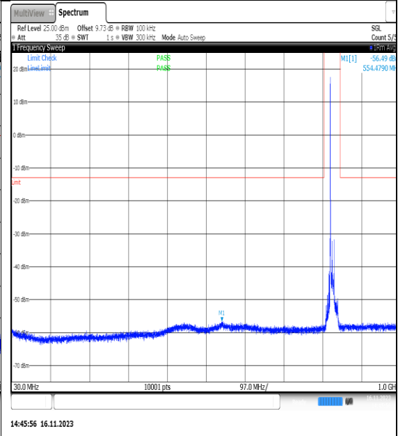
NTVN_N5_PC3_15_10_L_TID8_NS_01_30_1000_#1
