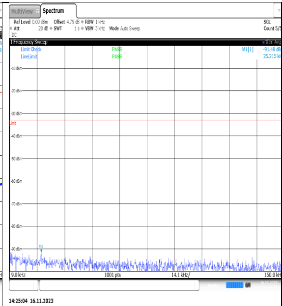
NTVN_N5_PC3_15_5_H_TID19_NS_01_0.009_0_15_#1
