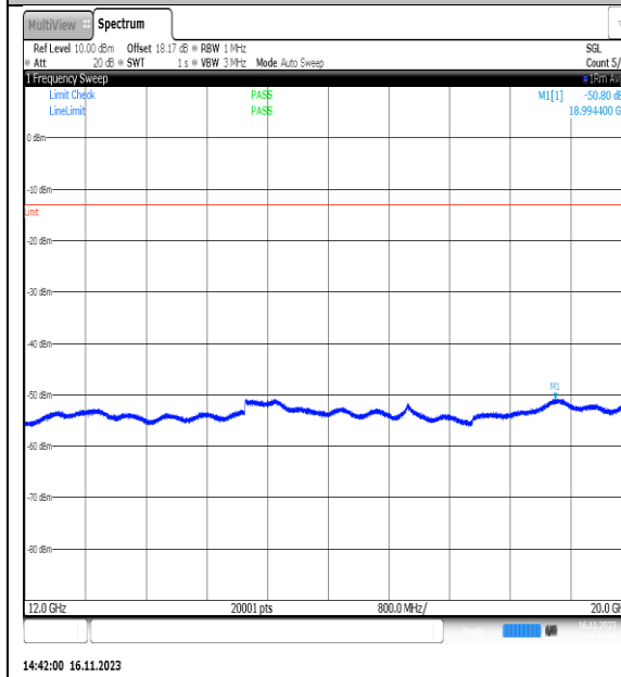
NTVN_N5_PC3_15_10_L_TID4_NS_01_12000_2_0000_#1
