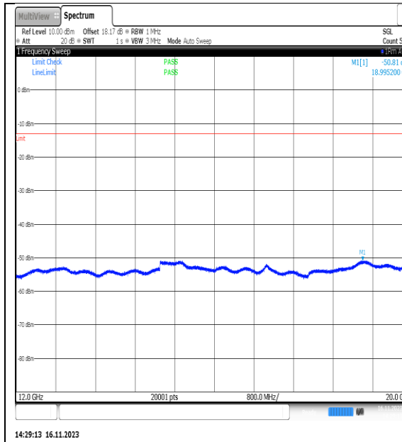
NTVN_N5_PC3_15_5_H_TID22_NS_01_12000_2_0000_#1
