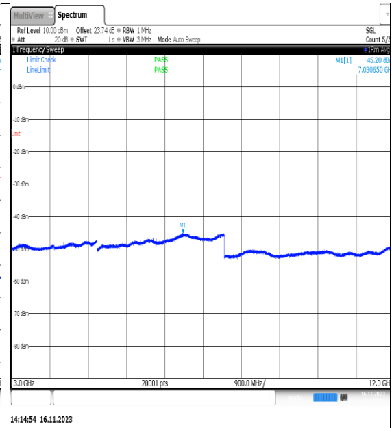
NTVN_N5_PC3_15_5_H_TID11_NS_01_3000_12_000_#1
