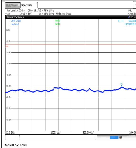
NTVN_N5_PC3_15_5_H_TID11_NS_01_12000_2_0000_#1
