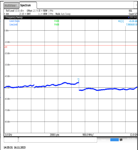
NTVN_N5_PC3_15_5_H_TID27_NS_01_3000_12_000_#1
