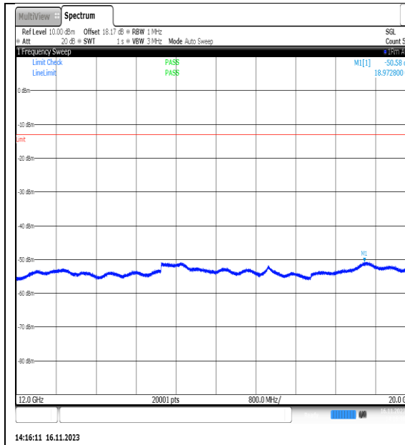
NTVN_N5_PC3_15_5_H_TID12_NS_01_12000_2_0000_#1
