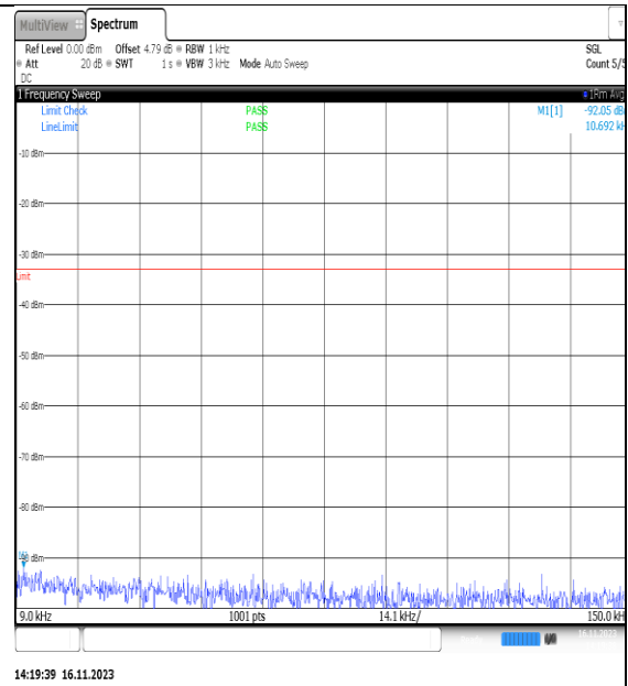
NTVN_N5_PC3_15_5_H_TID15_NS_01_0.009_0_15_#1
