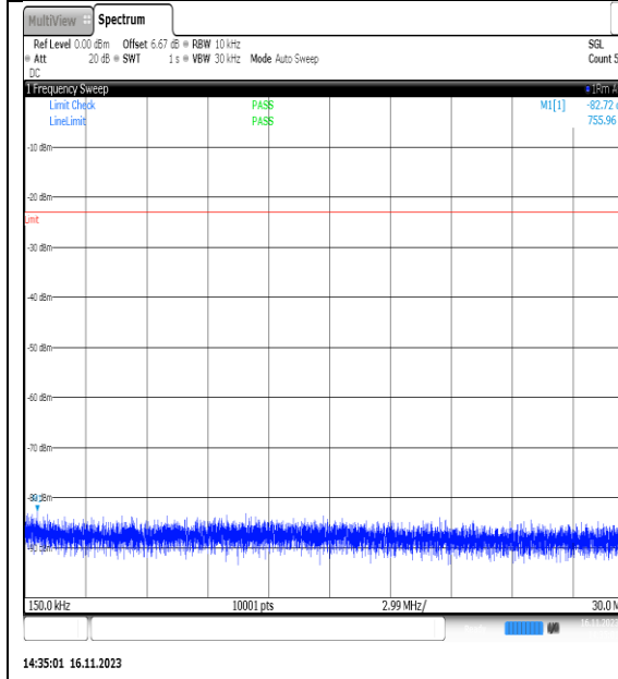
NTVN_N5_PC3_15_5_H_TID27_NS_01_0.15_30_#1
