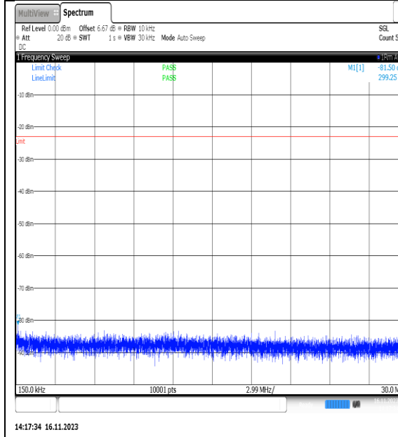
NTVN_N5_PC3_15_5_H_TID13_NS_01_0.15_30_#1
