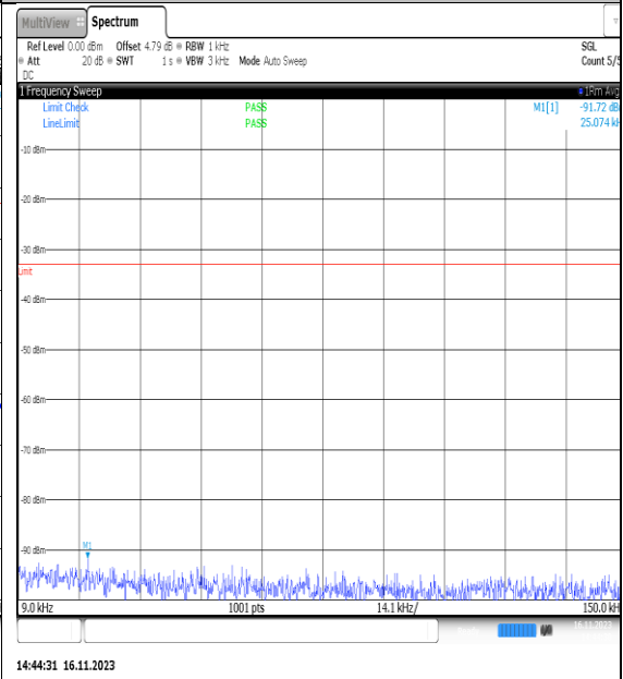
NTVN_N5_PC3_15_10_L_TID7_NS_01_0.009_0.15_#1
