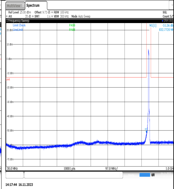
NTVN_N5_PC3_15_5_H_TID13_NS_01_30_1000_#1
