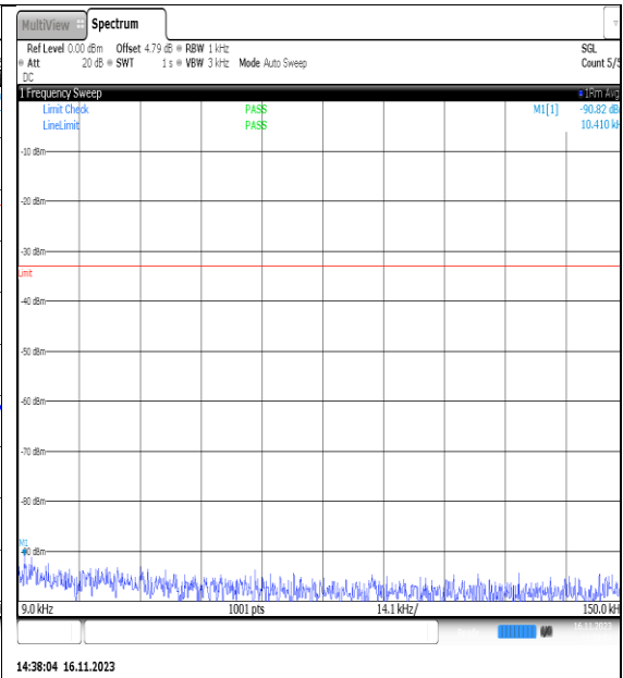
NTVN_N5_PC3_15_10_L_TID2_NS_01_0.009_0.15_#1
