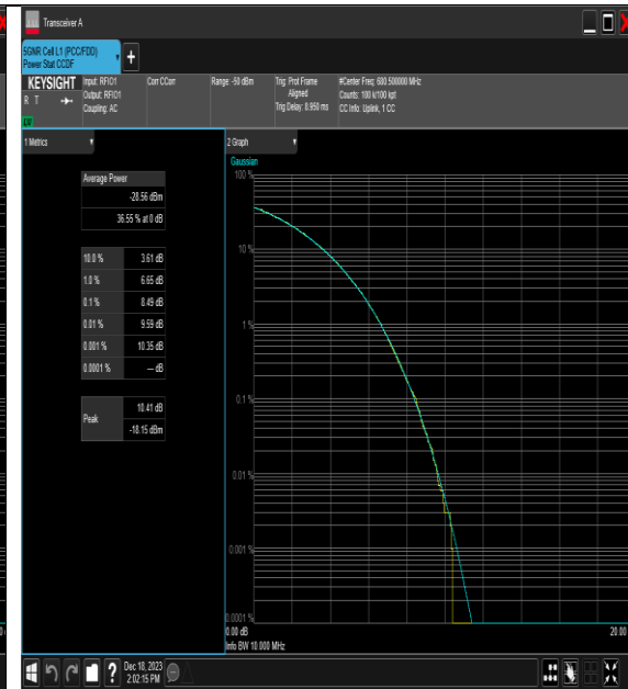
NTNV_N71_PC3_15_10_M_TID4_#1
