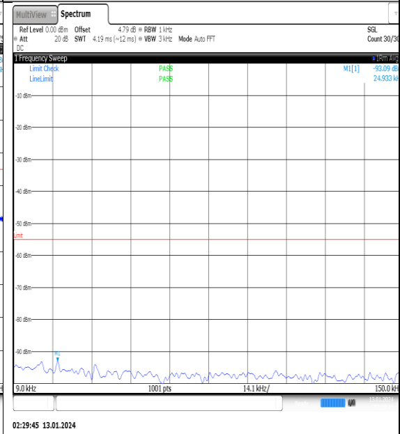
NTNV_N41_PC2_30_100_L_TID15_NS_01_0.00_9.0.15_#1
