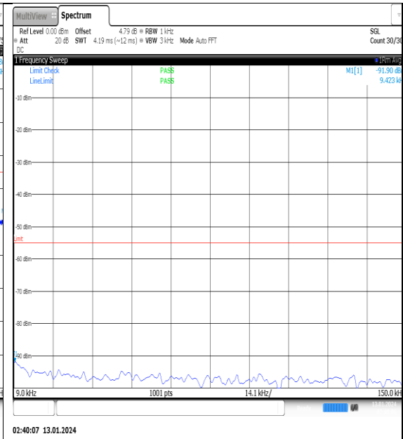
NTVN_N41_PC2_30_100_M_TID3_NS_01_0.009 _0.15_#1
