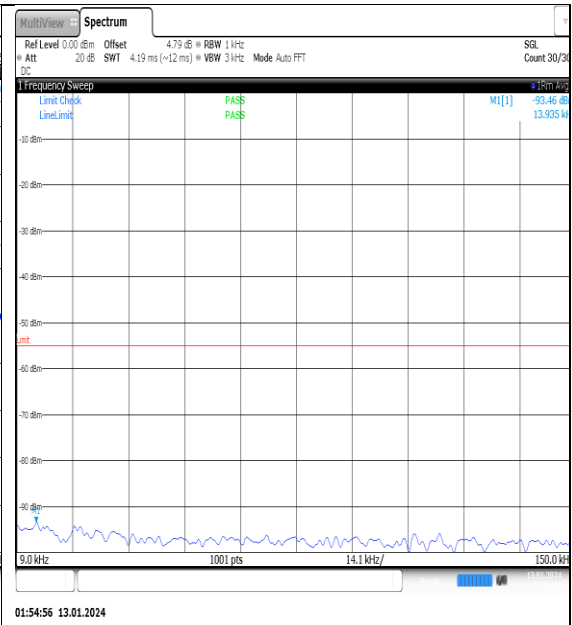
NTNV_N41_PC2_30_100_L_TID4_NS_01_0.009_0.15_#1
