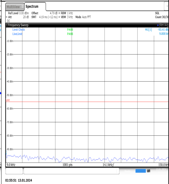
NTNV_N41_PC2_30_100_M_TID8_NS_01_0.009_0.15_#1
