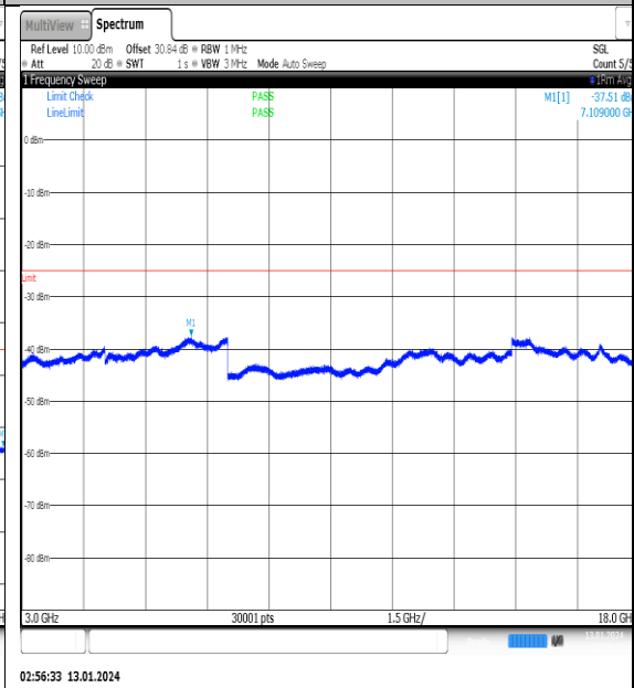
NTNV_N41_PC2_30_100_M_TID8_NS_01_3000_18000_#1
