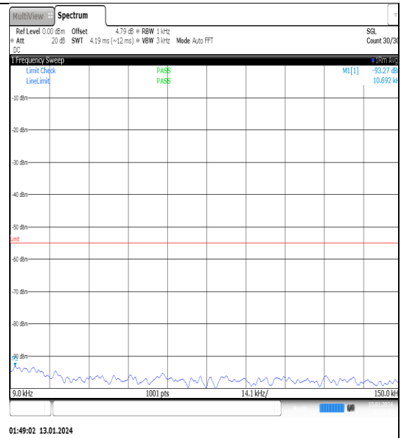
NTNV_N41_PC2_30_100_L_TID2_NS_01_0.009_0.15_#1
