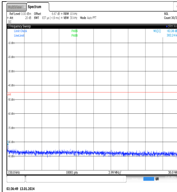
NTNV_N41_PC2_30_100_M_TID2_NS_01_0.15_30_#1
