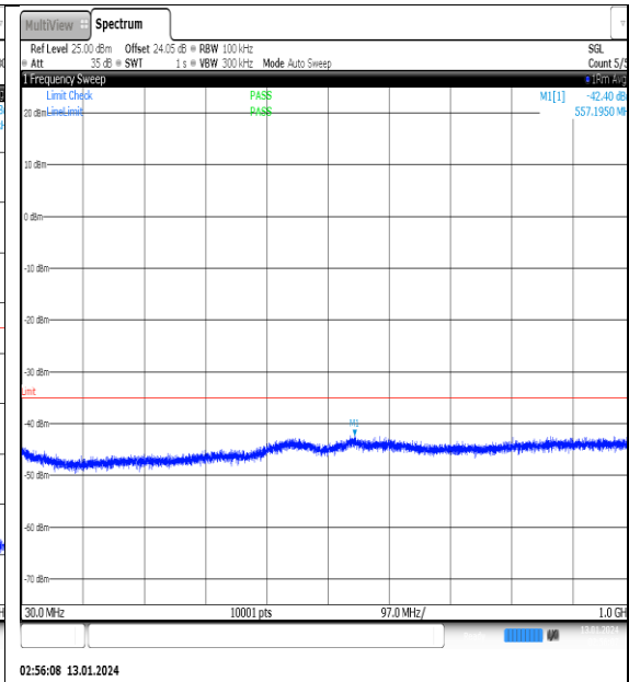
NTNV_N41_PC2_30_100_M_TID8_NS_01_30_1000_#1
