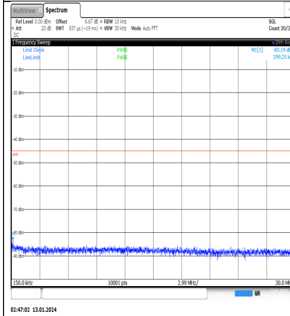
NTVN_N41_PC2_30_100_M_TID5_NS_01_0.15_30_#1
