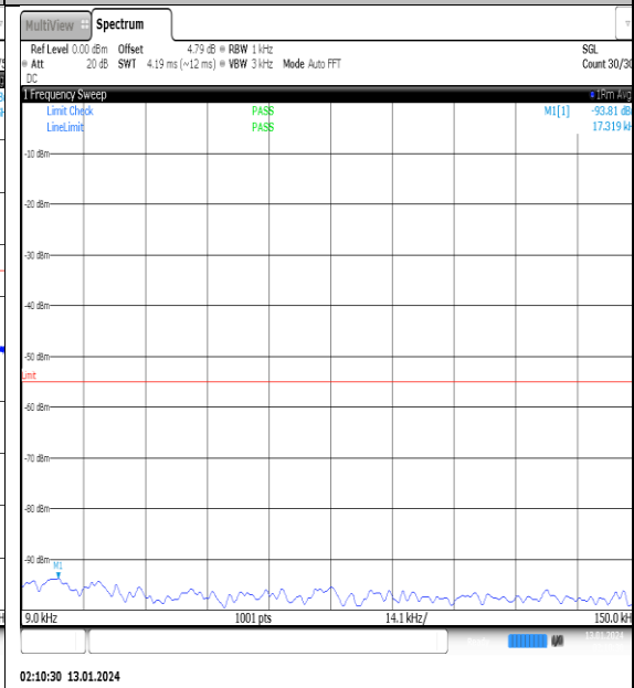
NTNV_N41_PC2_30_100_L_TID9_NS_01_0.009_0.15_#1
