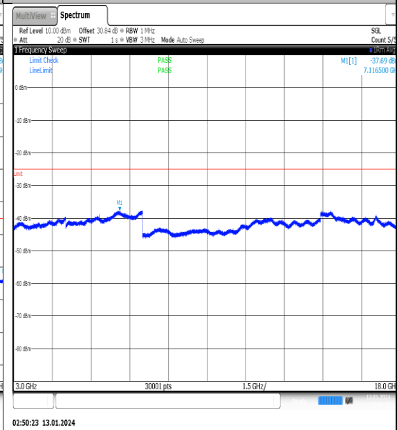
NTNV_N41_PC2_30_100_M_TID6_NS_01_3000_18000_#1
