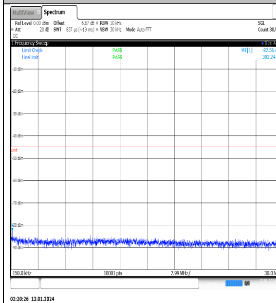
NTNV_N41_PC2_30_100_L_TID12_NS_01_0.15_30_#1
