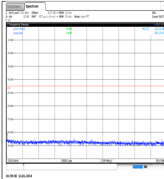
NTNV_N41_PC2_30_90_H_TID14_NS_01_0.15_30_#1
