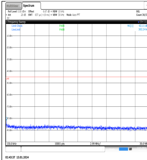
NTNV_N41_PC2_30_100_M_TID4_NS_01_0.15_30_#1
