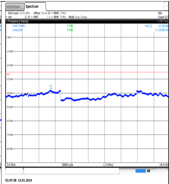
NTVN_N41_PC2_30_100_M_TID5_NS_01_3000_18000_#1
