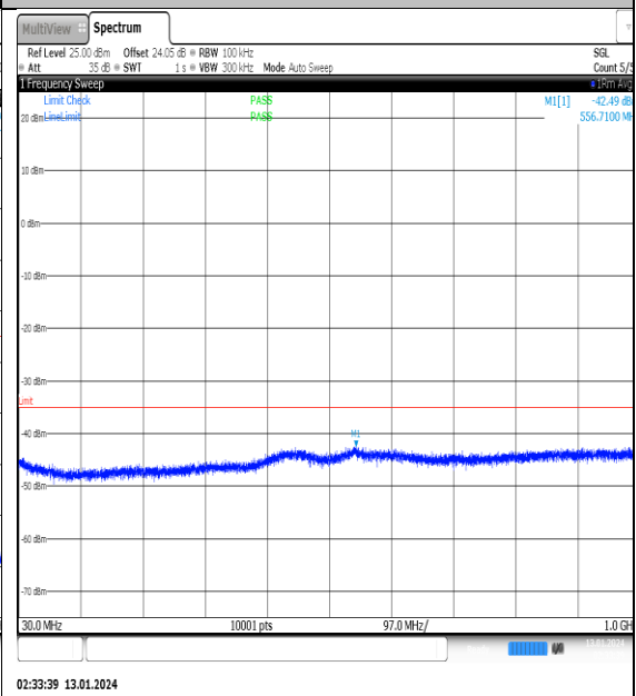
NTNV_N41_PC2_30_100_M_TID1_NS_01_30_1000_#1
