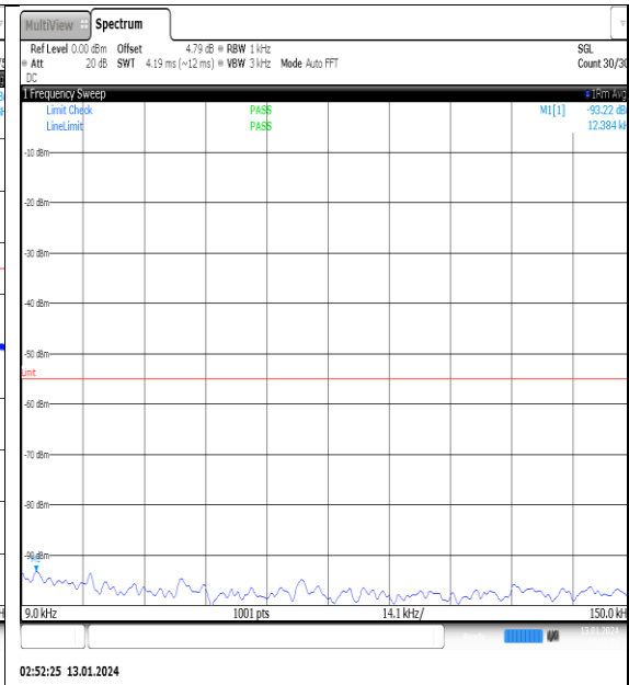
NTVN_N41_PC2_30_100_M_TID7_NS_01_0.009 _0.15_#1
