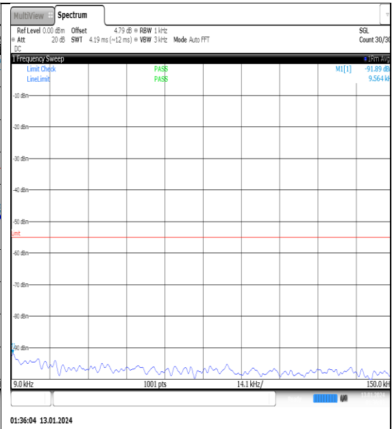
NTVN_N41_PC2_30_90_H_TID13_NS_01_0.009_0.15_#1
