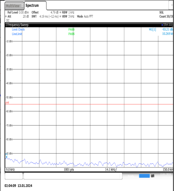
NTNV_N41_PC2_30_100_L_TID7_NS_01_0.009_0.15_#1
