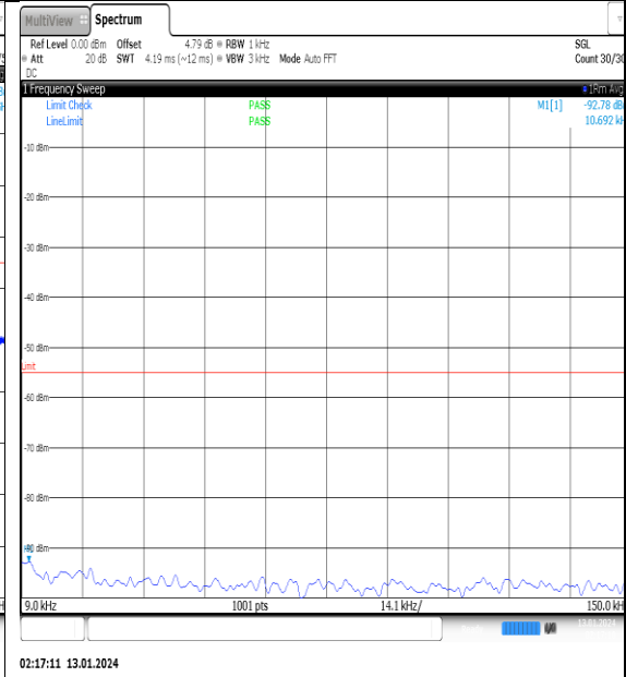
NTNV_N41_PC2_30_100_L_TID11_NS_01_0.00_9_0.15_#1
