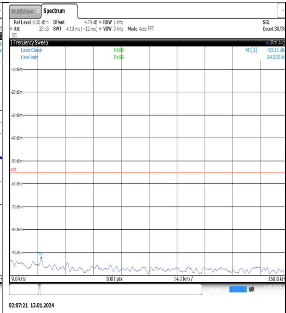
NTNV_N41_PC2_30_100_L_TID8_NS_01_0.009_0.15_#1
