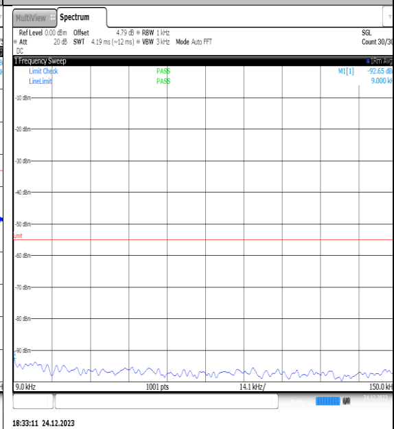
NTVN_N41_PC2_30_90_M_TID5_NS_01_0.009_0.15_#1
