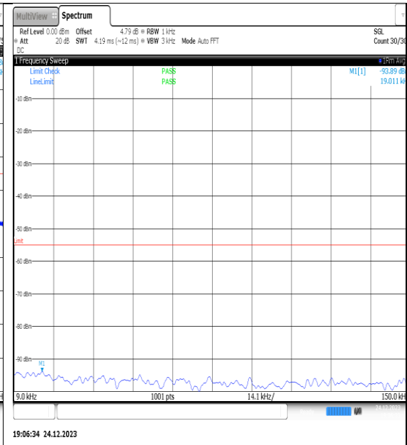
NTVN_N41_PC2_30_90_H_TID1_NS_01_0.009_0.15_#1
