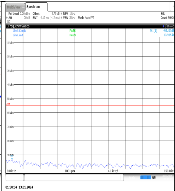
NTVN_N41_PC2_30_90_H_TID11_NS_01_0.009_0.15_#1
