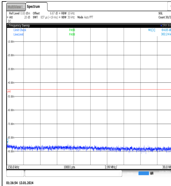
NTNV_N41_PC2_30_90_H_TID10_NS_01_0.15_30_#1
