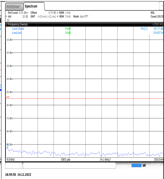
NTVN_N41_PC2_30_90_M_TID14_NS_01_0.009_0.15_#1
