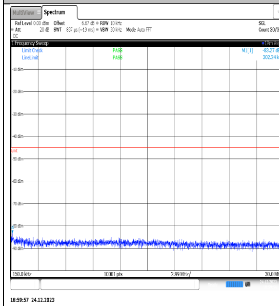
NTVN_N41_PC2_30_90_M_TID14_NS_01_0.15_30_#1
