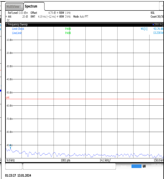
NTVN_N41_PC2_30_90_H_TID9_NS_01_0.009_0.15_#1
