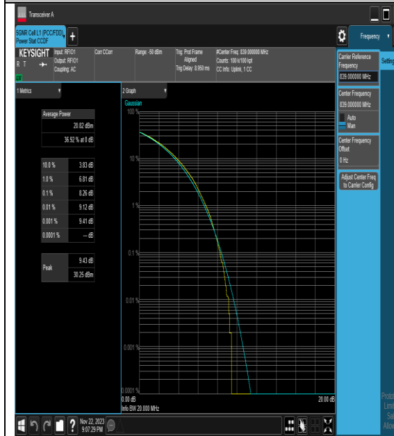
NTNV_N5_PC3_15_20_H_TID7_#1
