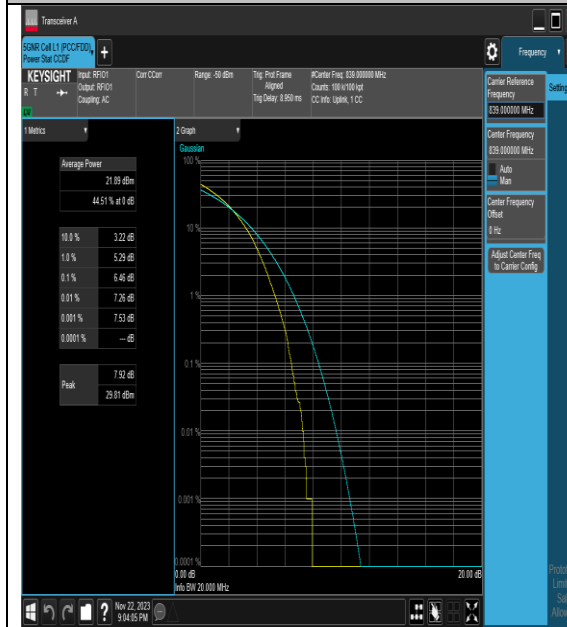
NTNV_N5_PC3_15_20_H_TID3_#1
