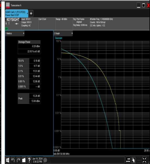
NTVN_N66_PC3_15_40_M_TID4_#1
