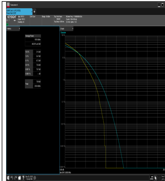
NTNV_N66_PC3_15_5_M_TID3_#1
