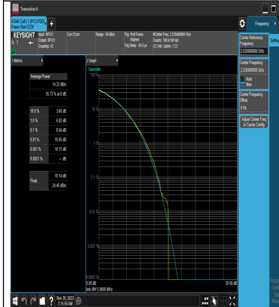
NTNV_N7_PC3_15_5_M_TID9_#1
