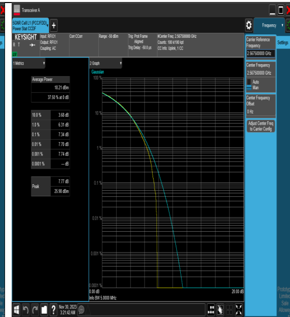
NTNV_N7_PC3_15_5_H_TID7_#1
