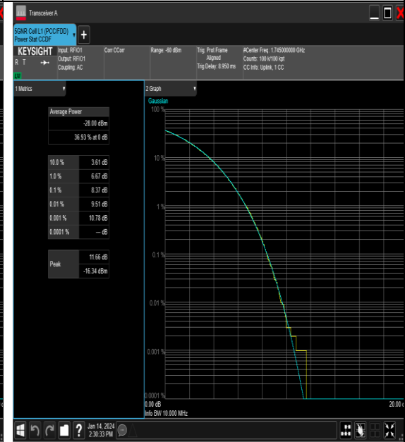
NTNV_N66_PC3_15_10_M_TID3_#1
