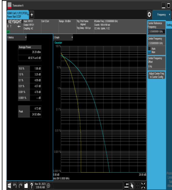
NTNV_N7_PC3_15_5_M_TID1_#1
