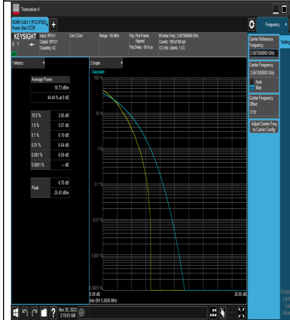
NTNV_N7_PC3_15_5_H_TID4_#1
