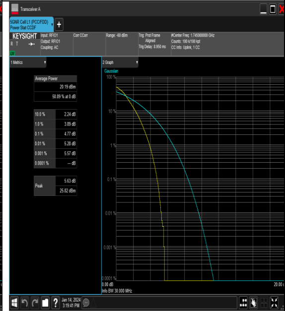
NTNV_N66_PC3_15_30_M_TID1_#1
