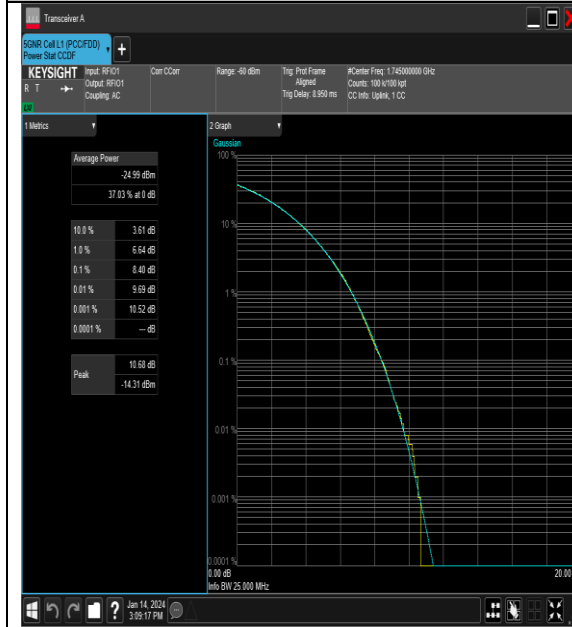
NTNV_N66_PC3_15_25_M_TID1_#1
