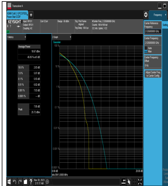
NTNV_N7_PC3_15_5_M_TID3_#1
