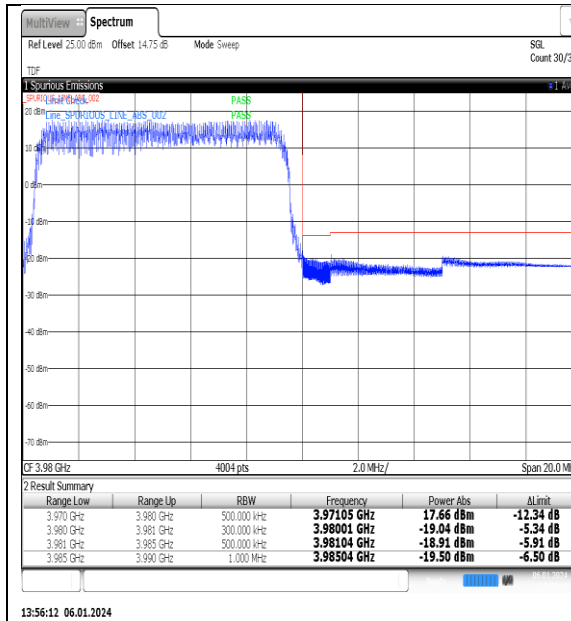
NTNV_N77-3700-3980_PC2_30_10_H_TID4_#1
