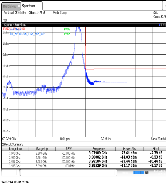
NTNV_N77-3700-3980_PC2_30_10_H_TID9_#1
