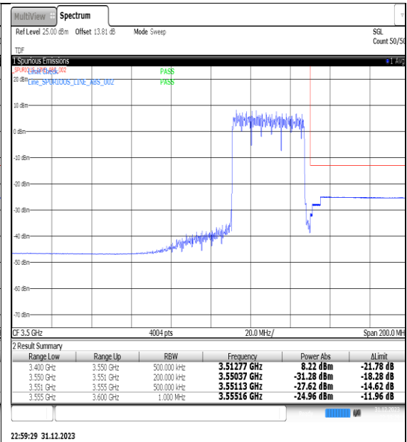
NTNV_N77-3450-3550_PC2_30_40_H_TID13_#1
