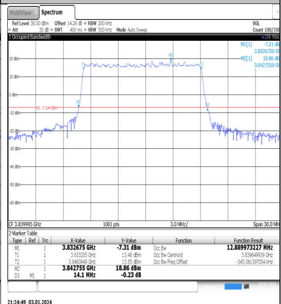
NTNV_N77-3700- 3980_PC2_30_15_M_TID2_Ant1#1
