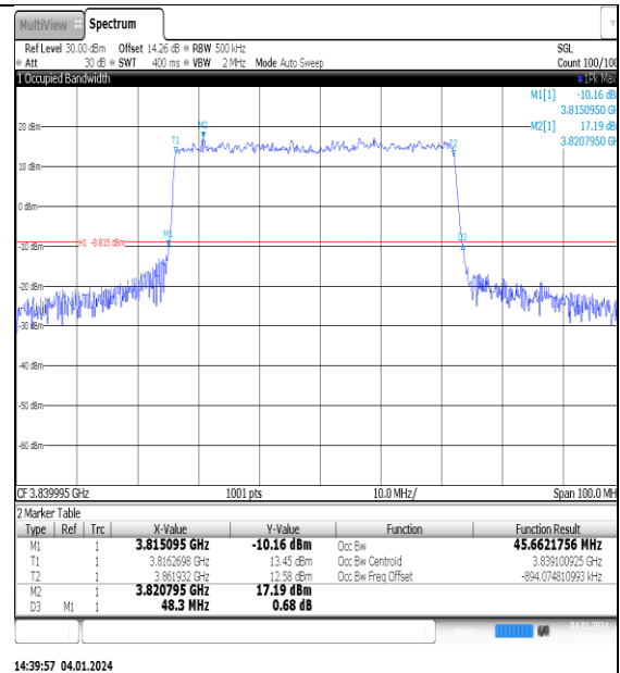
NTNV_N77-3700- 3980_PC2_30_50_M_TID3_Ant1#1
