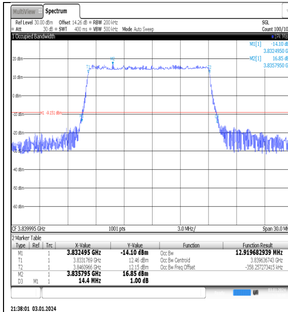
NTNV_N77-3700- 3980_PC2_30_15_M_TID3_Ant1#1
