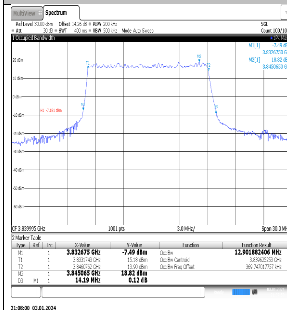
NTNV_N77-3700- 3980_PC2_30_15_M_TID1_Ant1#1
