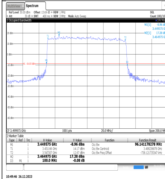
NTNV_N77-3450- 3550_PC2_30_100_M_TID3_Ant1#1
