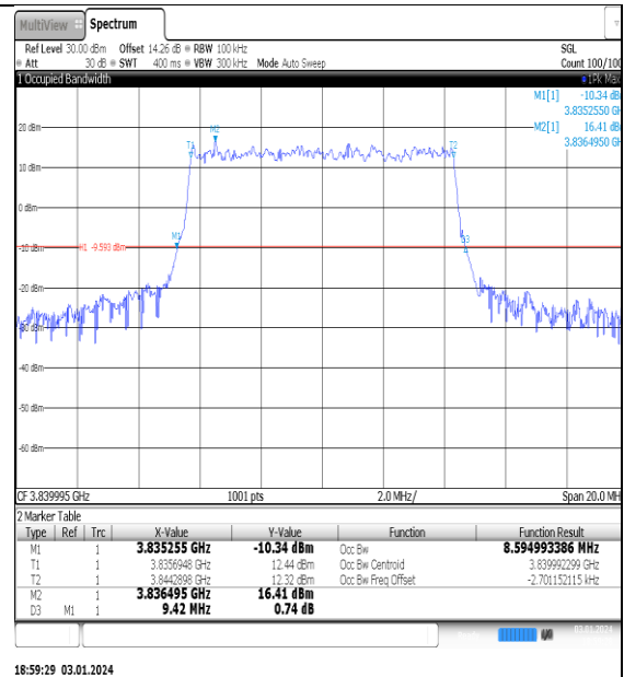
NTNV_N77-3700- 3980_PC2_30_10_M_TID3_Ant1#1
