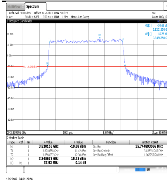
NTNV_N77-3700- 3980_PC2_30_40_M_TID4_Ant1#1
