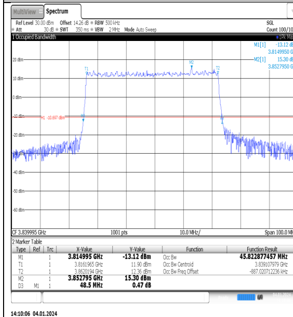
NTNV_N77-3700- 3980_PC2_30_50_M_TID4_Ant1#1
