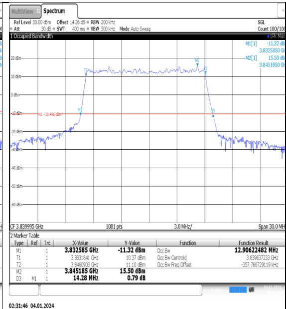
NTNV_N77-3700- 3980_PC2_30_15_M_TID4_Ant1#1
