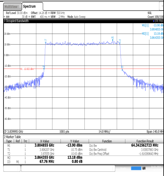
NTNV_N77-3700- 3980_PC2_30_70_M_TID4_Ant1#1
