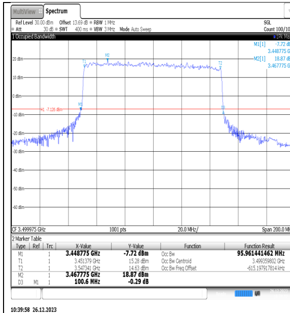
NTNV_N77-3450- 3550_PC2_30_100_M_TID1_Ant1#1
