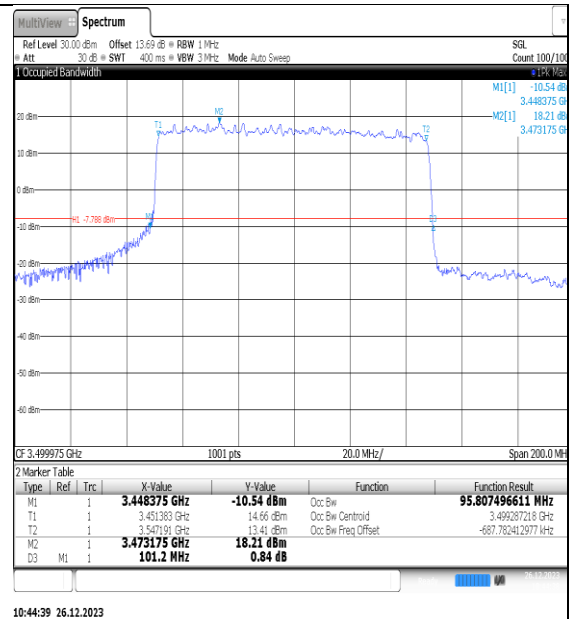
NTNV_N77-3450- 3550_PC2_30_100_M_TID2_Ant1#1
