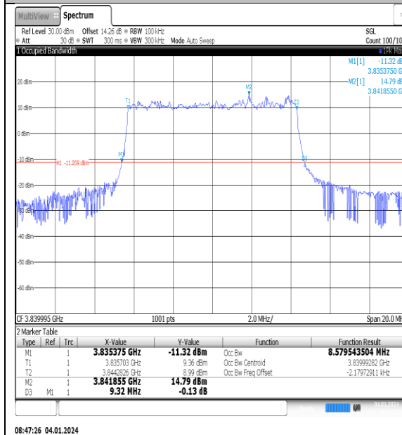
NTNV_N77-3700- 3980_PC2_30_10_M_TID4_Ant1#1
