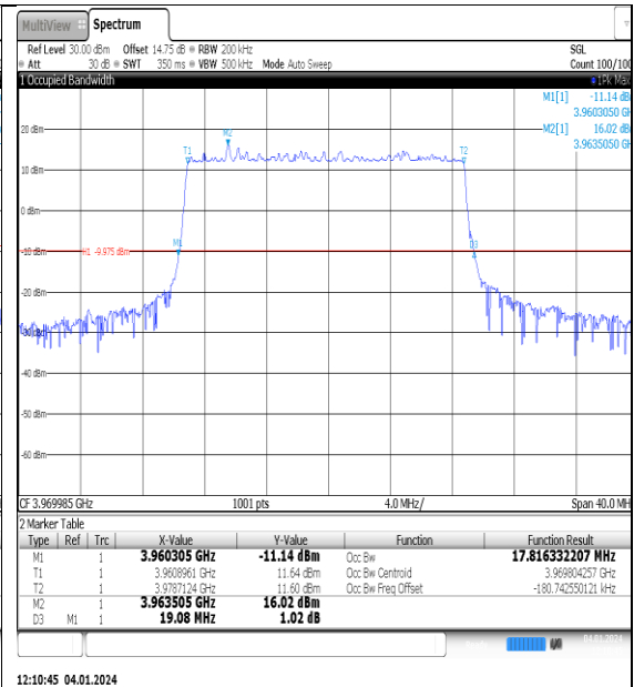
NTNV_N77-3700- 3980_PC2_30_20_H_TID4_Ant1#1
