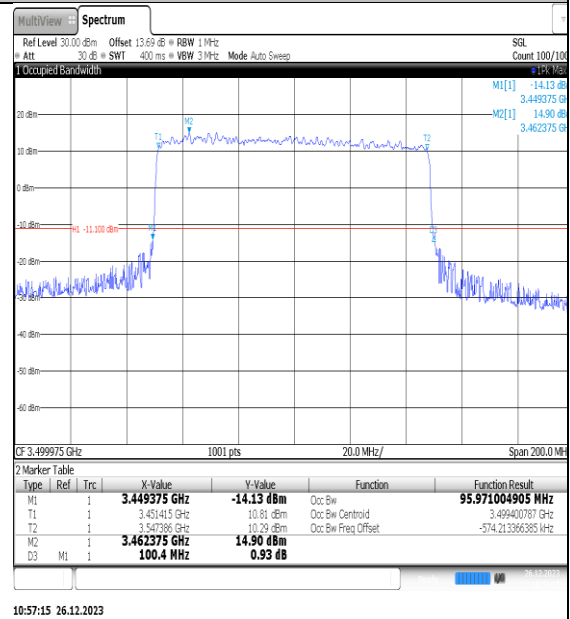
NTNV_N77-3450- 3550_PC2_30_100_M_TID4_Ant1#1
