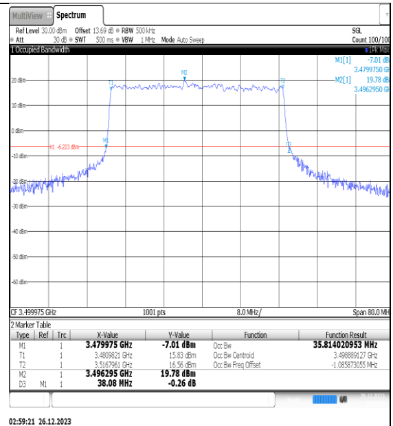
NTNV_N77-3450- 3550_PC2_30_40_M_TID2_Ant1#1
