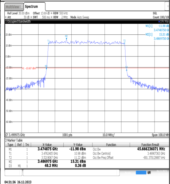
NTNV_N77-3450- 3550_PC2_30_50_M_TID4_Ant1#1
