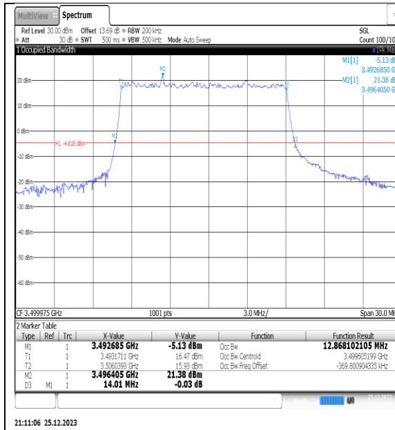
NTNV_N77-3450- 3550_PC2_30_15_M_TID1_Ant1#1
