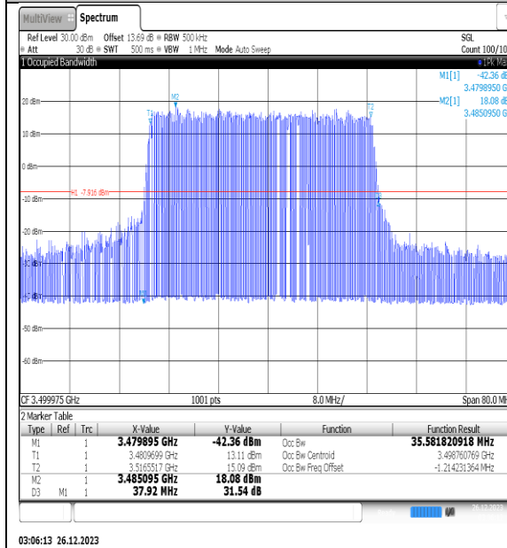
NTNV_N77-3450- 3550_PC2_30_40_M_TID3_Ant1#1
