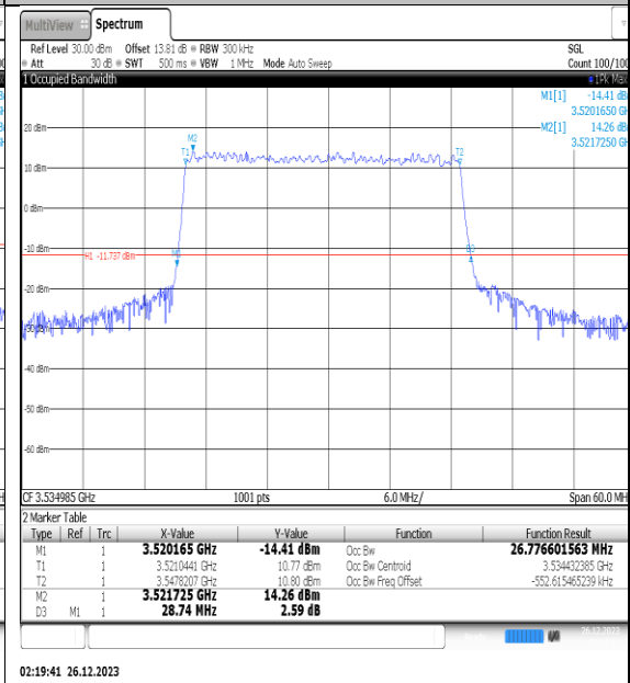
NTNV_N77-3450-3550_PC2_30_30_H_TID4_Ant1#1
