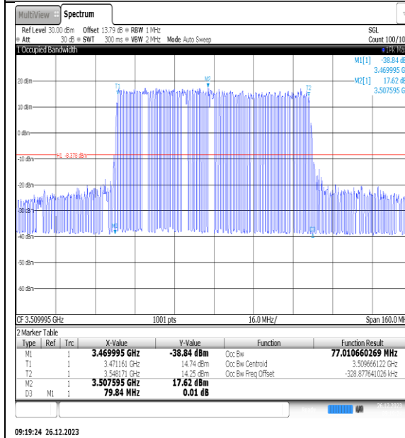
NTNV_N77-3450- 3550_PC2_30_80_H_TID3_Ant1#1
