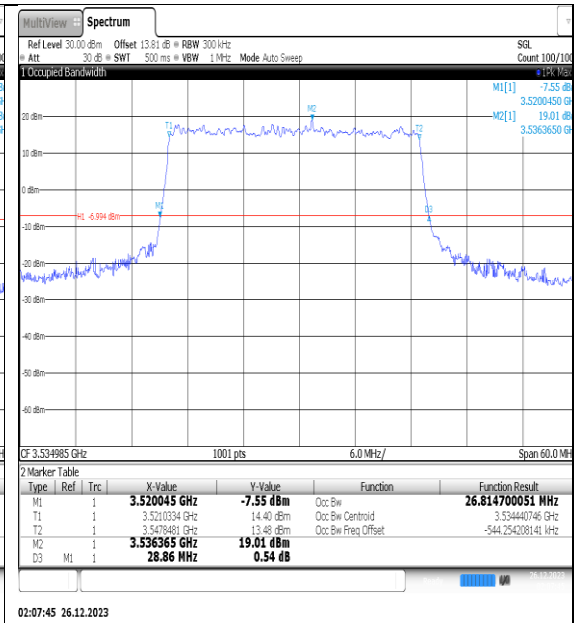
NTNV_N77-3450-3550_PC2_30_30_H_TID2_Ant1#1
