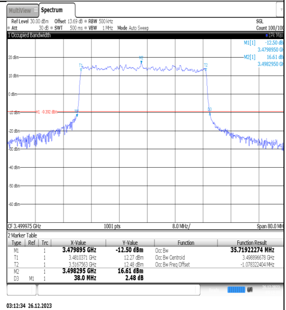
NTNV_N77-3450- 3550_PC2_30_40_M_TID4_Ant1#1
