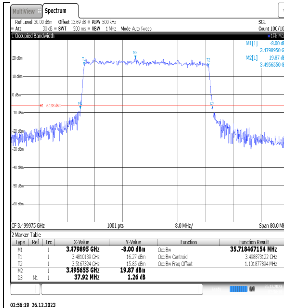
NTNV_N77-3450- 3550_PC2_30_40_M_TID1_Ant1#1
