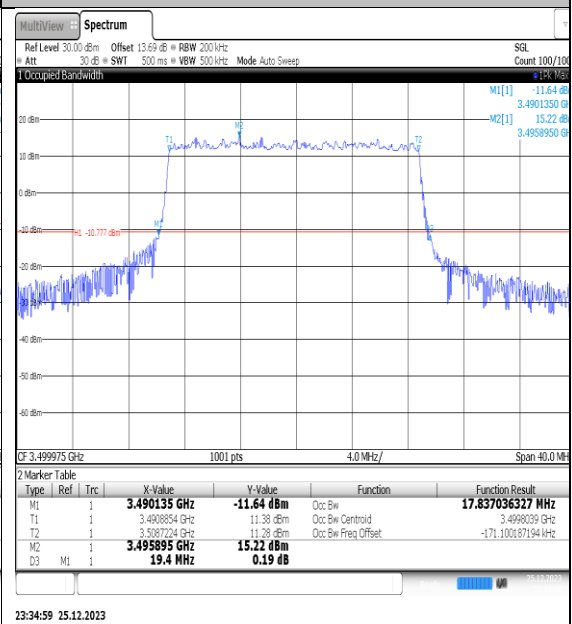
NTNV_N77-3450- 3550_PC2_30_20_M_TID4_Ant1#1
