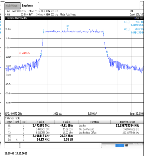
NTNV_N77-3450- 3550_PC2_30_15_M_TID2_Ant1#1
