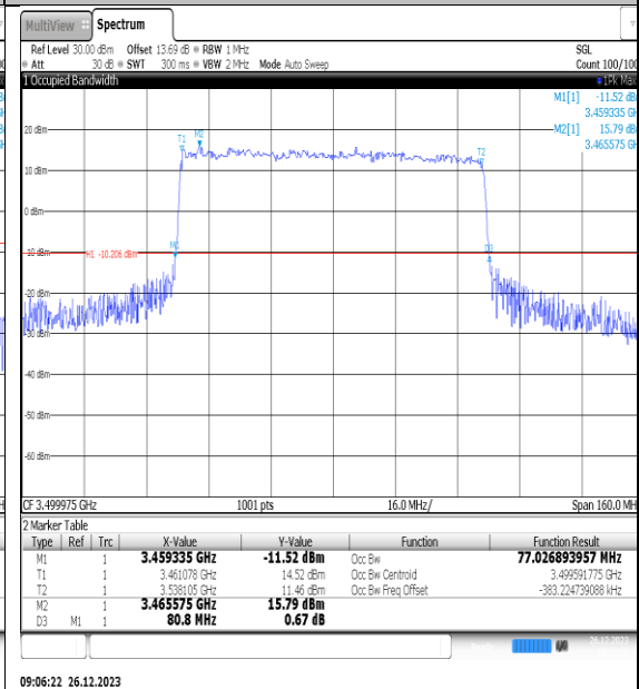
NTNV_N77-3450- 3550_PC2_30_80_M_TID4_Ant1#1
