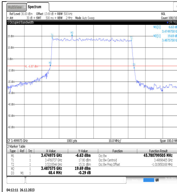
NTNV_N77-3450- 3550_PC2_30_50_M_TID1_Ant1#1
