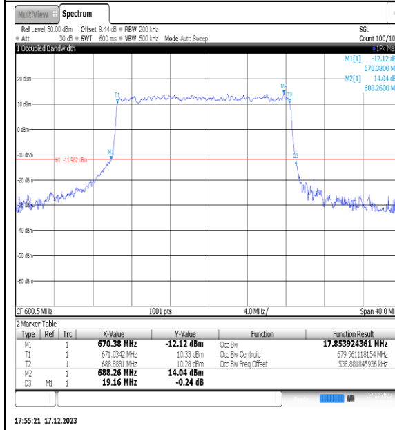
NTNV_N71_PC3_15_20_M_TID3_Ant1#1
