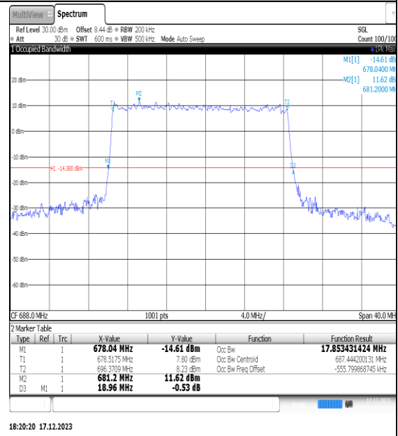
NTNV_N71_PC3_15_20_H_TID4_Ant1#1
