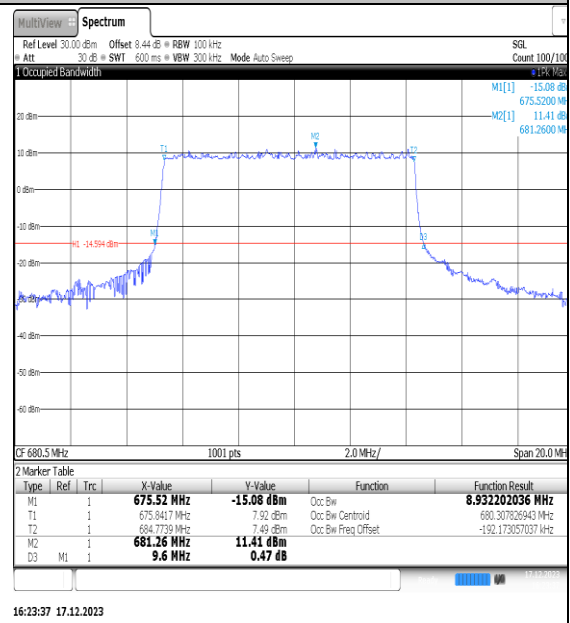
NTNV_N71_PC3_15_10_M_TID4_Ant1#1
