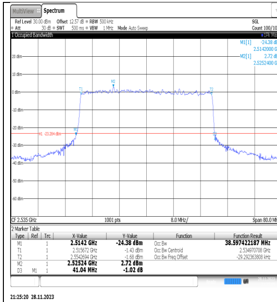
NTNV_N7_PC3_15_40_M_TID1_Ant#1
