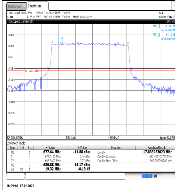
NTNV_N71_PC3_15_20_H_TID3_Ant1#1
