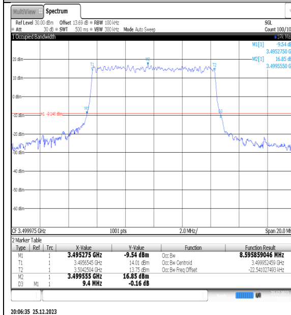
NTNV_N77-3450- 3550_PC2_30_10_M_TID3_Ant1#1
