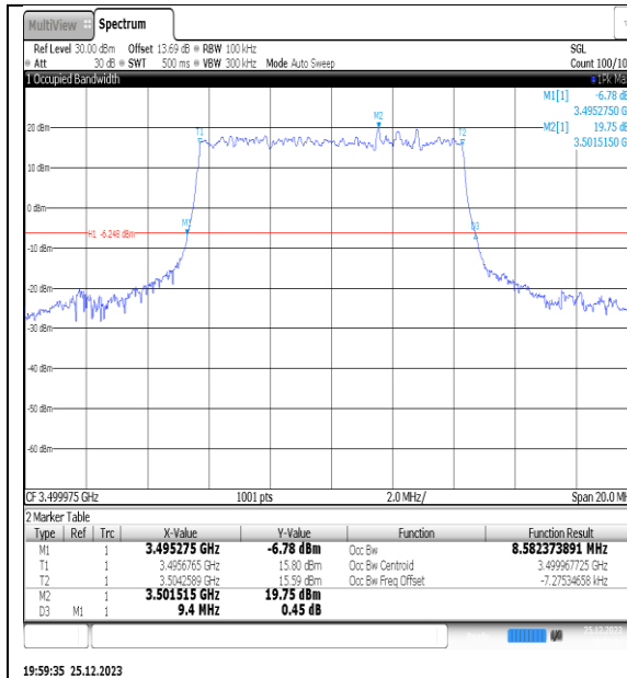
NTNV_N77-3450- 3550_PC2_30_10_M_TID1_Ant1#1
