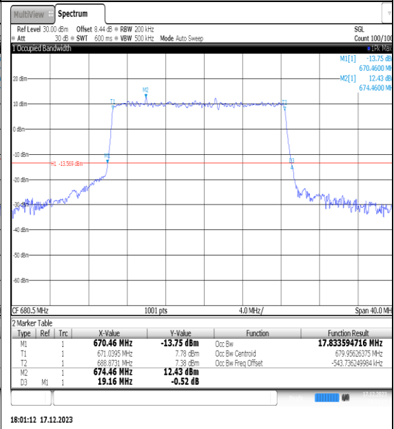
NTNV_N71_PC3_15_20_M_TID4_Ant1#1
