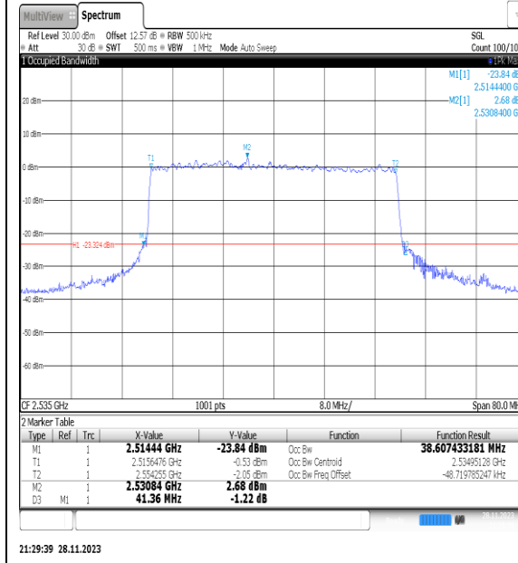
NTNV_N7_PC3_15_40_M_TID3_Ant#1
