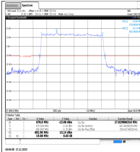
NTNV_N71_PC3_15_20_H_TID1_Ant1#1
