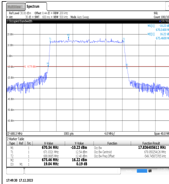
NTNV_N71_PC3_15_20_M_TID1_Ant1#1
