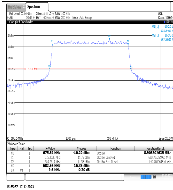
NTNV_N71_PC3_15_10_M_TID1_Ant1#1
