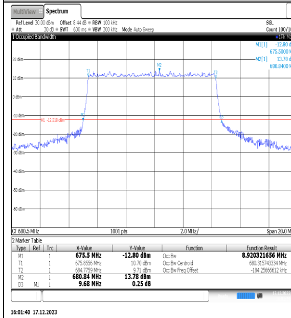
NTNV_N71_PC3_15_10_M_TID3_Ant1#1
