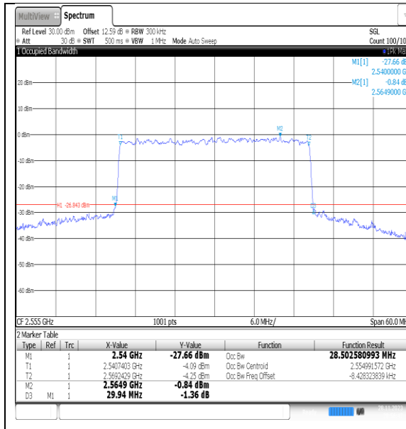
NTNV_N7_PC3_15_30_H_TID5_Ant#1
