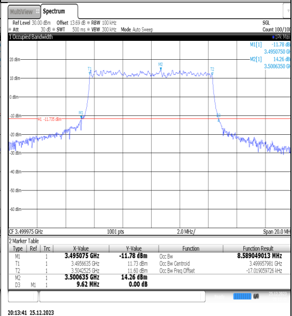
NTNV_N77-3450- 3550_PC2_30_10_M_TID4_Ant1#1
