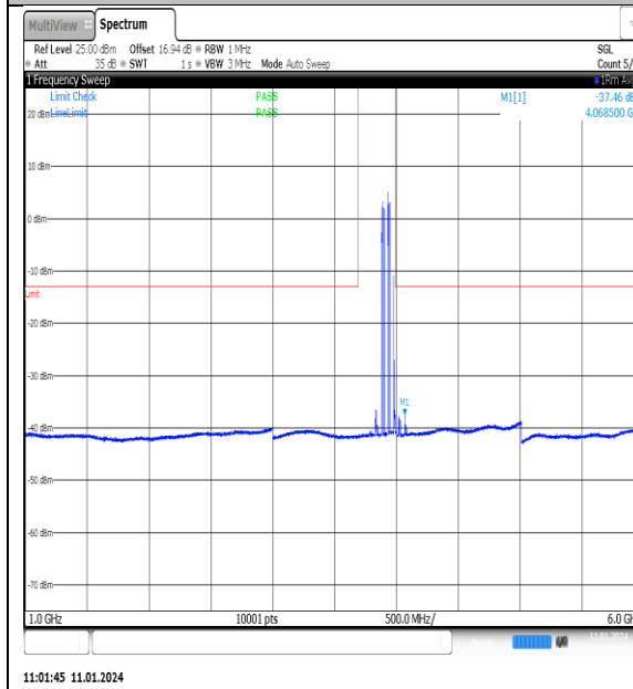
NTNV_N77-3700-3980_PC2_30_100_H_TID1_NS_01_1000_6000_#1
