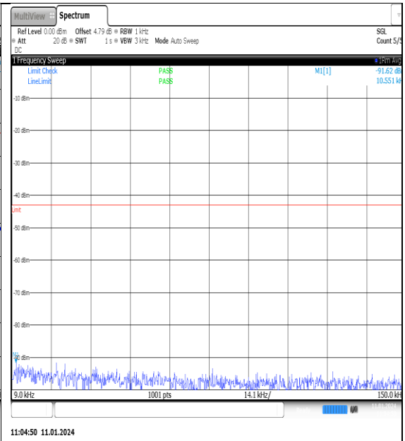
NTNV_N77-3700- 3980_PC2_30_100_H_TID2_NS_01_0.009_0.15_#1
