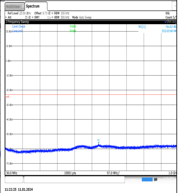
NTNV_N77-3700- 3980_PC2_30_100_H_TID6_NS_01_30_1000_#1
