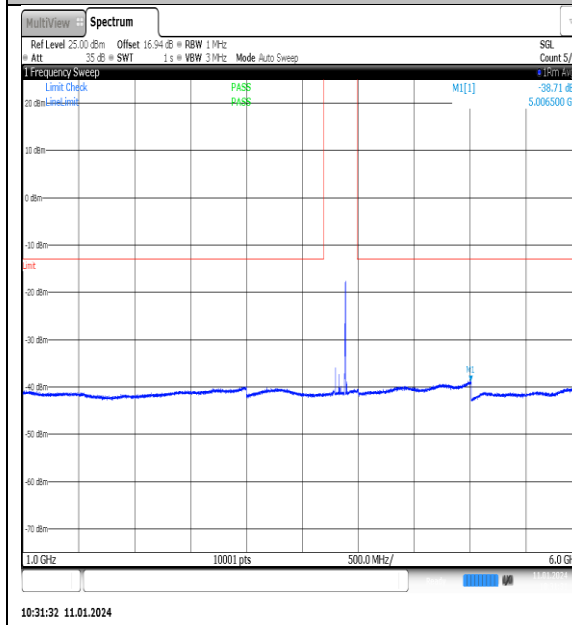
NTNV_N77-3700- 3980_PC2_30_100_M_TID6_NS_01_1000_6000_#1
