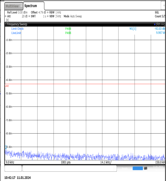
NTN_V_N77-3700- 3980_PC2_30_100_M_TID10_NS_01_0.009_0.15 #1
