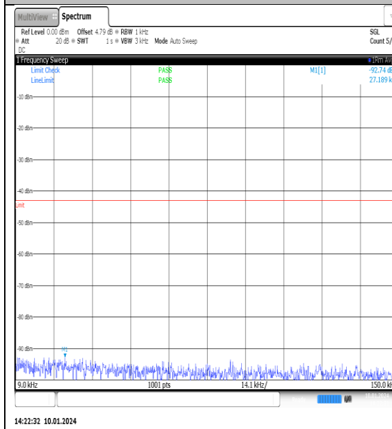
NTNV_N77-3700- 3980_PC2_30_100_M_TID4_NS_01_0.009_0.15_#1
