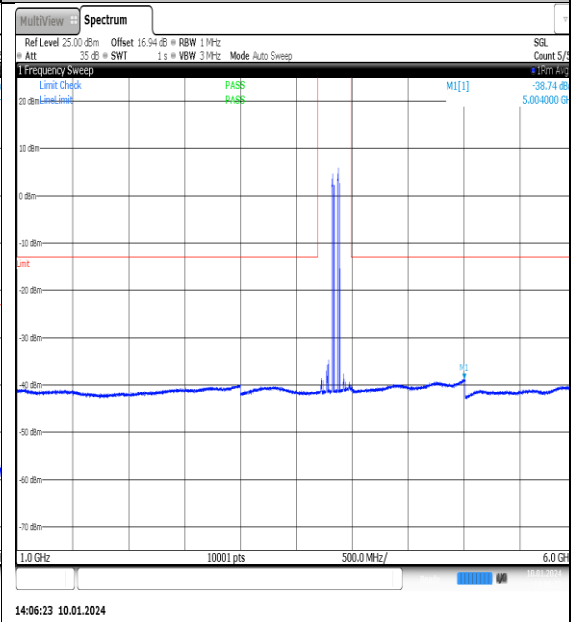
NTNV_N77-3700- 3980_PC2_30_100_M_TID1_NS_01_1000_6000_ #1
