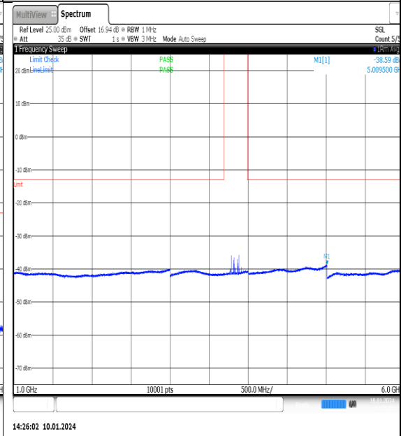
NTNV_N77-3700- 3980_PC2_30_100_M_TID5_NS_01_1000_6000_ #1
