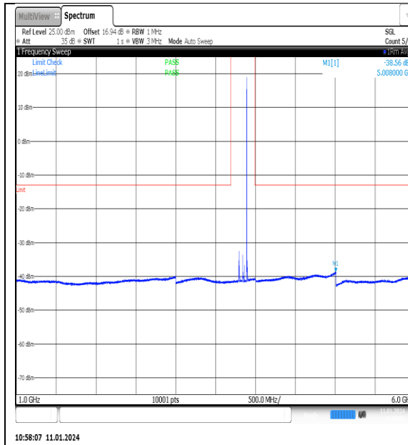
NTN_V_N77-3700- 3980_PC2_30_100_M_TID15_NS_01_1000_6000 #1
