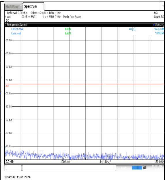
NTNV_N77-3700- 3980_PC2_30_100_M_TID11_NS_01_0.009_0.15 _#1
