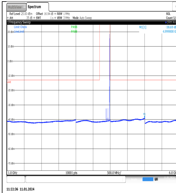
NTN_V_N77-3700- 3980_PC2_30_100_H_TID6_NS_01_1000_6000_ #1
