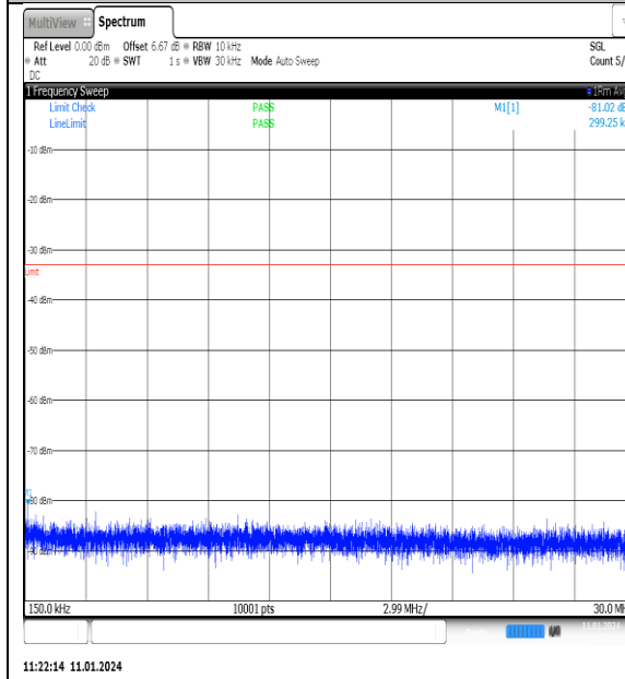
NTNV_N77-3700- 3980_PC2_30_100_H_TID6_NS_01_0.15_30_#1
