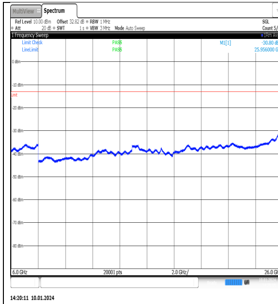
NTNV_N77-3700- 3980_PC2_30_100_M_TID3_NS_01_6000_26000 #1
