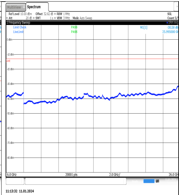
NTN_V_N77-3700- 3980_PC2_30_100_H_TID4_NS_01_6000_26000 #1
