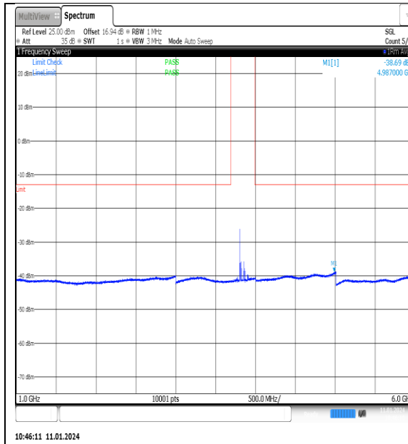
NTNV_N77-3700- 3980_PC2_30_100_M_TID11_NS_01_1000_6000 _#1
