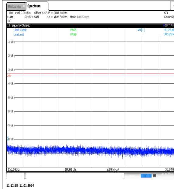
NTNV_N77-3700- 3980_PC2_30_100_H_TID4_NS_01_0.15_30_#1
