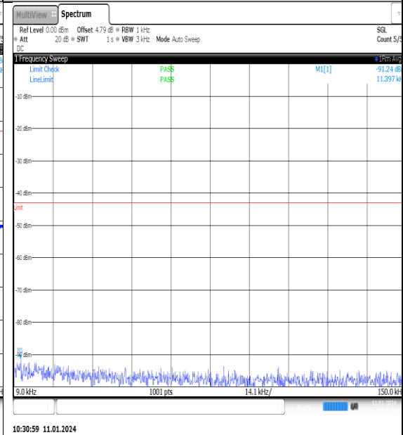
NTN_V_N77-3700- 3980_PC2_30_100_M_TID6_NS_01_0.009_0.15_ #1
