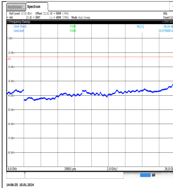
NTNV_N77-3700- 3980_PC2_30_100_M_TID1_NS_01_6000_26000 #1
