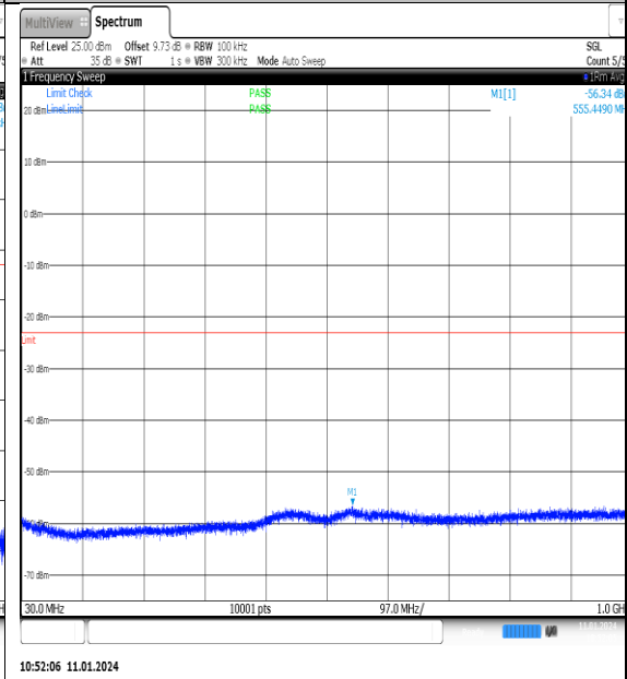
NTNV_N77-3700- 3980_PC2_30_100_M_TID13_NS_01_30_1000_# 1
