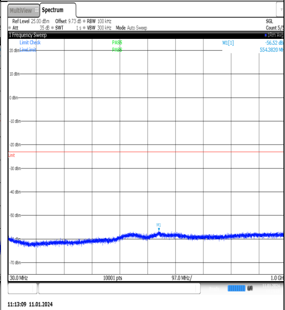
NTNV_N77-3700- 3980_PC2_30_100_H_TID4_NS_01_30_1000_#1
