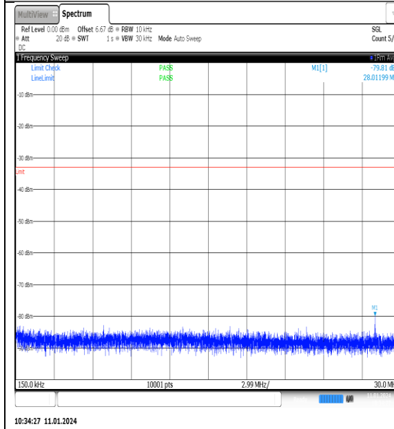
NTNV_N77-3700- 3980_PC2_30_100_M_TID7_NS_01_0.15_30_#1
