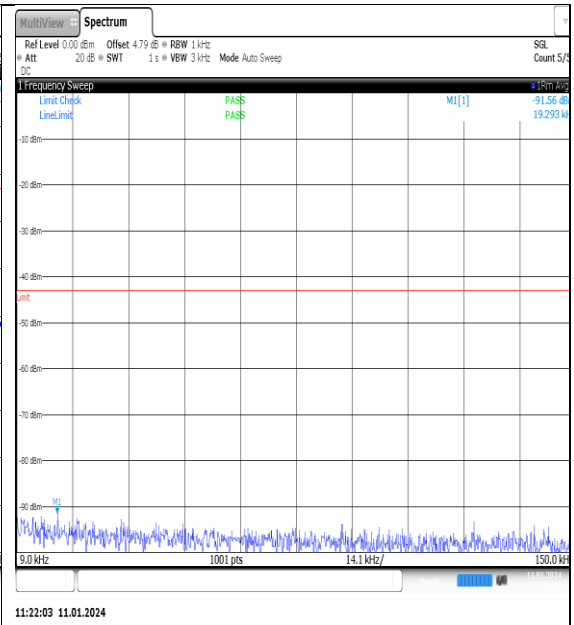
NTNV_N77-3700- 3980_PC2_30_100_H_TID6_NS_01_0.009_0.15_#1
