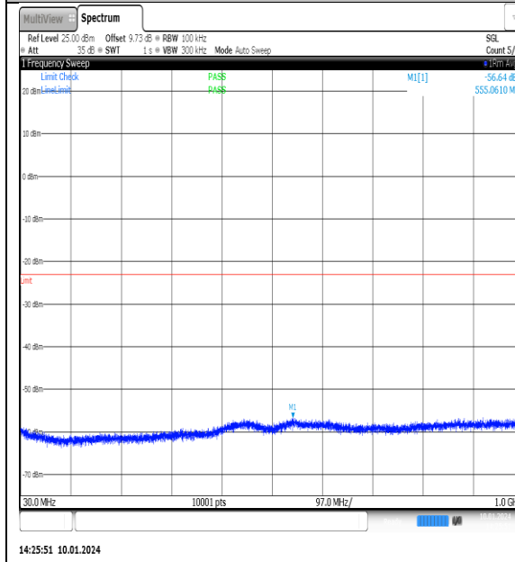
NTNV_N77-3700- 3980_PC2_30_100_M_TID5_NS_01_30_1000_#1
