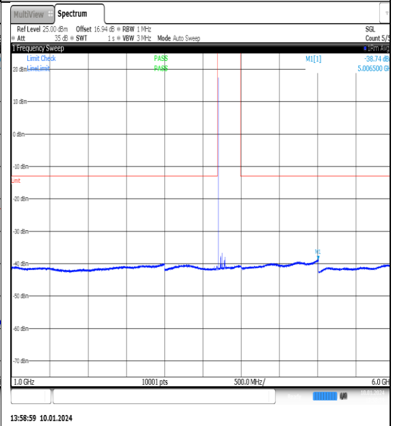
NTNV_N77-3700- 3980_PC2_30_100_L_TID14_NS_01_1000_6000 #1
