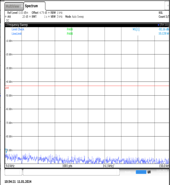
NTN_V_N77-3700- 3980_PC2_30_100_M_TID14_NS_01_0.009_0.15 #1
