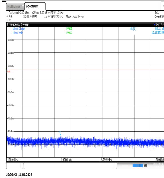
NTNV_N77-3700- 3980_PC2_30_100_M_TID9_NS_01_0.15_30_#1
