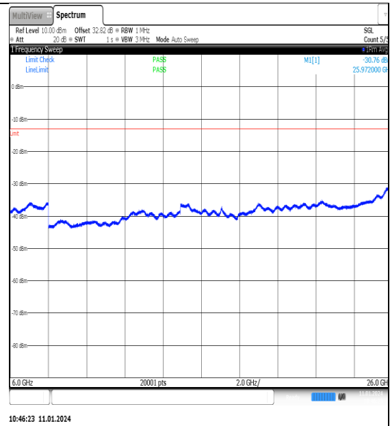
NTNV_N77-3700- 3980_PC2_30_100_M_TID11_NS_01_6000_2600 0_#1
