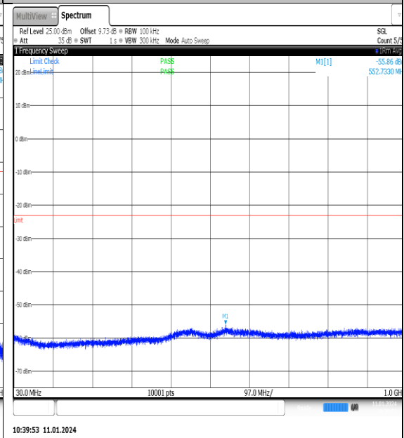
NTNV_N77-3700- 3980_PC2_30_100_M_TID9_NS_01_30_1000_#1
