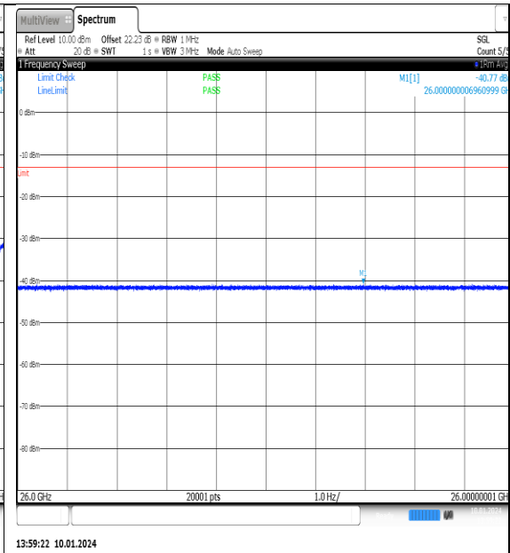
NTNV_N77-3700- 3980_PC2_30_100_L_TID14_NS_01_26000_400 _00_#1
