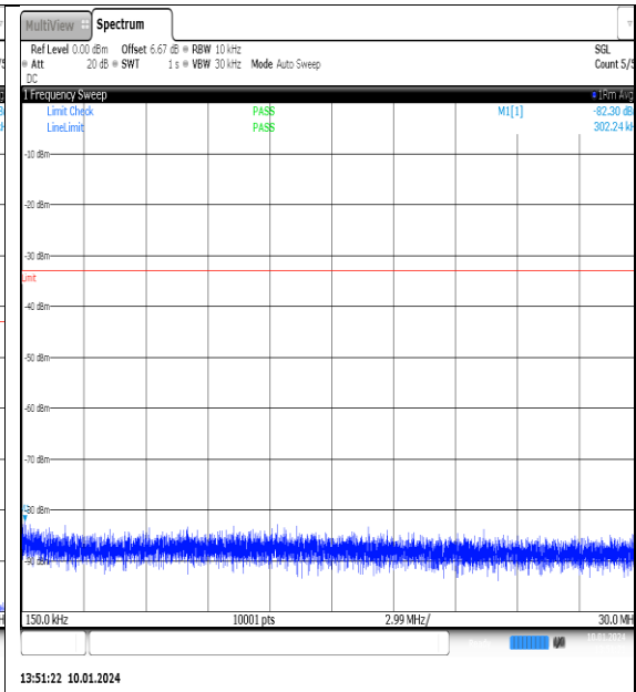
NTNV_N77-3700- 3980_PC2_30_100_L_TID12_NS_01_0.15_30_#1
