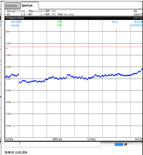
NTN_V_N77-3700- 3980_PC2_30_100_M_TID15_NS_01_6000_2600 0_#1
