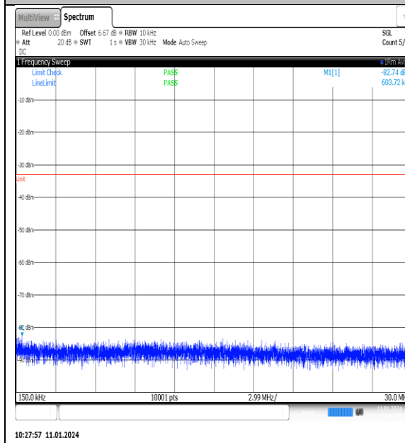
NTNV_N77-3700- 3980_PC2_30_70_M_TID14_NS_01_0.15_30_#1
