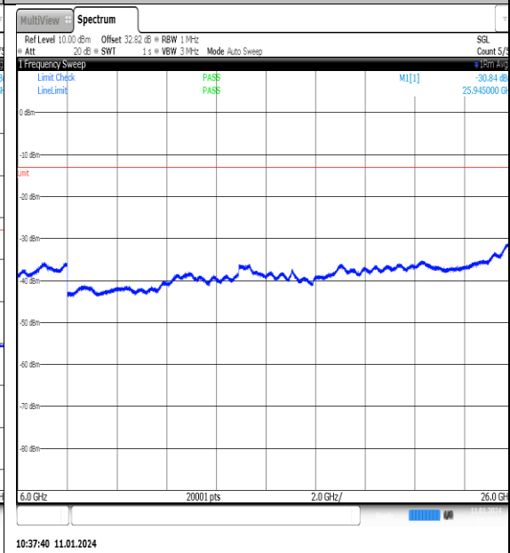
NTNV_N77-3700- 3980_PC2_30_100_M_TID8_NS_01_6000_26000_#1
