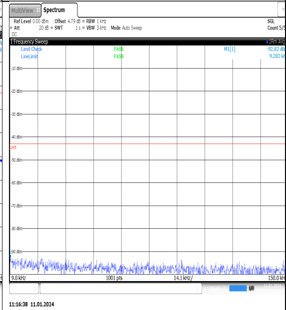
NTN_V_N77-3700- 3980_PC2_30_100_H_TID5_NS_01_0.009_0.15_ #1
