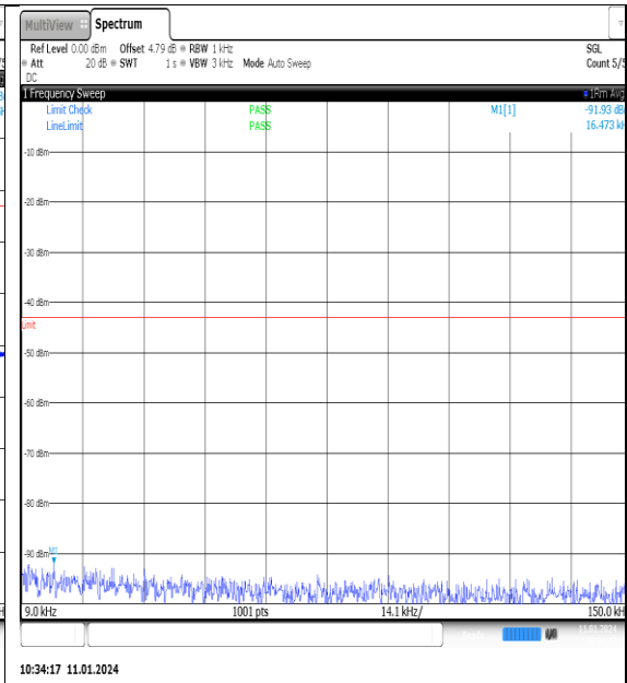
NTNV_N77-3700- 3980_PC2_30_100_M_TID7_NS_01_0.009_0.15_#1
