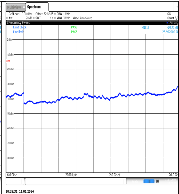
NTN_V_N77-3700- 3980_PC2_30_70_M_TID14_NS_01_6000_26000 #1
