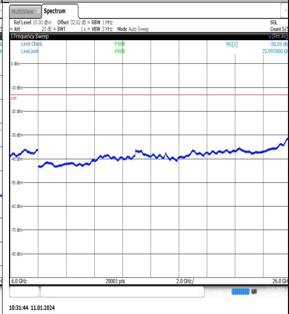
NTNV_N77-3700- 3980_PC2_30_100_M_TID6_NS_01_6000_26000_#1
