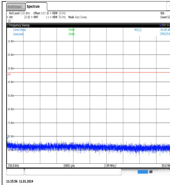
NTNV_N77-3700-3980_PC2_30_100_H_TID7_NS_01_0.15_30_#1
