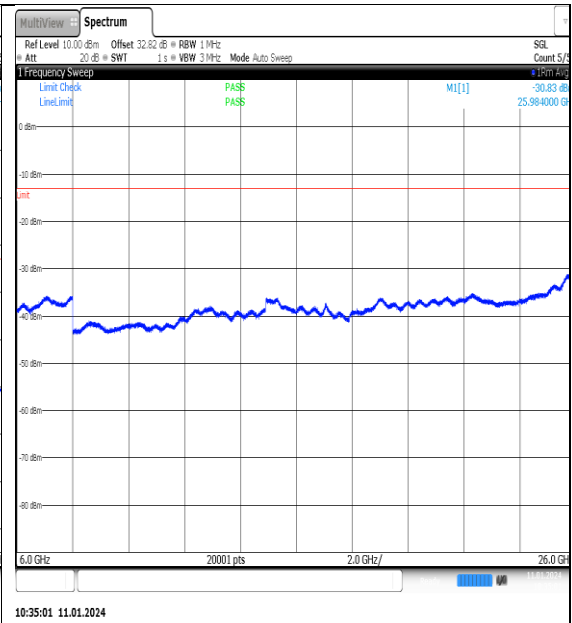
NTN_V_N77-3700- 3980_PC2_30_100_M_TID7_NS_01_6000_26000 #1
