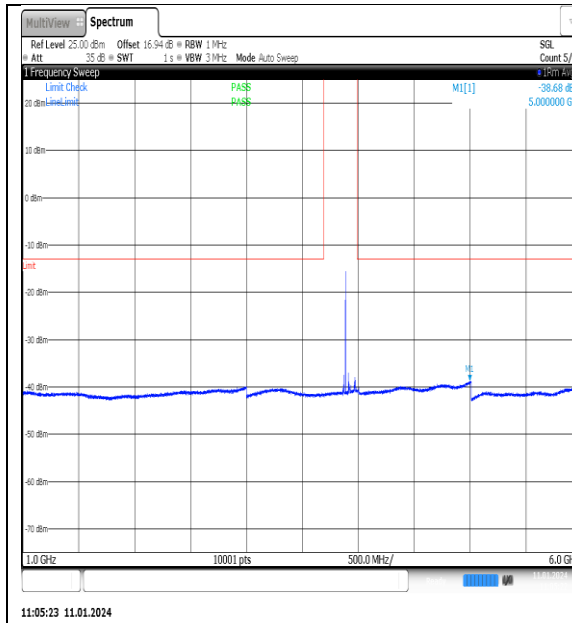
NTN_V_N77-3700- 3980_PC2_30_100_H_TID2_NS_01_1000_6000_ #1
