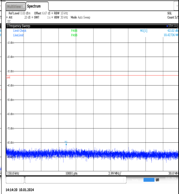
NTNV_N77-3700- 3980_PC2_30_100_M_TID2_NS_01_0.15_30_#1
