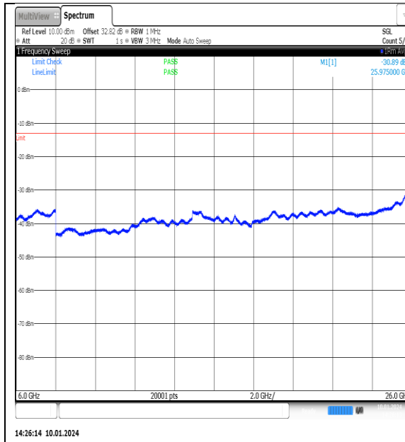
NTNV_N77-3700- 3980_PC2_30_100_M_TID5_NS_01_6000_26000 _#1
