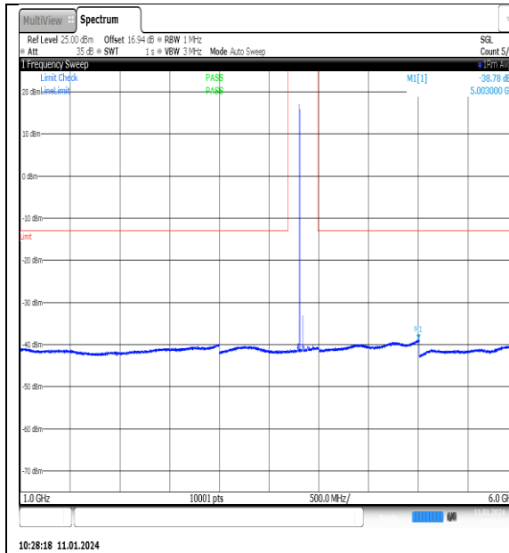
NTN_V_N77-3700- 3980_PC2_30_70_M_TID14_NS_01_1000_6000_ #1
