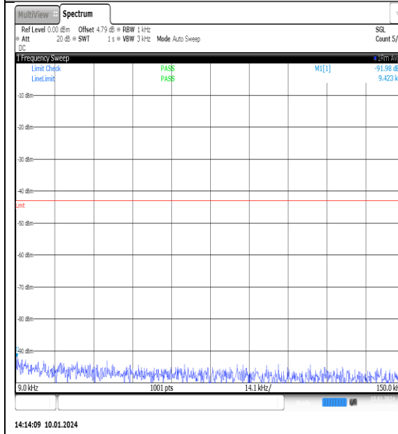
NTNV_N77-3700- 3980_PC2_30_100_M_TID2_NS_01_0.009_0.15_#1
