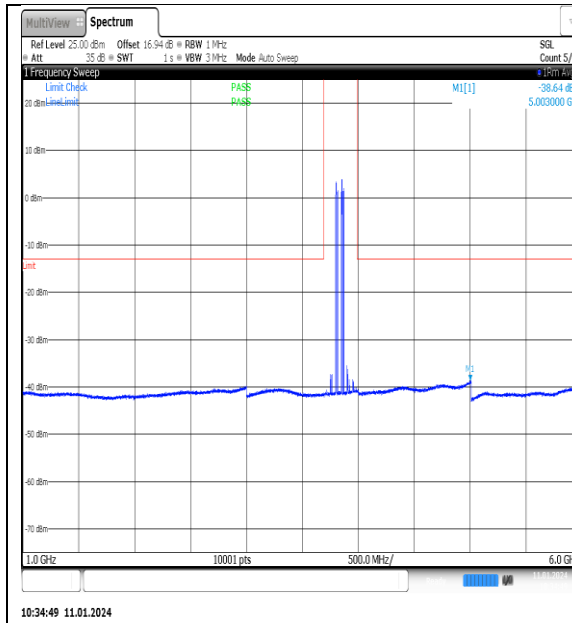
NTN_V_N77-3700- 3980_PC2_30_100_M_TID7_NS_01_1000_6000_ #1
