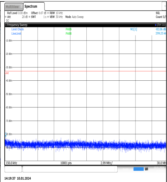
NTNV_N77-3700- 3980_PC2_30_100_M_TID3_NS_01_0.15_30_#1
