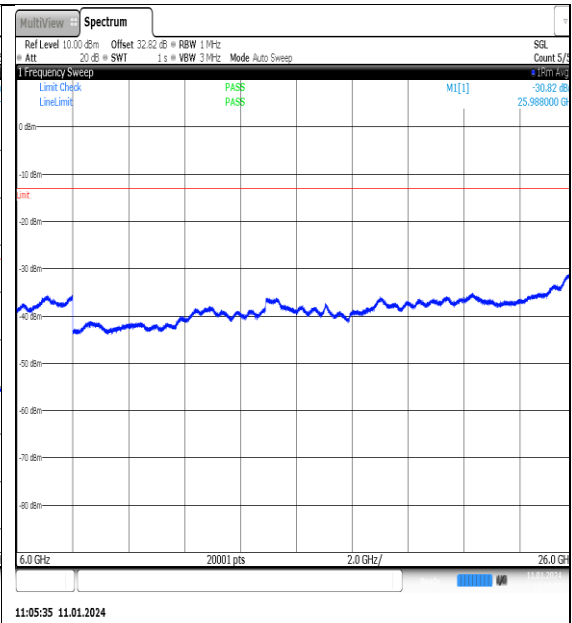
NTN_V_N77-3700- 3980_PC2_30_100_H_TID2_NS_01_6000_26000 #1
