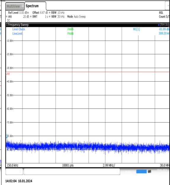
NTNV_N77-3700- 3980_PC2_30_100_L_TID15_NS_01_0.15_30_#1
