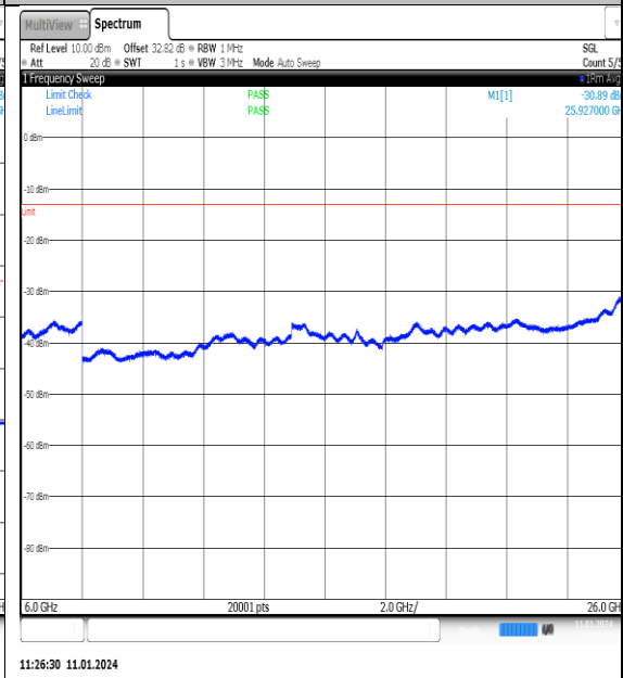
NTNV_N77-3700-3980_PC2_30_100_H_TID7_NS_01_6000_26000_#1
