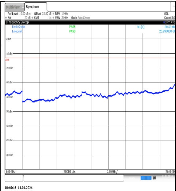
NTN_V_N77-3700- 3980_PC2_30_100_M_TID9_NS_01_6000_26000 #1
