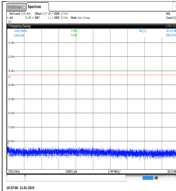
NTNV_N77-3700- 3980_PC2_30_100_M_TID8_NS_01_0.15_30_#1
