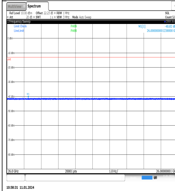
NTN_V_N77-3700- 3980_PC2_30_100_M_TID15_NS_01_26000_400 00_#1
