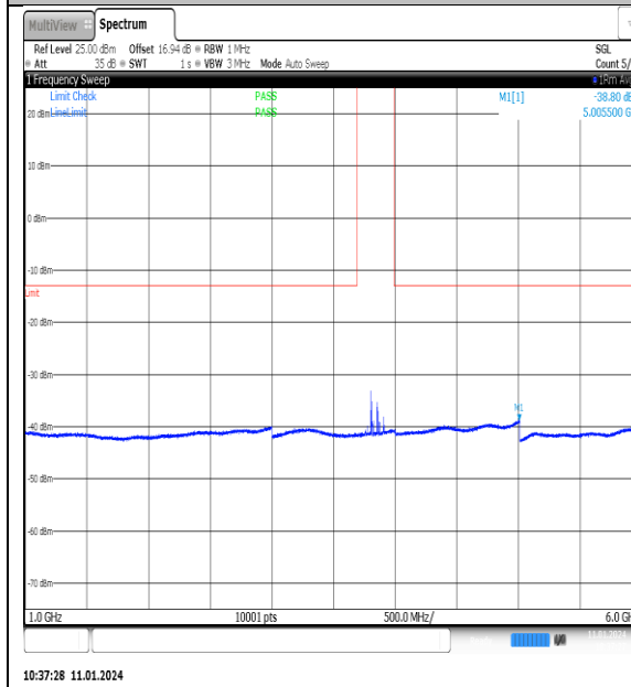
NTNV_N77-3700- 3980_PC2_30_100_M_TID8_NS_01_1000_6000_#1
