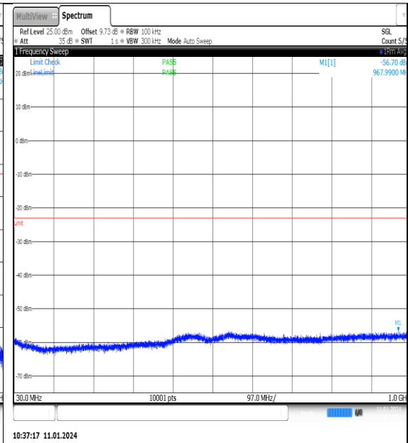
NTNV_N77-3700- 3980_PC2_30_100_M_TID8_NS_01_30_1000_#1
