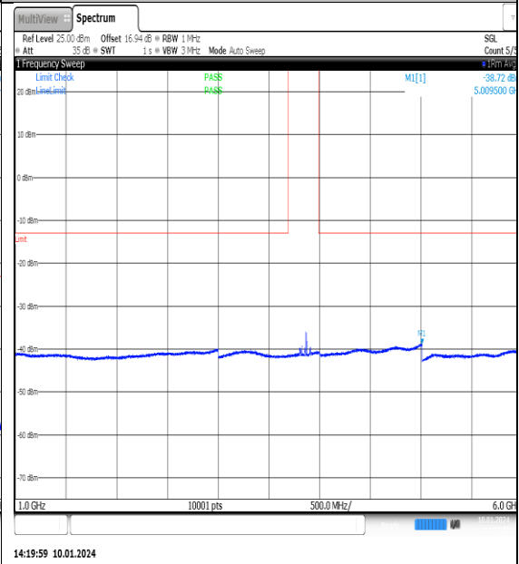
NTNV_N77-3700- 3980_PC2_30_100_M_TID3_NS_01_1000_6000_ #1
