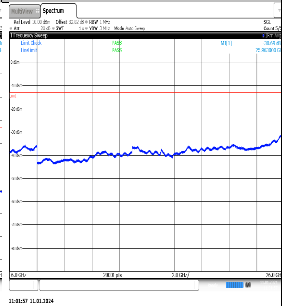
NTNV_N77-3700-3980_PC2_30_100_H_TID1_NS_01_6000_26000_#1
