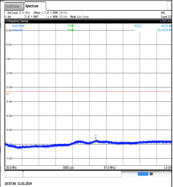
NTNV_N77-3700- 3980_PC2_30_100_M_TID15_NS_01_30_1000_# 1
