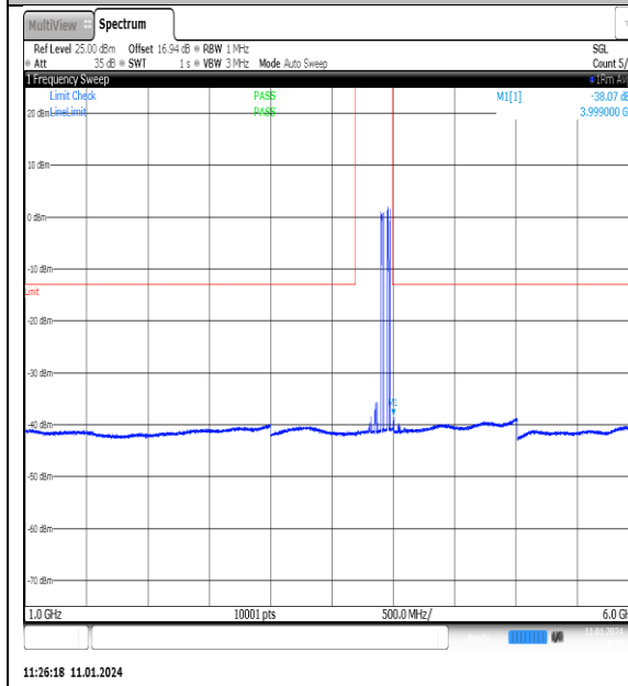
NTNV_N77-3700-3980_PC2_30_100_H_TID7_NS_01_1000_6000_#1
