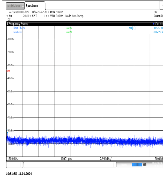
NTNV_N77-3700- 3980_PC2_30_100_M_TID13_NS_01_0.15_30_# 1
