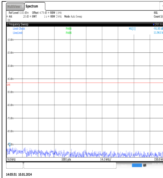
NTNV_N77-3700- 3980_PC2_30_100_M_TID1_NS_01_0.009_0.15_ #1
