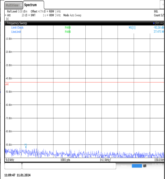
NTN_V_N77-3700- 3980_PC2_30_100_H_TID3_NS_01_0.009_0.15_ #1
