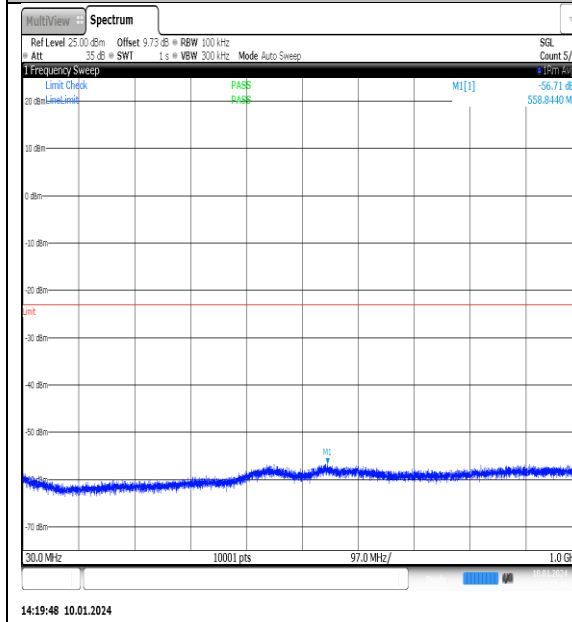
NTNV_N77-3700- 3980_PC2_30_100_M_TID3_NS_01_30_1000_#1
