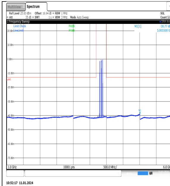
NTN_V_N77-3700- 3980_PC2_30_100_M_TID13_NS_01_1000_6000 #1
