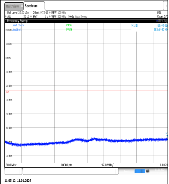
NTNV_N77-3700- 3980_PC2_30_100_H_TID2_NS_01_30_1000_#1
