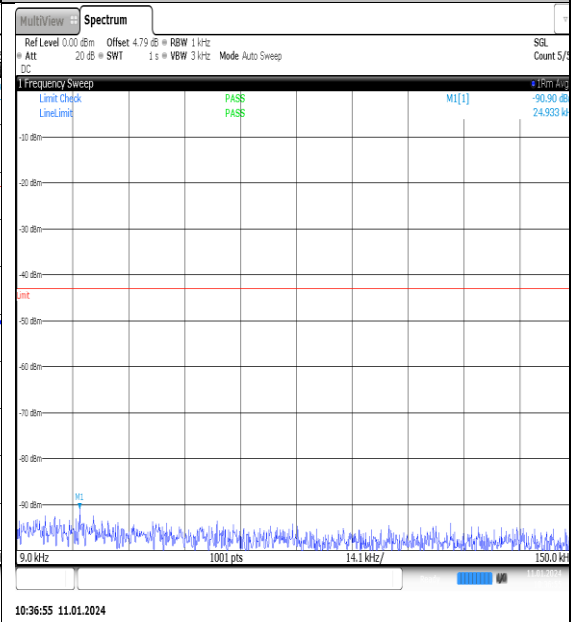
NTN_V_N77-3700- 3980_PC2_30_100_M_TID8_NS_01_0.009_0.15_ #1
