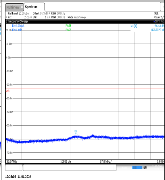
NTNV_N77-3700- 3980_PC2_30_70_M_TID14_NS_01_30_1000_#1
