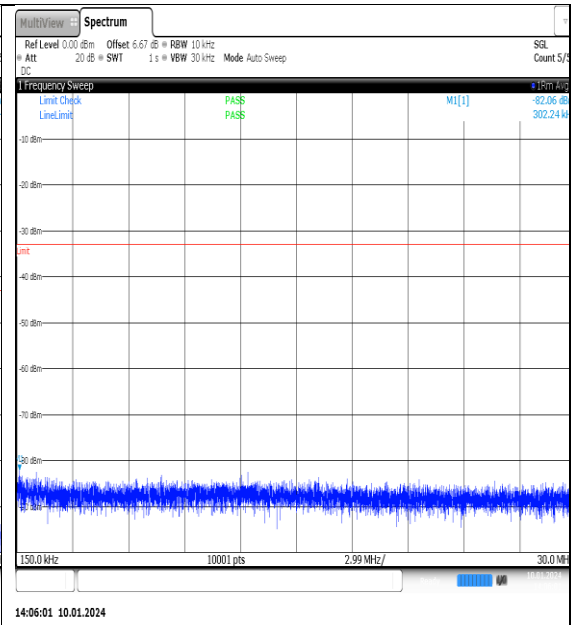
NTNV_N77-3700- 3980_PC2_30_100_M_TID1_NS_01_0.15_30_#1
