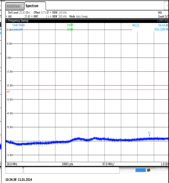
NTNV_N77-3700- 3980_PC2_30_100_M_TID7_NS_01_30_1000_#1
