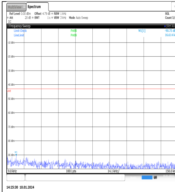
NTNV_N77-3700- 3980_PC2_30_100_M_TID5_NS_01_0.009_0.15_ #1
