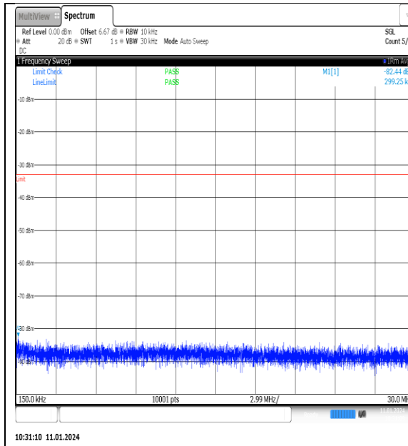
NTNV_N77-3700- 3980_PC2_30_100_M_TID6_NS_01_0.15_30_#1
