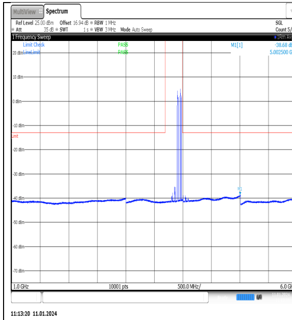
NTN_V_N77-3700- 3980_PC2_30_100_H_TID4_NS_01_1000_6000_ #1
