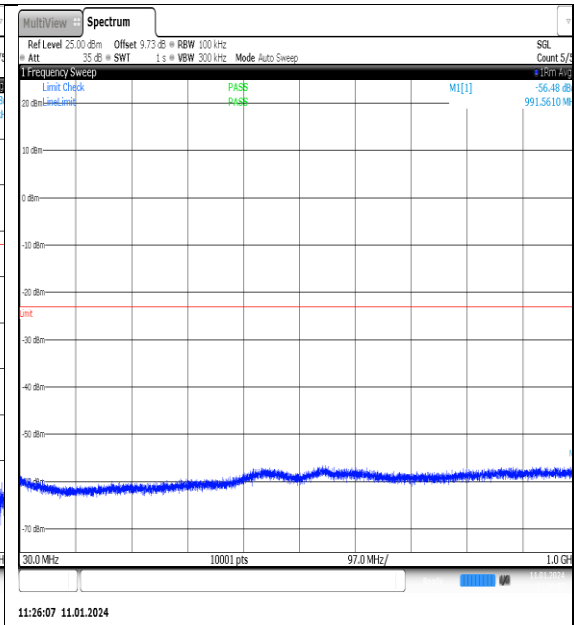
NTNV_N77-3700-3980_PC2_30_100_H_TID7_NS_01_30_1000_#1
