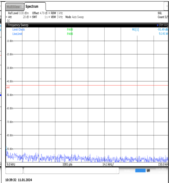
NTNV_N77-3700- 3980_PC2_30_100_M_TID9_NS_01_0.009_0.15_ #1
