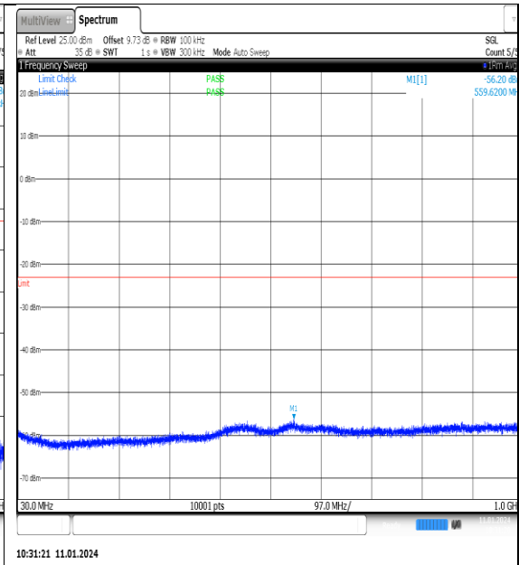
NTNV_N77-3700- 3980_PC2_30_100_M_TID6_NS_01_30_1000_#1
