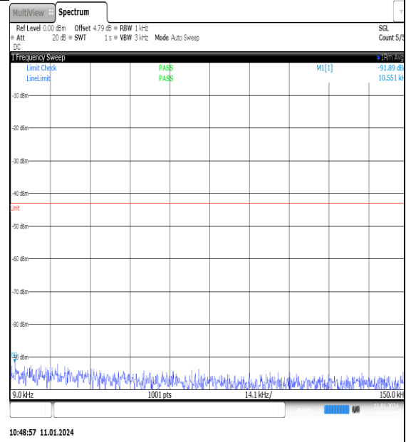
NTNV_N77-3700- 3980_PC2_30_100_M_TID12_NS_01_0.009_0.15 _#1
