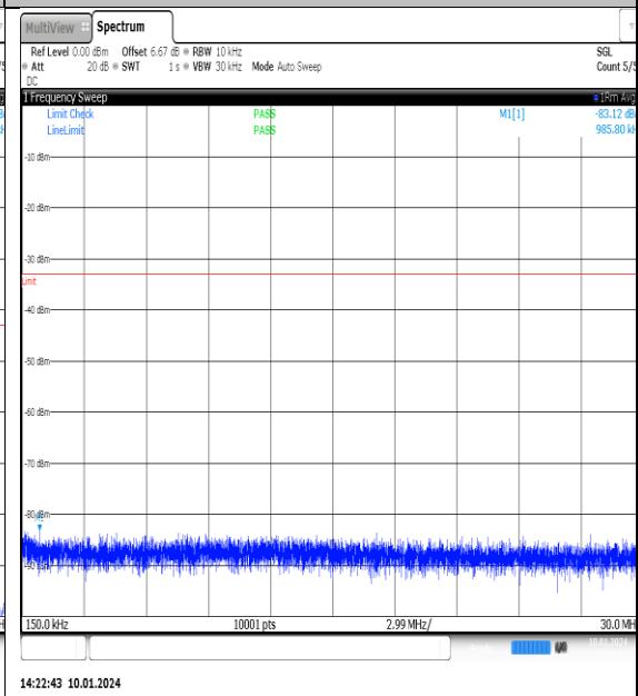
NTNV_N77-3700- 3980_PC2_30_100_M_TID4_NS_01_0.15_30_#1
