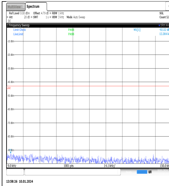
NTNV_N77-3700- 3980_PC2_30_100_L_TID14_NS_01_0.009_0.15 #1
