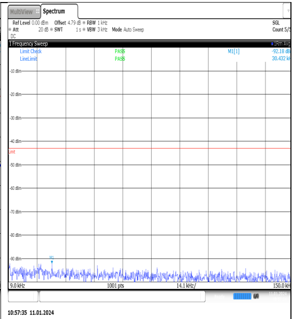
NTNV_N77-3700- 3980_PC2_30_100_M_TID15_NS_01_0.009_0.15 _#1
