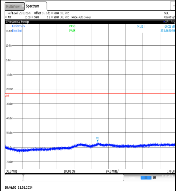
NTNV_N77-3700- 3980_PC2_30_100_M_TID11_NS_01_30_1000_# 1
