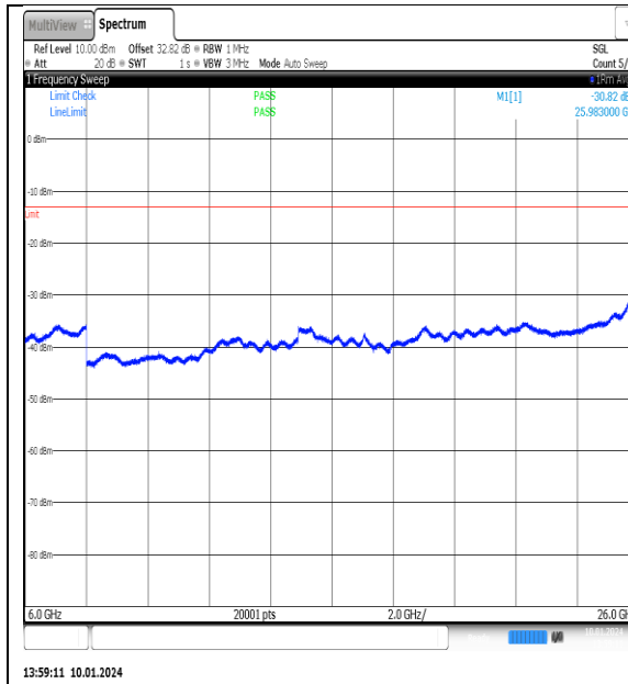
NTNV_N77-3700- 3980_PC2_30_100_L_TID14_NS_01_6000_2600 _0_#1
