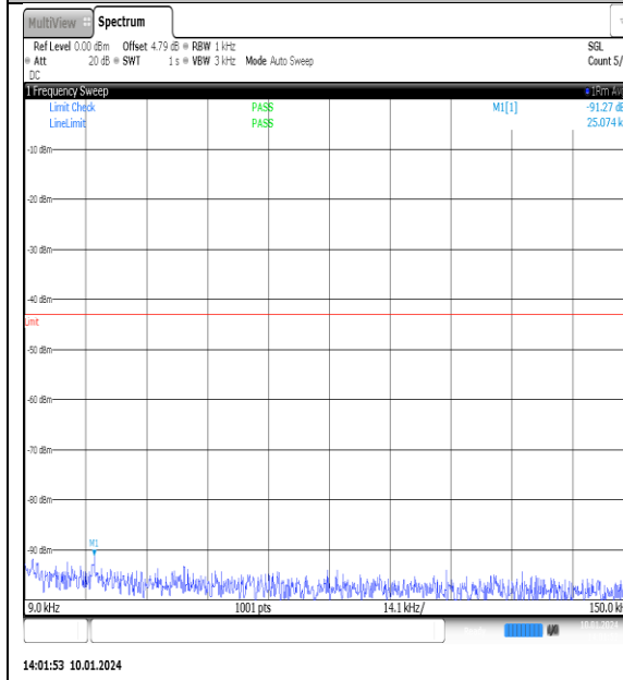
NTNV_N77-3700- 3980_PC2_30_100_L_TID15_NS_01_0.009_0.15 _#1
