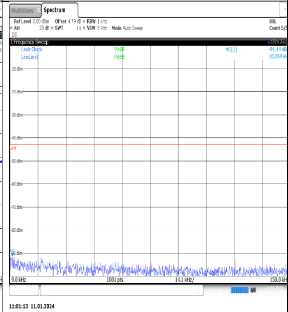
NTN_V_N77-3700- 3980_PC2_30_100_H_TID1_NS_01_0.009_0.15_#1
