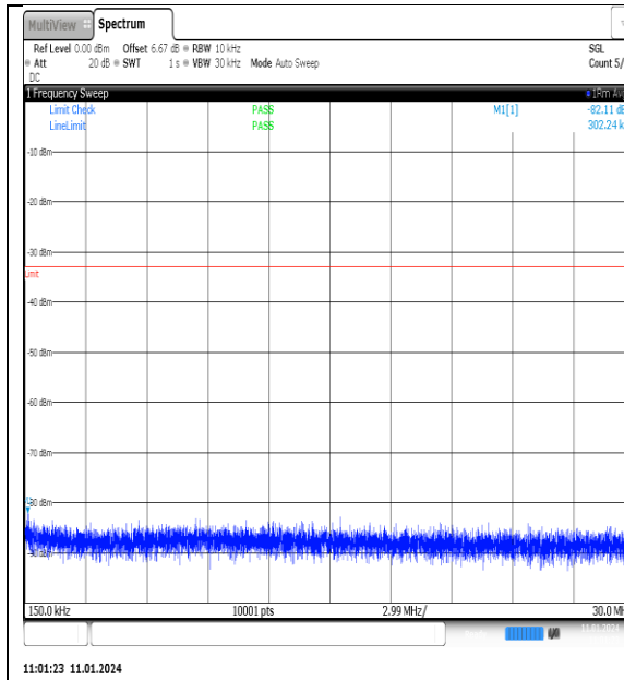
NTNV_N77-3700-3980_PC2_30_100_H_TID1_NS_01_0.15_30_#1
