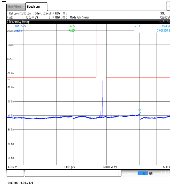
NTN_V_N77-3700- 3980_PC2_30_100_M_TID9_NS_01_1000_6000_ #1
