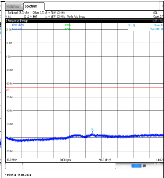
NTNV_N77-3700-3980_PC2_30_100_H_TID1_NS_01_30_1000_#1
