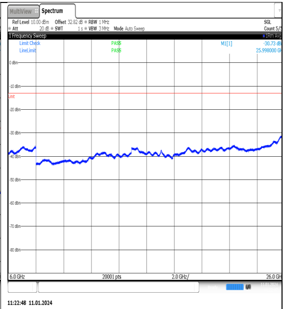
NTN_V_N77-3700- 3980_PC2_30_100_H_TID6_NS_01_6000_26000 #1
