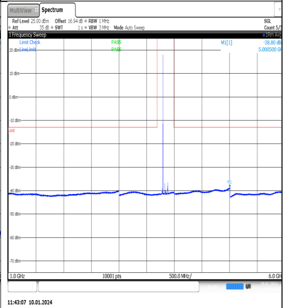
NTN_V_N77-3700- 3980_PC2_30_90_M_TID14_NS_01_1000_6000_ #1
