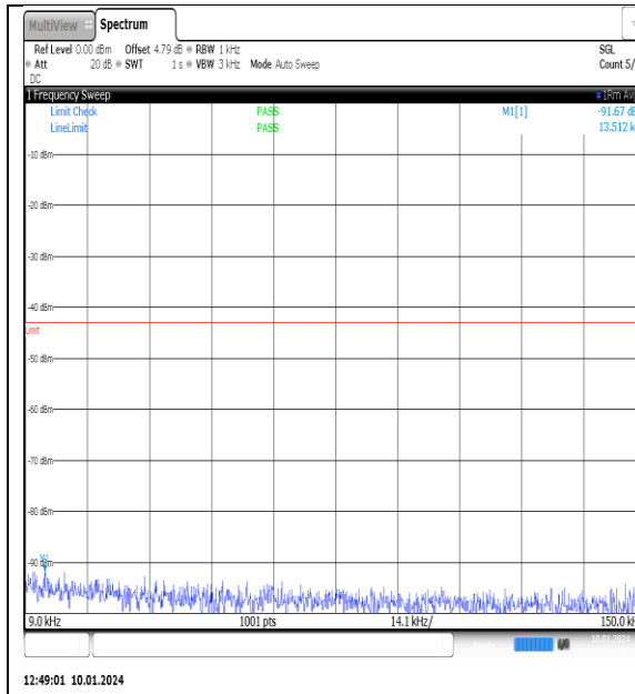
NTN_V_N77-3700- 3980_PC2_30_90_H_TID13_NS_01_0.009_0.15_ #1
