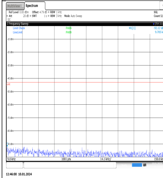
NTNV_N77-3700- 3980_PC2_30_90_H_TID12_NS_01_0.009_0.15_#1
