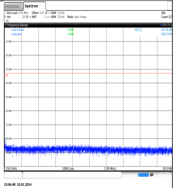
NTNV_N77-3700- 3980_PC2_30_100_L_TID1_NS_01_0.15_30_#1
