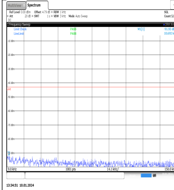
NTNV_N77-3700-3980_PC2_30_100_L_TID9_NS_01_0.009_0.15_#1
