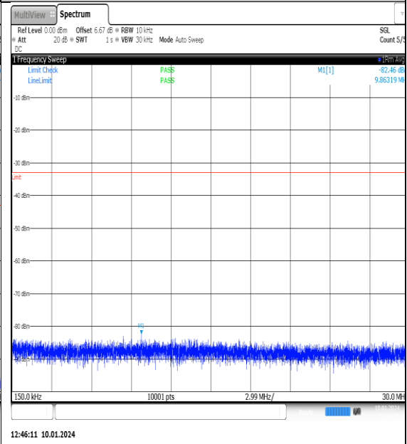
NTNV_N77-3700- 3980_PC2_30_90_H_TID12_NS_01_0.15_30_#1
