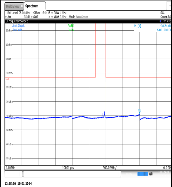
NTNV_N77-3700- 3980_PC2_30_90_H_TID15_NS_01_1000_6000_ #1
