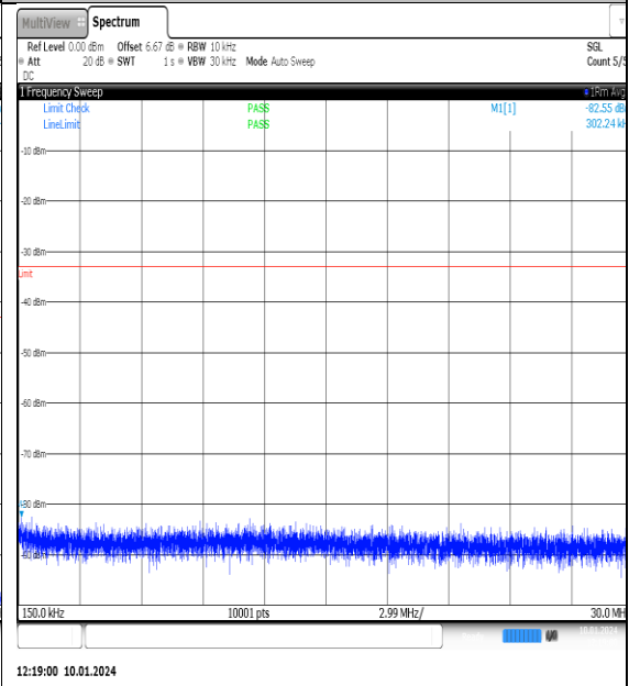
NTNV_N77-3700- 3980_PC2_30_90_H_TID6_NS_01_0.15_30_#1
