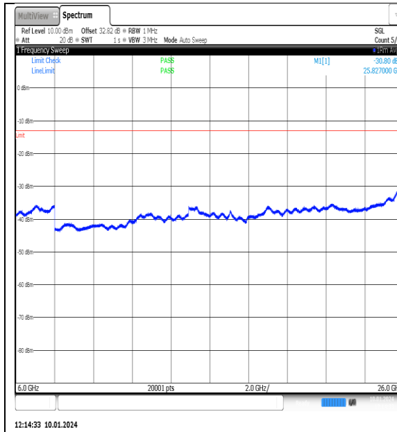
NTNV_N77-3700- 3980_PC2_30_90_H_TID5_NS_01_6000_26000_#1
