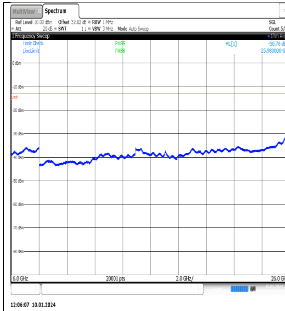
NTNV_N77-3700- 3980_PC2_30_90_H_TID3_NS_01_6000_26000_#1
