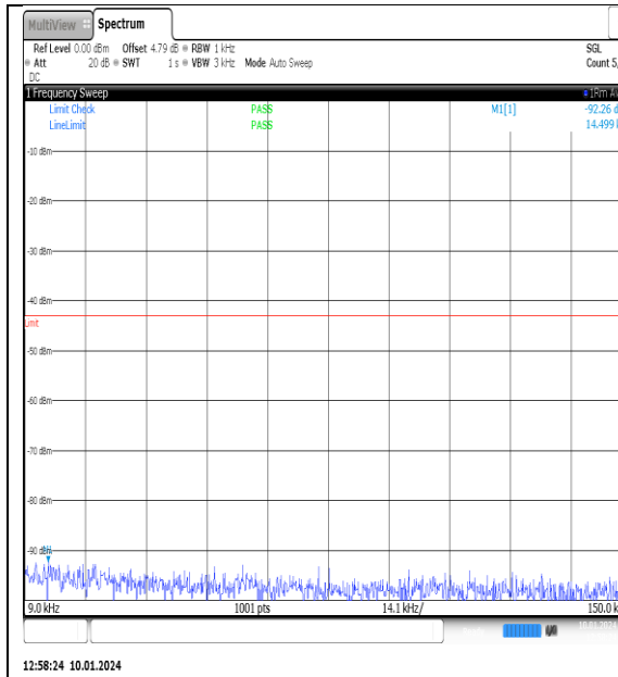
NTNV_N77-3700- 3980_PC2_30_90_H_TID15_NS_01_0.009_0.15_ #1
