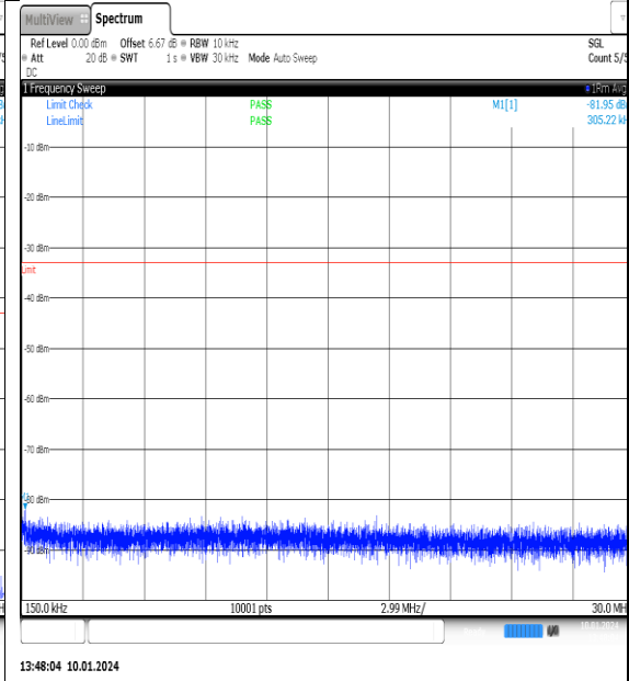
NTNV_N77-3700- 3980_PC2_30_100_L_TID11_NS_01_0.15_30_#1
