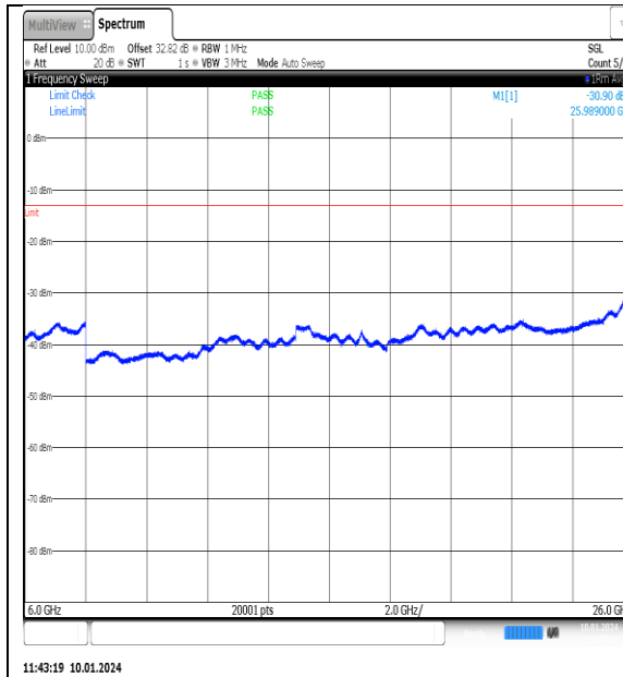
NTNV_N77-3700- 3980_PC2_30_90_M_TID14_NS_01_6000_26000 _#1
