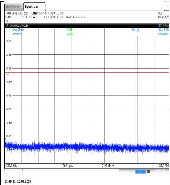
NTN_V_N77-3700- 3980_PC2_30_90_H_TID13_NS_01_0.15_30_#1
