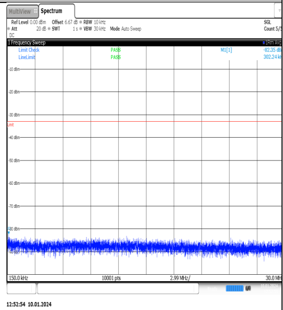
NTNV_N77-3700- 3980_PC2_30_90_H_TID14_NS_01_0.15_30_#1
