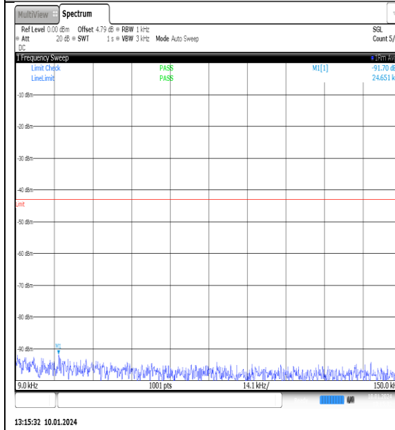
NTNV_N77-3700- 3980_PC2_30_100_L_TID3_NS_01_0.009_0.15_#1
