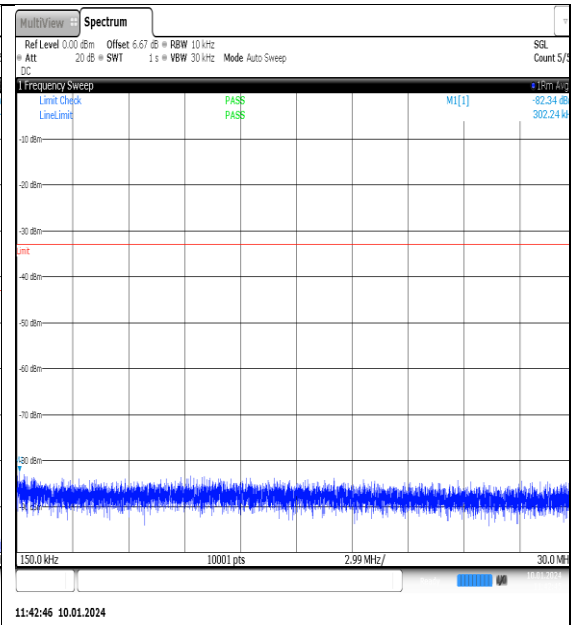
NTN_V_N77-3700- 3980_PC2_30_90_M_TID14_NS_01_0.15_30_#1
