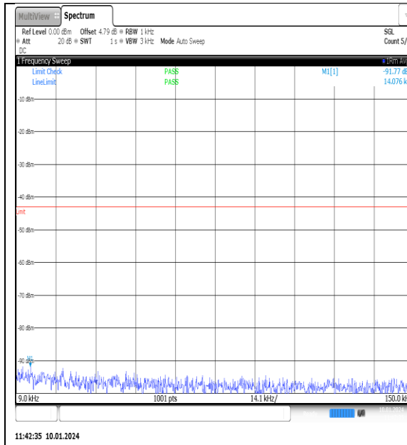
NTN_V_N77-3700- 3980_PC2_30_90_M_TID14_NS_01_0.009_0.15_ #1
