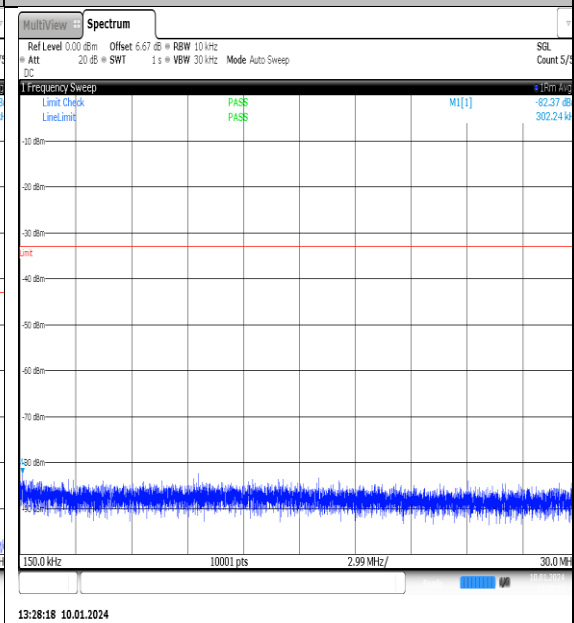
NTNV_N77-3700- 3980_PC2_30_100_L_TID7_NS_01_0.15_30_#1
