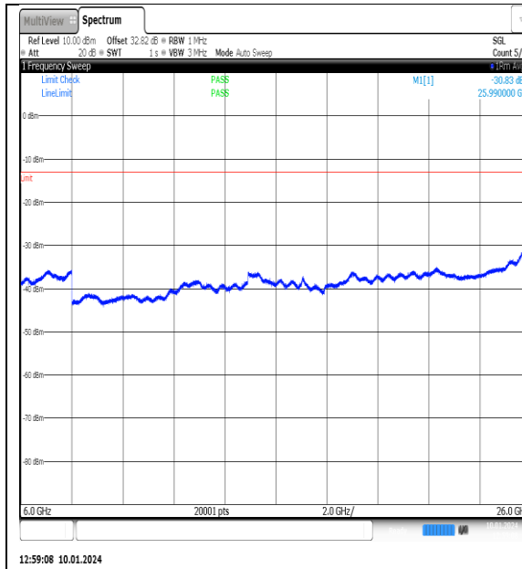
NTNV_N77-3700- 3980_PC2_30_90_H_TID15_NS_01_6000_26000 _#1
