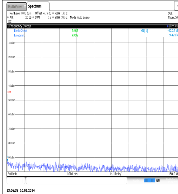
NTNV_N77-3700- 3980_PC2_30_100_L_TID1_NS_01_0.009_0.15_#1
