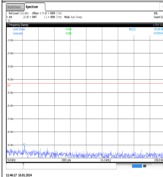
NTNV_N77-3700- 3980_PC2_30_90_M_TID15_NS_01_0.009_0.15_#1
