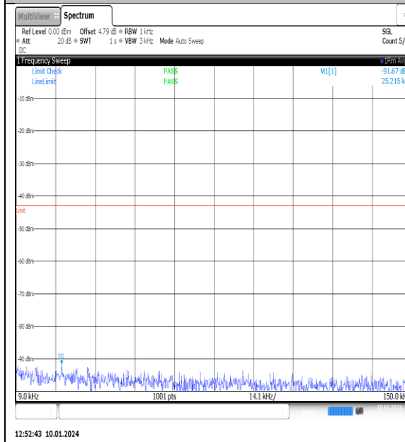
NTNV_N77-3700- 3980_PC2_30_90_H_TID14_NS_01_0.009_0.15_#1
