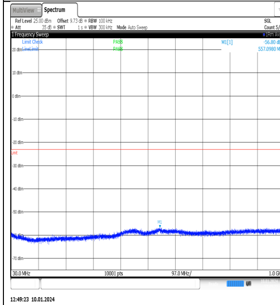
NTN_V_N77-3700- 3980_PC2_30_90_H_TID13_NS_01_30_1000_#1
