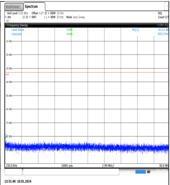
NTNV_N77-3700- 3980_PC2_30_100_L_TID8_NS_01_0.15_30_#1
