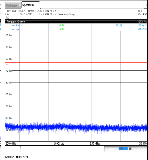
NTNV_N77-3700- 3980_PC2_30_90_H_TID4_NS_01_0.15_30_#1
