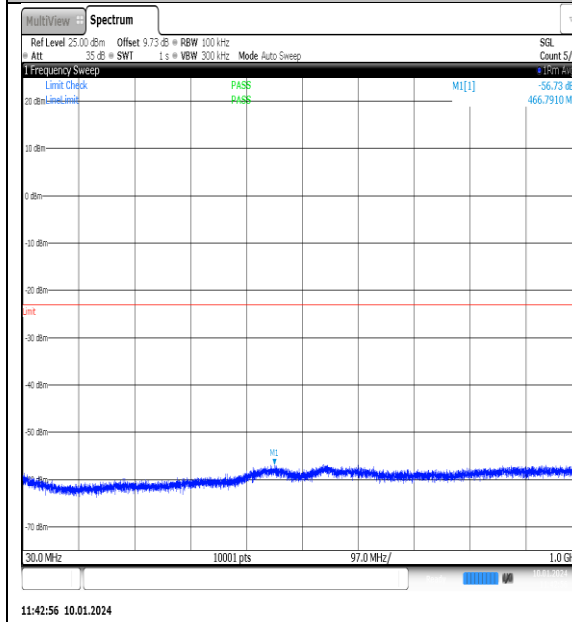
NTN_V_N77-3700- 3980_PC2_30_90_M_TID14_NS_01_30_1000_#1
