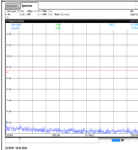
NTNV_N77-3700- 3980_PC2_30_100_L_TID7_NS_01_0.009_0.15_#1
