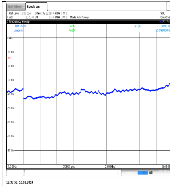
NTNV_N77-3700- 3980_PC2_30_90_H_TID9_NS_01_6000_26000_#1
