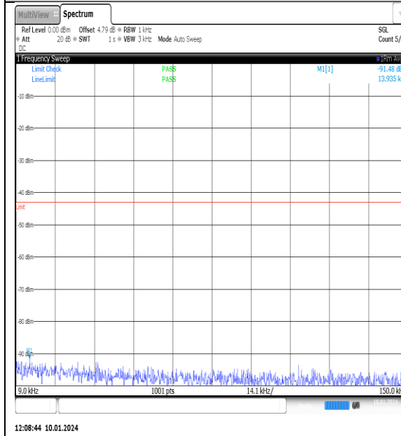
NTNV_N77-3700- 3980_PC2_30_90_H_TID4_NS_01_0.009_0.15_#1
