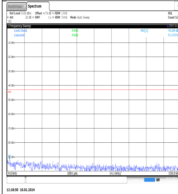
NTNV_N77-3700- 3980_PC2_30_90_H_TID6_NS_01_0.009_0.15_#1
