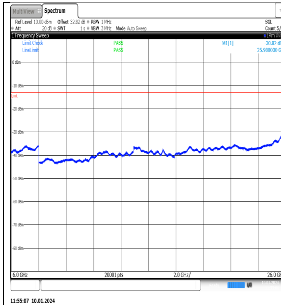
NTNV_N77-3700- 3980_PC2_30_90_H_TID1_NS_01_6000_26000_#1
