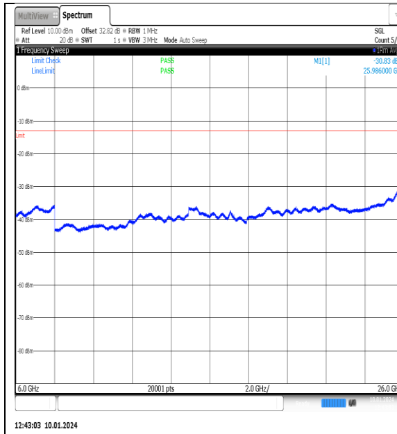
NTNV_N77-3700- 3980_PC2_30_90_H_TID11_NS_01_6000_26000 #1
