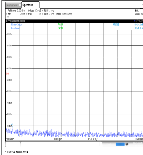
NTNV_N77-3700- 3980_PC2_30_90_H_TID2_NS_01_0.009_0.15_#1
