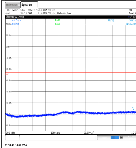
NTNV_N77-3700- 3980_PC2_30_90_H_TID15_NS_01_30_1000_#1
