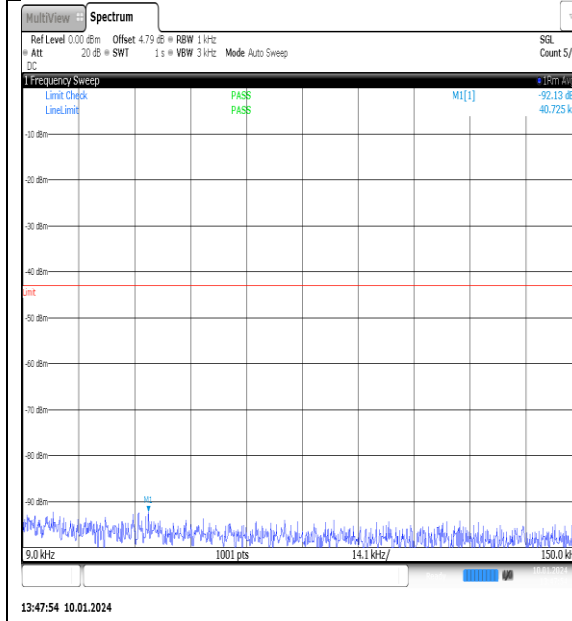
NTNV_N77-3700- 3980_PC2_30_100_L_TID11_NS_01_0.009_0.15 _#1
