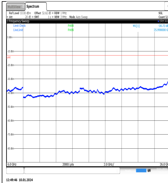
NTNV_N77-3700- 3980_PC2_30_90_H_TID13_NS_01_6000_26000 _#1
