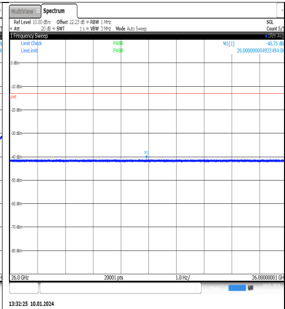
NTNV_N77-3700-3980_PC2_30_100_L_TID8_NS_01_26000_4000_0_#1
