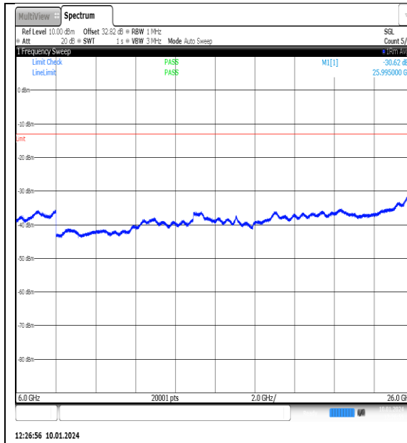
NTNV_N77-3700- 3980_PC2_30_90_H_TID7_NS_01_6000_26000_ #1
