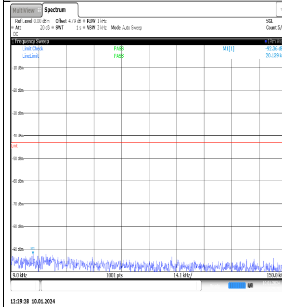
NTNV_N77-3700- 3980_PC2_30_90_H_TID8_NS_01_0.009_0.15_# 1
