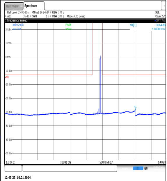
NTN_V_N77-3700- 3980_PC2_30_90_H_TID13_NS_01_1000_6000_ #1
