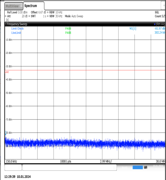
NTNV_N77-3700- 3980_PC2_30_90_H_TID8_NS_01_0.15_30_#1
