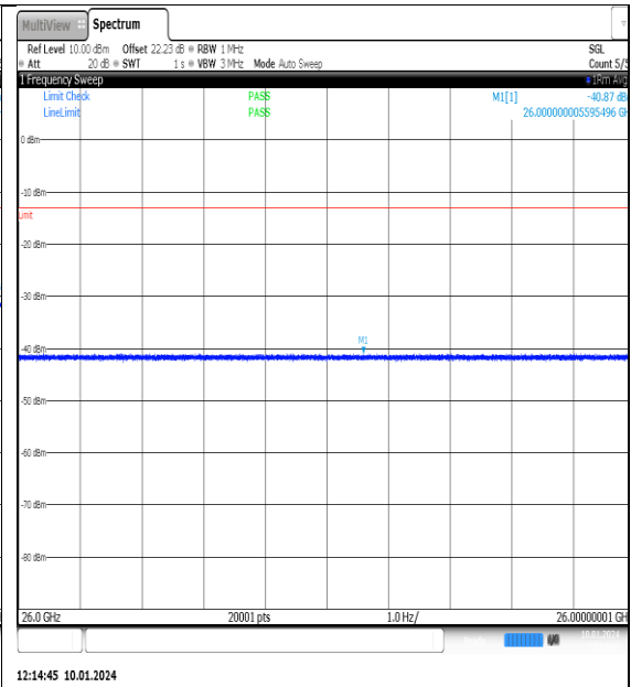
NTNV_N77-3700- 3980_PC2_30_90_H_TID5_NS_01_26000_40000_#1
