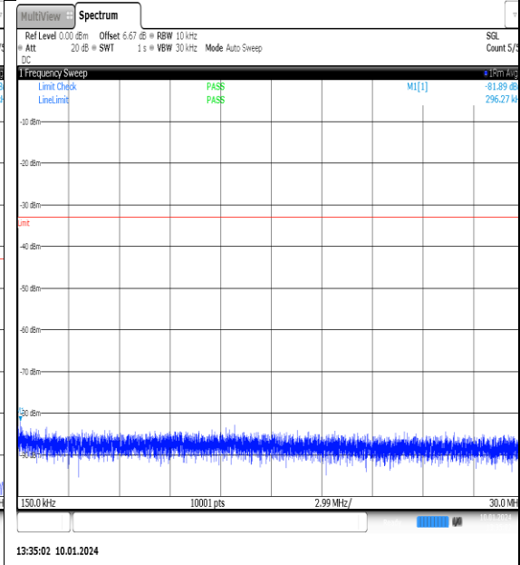
NTNV_N77-3700-3980_PC2_30_100_L_TID9_NS_01_0.15_30_#1
