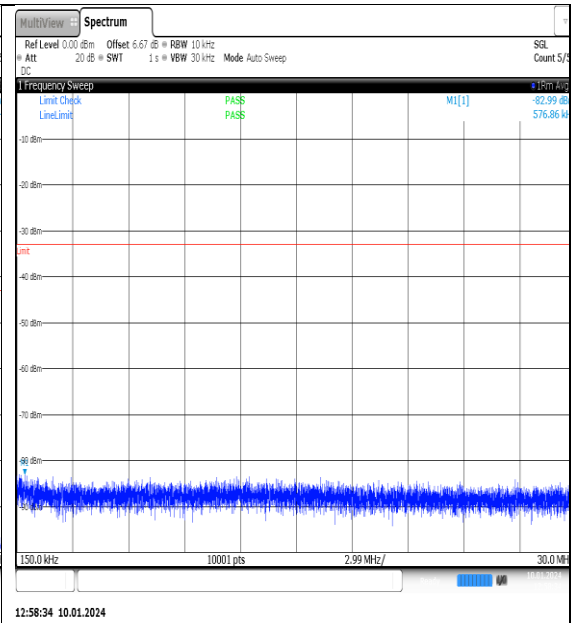
NTNV_N77-3700- 3980_PC2_30_90_H_TID15_NS_01_0.15_30_#1
