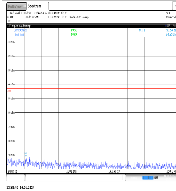
NTNV_N77-3700- 3980_PC2_30_90_H_TID10_NS_01_0.009_0.15_#1
