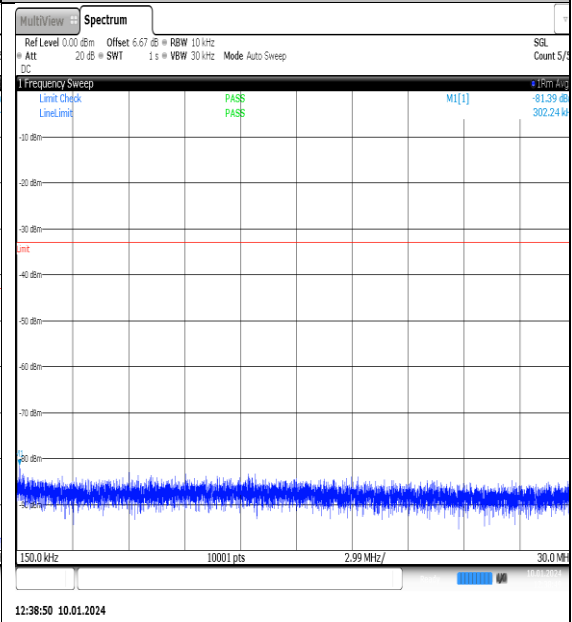
NTNV_N77-3700- 3980_PC2_30_90_H_TID10_NS_01_0.15_30_#1
