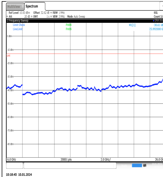
NTNV_N77-3700- 3980_PC2_30_90_L_TID11_NS_01_6000_26000 _#1
