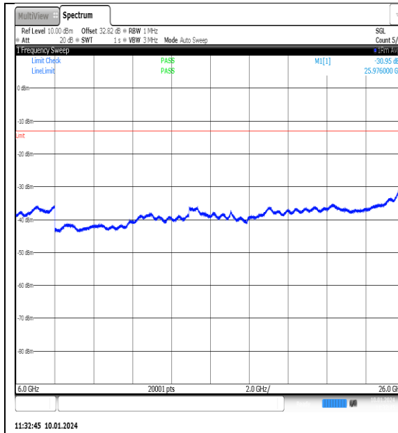
NTNV_N77-3700- 3980_PC2_30_90_M_TID12_NS_01_6000_26000 _#1
