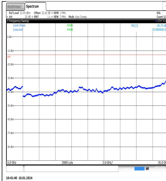
NTNV_N77-3700- 3980_PC2_30_90_M_TID2_NS_01_6000_26000_#1
