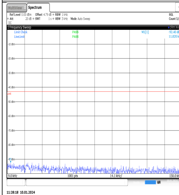
NTNV_N77-3700- 3980_PC2_30_90_M_TID11_NS_01_0.009_0.15_#1
