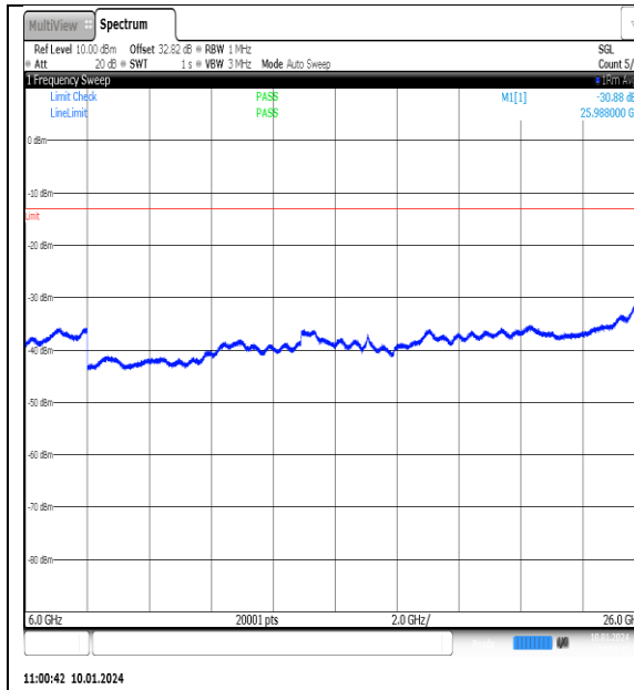
NTNV_N77-3700- 3980_PC2_30_90_M_TID6_NS_01_6000_26000_ #1
