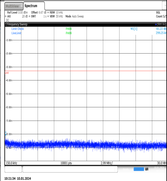
NTNV_N77-3700- 3980_PC2_30_90_L_TID12_NS_01_0.15_30_#1
