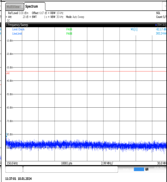
NTNV_N77-3700- 3980_PC2_30_90_M_TID13_NS_01_0.15_30_#1
