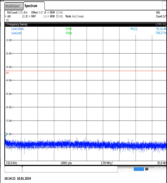
NTNV_N77-3700- 3980_PC2_30_90_L_TID10_NS_01_0.15_30_#1
