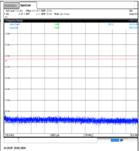
NTN_V_N77-3700- 3980_PC2_30_90_M_TID10_NS_01_0.15_30_#1
