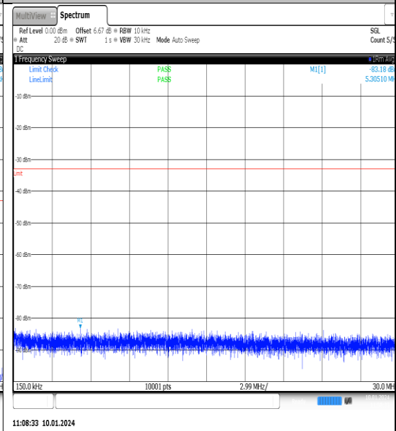
NTNV_N77-3700- 3980_PC2_30_90_M_TID7_NS_01_0.15_30_#1
