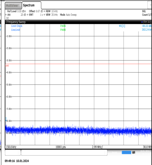
NTNV_N77-3700- 3980_PC2_30_90_L_TID4_NS_01_0.15_30_#1
