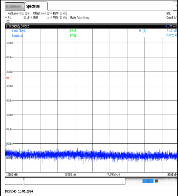
NTNV_N77-3700- 3980_PC2_30_90_L_TID8_NS_01_0.15_30_#1
