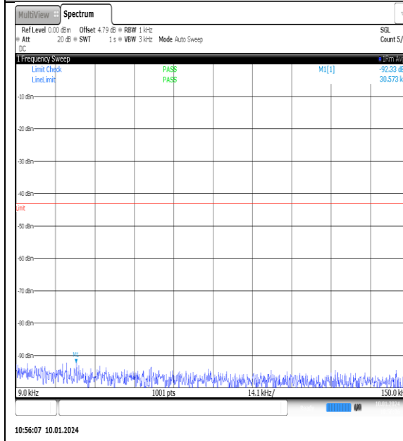
NTNV_N77-3700- 3980_PC2_30_90_M_TID5_NS_01_0.009_0.15_#1
