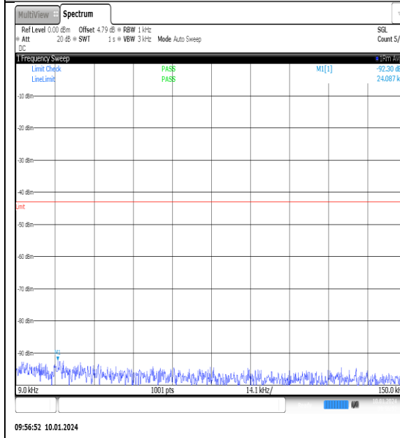
NTNV_N77-3700- 3980_PC2_30_90_L_TID6_NS_01_0.009_0.15_#1
