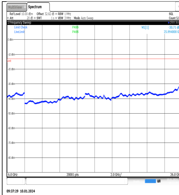
NTNV_N77-3700- 3980_PC2_30_90_L_TID1_NS_01_6000_26000_ #1
