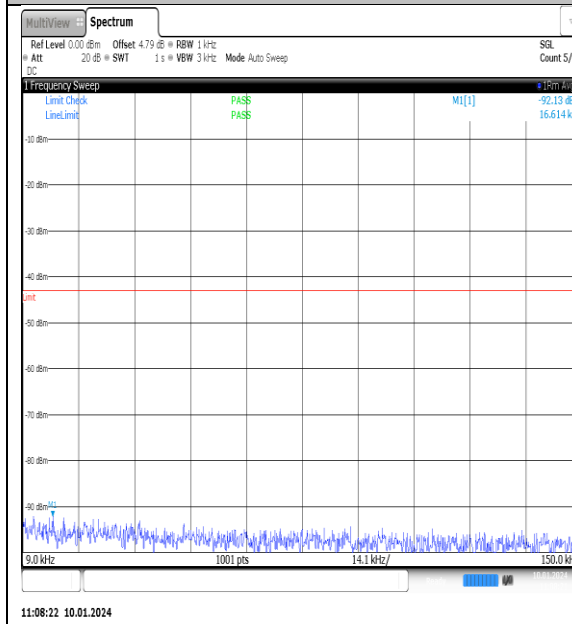
NTNV_N77-3700- 3980_PC2_30_90_M_TID7_NS_01_0.009_0.15_# 1
