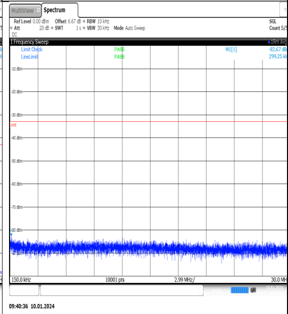
NTNV_N77-3700- 3980_PC2_30_90_L_TID2_NS_01_0.15_30_#1
