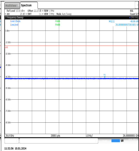
NTNV_N77-3700- 3980_PC2_30_90_M_TID12_NS_01_26000_4000 0_#1
