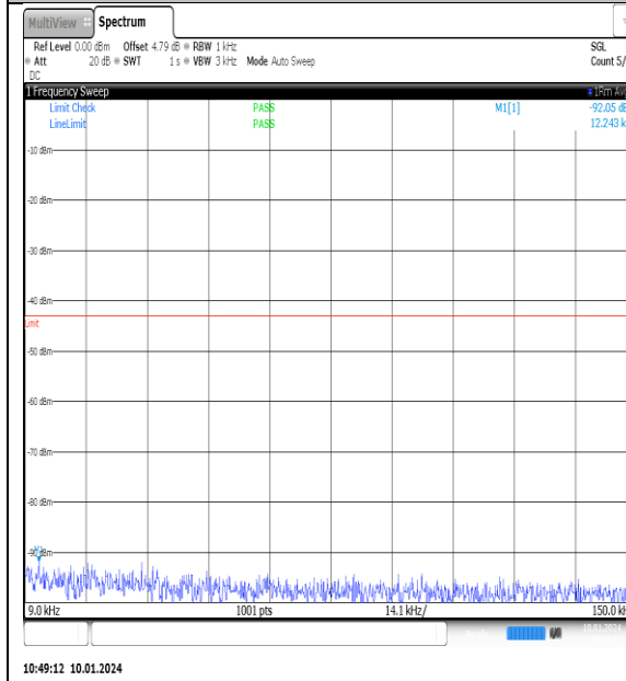
NTNV_N77-3700- 3980_PC2_30_90_M_TID3_NS_01_0.009_0.15_#1
