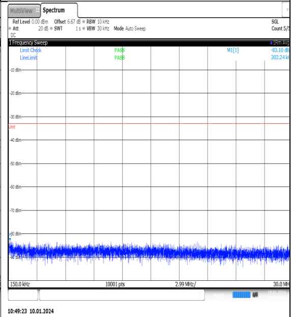
NTNV_N77-3700- 3980_PC2_30_90_M_TID3_NS_01_0.15_30_#1
