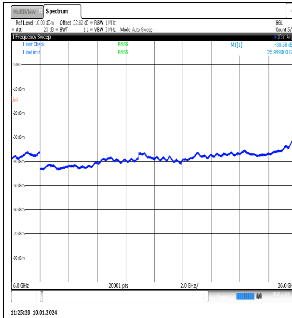
NTNV_N77-3700- 3980_PC2_30_90_M_TID10_NS_01_6000_26000 #1
