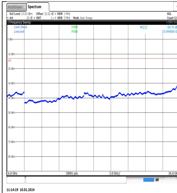
NTNV_N77-3700- 3980_PC2_30_90_M_TID8_NS_01_6000_26000_ #1
