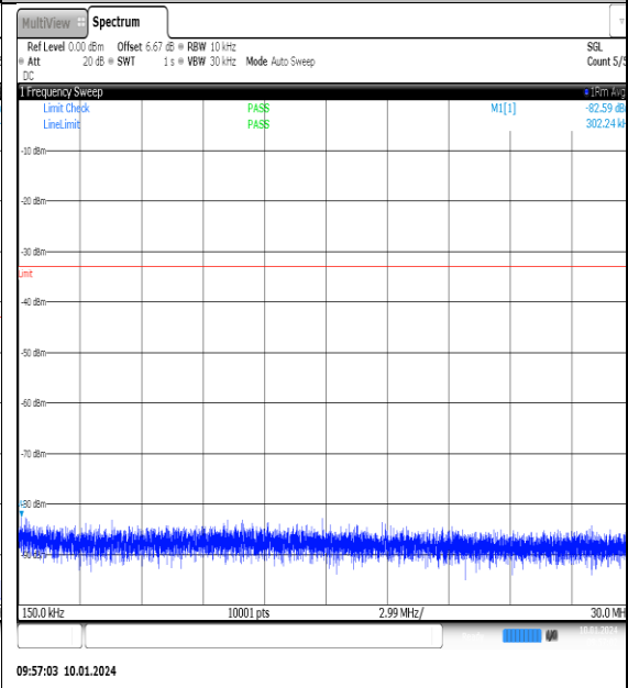
NTNV_N77-3700- 3980_PC2_30_90_L_TID6_NS_01_0.15_30_#1
