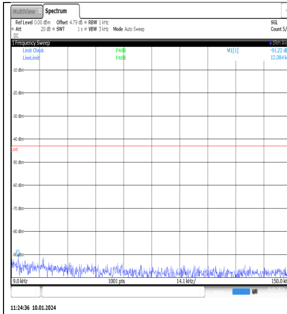
NTN_V_N77-3700- 3980_PC2_30_90_M_TID10_NS_01_0.009_0.15_ #1
