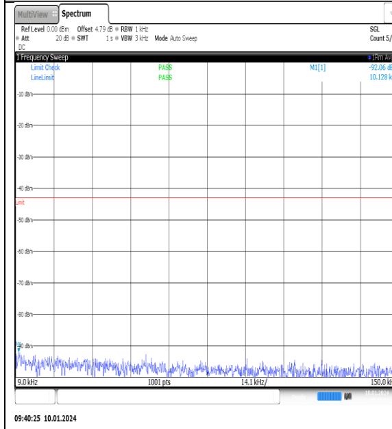
NTNV_N77-3700- 3980_PC2_30_90_L_TID2_NS_01_0.009_0.15_# 1
