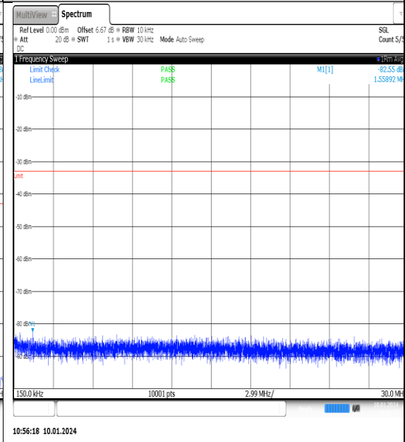
NTNV_N77-3700- 3980_PC2_30_90_M_TID5_NS_01_0.15_30_#1
