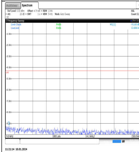
NTNV_N77-3700- 3980_PC2_30_90_M_TID9_NS_01_0.009_0.15_# 1
