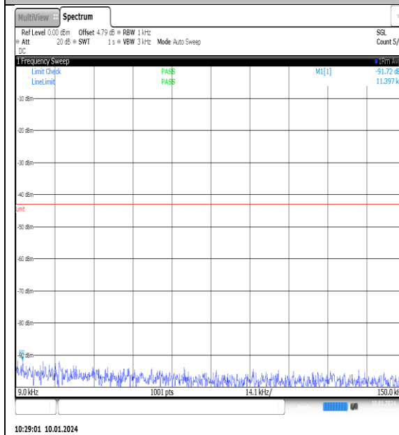
NTNV_N77-3700- 3980_PC2_30_90_L_TID14_NS_01_0.009_0.15_#1
