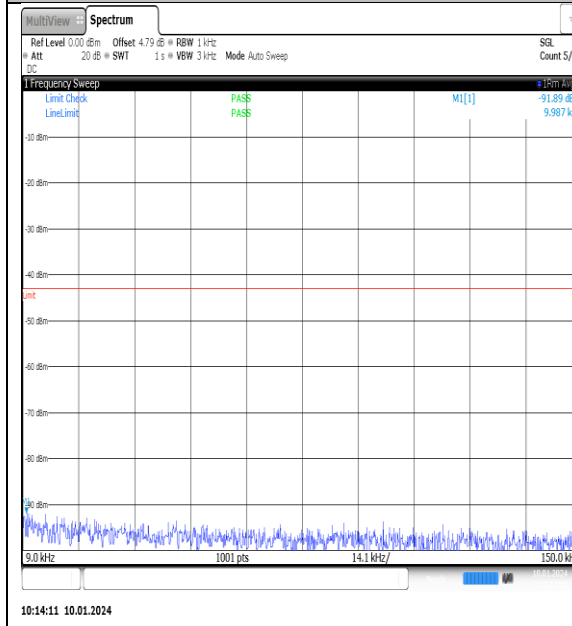
NTNV_N77-3700- 3980_PC2_30_90_L_TID10_NS_01_0.009_0.15_#1
