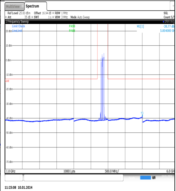
NTN_V_N77-3700- 3980_PC2_30_90_M_TID10_NS_01_1000_6000_ #1
