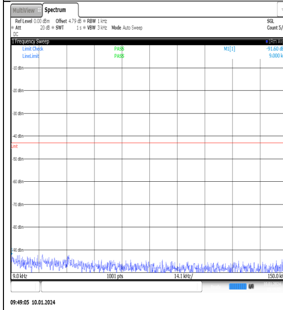
NTNV_N77-3700- 3980_PC2_30_90_L_TID4_NS_01_0.009_0.15_#1
