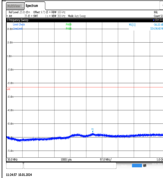
NTN_V_N77-3700- 3980_PC2_30_90_M_TID10_NS_01_30_1000_#1
