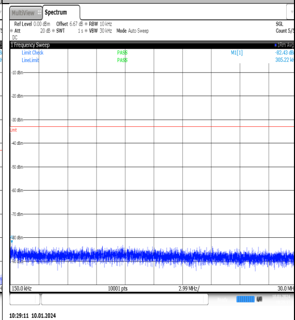
NTNV_N77-3700- 3980_PC2_30_90_L_TID14_NS_01_0.15_30_#1
