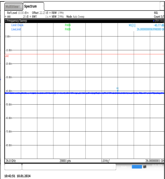
NTNV_N77-3700- 3980_PC2_30_90_M_TID2_NS_01_26000_40000_#1
