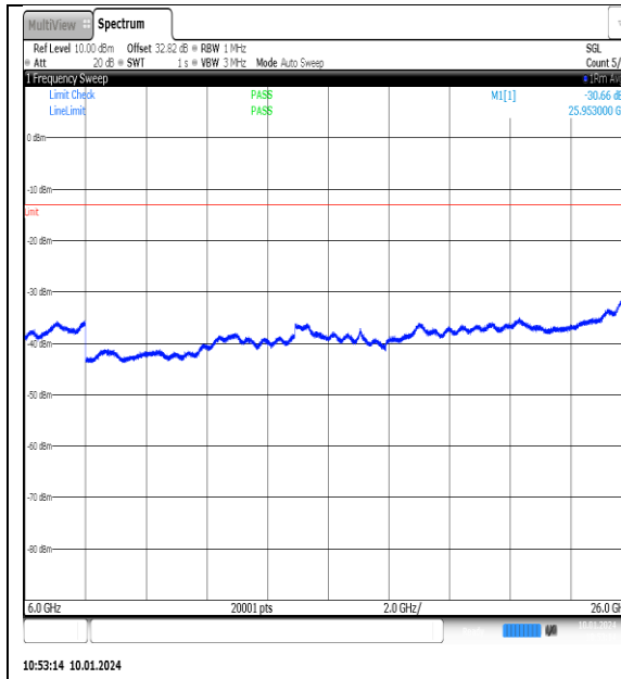
NTNV_N77-3700- 3980_PC2_30_90_M_TID4_NS_01_6000_26000_#1
