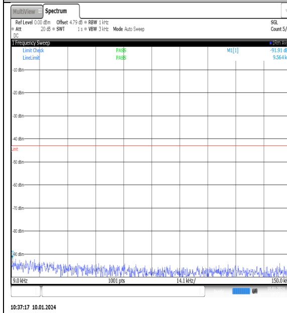
NTNV_N77-3700- 3980_PC2_30_90_M_TID1_NS_01_0.009_0.15_# 1
