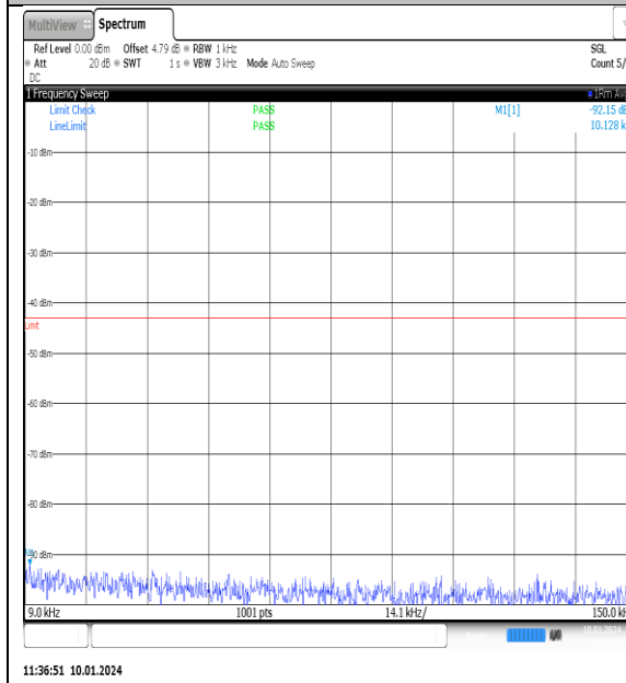
NTNV_N77-3700- 3980_PC2_30_90_M_TID13_NS_01_0.009_0.15_#1
