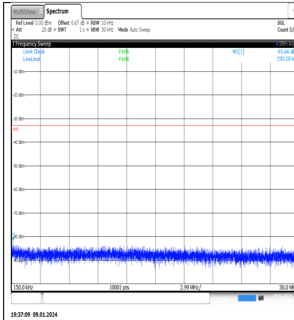
NTNV_N77-3700- 3980_PC2_30_80_M_TID4_NS_01_0.15_30_#1
