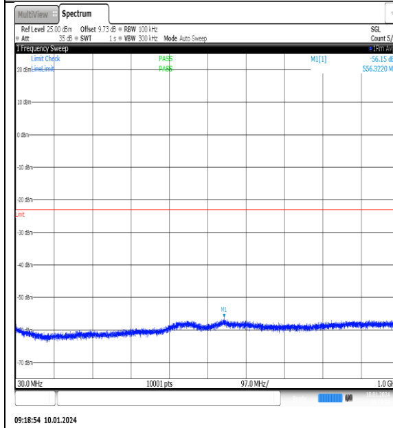
NTNV_N77-3700- 3980_PC2_30_80_H_TID12_NS_01_30_1000_#1
