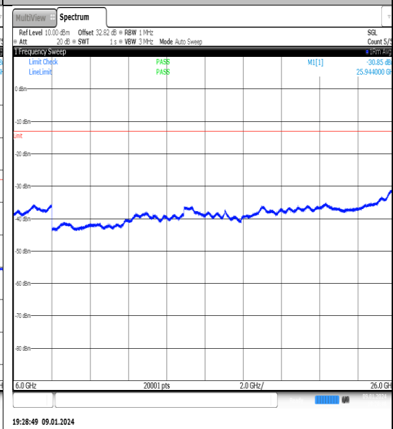
NTNV_N77-3700- 3980_PC2_30_80_M_TID2_NS_01_6000_26000_#1
