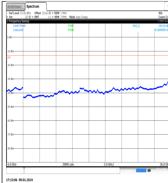
NTNV_N77-3700- 3980_PC2_30_70_H_TID10_NS_01_6000_26000 _#1
