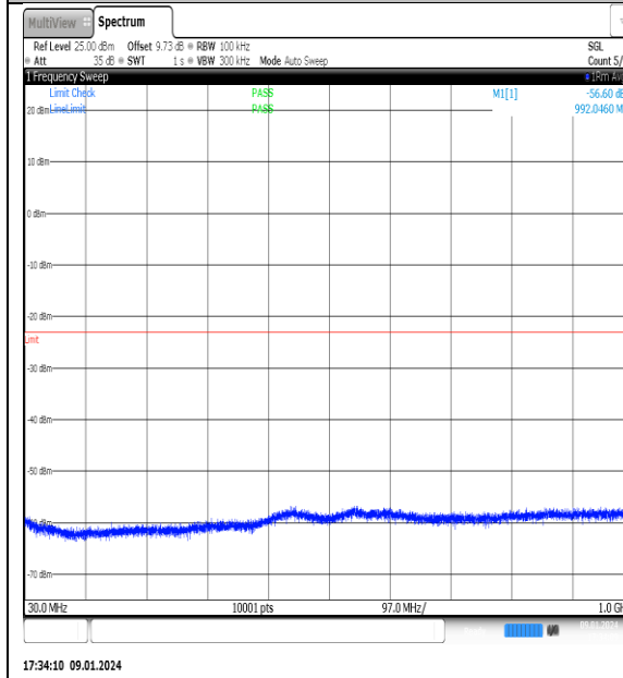
NTN_V_N77-3700- 3980_PC2_30_70_H_TID14_NS_01_30_1000_#1
