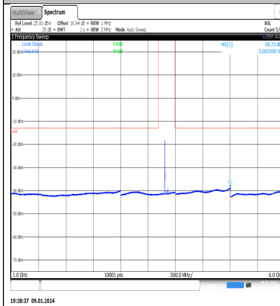
NTNV_N77-3700- 3980_PC2_30_80_M_TID2_NS_01_1000_6000_#1
