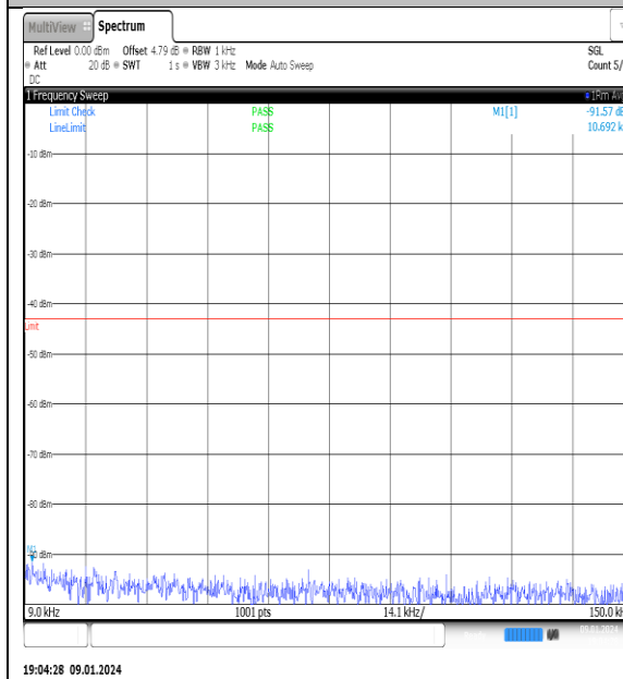
NTNV_N77-3700- 3980_PC2_30_80_L_TID14_NS_01_0.009_0.15_#1
