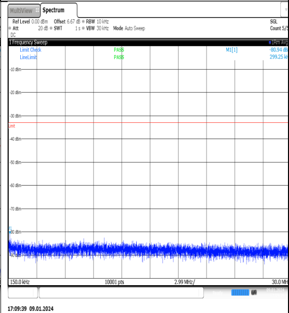
NTNV_N77-3700- 3980_PC2_30_70_H_TID9_NS_01_0.15_30_#1
