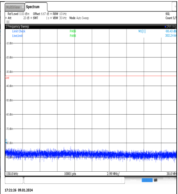
NTNV_N77-3700- 3980_PC2_30_70_H_TID12_NS_01_0.15_30_#1
