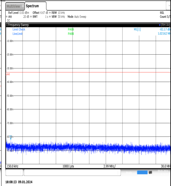
NTNV_N77-3700- 3980_PC2_30_80_L_TID4_NS_01_0.15_30_#1
