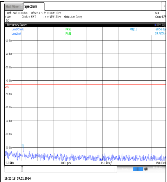
NTNV_N77-3700- 3980_PC2_30_80_M_TID1_NS_01_0.009_0.15_# 1
