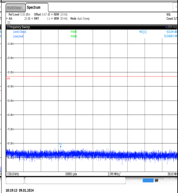
NTNV_N77-3700- 3980_PC2_30_80_L_TID6_NS_01_0.15_30_#1
