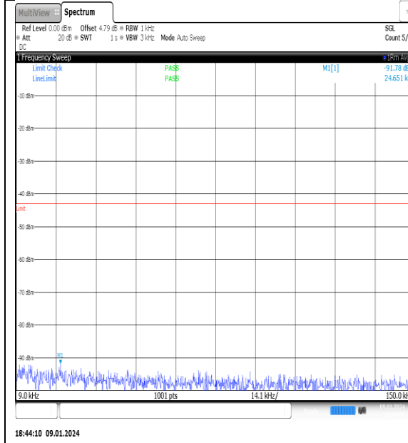
NTNV_N77-3700- 3980_PC2_30_80_L_TID12_NS_01_0.009_0.15_#1
