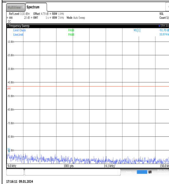
NTNV_N77-3700- 3980_PC2_30_70_H_TID11_NS_01_0.009_0.15_#1
