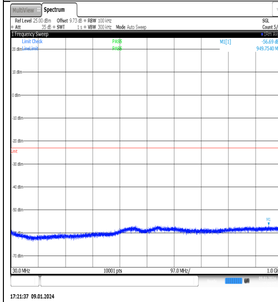
NTNV_N77-3700- 3980_PC2_30_70_H_TID12_NS_01_30_1000_#1
