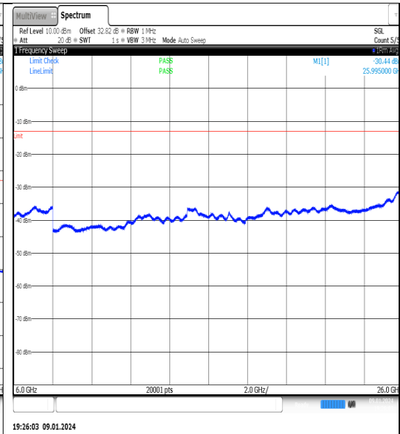
19:26:03 09.01.2024 NTNV_N77-3700- 3980_PC2_30_80_M_TID1_NS_01_6000_26000_# #1
