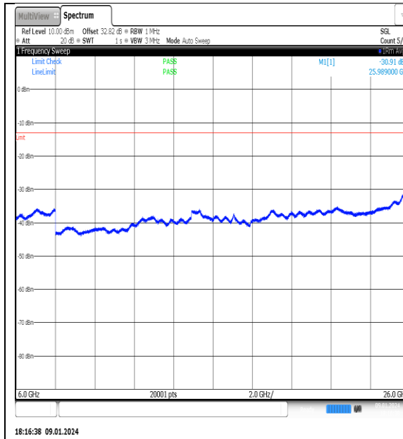
NTNV_N77-3700- 3980_PC2_30_80_L_TID5_NS_01_6000_26000_ #1
