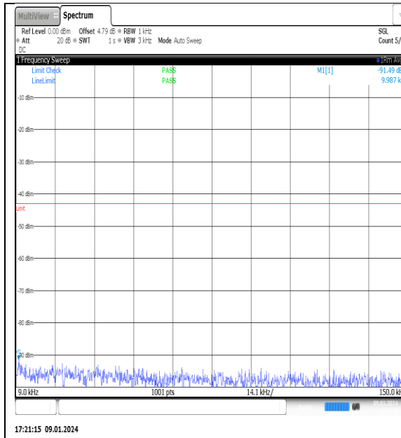
NTNV_N77-3700- 3980_PC2_30_70_H_TID12_NS_01_0.009_0.15_ #1
