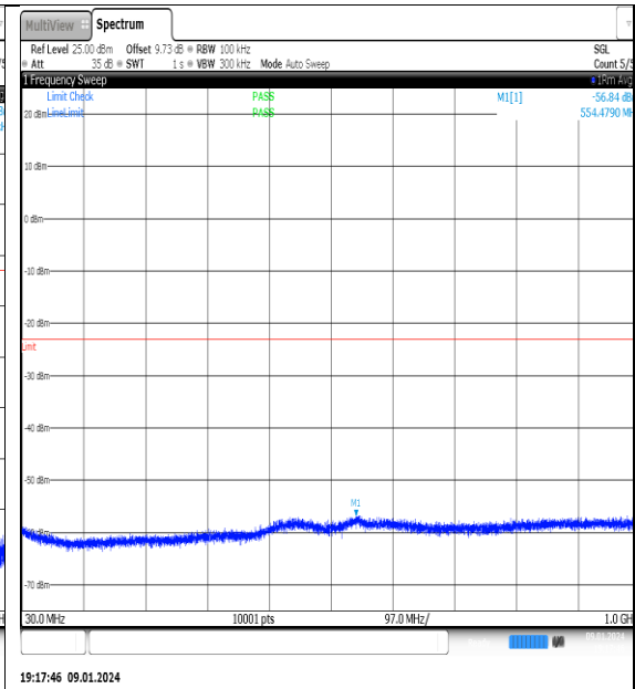
NTNV_N77-3700- 3980_PC2_30_80_L_TID15_NS_01_30_1000_#1
