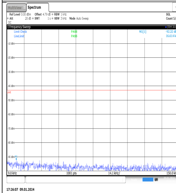
NTNV_N77-3700- 3980_PC2_30_70_H_TID13_NS_01_0.009_0.15_#1
