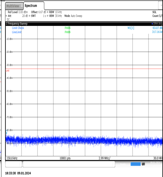
NTNV_N77-3700- 3980_PC2_30_80_L_TID10_NS_01_0.15_30_#1
