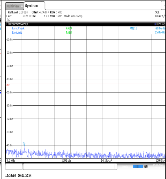
19:28:04 09.01.2024 NTNV_N77-3700- 3980_PC2_30_80_M_TID2_NS_01_0.009_0.15_# 1
