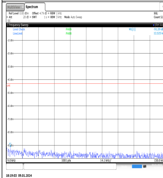
NTNV_N77-3700- 3980_PC2_30_80_L_TID6_NS_01_0.009_0.15_# 1
