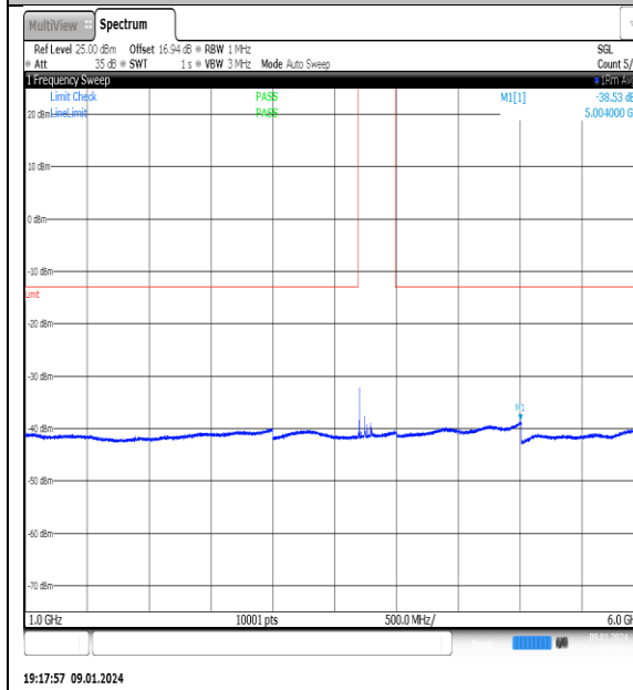
NTNV_N77-3700- 3980_PC2_30_80_L_TID15_NS_01_1000_6000_#1
