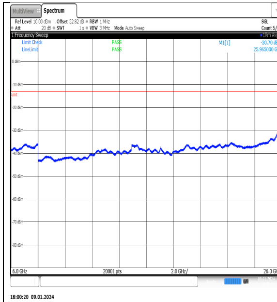
NTNV_N77-3700- 3980_PC2_30_80_L_TID3_NS_01_6000_26000_ #1
