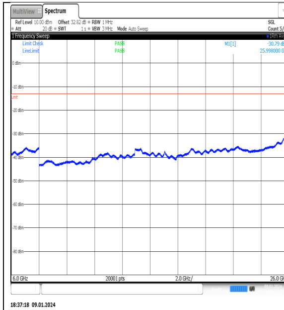
NTNV_N77-3700- 3980_PC2_30_80_L_TID11_NS_01_6000_26000 _#1
