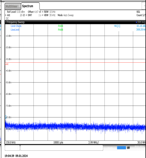
NTNV_N77-3700- 3980_PC2_30_80_L_TID14_NS_01_0.15_30_#1
