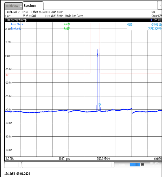
NTN_V_N77-3700- 3980_PC2_30_70_H_TID10_NS_01_1000_6000_ #1
