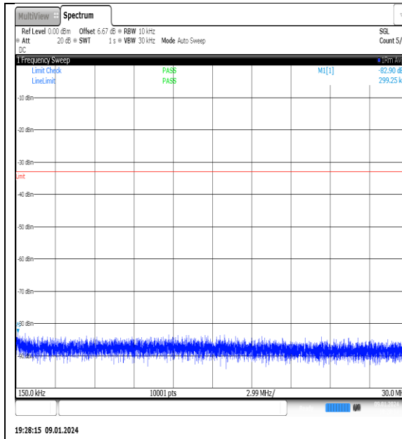
NTNV_N77-3700- 3980_PC2_30_80_M_TID2_NS_01_0.15_30_#1
