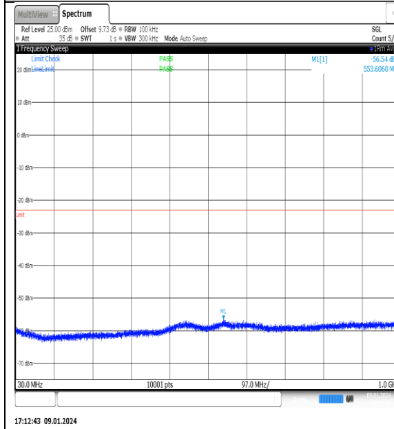
NTN_V_N77-3700- 3980_PC2_30_70_H_TID10_NS_01_30_1000_#1
