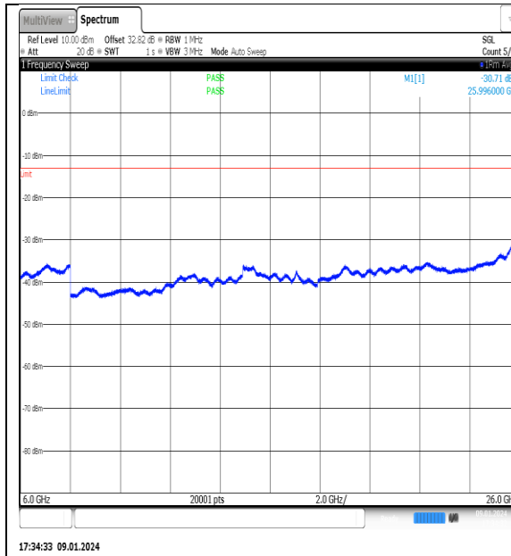
NTNV_N77-3700- 3980_PC2_30_70_H_TID14_NS_01_6000_26000 _#1
