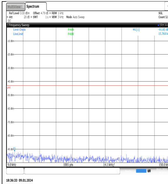
NTN_V_N77-3700- 3980_PC2_30_80_L_TID11_NS_01_0.009_0.15_ #1
