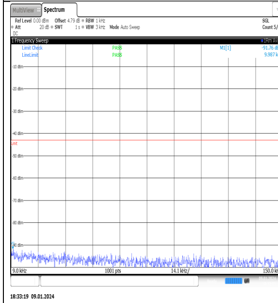
NTNV_N77-3700- 3980_PC2_30_80_L_TID10_NS_01_0.009_0.15_ #1
