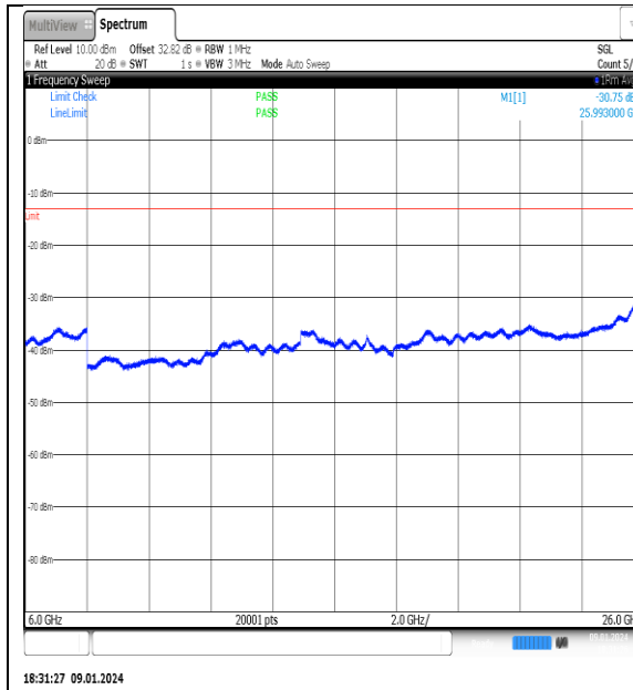
NTNV_N77-3700- 3980_PC2_30_80_L_TID9_NS_01_6000_26000_ #1
