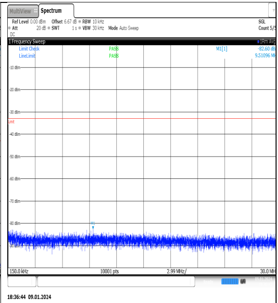
NTN_V_N77-3700- 3980_PC2_30_80_L_TID11_NS_01_0.15_30_#1
