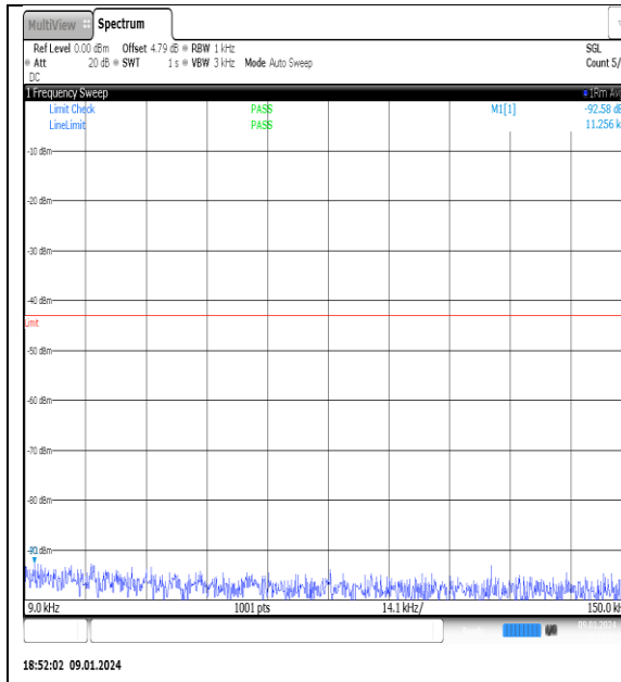
NTNV_N77-3700- 3980_PC2_30_80_L_TID13_NS_01_0.009_0.15_ #1
