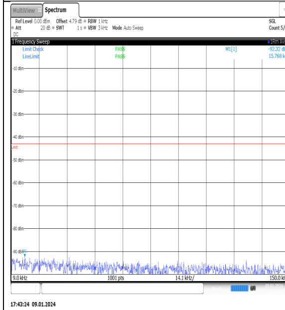
NTNV_N77-3700- 3980_PC2_30_70_H_TID15_NS_01_0.009_0.15_#1
