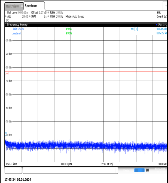
NTNV_N77-3700- 3980_PC2_30_70_H_TID15_NS_01_0.15_30_#1
