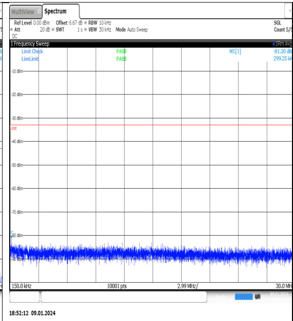
NTNV_N77-3700- 3980_PC2_30_80_L_TID13_NS_01_0.15_30_#1
