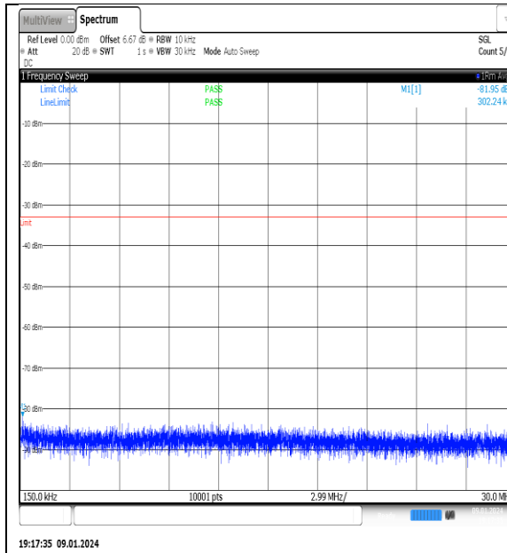
NTNV_N77-3700- 3980_PC2_30_80_L_TID15_NS_01_0.15_30_#1
