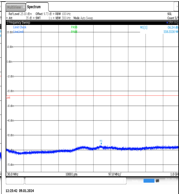
NTNV_N77-3700-3980_PC2_30_70_M_TID1_NS_01_30_1000_#1
