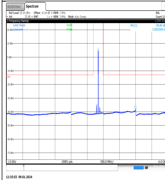
NTNV_N77-3700-3980_PC2_30_70_M_TID1_NS_01_1000_6000_#1
