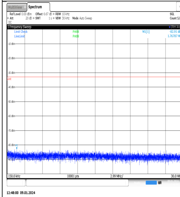
NTNV_N77-3700- 3980_PC2_30_70_M_TID4_NS_01_0.15_30_#1
