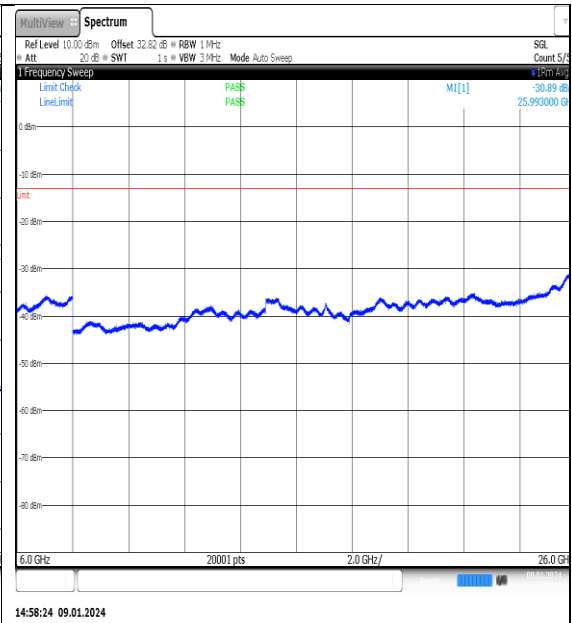
NTN_V_N77-3700- 3980_PC2_30_60_H_TID4_NS_01_6000_26000_# #1
