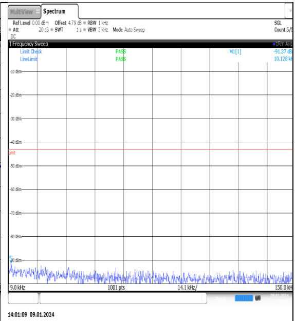
NTNV_N77-3700- 3980_PC2_30_70_M_TID12_NS_01_0.009_0.15_ #1
