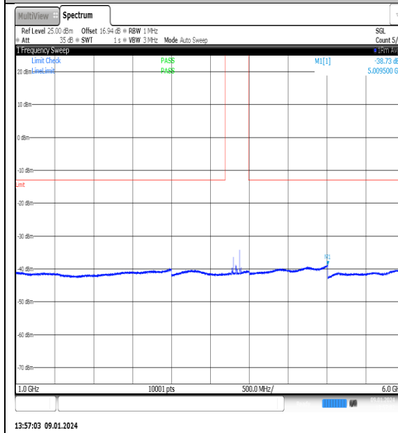
NTNV_N77-3700- 3980_PC2_30_70_M_TID11_NS_01_1000_6000_#1
