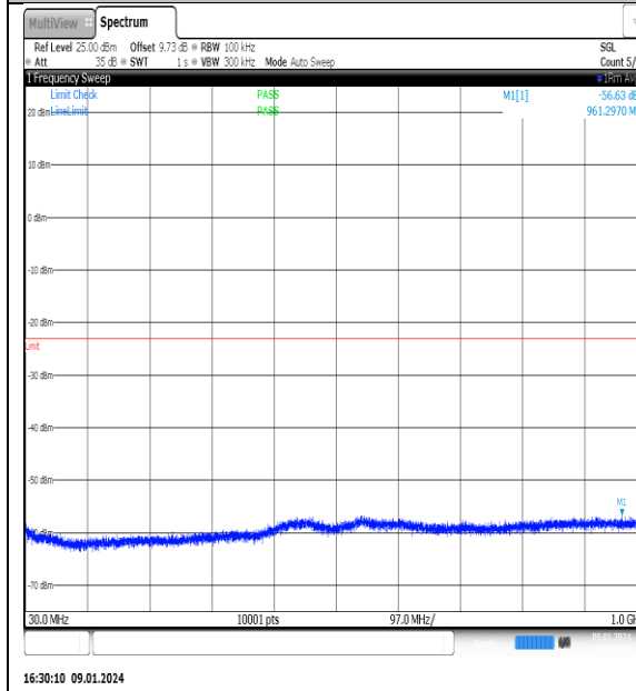
NTN_V_N77-3700- 3980_PC2_30_70_M_TID15_NS_01_30_1000_#1
