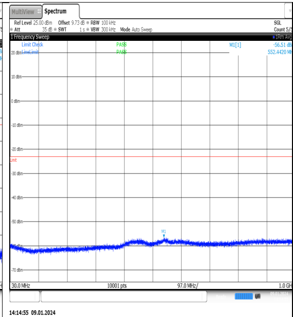
NTNV_N77-3700-3980_PC2_30_70_M_TID13_NS_01_30_1000_#1
