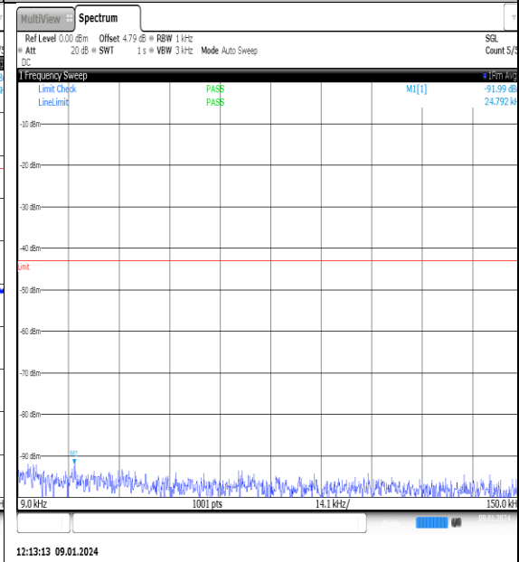
NTN_V_N77-3700- 3980_PC2_30_70_L_TID14_NS_01_0.009_0.15_ #1
