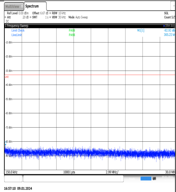
NTNV_N77-3700- 3980_PC2_30_70_H_TID5_NS_01_0.15_30_#1
