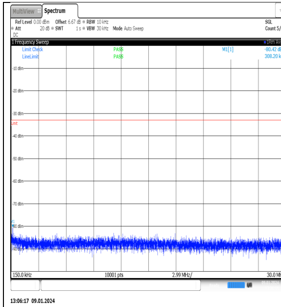
NTNV_N77-3700- 3980_PC2_30_70_M_TID7_NS_01_0.15_30_#1
