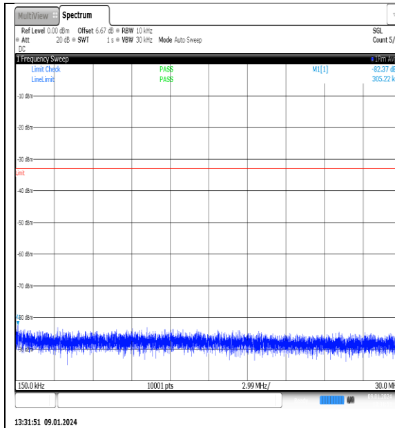
NTNV_N77-3700- 3980_PC2_30_70_M_TID9_NS_01_0.15_30_#1
