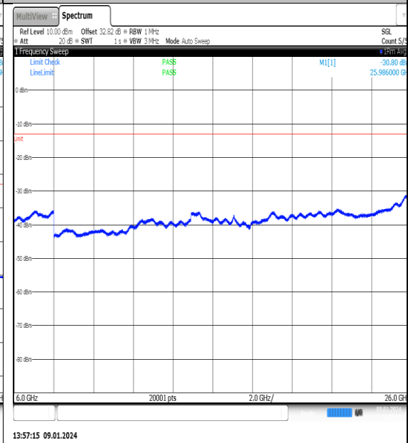
NTNV_N77-3700- 3980_PC2_30_70_M_TID11_NS_01_6000_26000_#1
