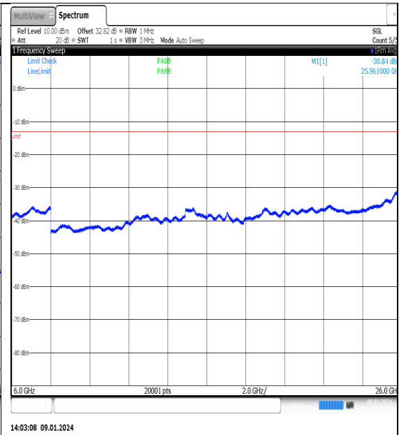
NTN_V_N77-3700- 3980_PC2_30_70_M_TID12_NS_01_6000_26000 #1
