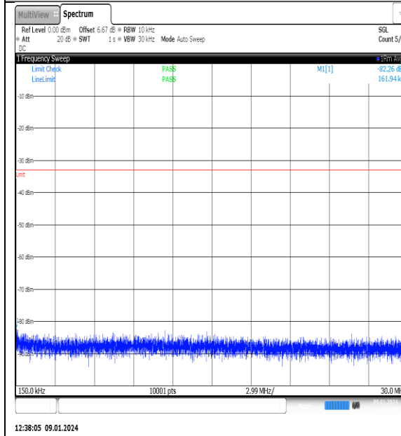
NTNV_N77-3700- 3980_PC2_30_70_M_TID2_NS_01_0.15_30_#1
