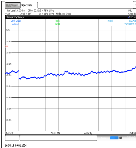
NTNV_N77-3700- 3980_PC2_30_70_H_TID4_NS_01_6000_26000_#1
