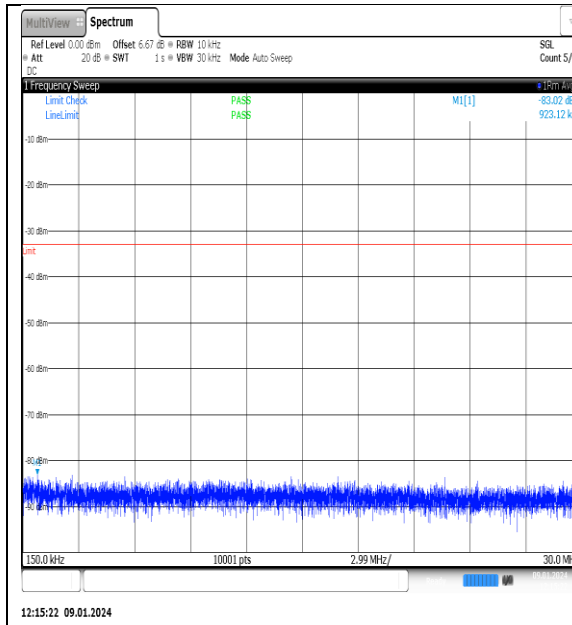
NTN_V_N77-3700- 3980_PC2_30_70_L_TID14_NS_01_0.15_30_#1
