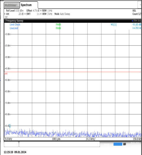
NTN_V_N77-3700- 3980_PC2_30_70_M_TID1_NS_01_0.009_0.15_# 1
