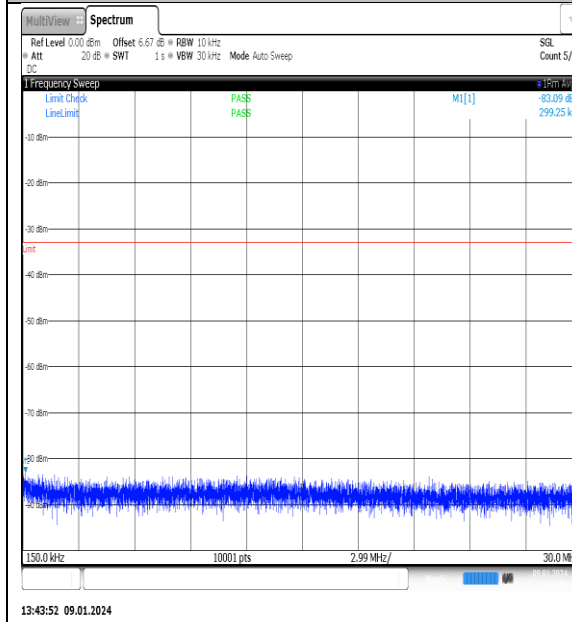
NTNV_N77-3700- 3980_PC2_30_70_M_TID10_NS_01_0.15_30_#1
