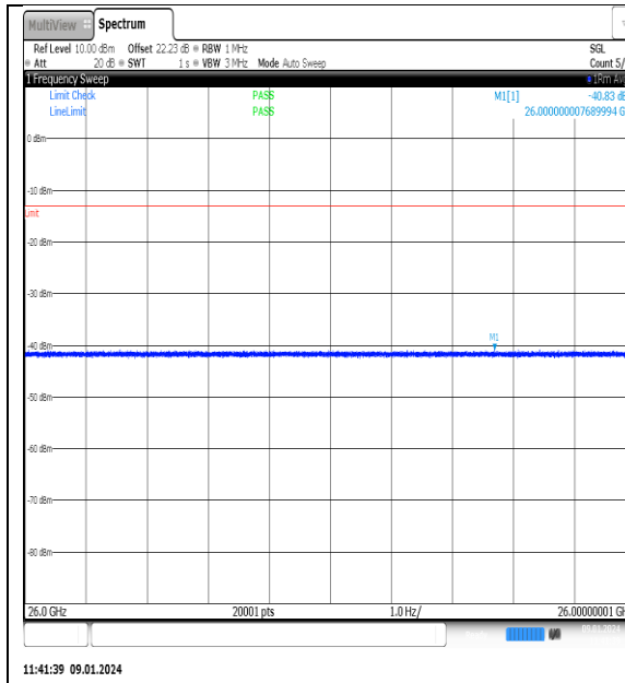
NTNV_N77-3700- 3980_PC2_30_70_L_TID8_NS_01_26000_40000 #1
