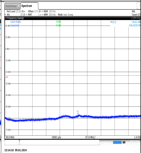
NTNV_N77-3700- 3980_PC2_30_70_M_TID8_NS_01_30_1000_#1
