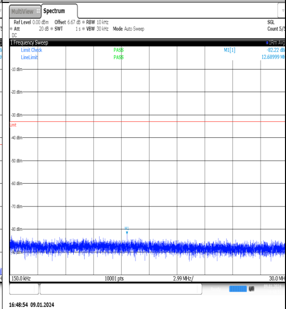
NTNV_N77-3700- 3980_PC2_30_70_H_TID3_NS_01_0.15_30_#1
