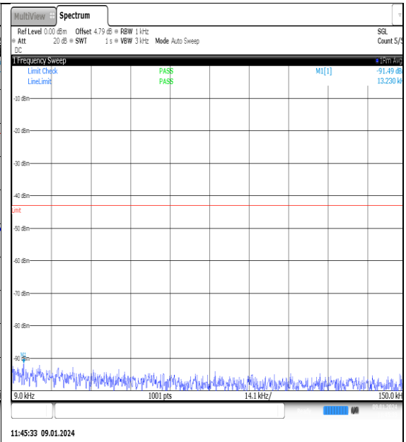
NTNV_N77-3700- 3980_PC2_30_70_L_TID9_NS_01_0.009_0.15_# 1
