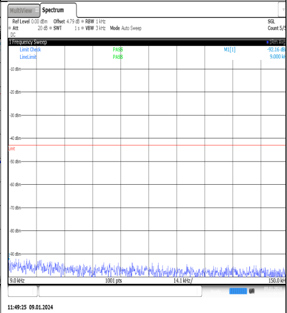
NTN V _N77-3700- 3980_PC2_30_70_L_TID10_NS_01_0.009_0.15_# #1
