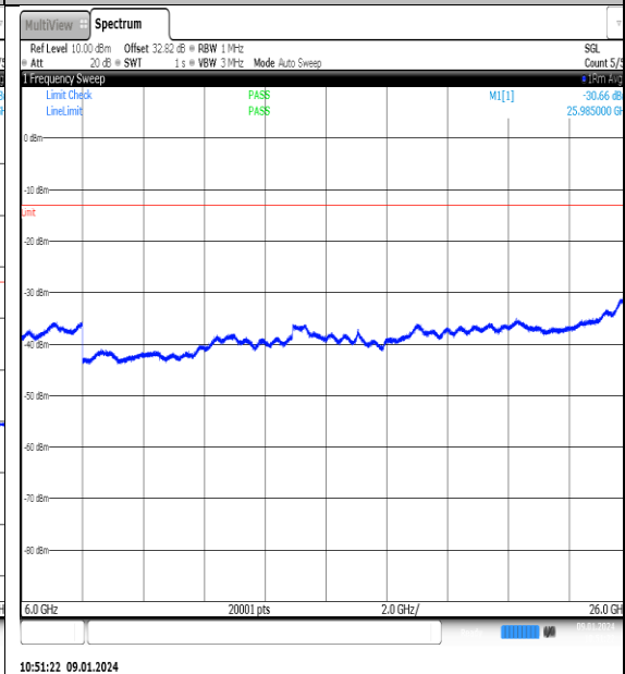
NTNV_N77-3700-3980_PC2_30_60_H_TID13_NS_01_6000_26000_#1
