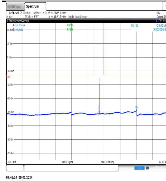
NTNV_N77-3700- 3980_PC2_30_60_M_TID15_NS_01_1000_6000_#1
