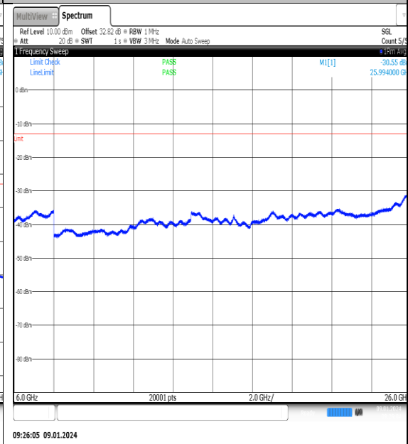
NTNV_N77-3700-3980_PC2_30_60_M_TID11_NS_01_6000_26000_#1
