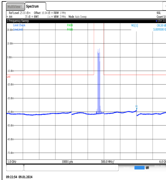
NTN_V_N77-3700- 3980_PC2_30_60_M_TID10_NS_01_1000_6000_ #1
