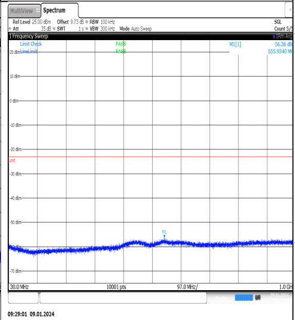
NTNV_N77-3700- 3980_PC2_30_60_M_TID12_NS_01_30_1000_#1
