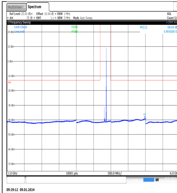
NTN_V_N77-3700- 3980_PC2_30_60_M_TID12_NS_01_1000_6000_ #1
