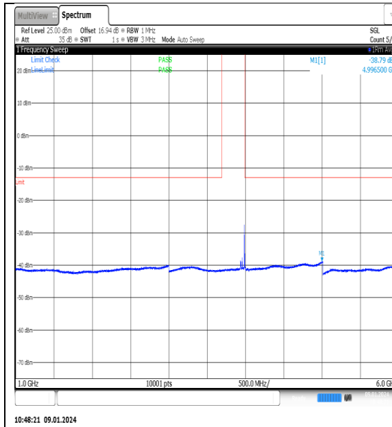
NTN_V_N77-3700- 3980_PC2_30_60_H_TID12_NS_01_1000_6000_ #1
