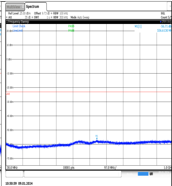
NTNV_N77-3700-3980_PC2_30_60_H_TID13_NS_01_30_1000_#1
