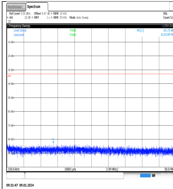
NTNV_N77-3700- 3980_PC2_30_60_M_TID13_NS_01_0.15_30_#1
