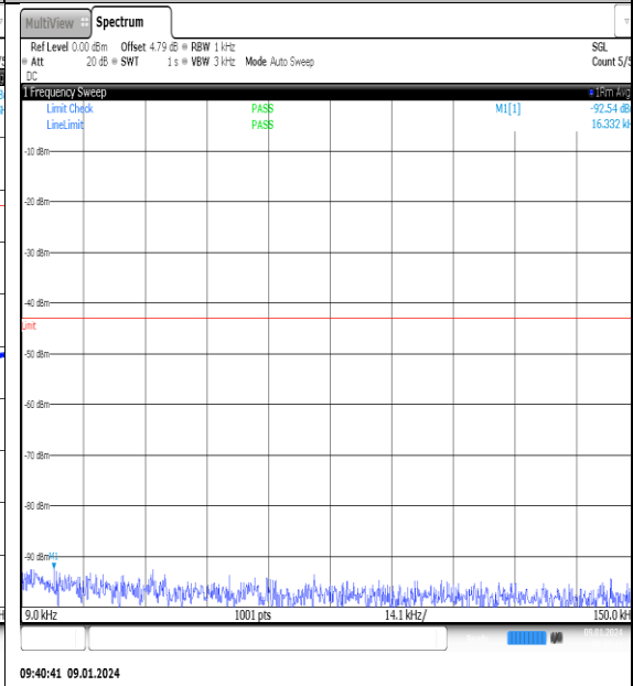
NTN_V_N77-3700- 3980_PC2_30_60_M_TID15_NS_01_0.009_0.15_ #1
