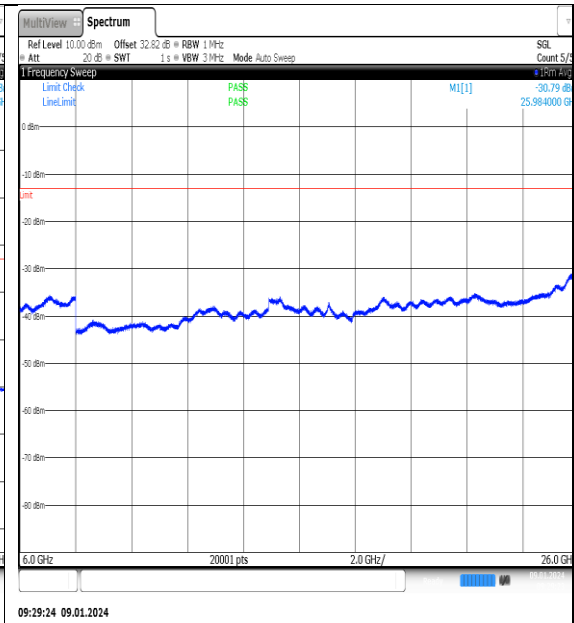
NTN_V_N77-3700- 3980_PC2_30_60_M_TID12_NS_01_6000_26000_ #1
