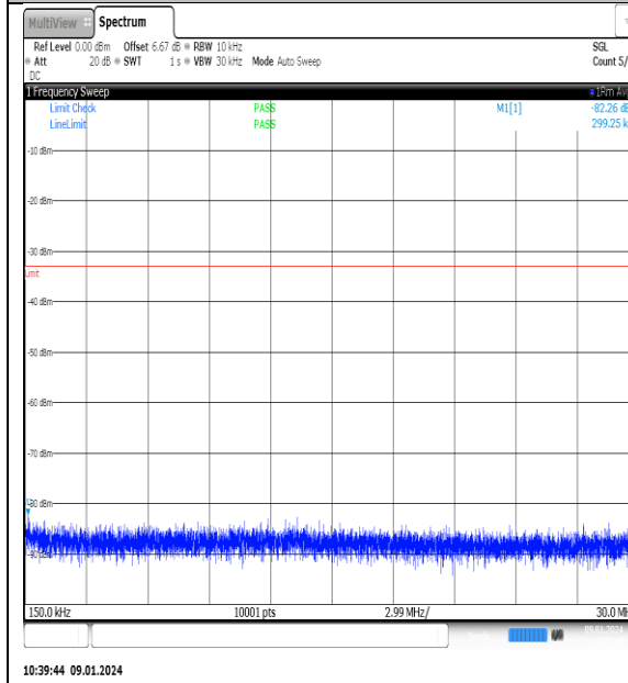
NTNV_N77-3700- 3980_PC2_30_60_H_TID10_NS_01_0.15_30_#1
