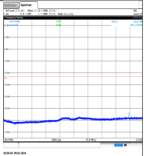
NTNV_N77-3700- 3980_PC2_30_60_H_TID14_NS_01_30_1000_#1
