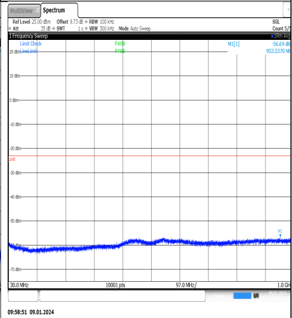
NTNV_N77-3700- 3980_PC2_30_60_H_TID3_NS_01_30_1000_#1
