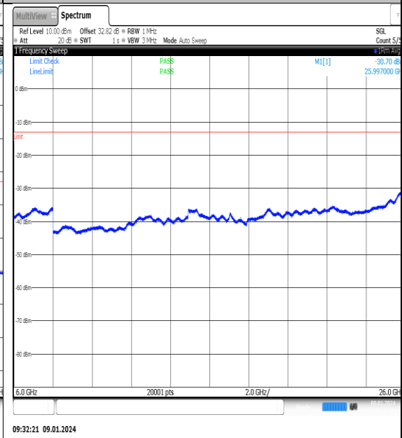
NTNV_N77-3700- 3980_PC2_30_60_M_TID13_NS_01_6000_26000_#1
