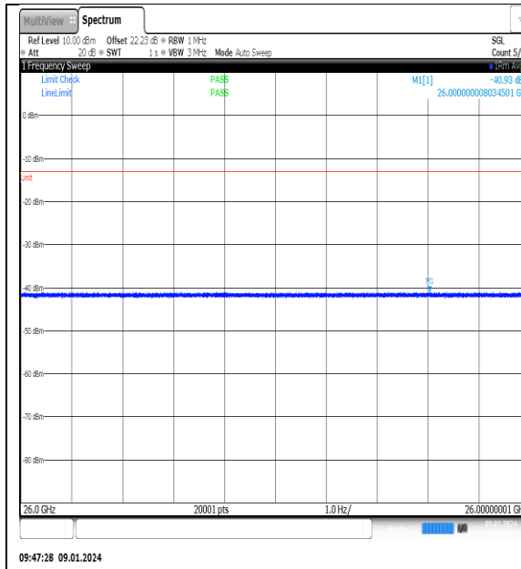
NTNV_N77-3700- 3980_PC2_30_60_H_TID2_NS_01_26000_40000 #1
