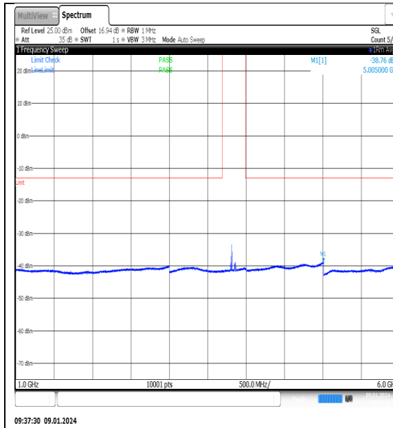
NTN_V_N77-3700- 3980_PC2_30_60_M_TID14_NS_01_1000_6000_ #1
