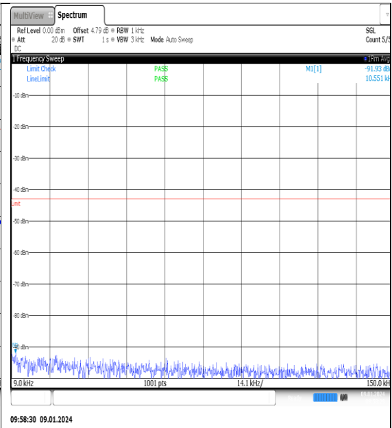
NTNV_N77-3700- 3980_PC2_30_60_H_TID3_NS_01_0.009_0.15_# 1
