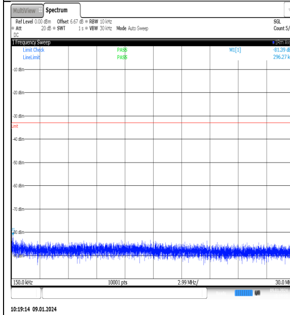
NTNV_N77-3700- 3980_PC2_30_60_H_TID6_NS_01_0.15_30_#1
