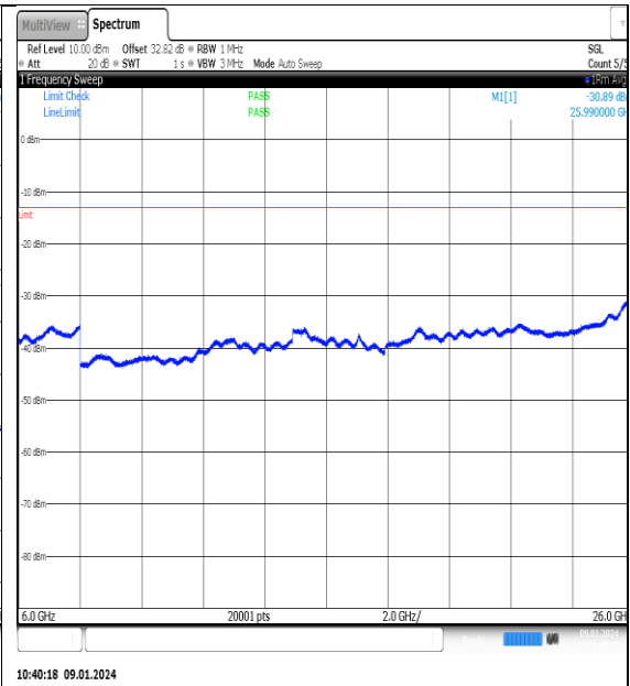
NTN_V_N77-3700- 3980_PC2_30_60_H_TID10_NS_01_6000_26000 #1
