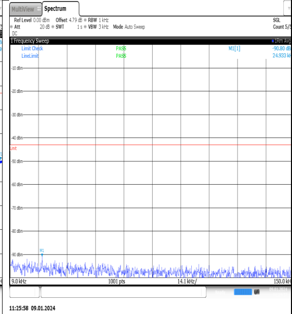
NTN_V_N77-3700- 3980_PC2_30_70_L_TID6_NS_01_0.009_0.15_# 1
