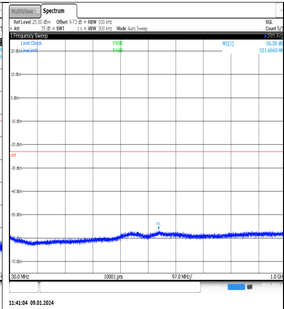
NTNV_N77-3700- 3980_PC2_30_70_L_TID8_NS_01_30_1000_#1
