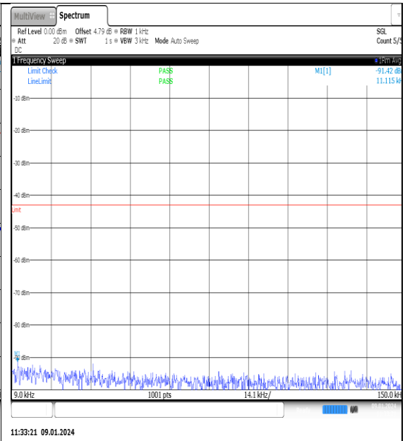
NTNV_N77-3700- 3980_PC2_30_70_L_TID7_NS_01_0.009_0.15_# 1
