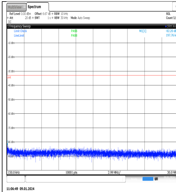
NTNV_N77-3700- 3980_PC2_30_70_L_TID2_NS_01_0.15_30_#1
