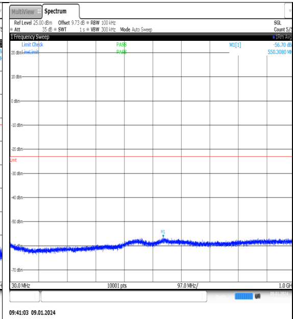
NTNV_N77-3700- 3980_PC2_30_60_M_TID15_NS_01_30_1000_#1
