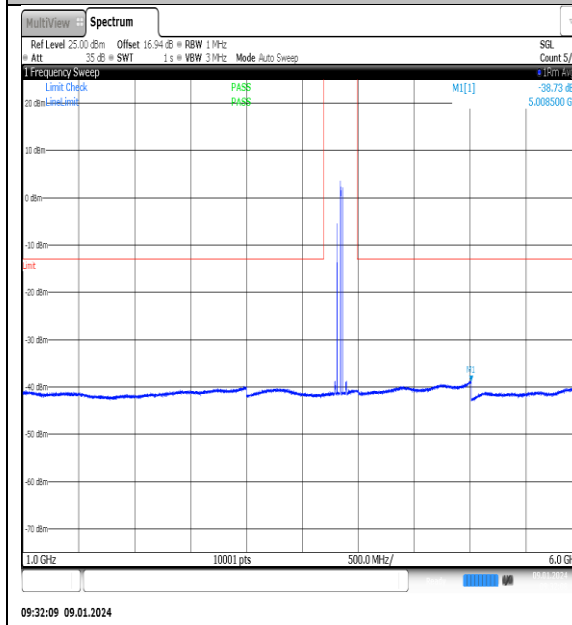
NTNV_N77-3700- 3980_PC2_30_60_M_TID13_NS_01_1000_6000_#1
