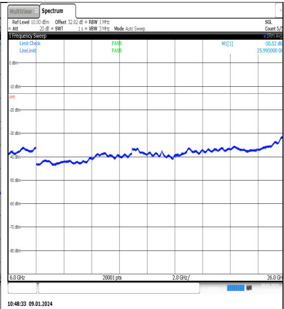
NTN_V_N77-3700- 3980_PC2_30_60_H_TID12_NS_01_6000_26000 #1
