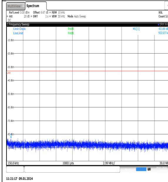
NTNV_N77-3700- 3980_PC2_30_70_L_TID5_NS_01_0.15_30_#1
