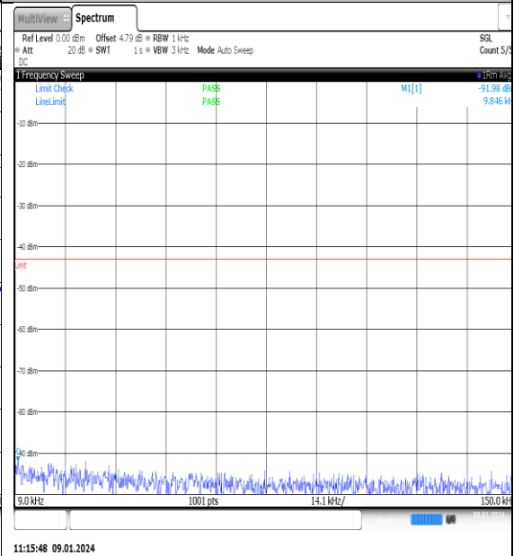
NTN_V_N77-3700- 3980_PC2_30_70_L_TID4_NS_01_0.009_0.15_# 1
