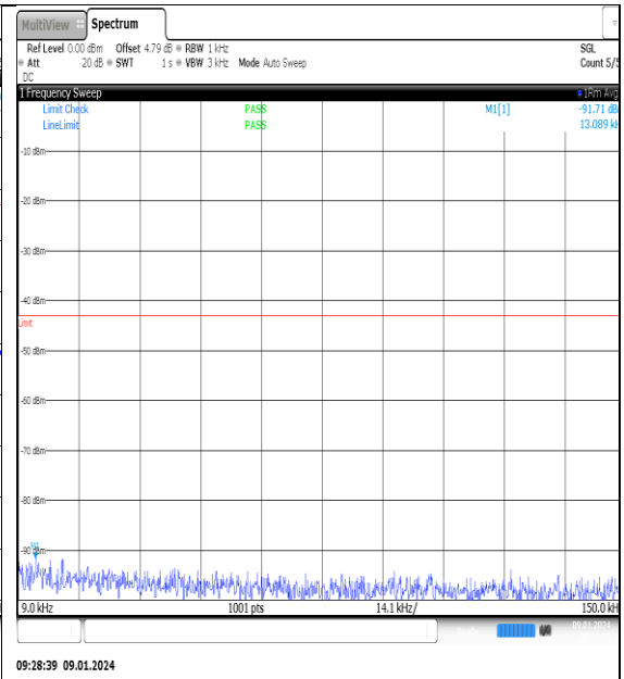
NTNV_N77-3700- 3980_PC2_30_60_M_TID12_NS_01_0.009_0.15_ #1
