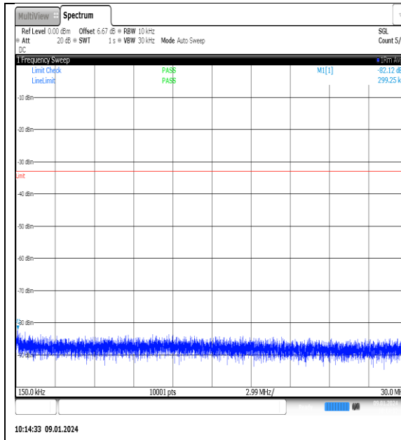
NTNV_N77-3700- 3980_PC2_30_60_H_TID5_NS_01_0.15_30_#1
