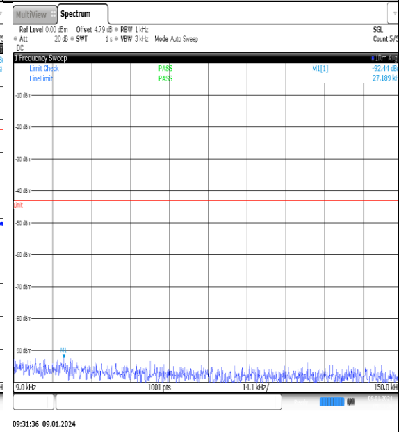
NTN_V_N77-3700- 3980_PC2_30_60_M_TID13_NS_01_0.009_0.15_ #1
