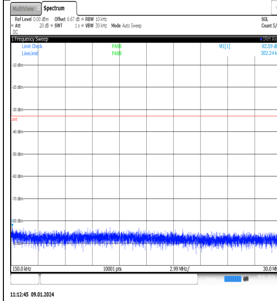
NTNV_N77-3700- 3980_PC2_30_70_L_TID3_NS_01_0.15_30_#1
