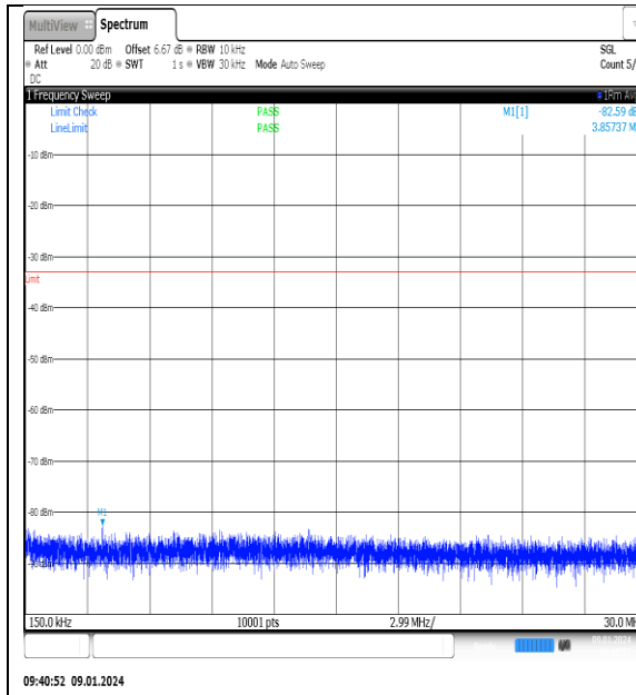
NTNV_N77-3700- 3980_PC2_30_60_M_TID15_NS_01_0.15_30_#1
