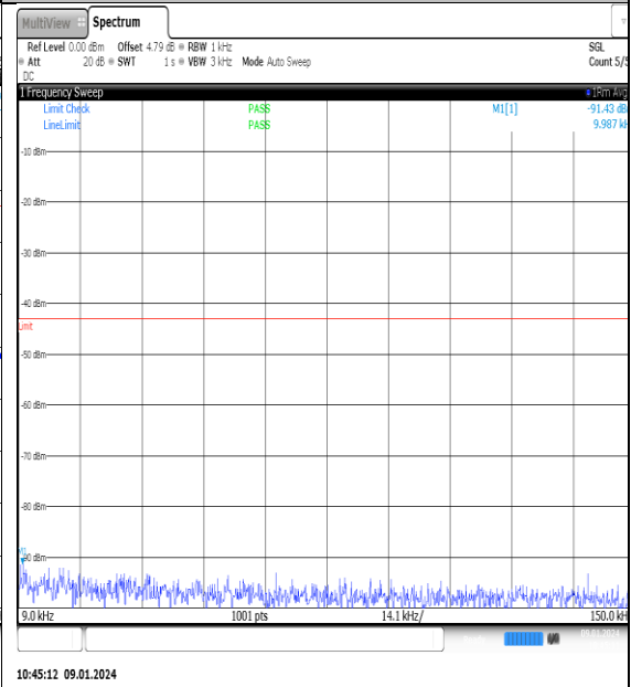
NTN_V_N77-3700- 3980_PC2_30_60_H_TID11_NS_01_0.009_0.15_ #1
