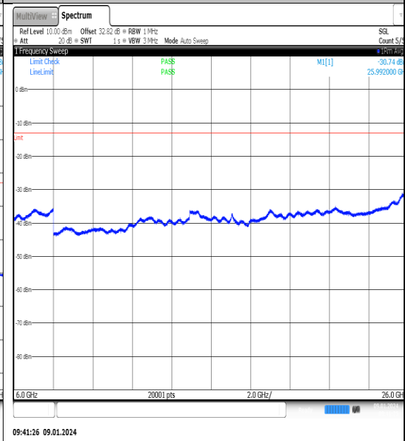
NTNV_N77-3700- 3980_PC2_30_60_M_TID15_NS_01_6000_26000_#1
