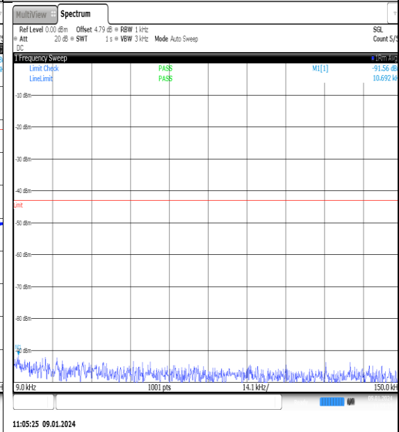
NTN_V_N77-3700- 3980_PC2_30_70_L_TID2_NS_01_0.009_0.15_# 1
