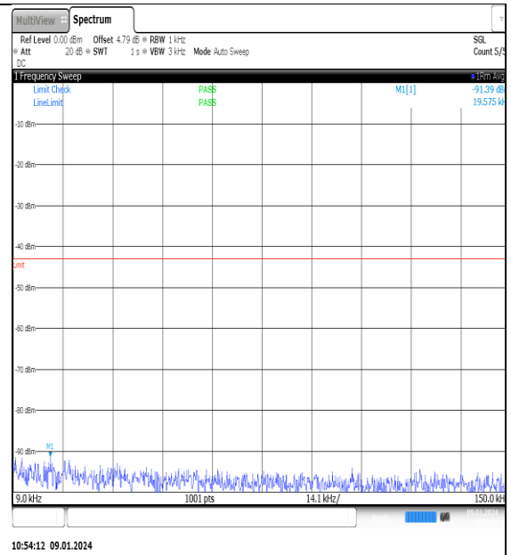
NTNV_N77-3700- 3980_PC2_30_60_H_TID14_NS_01_0.009_0.15_ #1
