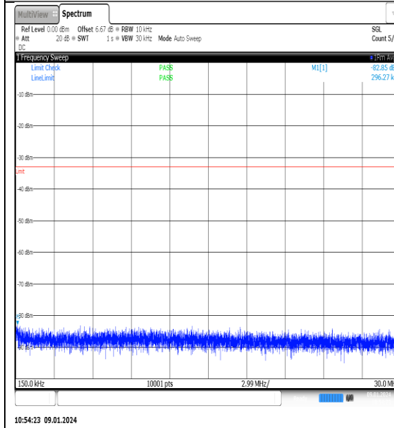
NTNV_N77-3700- 3980_PC2_30_60_H_TID14_NS_01_0.15_30_#1
