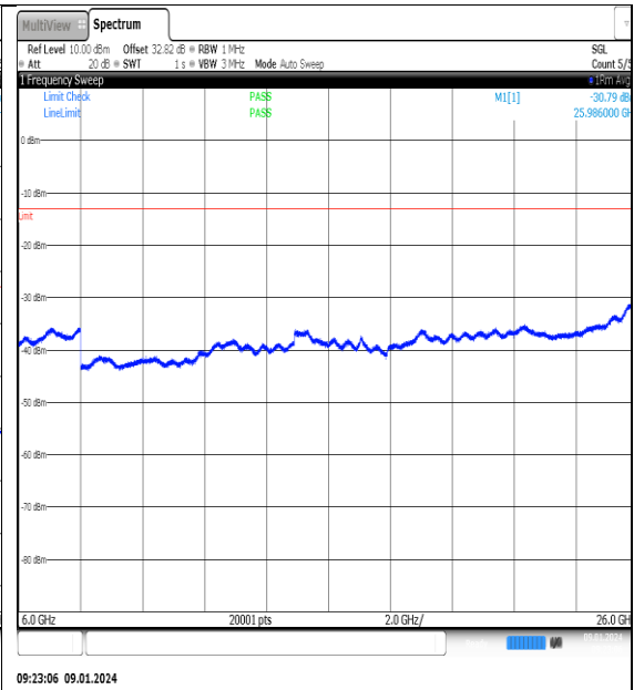
NTN_V_N77-3700- 3980_PC2_30_60_M_TID10_NS_01_6000_26000 #1
