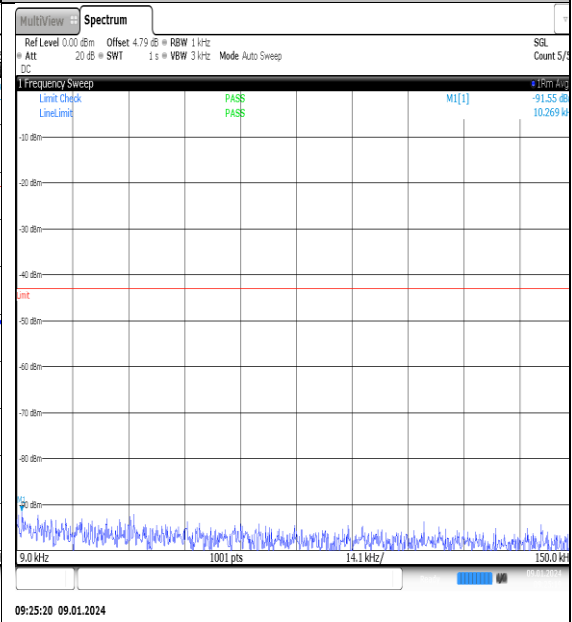
NTN_V_N77-3700- 3980_PC2_30_60_M_TID11_NS_01_0.009_0.15_ #1
