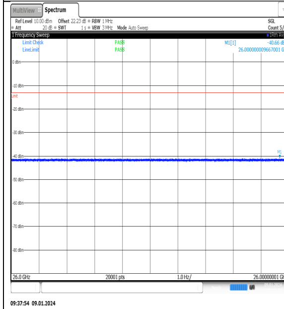
NTN_V_N77-3700- 3980_PC2_30_60_M_TID14_NS_01_26000_4000_ 0_#1
