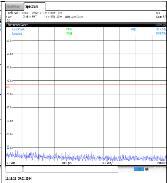
NTNV_N77-3700- 3980_PC2_30_70_L_TID3_NS_01_0.009_0.15_# 1
