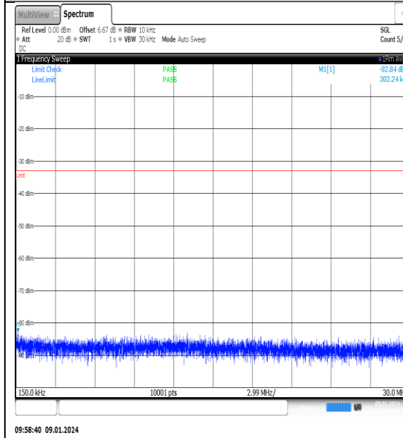
NTNV_N77-3700- 3980_PC2_30_60_H_TID3_NS_01_0.15_30_#1
