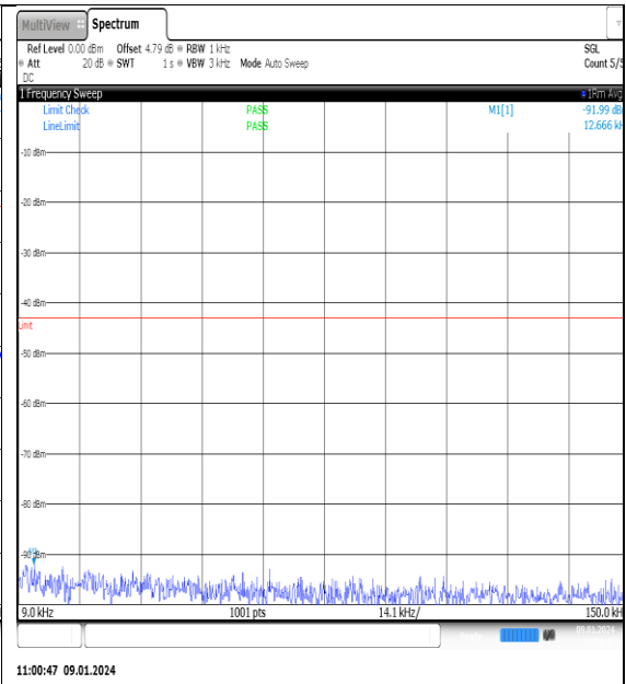
NTNV_N77-3700- 3980_PC2_30_70_L_TID1_NS_01_0.009_0.15_# 1
