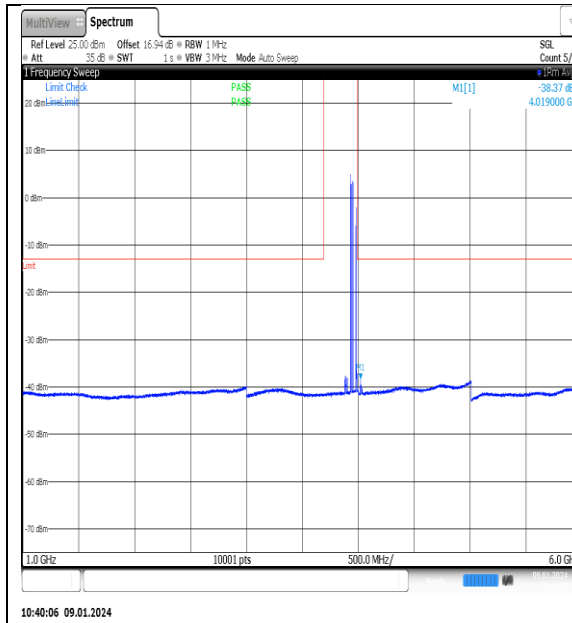
NTN_V_N77-3700- 3980_PC2_30_60_H_TID10_NS_01_1000_6000_ #1
