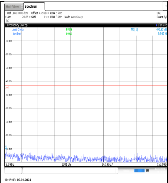
NTNV_N77-3700- 3980_PC2_30_60_H_TID6_NS_01_0.009_0.15_# 1
