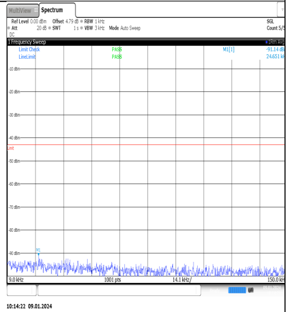
10:14:22 09.01.2024 NTN_V_N77-3700- 3980_PC2_30_60_H_TID5_NS_01_0.009_0.15_# 1
