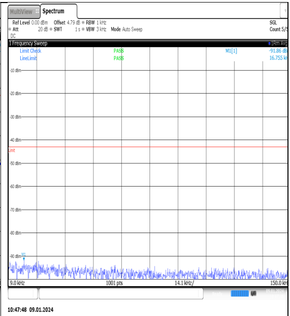
NTNV_N77-3700- 3980_PC2_30_60_H_TID12_NS_01_0.009_0.15_#1
