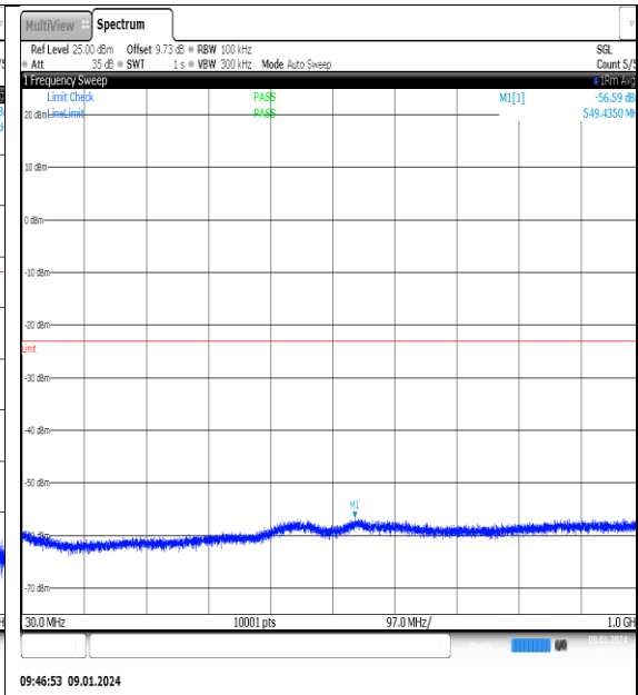
09:46:53 09.01.2024 NTNV_N77-3700- 3980_PC2_30_60_H_TID2_NS_01_30_1000_#1
