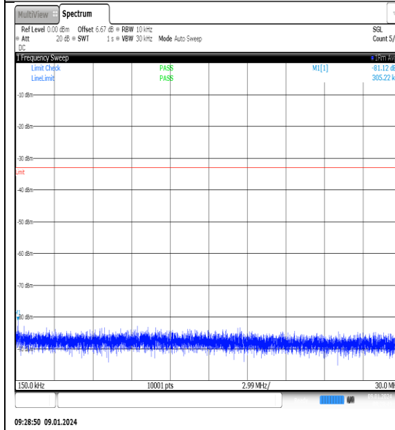
NTNV_N77-3700- 3980_PC2_30_60_M_TID12_NS_01_0.15_30_#1
