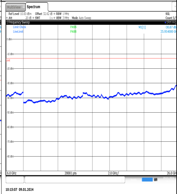
NTNV_N77-3700- 3980_PC2_30_60_H_TID5_NS_01_6000_26000_#1
