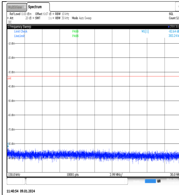
NTNV_N77-3700- 3980_PC2_30_70_L_TID8_NS_01_0.15_30_#1
