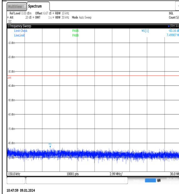
NTNV_N77-3700- 3980_PC2_30_60_H_TID12_NS_01_0.15_30_#1
