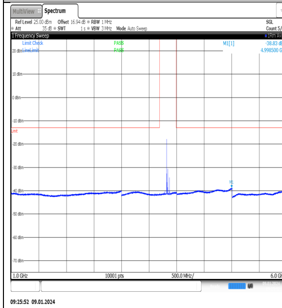
NTNV_N77-3700-3980_PC2_30_60_M_TID11_NS_01_1000_6000_#1
