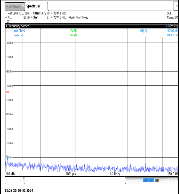
NTNV_N77-3700- 3980_PC2_30_60_H_TID7_NS_01_0.009_0.15_# 1
