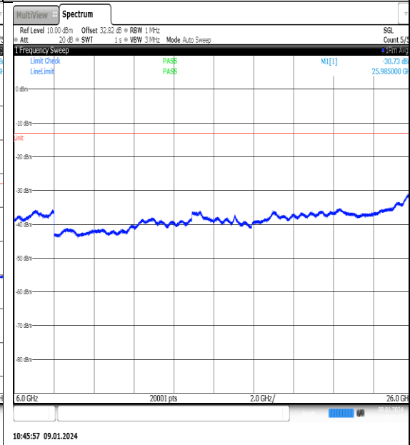
NTNV_N77-3700-3980_PC2_30_60_H_TID11_NS_01_6000_26000_#1
