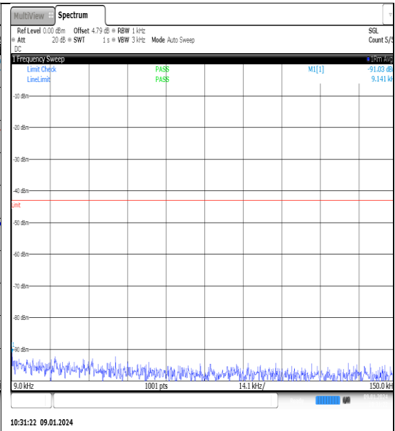
NTNV_N77-3700- 3980_PC2_30_60_H_TID8_NS_01_0.009_0.15_# 1
