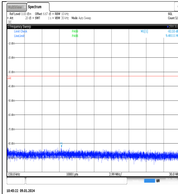
NTNV_N77-3700-3980_PC2_30_60_H_TID11_NS_01_0.15_30_#1
