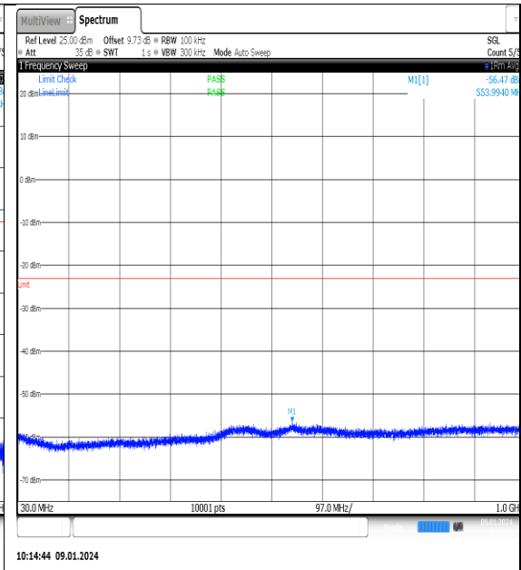
NTNV_N77-3700- 3980_PC2_30_60_H_TID5_NS_01_30_1000_#1
