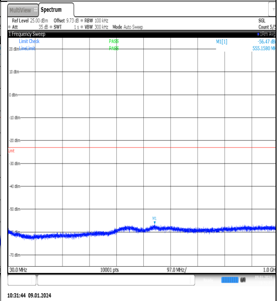
NTNV_N77-3700- 3980_PC2_30_60_H_TID8_NS_01_30_1000_#1
