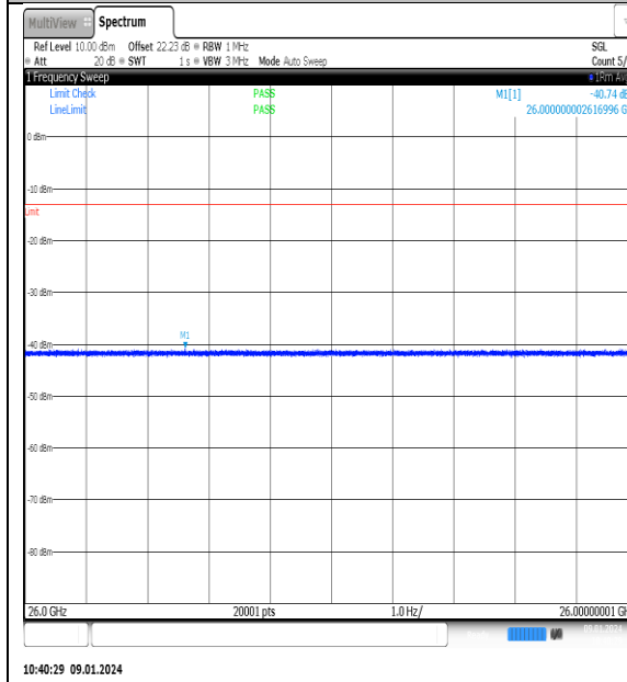
NTN_V_N77-3700- 3980_PC2_30_60_H_TID10_NS_01_26000_4000 0_#1
