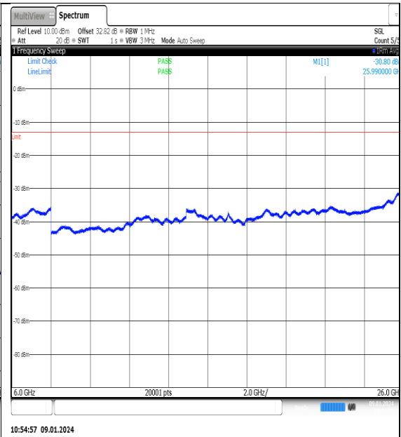
NTN_V_N77-3700- 3980_PC2_30_60_H_TID14_NS_01_6000_26000_ #1
