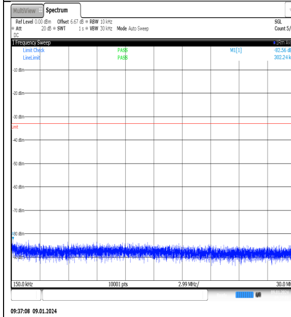
NTNV_N77-3700- 3980_PC2_30_60_M_TID14_NS_01_0.15_30_#1
