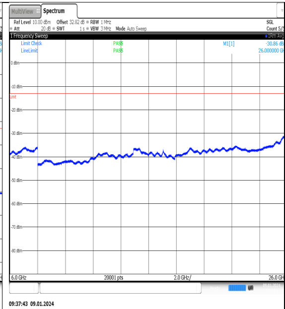
NTN_V_N77-3700- 3980_PC2_30_60_M_TID14_NS_01_6000_26000_ #1
