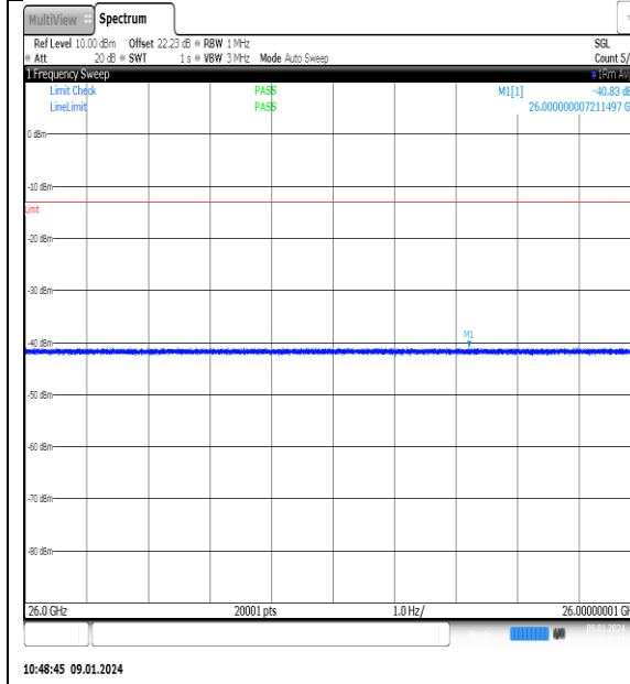
NTN_V_N77-3700- 3980_PC2_30_60_H_TID12_NS_01_26000_4000 0_#1
