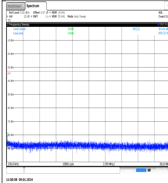
NTNV_N77-3700- 3980_PC2_30_70_L_TID1_NS_01_0.15_30_#1
