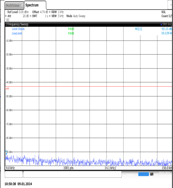
NTN_V_N77-3700- 3980_PC2_30_60_H_TID13_NS_01_0.009_0.15_ #1
