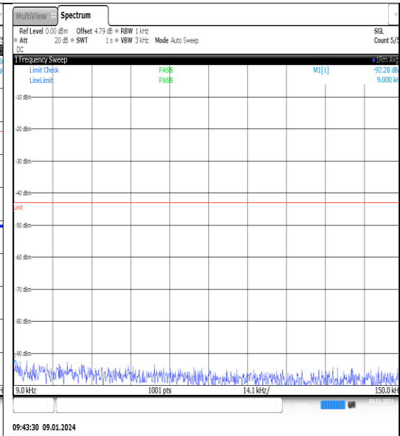
NTNV_N77-3700- 3980_PC2_30_60_H_TID1_NS_01_0.009_0.15_# 1
