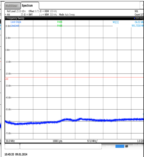
NTNV_N77-3700-3980_PC2_30_60_H_TID11_NS_01_30_1000_#1
