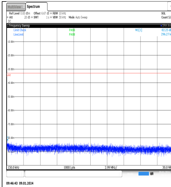
09:46:43 09.01.2024 NTNV_N77-3700- 3980_PC2_30_60_H_TID2_NS_01_0.15_30_#1
