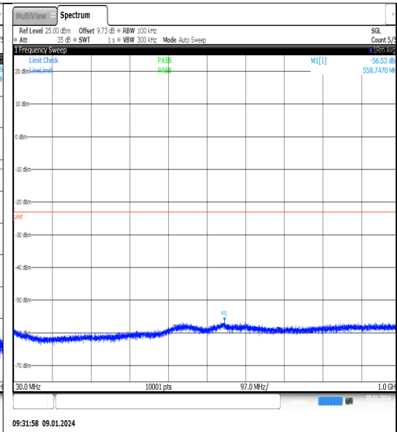
NTNV_N77-3700- 3980_PC2_30_60_M_TID13_NS_01_30_1000_#1
