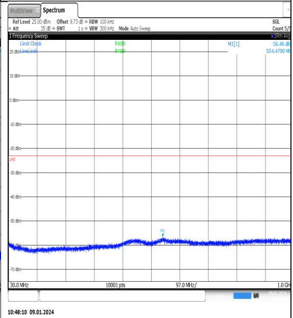
NTNV_N77-3700- 3980_PC2_30_60_H_TID12_NS_01_30_1000_#1
