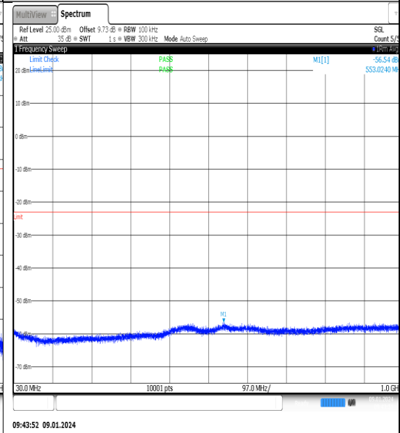
NTNV_N77-3700- 3980_PC2_30_60_H_TID1_NS_01_30_1000_#1
