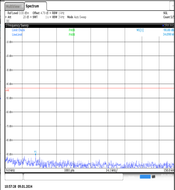
NTN_V_N77-3700- 3980_PC2_30_60_H_TID15_NS_01_0.009_0.15_ #1
