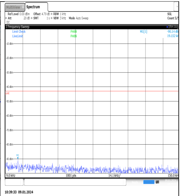
NTNV_N77-3700- 3980_PC2_30_60_H_TID10_NS_01_0.009_0.15_ #1
