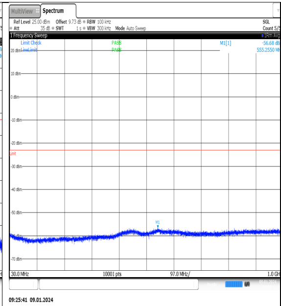
NTNV_N77-3700-3980_PC2_30_60_M_TID11_NS_01_30_1000_#1
