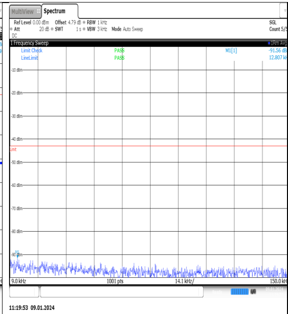
NTNV_N77-3700- 3980_PC2_30_70_L_TID5_NS_01_0.009_0.15_# 1
