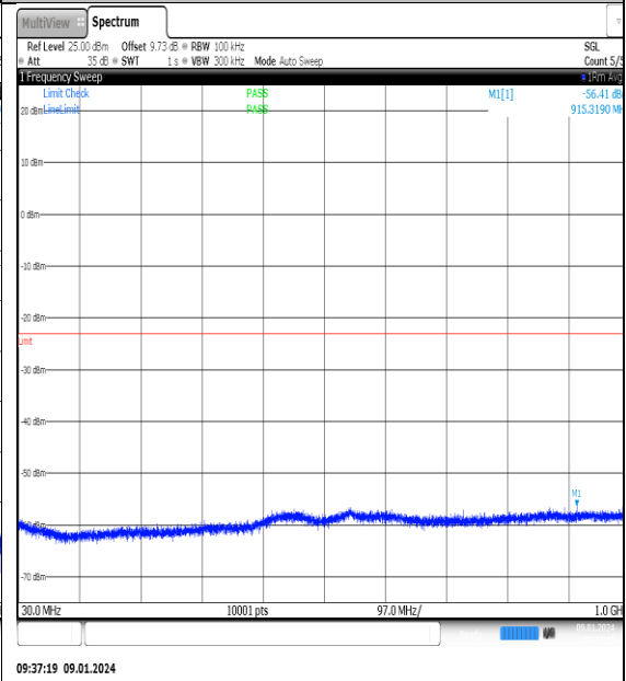
NTNV_N77-3700- 3980_PC2_30_60_M_TID14_NS_01_30_1000_#1
