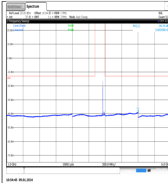
NTN_V_N77-3700- 3980_PC2_30_60_H_TID14_NS_01_1000_6000_ #1
