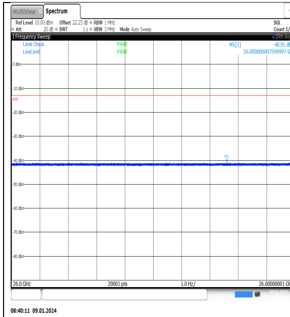
NTNV_N77-3700- 3980_PC2_30_60_L_TID14_NS_01_26000_4000 0_#1
