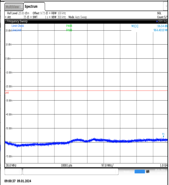
NTNV_N77-3700- 3980_PC2_30_60_M_TID4_NS_01_30_1000_#1
