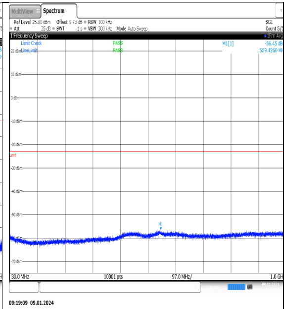
NTNV_N77-3700- 3980_PC2_30_60_M_TID9_NS_01_30_1000_#1
