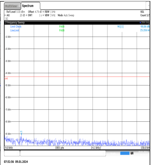
NTNV_N77-3700- 3980_PC2_30_60_L_TID1_NS_01_0.009_0.15_# 1
