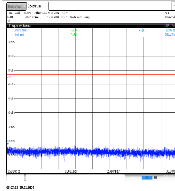
NTNV_N77-3700- 3980_PC2_30_60_L_TID3_NS_01_0.15_30_#1
