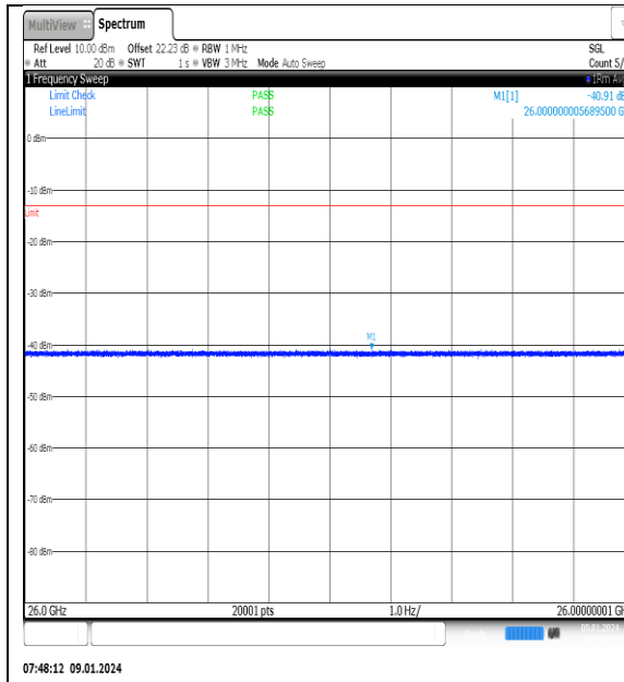
NTNV_N77-3700- 3980_PC2_30_50_H_TID15_NS_01_26000_4000 0_#1
