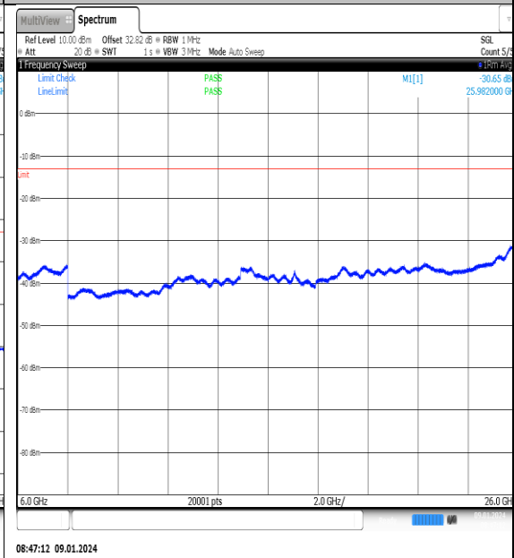
08:47:12 09.01.2024 NTN_V_N77-3700- 3980_PC2_30_60_M_TID1_NS_01_6000_26000_#1
