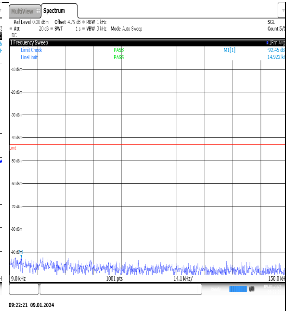
NTNV_N77-3700- 3980_PC2_30_60_M_TID10_NS_01_0.009_0.15_ #1
