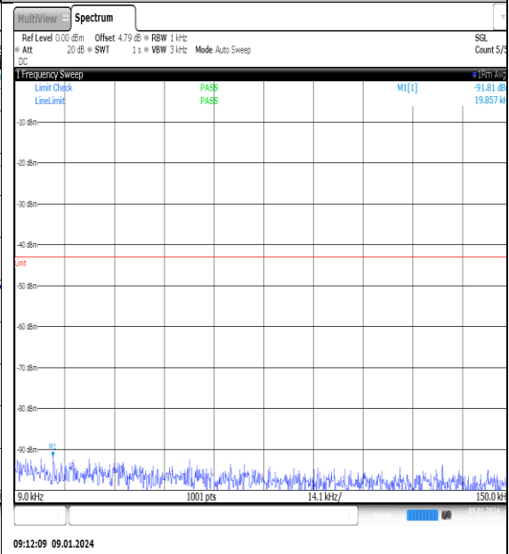
NTN_V_N77-3700- 3980_PC2_30_60_M_TID7_NS_01_0.009_0.15_# 1
