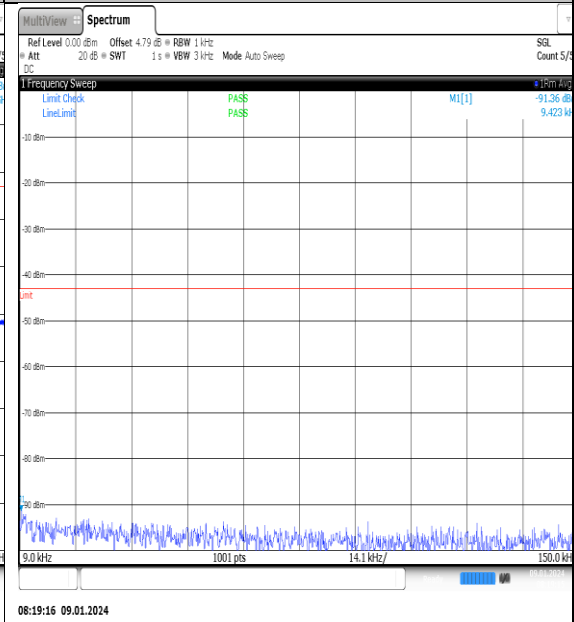
NTN_V_N77-3700- 3980_PC2_30_60_L_TID8_NS_01_0.009_0.15_# 1
