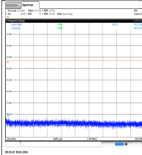
NTNV_N77-3700- 3980_PC2_30_60_M_TID8_NS_01_0.15_30_#1
