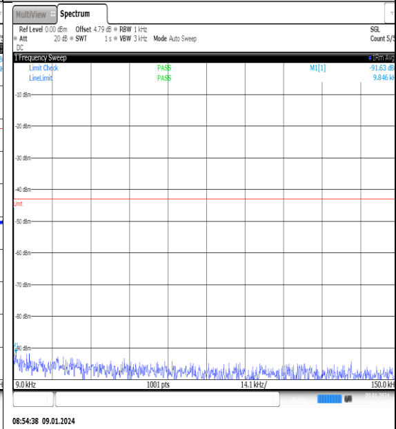
NTN_V_N77-3700- 3980_PC2_30_60_M_TID3_NS_01_0.009_0.15_# 1
