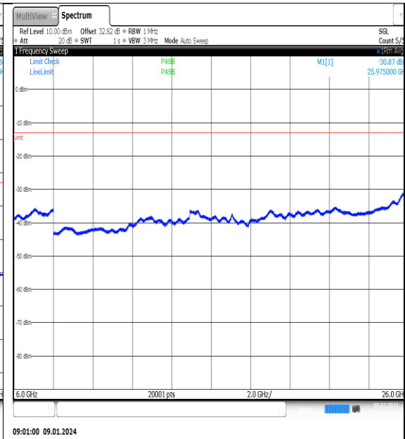
NTN_V_N77-3700- 3980_PC2_30_60_M_TID4_NS_01_6000_26000_# #1
