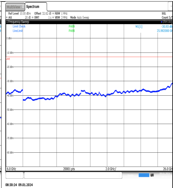
NTN_V_N77-3700- 3980_PC2_30_60_L_TID11_NS_01_6000_26000 #1
