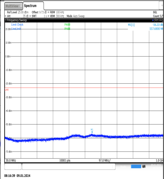
NTNV_N77-3700- 3980_PC2_30_60_L_TID7_NS_01_30_1000_#1
