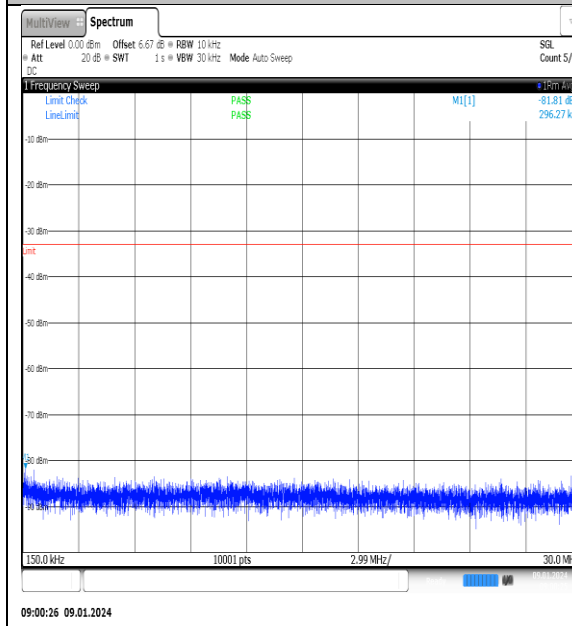
NTNV_N77-3700- 3980_PC2_30_60_M_TID4_NS_01_0.15_30_#1
