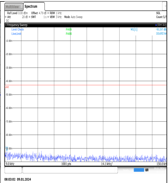
NTNV_N77-3700- 3980_PC2_30_60_L_TID3_NS_01_0.009_0.15_# 1
