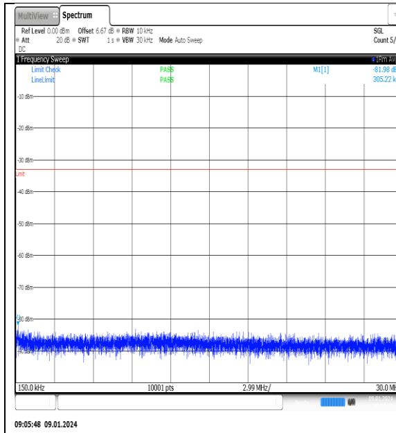
NTNV_N77-3700- 3980_PC2_30_60_M_TID5_NS_01_0.15_30_#1
