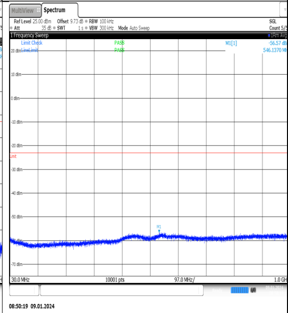
NTNV_N77-3700- 3980_PC2_30_60_M_TID2_NS_01_30_1000_#1
