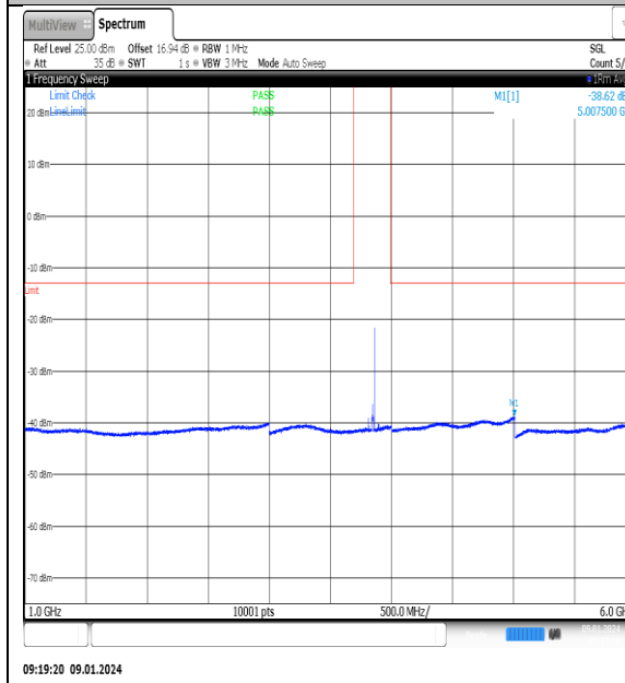
NTNV_N77-3700- 3980_PC2_30_60_M_TID9_NS_01_1000_6000_#1
