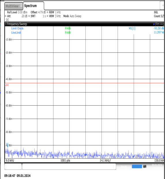
NTNV_N77-3700- 3980_PC2_30_60_M_TID9_NS_01_0.009_0.15_# 1
