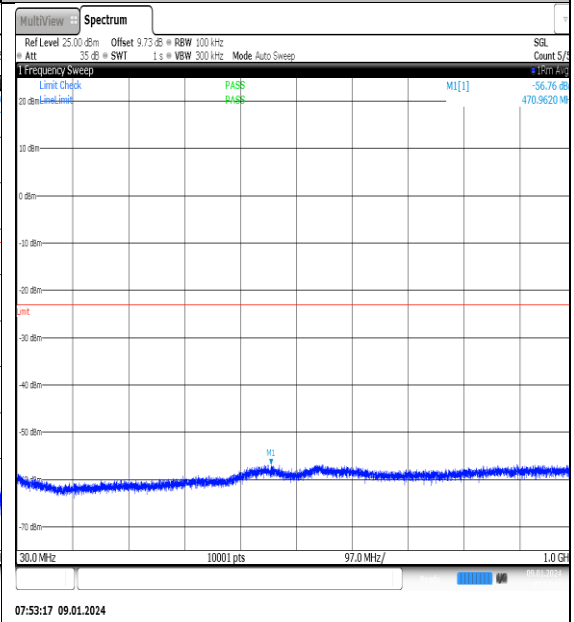
NTNV_N77-3700- 3980_PC2_30_60_L_TID1_NS_01_30_1000_#1
