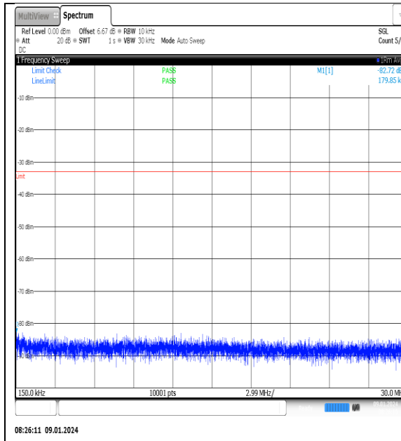
NTNV_N77-3700-3980_PC2_30_60_L_TID10_NS_01_0.15_30_#1
