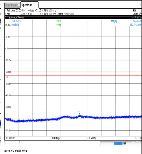
NTNV_N77-3700- 3980_PC2_30_60_L_TID13_NS_01_30_1000_#1
