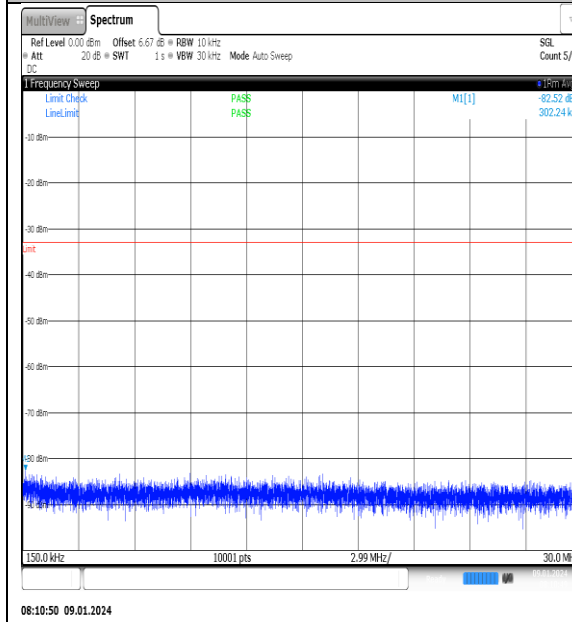
NTNV_N77-3700- 3980_PC2_30_60_L_TID5_NS_01_0.15_30_#1
