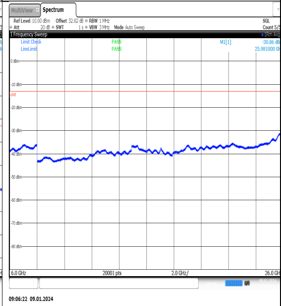
NTNV_N77-3700- 3980_PC2_30_60_M_TID5_NS_01_6000_26000_#1
