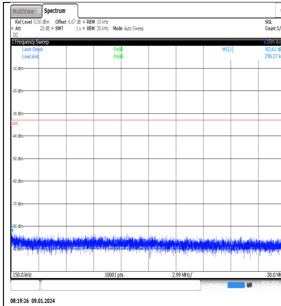
NTNV_N77-3700- 3980_PC2_30_60_L_TID8_NS_01_0.15_30_#1
