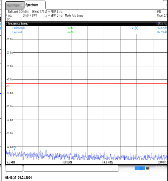
NTNV_N77-3700- 3980_PC2_30_60_M_TID1_NS_01_0.009_0.15_# 1
