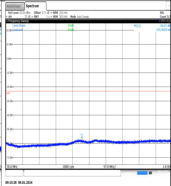
NTNV_N77-3700- 3980_PC2_30_60_M_TID8_NS_01_30_1000_#1
