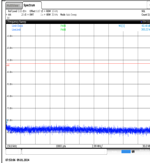
NTNV_N77-3700- 3980_PC2_30_60_L_TID1_NS_01_0.15_30_#1
