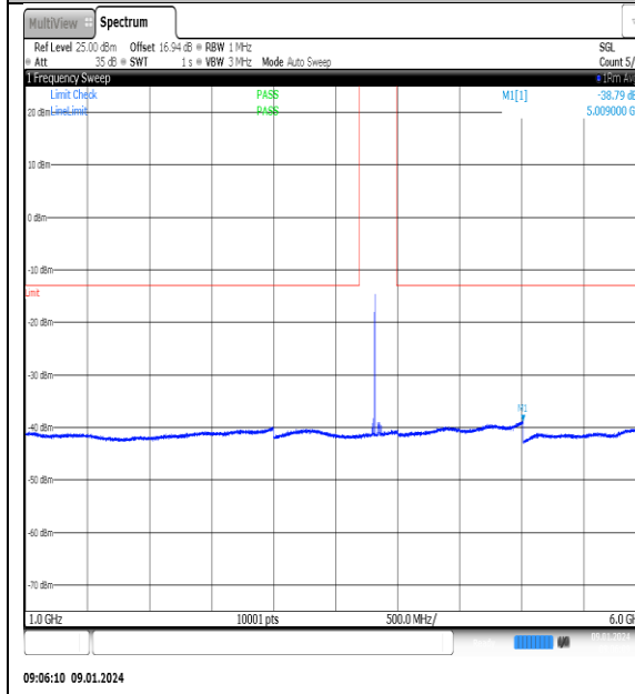
NTNV_N77-3700- 3980_PC2_30_60_M_TID5_NS_01_1000_6000_#1
