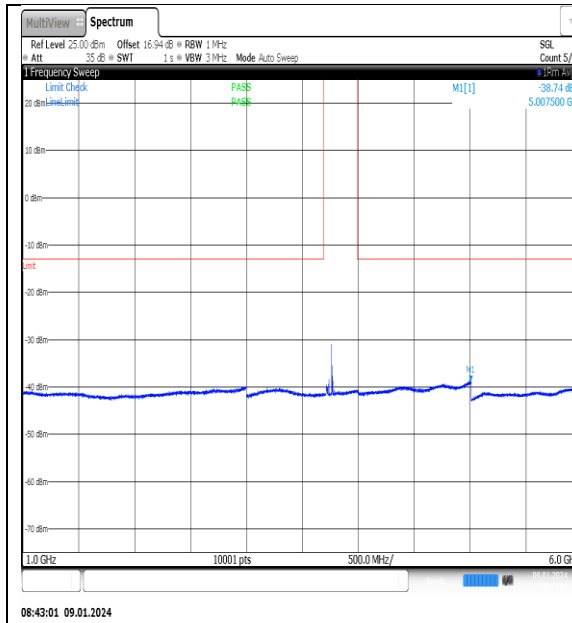
NTNV_N77-3700- 3980_PC2_30_60_L_TID15_NS_01_1000_6000_ #1
