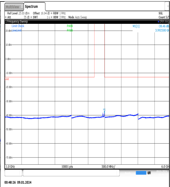
NTNV_N77-3700- 3980_PC2_30_50_H_TID12_NS_01_1000_6000_#1
