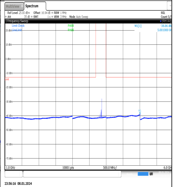
NTNV_N77-3700- 3980_PC2_30_50_M_TID12_NS_01_1000_6000_ #1
