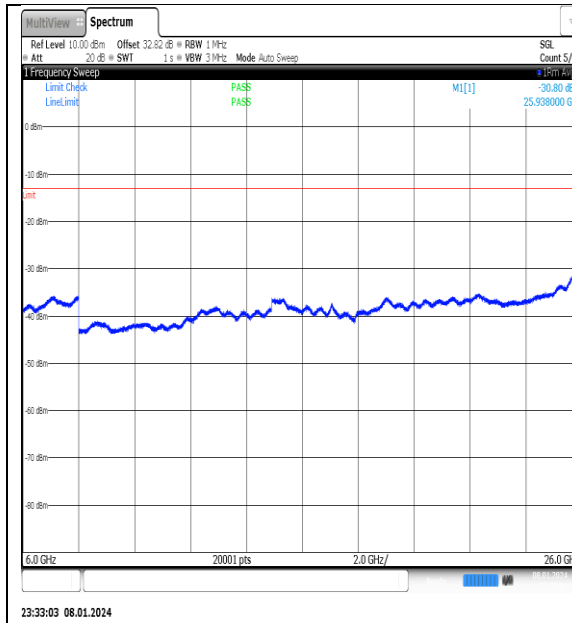
NTNV_N77-3700- 3980_PC2_30_50_M_TID6_NS_01_6000_26000_ #1
