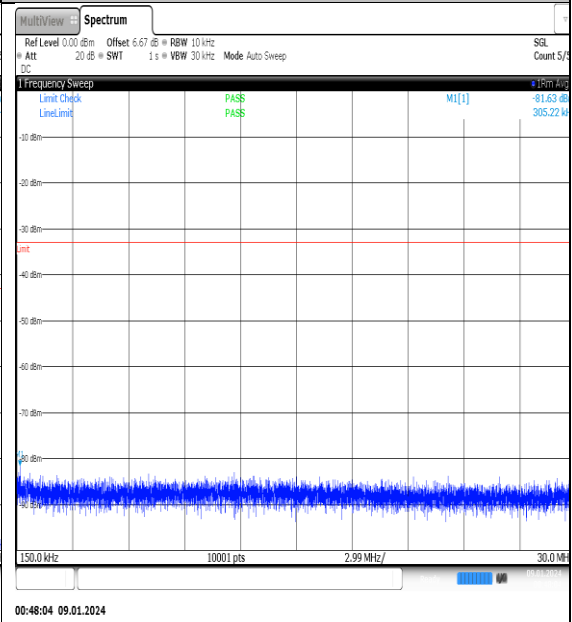
NTNV_N77-3700- 3980_PC2_30_50_H_TID12_NS_01_0.15_30_#1
