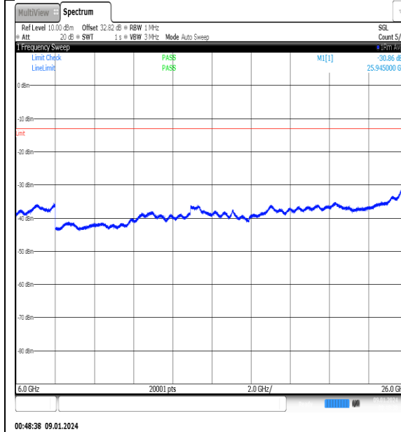
NTNV_N77-3700- 3980_PC2_30_50_H_TID12_NS_01_6000_26000_#1
