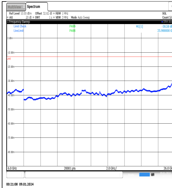
NTNV_N77-3700- 3980_PC2_30_50_H_TID3_NS_01_6000_26000_#1
