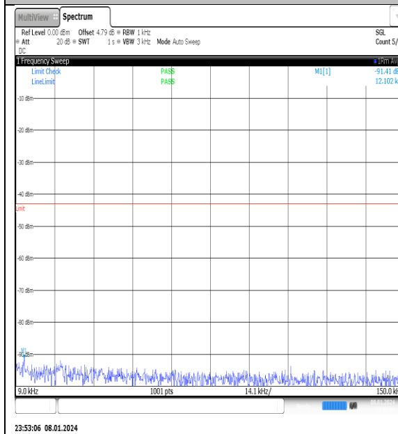
NTNV_N77-3700- 3980_PC2_30_50_M_TID11_NS_01_0.009_0.15_#1
