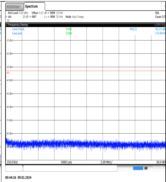
NTNV_N77-3700- 3980_PC2_30_50_H_TID11_NS_01_0.15_30_#1
