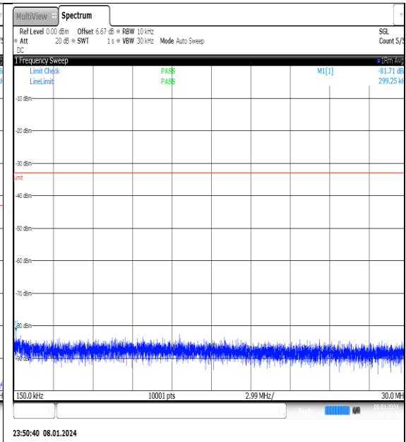
NTNV_N77-3700- 3980_PC2_30_50_M_TID10_NS_01_0.15_30_#1
