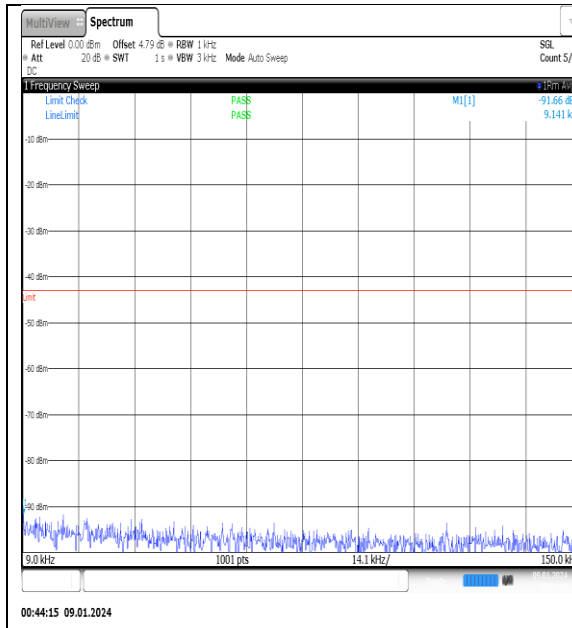
NTNV_N77-3700- 3980_PC2_30_50_H_TID11_NS_01_0.009_0.15_#1
