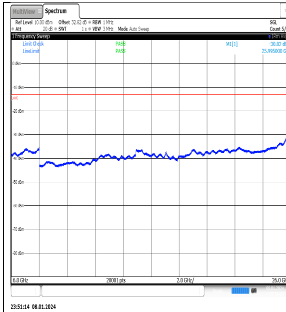
NTNV_N77-3700- 3980_PC2_30_50_M_TID10_NS_01_6000_26000 #1
