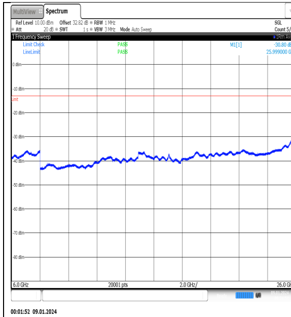
NTNV_N77-3700- 3980_PC2_30_50_M_TID14_NS_01_6000_26000 _#1
