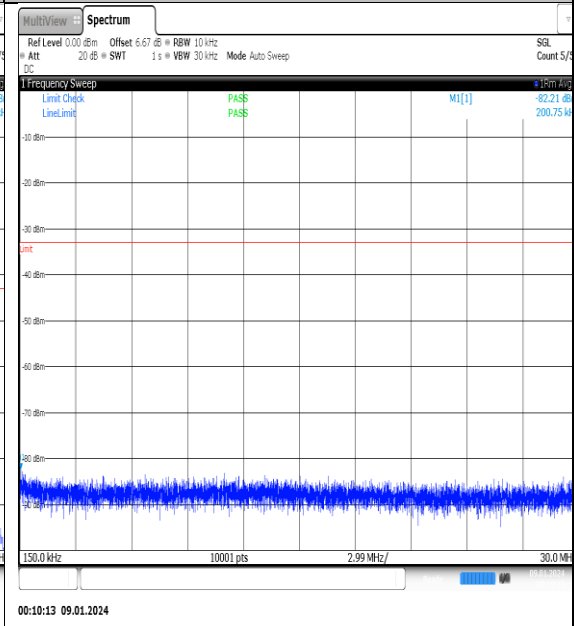
NTNV_N77-3700- 3980_PC2_30_50_H_TID2_NS_01_0.15_30_#1
