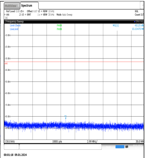
NTNV_N77-3700- 3980_PC2_30_50_M_TID14_NS_01_0.15_30_#1
