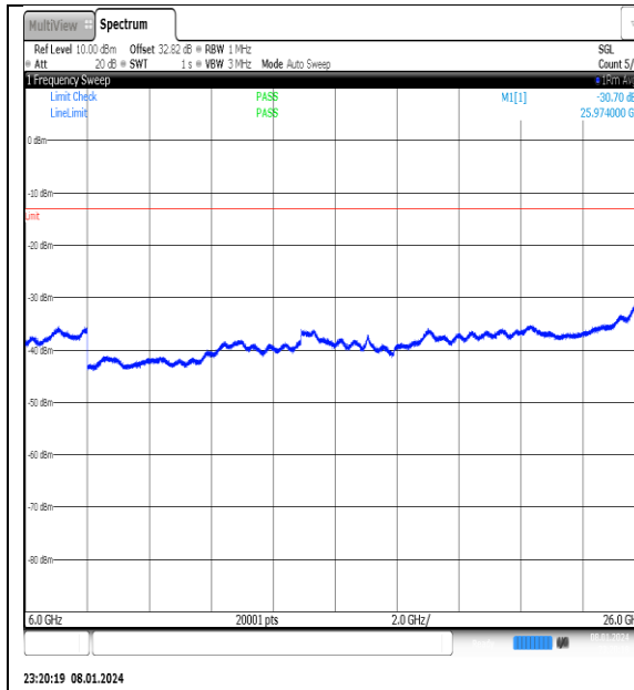
NTNV_N77-3700- 3980_PC2_30_50_M_TID2_NS_01_6000_26000_ #1
