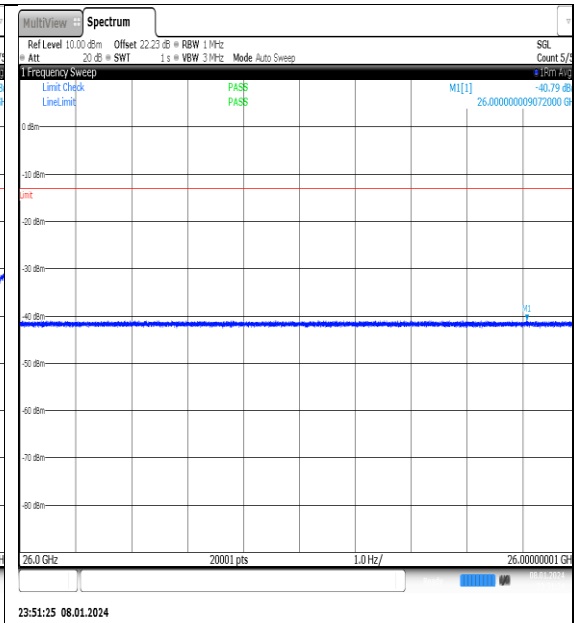
NTNV_N77-3700- 3980_PC2_30_50_M_TID10_NS_01_26000_4000 0_#1
