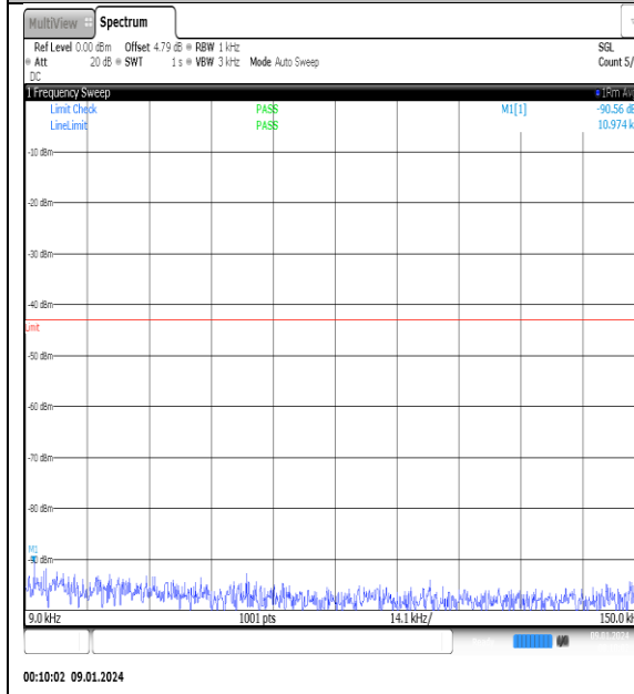
NTNV_N77-3700- 3980_PC2_30_50_H_TID2_NS_01_0.009_0.15_#1
