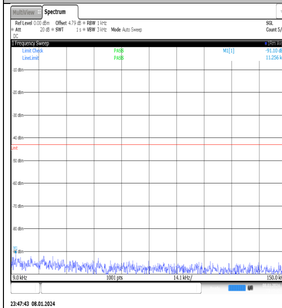
NTNV_N77-3700- 3980_PC2_30_50_M_TID9_NS_01_0.009_0.15_#1
