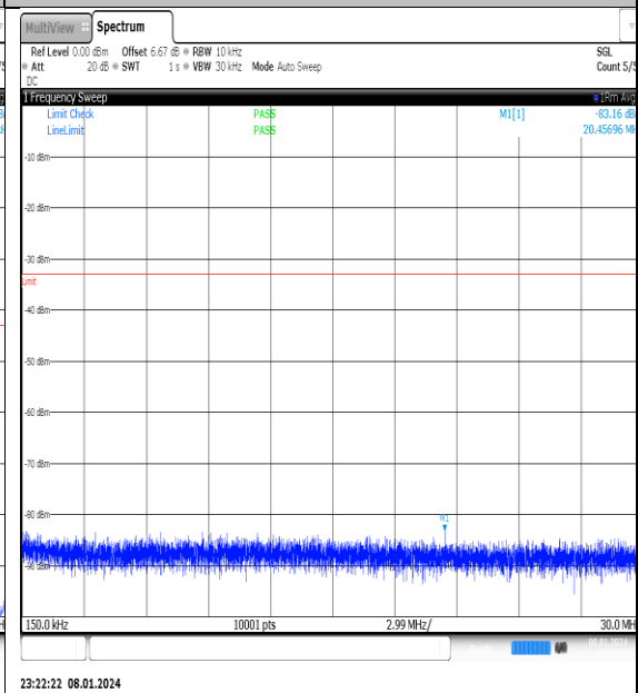
NTNV_N77-3700- 3980_PC2_30_50_M_TID3_NS_01_0.15_30_#1
