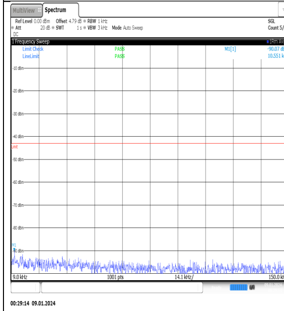
NTNV_N77-3700- 3980_PC2_30_50_H_TID6_NS_01_0.009_0.15_#1
