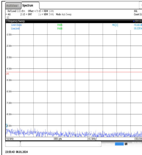
NTNV_N77-3700- 3980_PC2_30_50_M_TID12_NS_01_0.009_0.15_ #1
