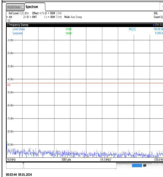
NTNV_N77-3700- 3980_PC2_30_50_M_TID15_NS_01_0.009_0.15_#1
