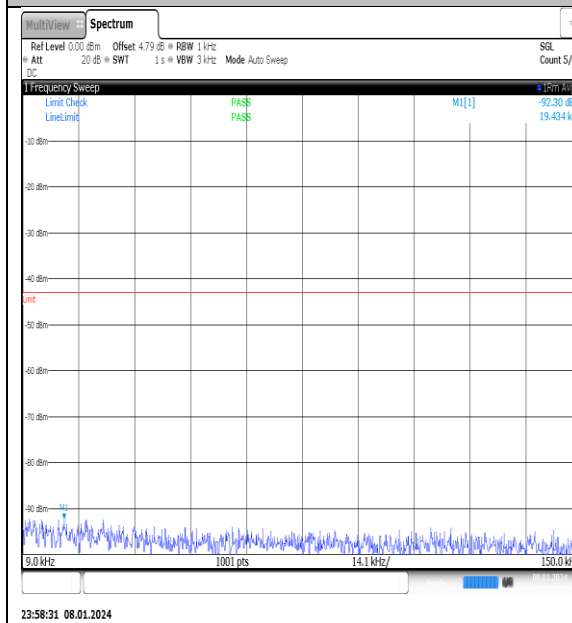
NTNV_N77-3700- 3980_PC2_30_50_M_TID13_NS_01_0.009_0.15_#1
