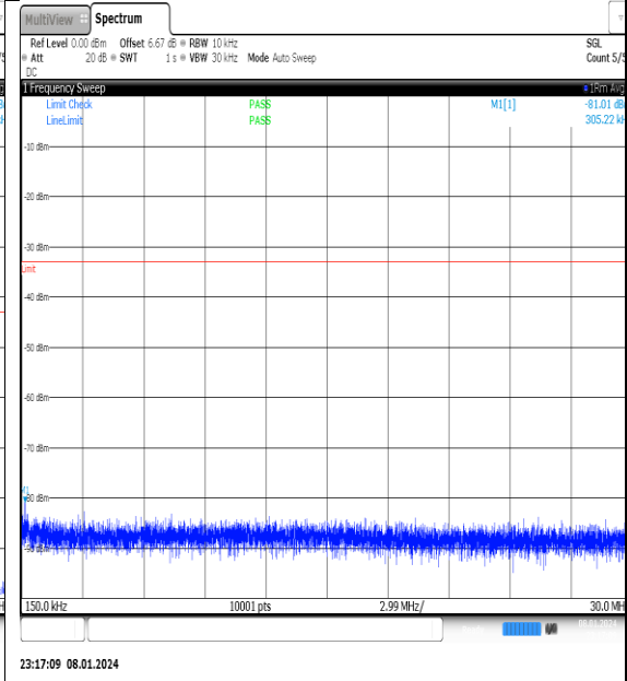
NTNV_N77-3700-3980_PC2_30_50_M_TID1_NS_01_0.15_30_#1
