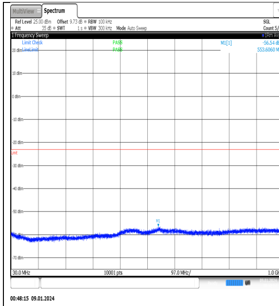
NTNV_N77-3700- 3980_PC2_30_50_H_TID12_NS_01_30_1000_#1
