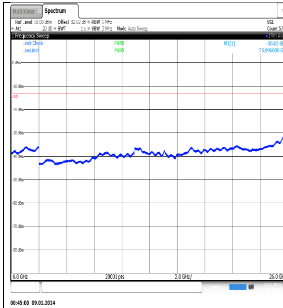
NTNV_N77-3700- 3980_PC2_30_50_H_TID11_NS_01_6000_26000 _#1
