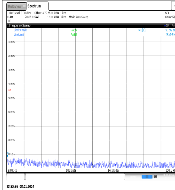
NTNV_N77-3700- 3980_PC2_30_50_M_TID7_NS_01_0.009_0.15_# 1
