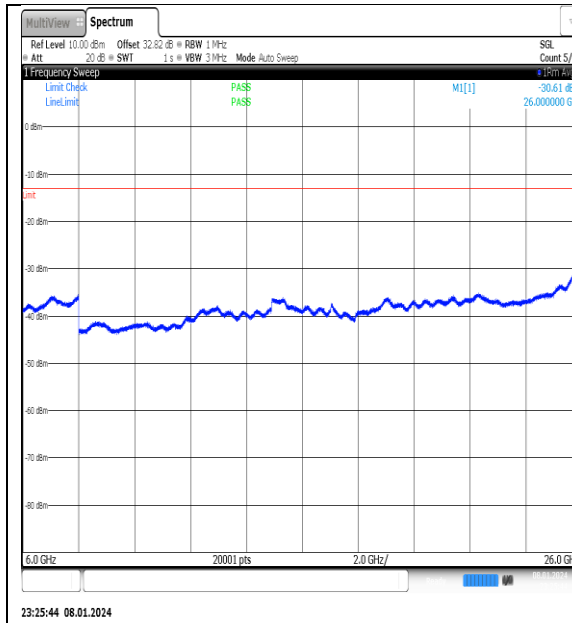
NTNV_N77-3700- 3980_PC2_30_50_M_TID4_NS_01_6000_26000_#1
