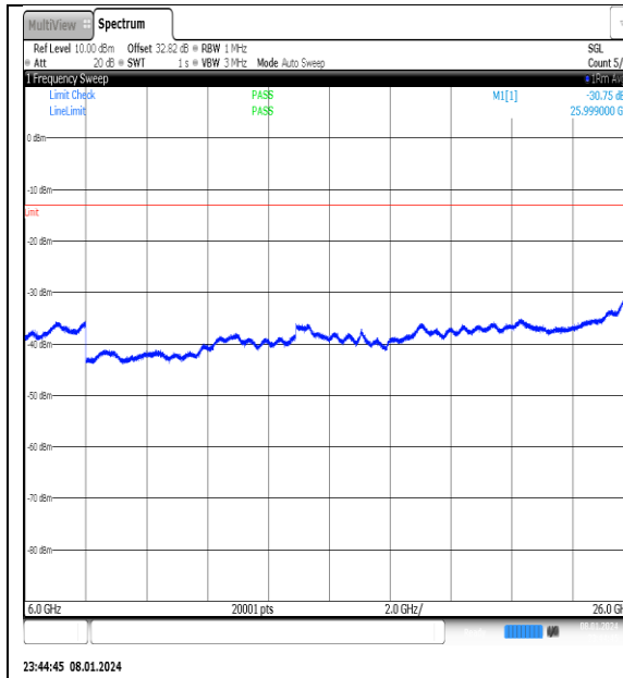
NTNV_N77-3700- 3980_PC2_30_50_M_TID8_NS_01_6000_26000_#1
