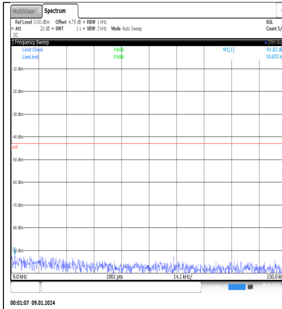
NTNV_N77-3700- 3980_PC2_30_50_M_TID14_NS_01_0.009_0.15_ #1
