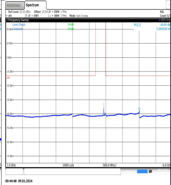
NTNV_N77-3700- 3980_PC2_30_50_H_TID11_NS_01_1000_6000_#1
