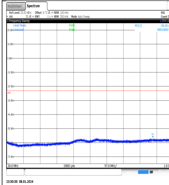
NTNV_N77-3700- 3980_PC2_30_50_M_TID10_NS_01_30_1000_#1
