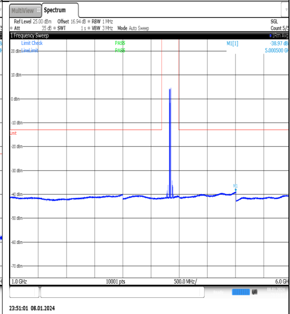
NTNV_N77-3700- 3980_PC2_30_50_M_TID10_NS_01_1000_6000_ #1
