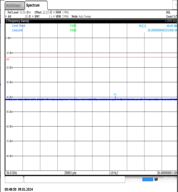
NTNV_N77-3700- 3980_PC2_30_50_H_TID12_NS_01_26000_4000_0_#1
