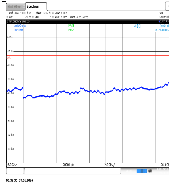
NTNV_N77-3700- 3980_PC2_30_50_H_TID7_NS_01_6000_26000_#1
