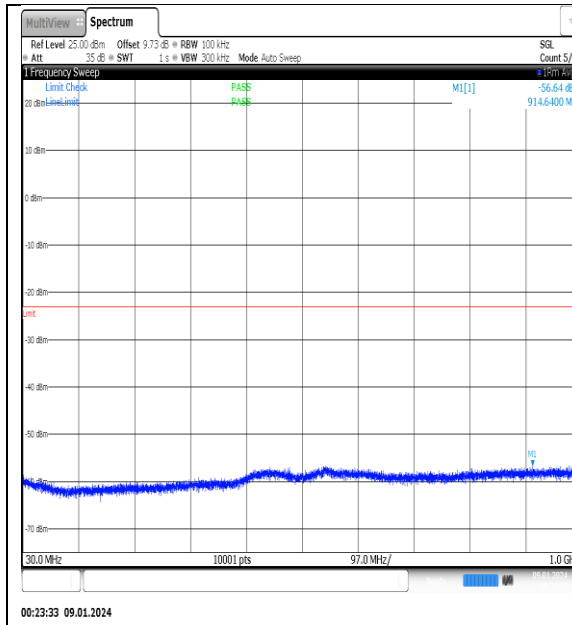
NTNV_N77-3700- 3980_PC2_30_50_H_TID4_NS_01_30_1000_#1
