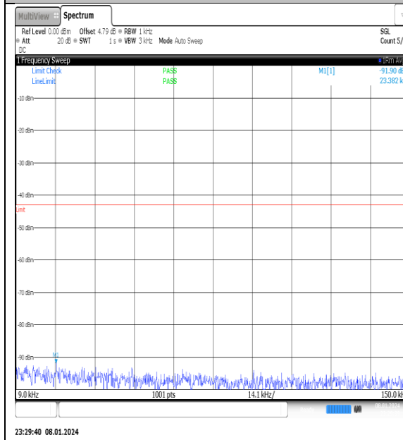
NTNV_N77-3700- 3980_PC2_30_50_M_TID5_NS_01_0.009_0.15_#1
