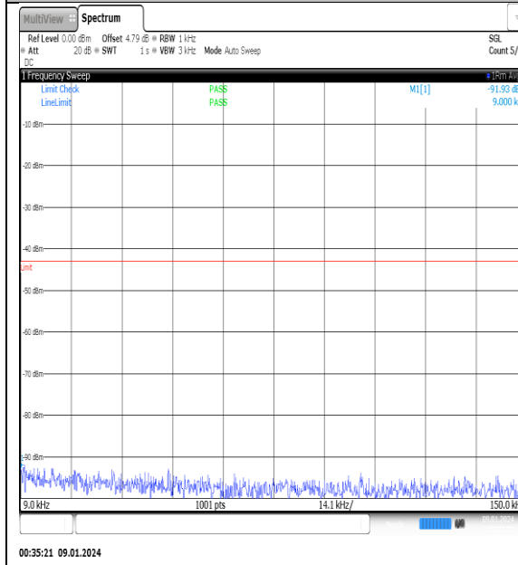
NTNV_N77-3700- 3980_PC2_30_50_H_TID8_NS_01_0.009_0.15_#1
