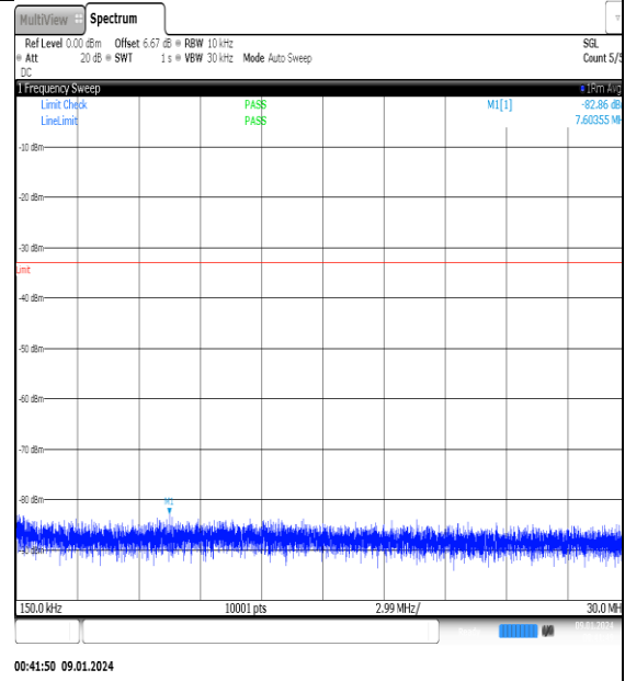
NTNV_N77-3700- 3980_PC2_30_50_H_TID10_NS_01_0.15_30_#1
