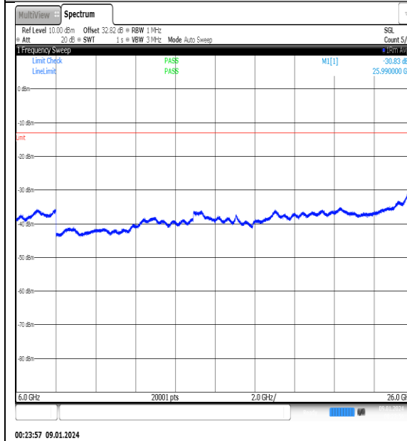
NTNV_N77-3700- 3980_PC2_30_50_H_TID4_NS_01_6000_26000_#1
