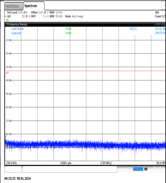
NTNV_N77-3700- 3980_PC2_30_50_H_TID4_NS_01_0.15_30_#1
