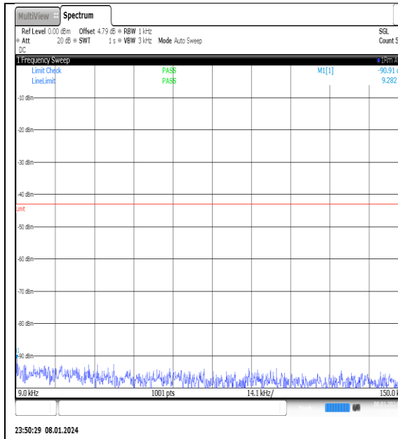
NTNV_N77-3700- 3980_PC2_30_50_M_TID10_NS_01_0.009_0.15_ #1
