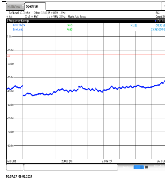
NTNV_N77-3700- 3980_PC2_30_50_H_TID1_NS_01_6000_26000_#1
