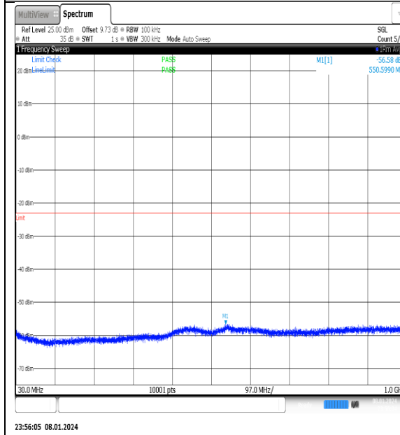
NTNV_N77-3700- 3980_PC2_30_50_M_TID12_NS_01_30_1000_#1
