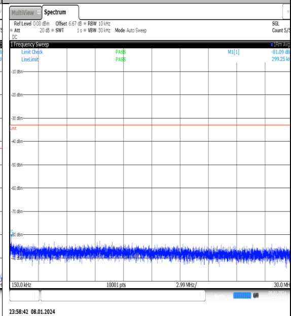
NTNV_N77-3700- 3980_PC2_30_50_M_TID13_NS_01_0.15_30_#1
