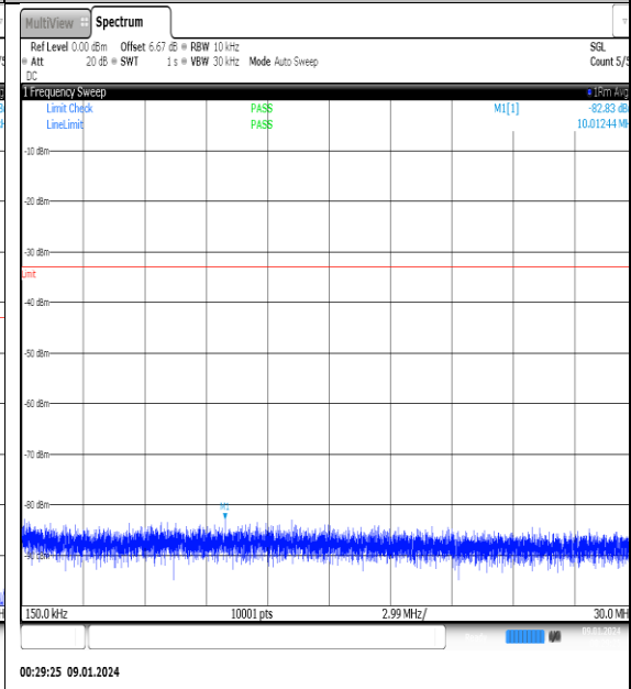
NTNV_N77-3700- 3980_PC2_30_50_H_TID6_NS_01_0.15_30_#1
