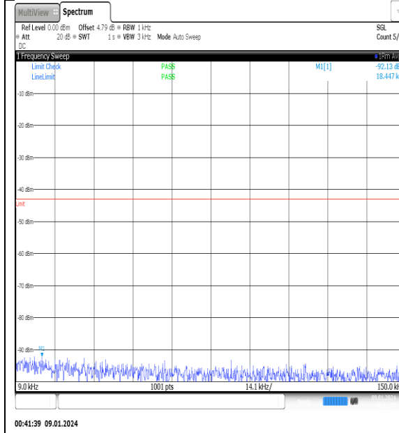
NTNV_N77-3700- 3980_PC2_30_50_H_TID10_NS_01_0.009_0.15_ #1
