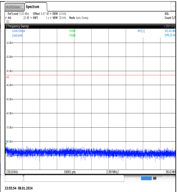
NTNV_N77-3700- 3980_PC2_30_50_M_TID12_NS_01_0.15_30_#1
