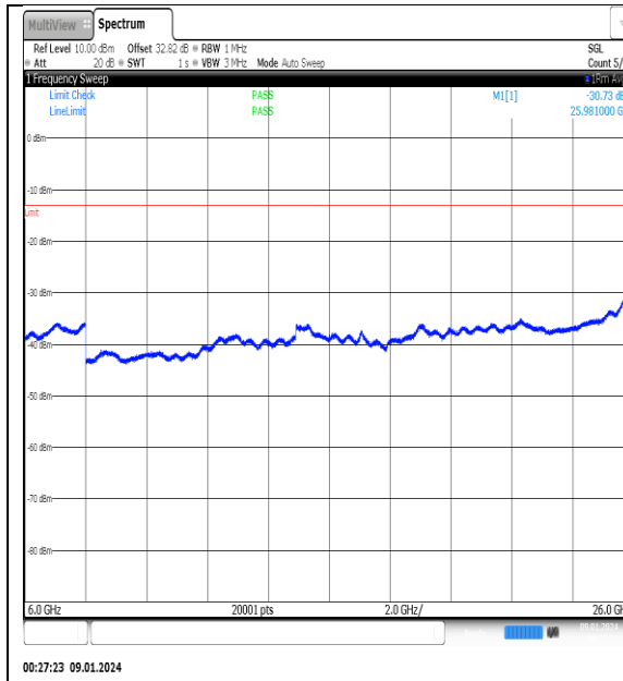
NTNV_N77-3700- 3980_PC2_30_50_H_TID5_NS_01_6000_26000_#1
