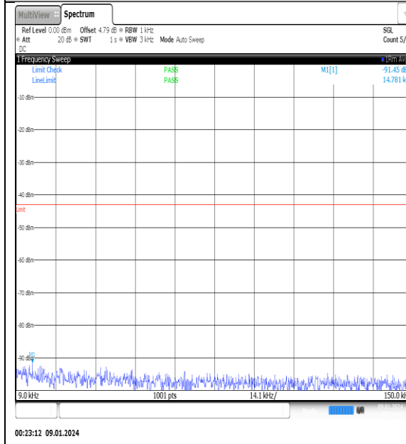
NTNV_N77-3700- 3980_PC2_30_50_H_TID4_NS_01_0.009_0.15_#1
