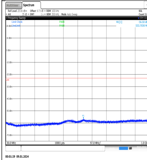
NTNV_N77-3700- 3980_PC2_30_50_M_TID14_NS_01_30_1000_#1
