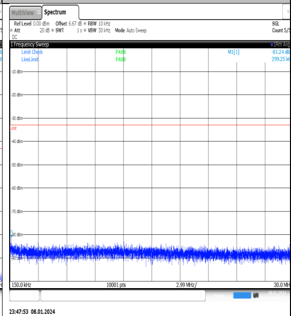
NTNV_N77-3700- 3980_PC2_30_50_M_TID9_NS_01_0.15_30_#1
