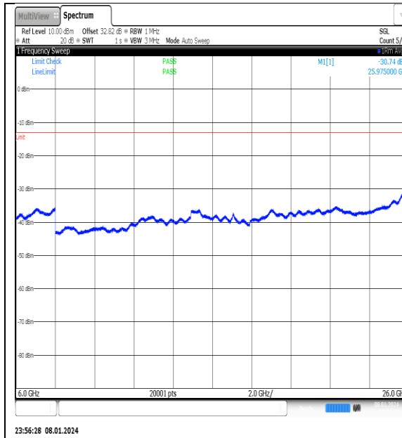
NTNV_N77-3700- 3980_PC2_30_50_M_TID12_NS_01_6000_26000 #1
