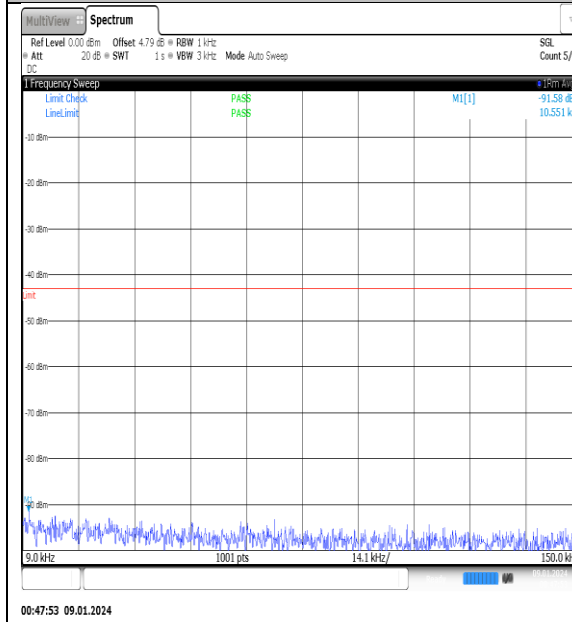
NTNV_N77-3700- 3980_PC2_30_50_H_TID12_NS_01_0.009_0.15_#1
