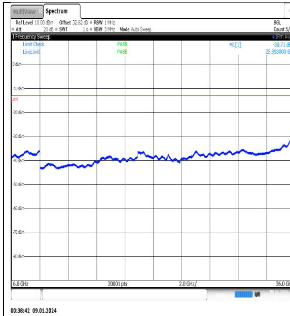
NTNV_N77-3700- 3980_PC2_30_50_H_TID9_NS_01_6000_26000_ #1
