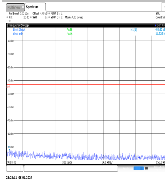
NTNV_N77-3700- 3980_PC2_30_50_M_TID3_NS_01_0.009_0.15_# 1
