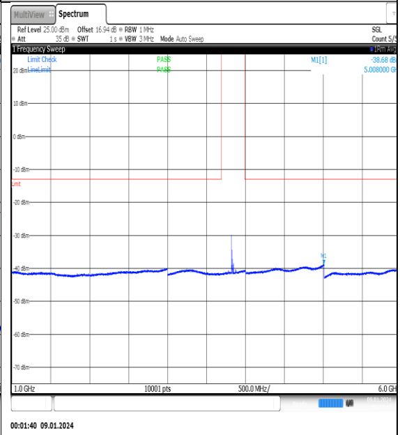
NTNV_N77-3700- 3980_PC2_30_50_M_TID14_NS_01_1000_6000_ #1
