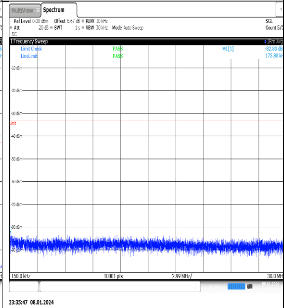
NTNV_N77-3700- 3980_PC2_30_50_M_TID7_NS_01_0.15_30_#1
