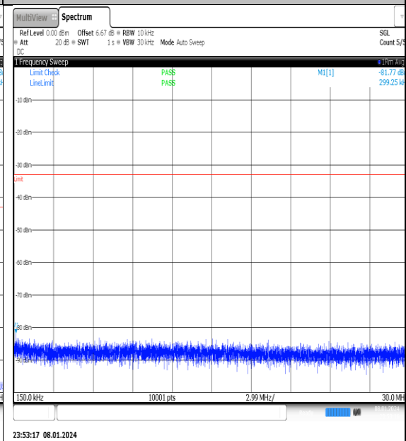
NTNV_N77-3700- 3980_PC2_30_50_M_TID11_NS_01_0.15_30_#1
