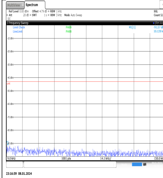
NTNV_N77-3700-3980_PC2_30_50_M_TID1_NS_01_0.009_0.15_#1
