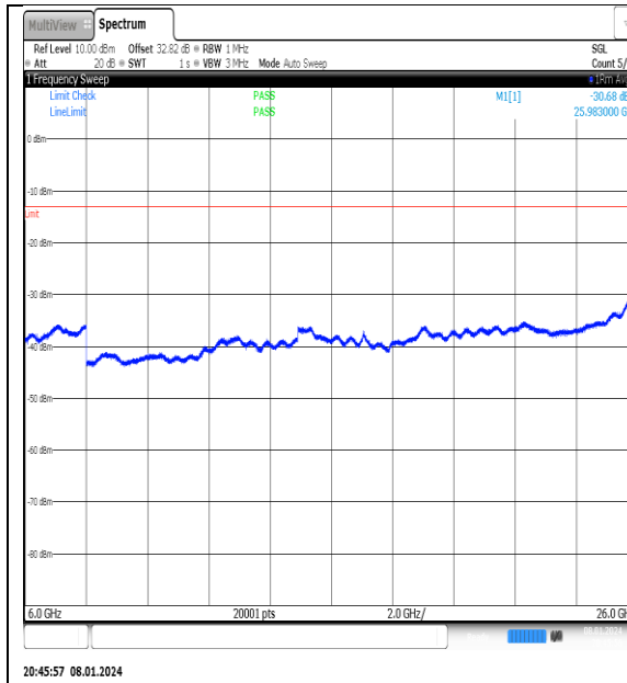
NTNV_N77-3700- 3980_PC2_30_40_L_TID14_NS_01_6000_26000 _#1
