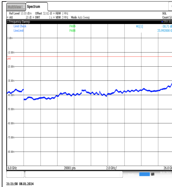
NTNV_N77-3700- 3980_PC2_30_40_M_TID11_NS_01_6000_26000 _#1
