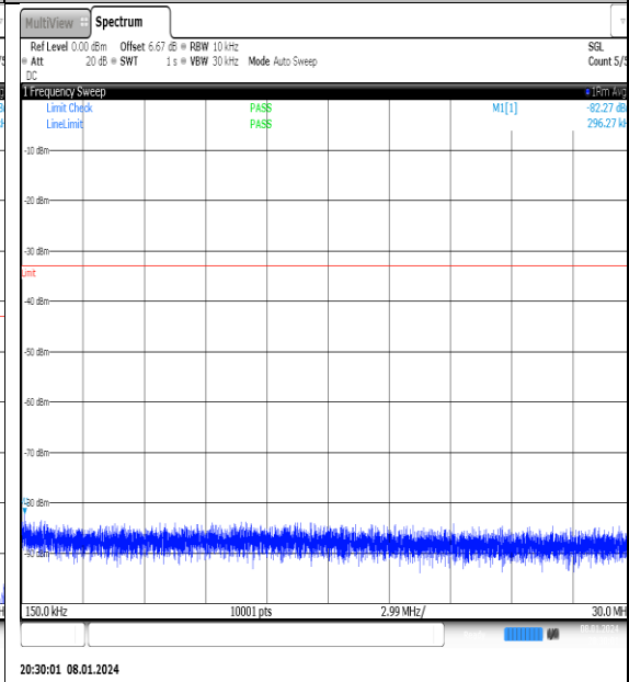
NTNV_N77-3700- 3980_PC2_30_40_L_TID9_NS_01_0.15_30_#1
