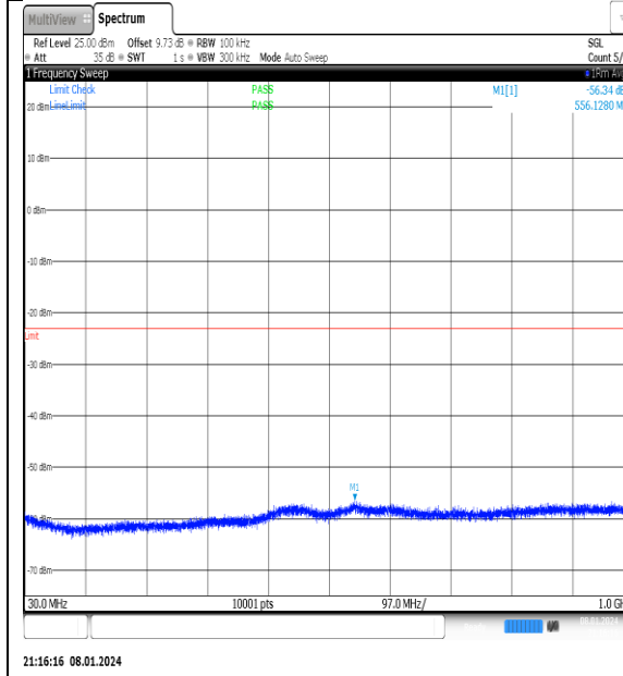
NTNV_N77-3700- 3980_PC2_30_40_M_TID9_NS_01_30_1000_#1
