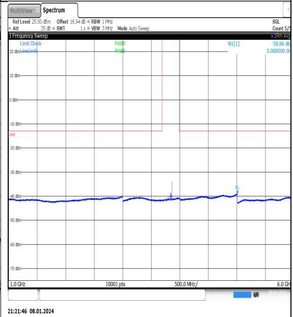
NTN_V_N77-3700- 3980_PC2_30_40_M_TID11_NS_01_1000_6000_ #1
