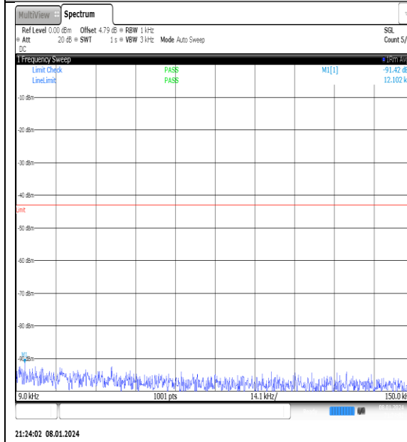
NTNV_N77-3700- 3980_PC2_30_40_M_TID12_NS_01_0.009_0.15_ _#1
