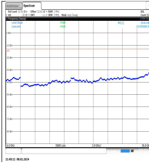
NTNV_N77-3700- 3980_PC2_30_40_H_TID2_NS_01_6000_26000_#1
