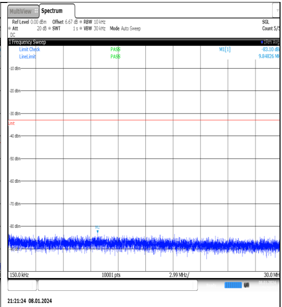
NTN_V_N77-3700- 3980_PC2_30_40_M_TID11_NS_01_0.15_30_#1
