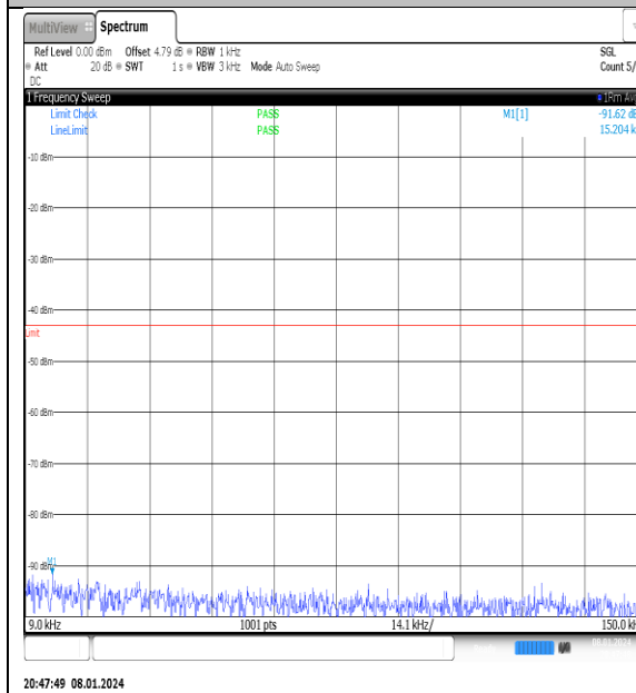
NTNV_N77-3700- 3980_PC2_30_40_L_TID15_NS_01_0.009_0.15_#1
