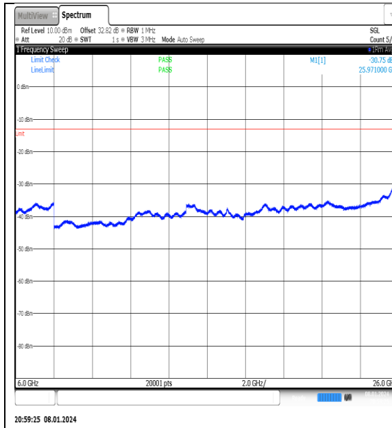
NTNV_N77-3700- 3980_PC2_30_40_M_TID3_NS_01_6000_26000_#1
