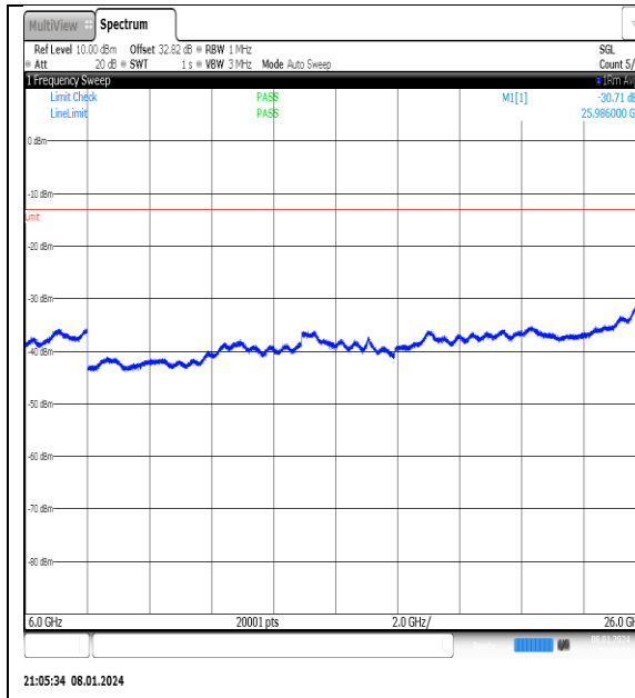
NTNV_N77-3700- 3980_PC2_30_40_M_TID5_NS_01_6000_26000_ #1
