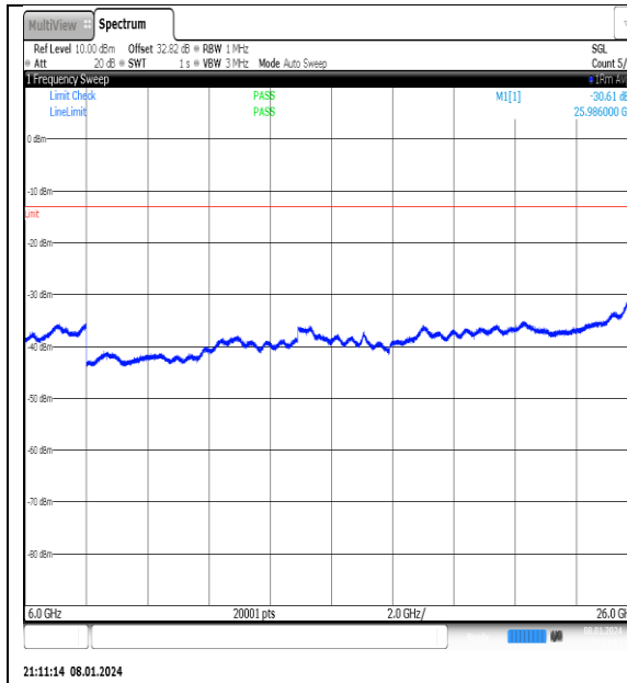
NTNV_N77-3700- 3980_PC2_30_40_M_TID7_NS_01_6000_26000_#1
