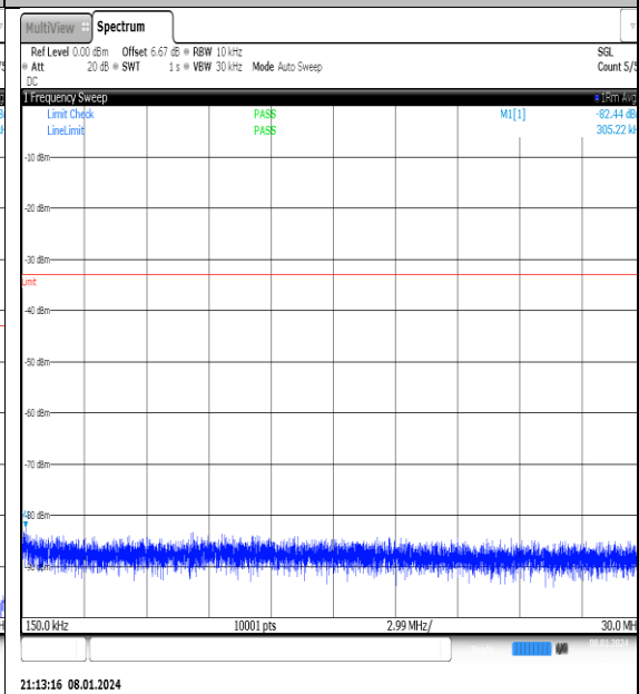
NTNV_N77-3700- 3980_PC2_30_40_M_TID8_NS_01_0.15_30_#1
