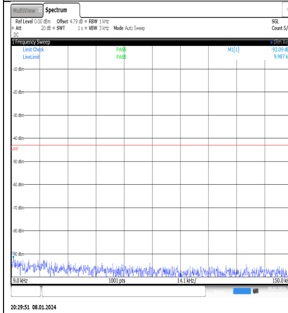
NTNV_N77-3700- 3980_PC2_30_40_L_TID9_NS_01_0.009_0.15_# 1
