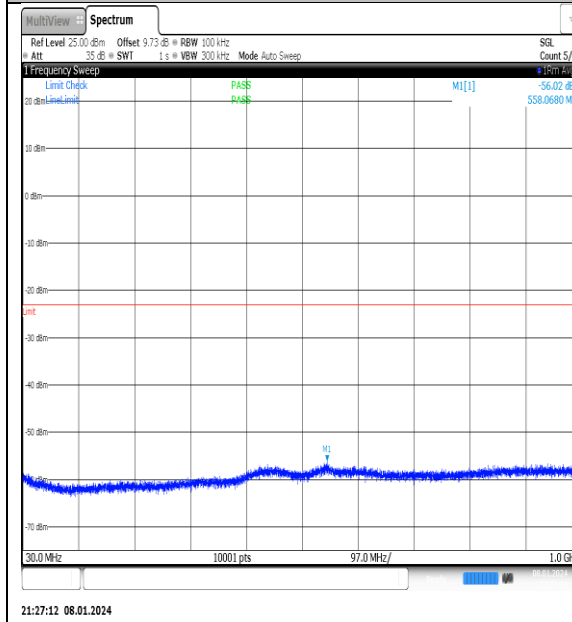
NTN_V_N77-3700- 3980_PC2_30_40_M_TID13_NS_01_30_1000_#1
