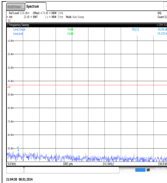
NTNV_N77-3700- 3980_PC2_30_40_M_TID5_NS_01_0.009_0.15_# 1
