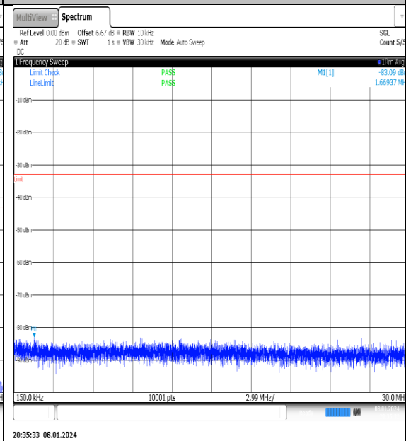
NTNV_N77-3700-3980_PC2_30_40_L_TID11_NS_01_0.15_30_#1
