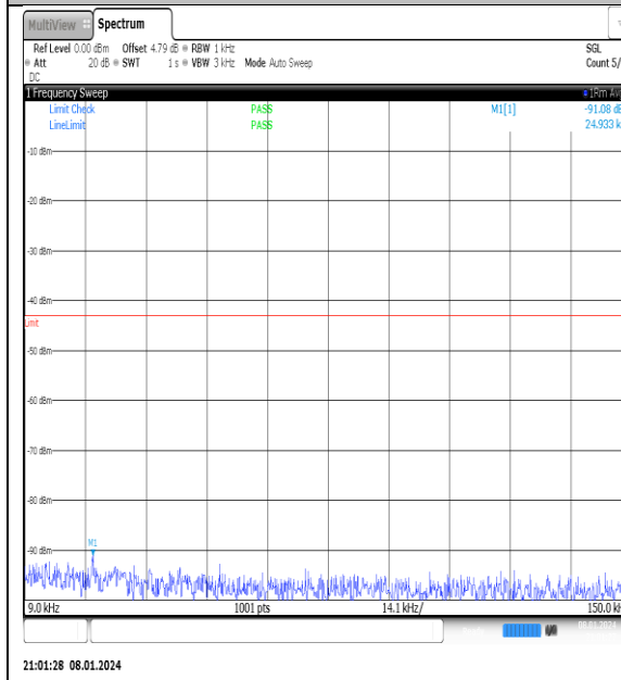
NTNV_N77-3700- 3980_PC2_30_40_M_TID4_NS_01_0.009_0.15_#1
