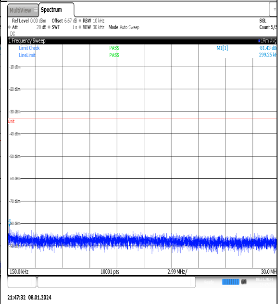
NTNV_N77-3700- 3980_PC2_30_40_H_TID3_NS_01_0.15_30_#1
