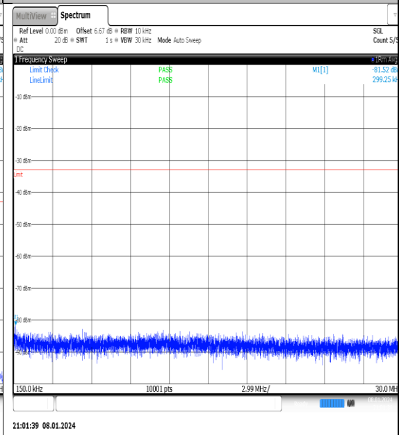
NTNV_N77-3700- 3980_PC2_30_40_M_TID4_NS_01_0.15_30_#1
