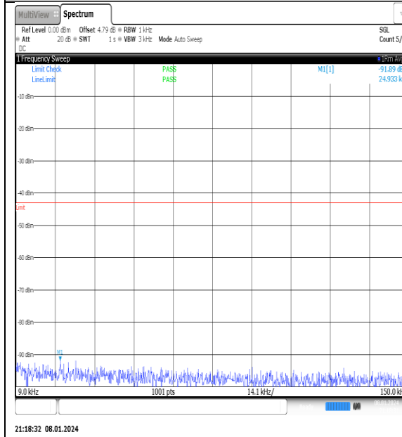
NTNV_N77-3700- 3980_PC2_30_40_M_TID10_NS_01_0.009_0.15_#1
