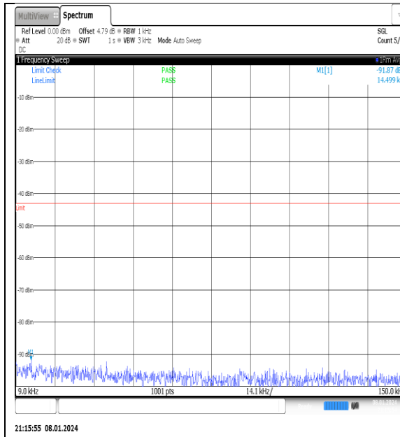
NTNV_N77-3700- 3980_PC2_30_40_M_TID9_NS_01_0.009_0.15_# 1
