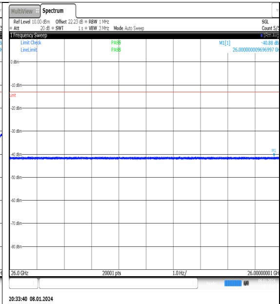
NTNV_N77-3700-3980_PC2_30_40_L_TID10_NS_01_26000_4000_0_#1
