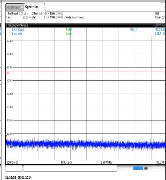
NTNV_N77-3700- 3980_PC2_30_40_M_TID14_NS_01_0.15_30_#1
