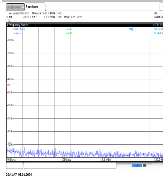
NTNV_N77-3700- 3980_PC2_30_40_L_TID13_NS_01_0.009_0.15_#1
