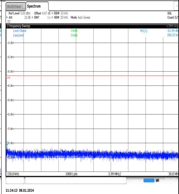
NTNV_N77-3700- 3980_PC2_30_40_M_TID12_NS_01_0.15_30_#1
