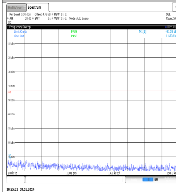
NTNV_N77-3700-3980_PC2_30_40_L_TID11_NS_01_0.009_0.15_#1
