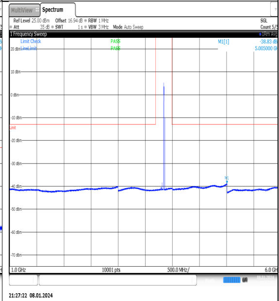
NTN_V_N77-3700- 3980_PC2_30_40_M_TID13_NS_01_1000_6000_ #1
