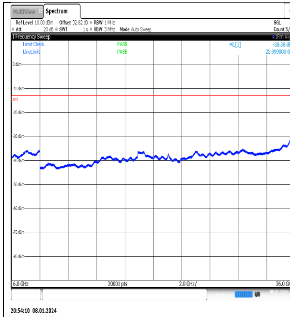
NTNV_N77-3700- 3980_PC2_30_40_M_TID1_NS_01_6000_26000_#1
