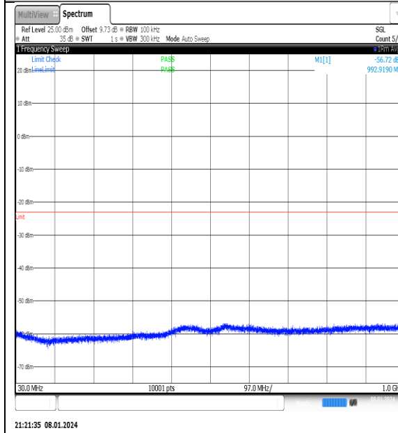
NTN_V_N77-3700- 3980_PC2_30_40_M_TID11_NS_01_30_1000_#1
