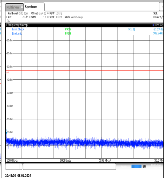
NTNV_N77-3700- 3980_PC2_30_40_L_TID15_NS_01_0.15_30_#1
