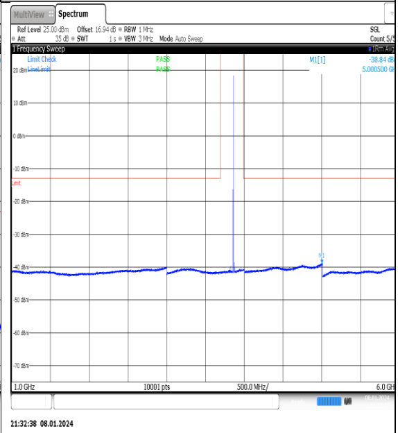
NTN_V_N77-3700- 3980_PC2_30_40_M_TID15_NS_01_1000_6000_ #1
