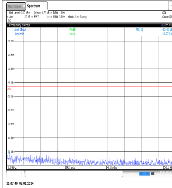
NTNV_N77-3700- 3980_PC2_30_40_M_TID6_NS_01_0.009_0.15_# 1
