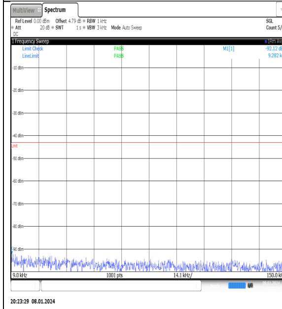
NTNV_N77-3700- 3980_PC2_30_40_L_TID7_NS_01_0.009_0.15_# 1
