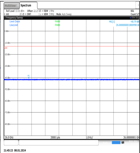
NTNV_N77-3700- 3980_PC2_30_40_H_TID2_NS_01_26000_40000_#1
