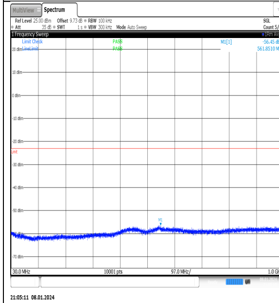
NTNV_N77-3700- 3980_PC2_30_40_M_TID5_NS_01_30_1000_#1
