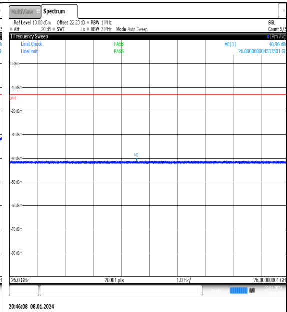
NTNV_N77-3700- 3980_PC2_30_40_L_TID14_NS_01_26000_4000 0_#1
