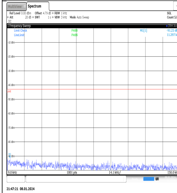
NTNV_N77-3700- 3980_PC2_30_40_H_TID3_NS_01_0.009_0.15_#1
