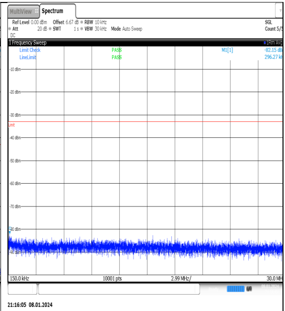
NTNV_N77-3700- 3980_PC2_30_40_M_TID9_NS_01_0.15_30_#1
