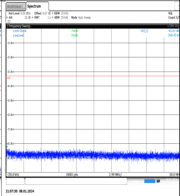
NTNV_N77-3700- 3980_PC2_30_40_M_TID6_NS_01_0.15_30_#1
