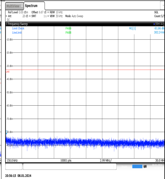
NTNV_N77-3700- 3980_PC2_30_40_M_TID2_NS_01_0.15_30_#1
