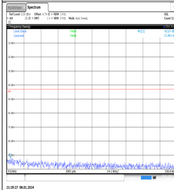
NTNV_N77-3700- 3980_PC2_30_40_M_TID14_NS_01_0.009_0.15_ _#1
