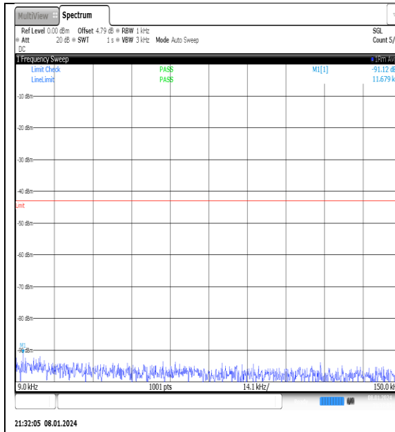
NTN_V_N77-3700- 3980_PC2_30_40_M_TID15_NS_01_0.009_0.15_ #1
