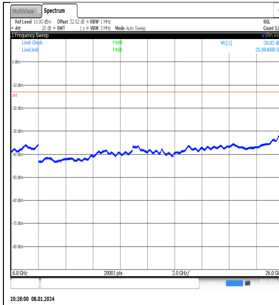
NTNV_N77-3700- 3980_PC2_30_40_L_TID8_NS_01_6000_26000_ #1
