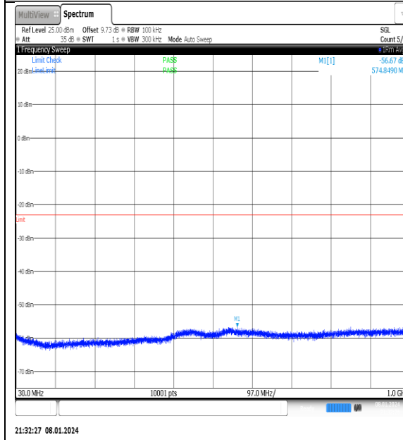
NTN_V_N77-3700- 3980_PC2_30_40_M_TID15_NS_01_30_1000_#1
