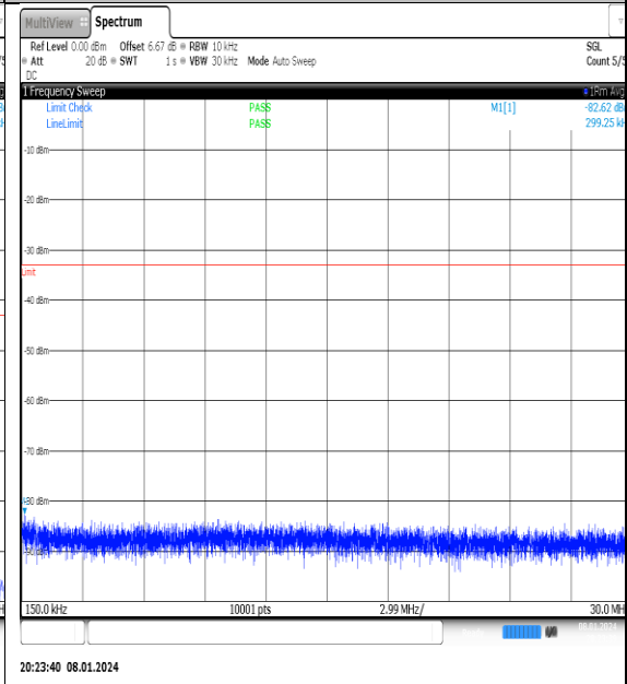
NTNV_N77-3700- 3980_PC2_30_40_L_TID7_NS_01_0.15_30_#1
