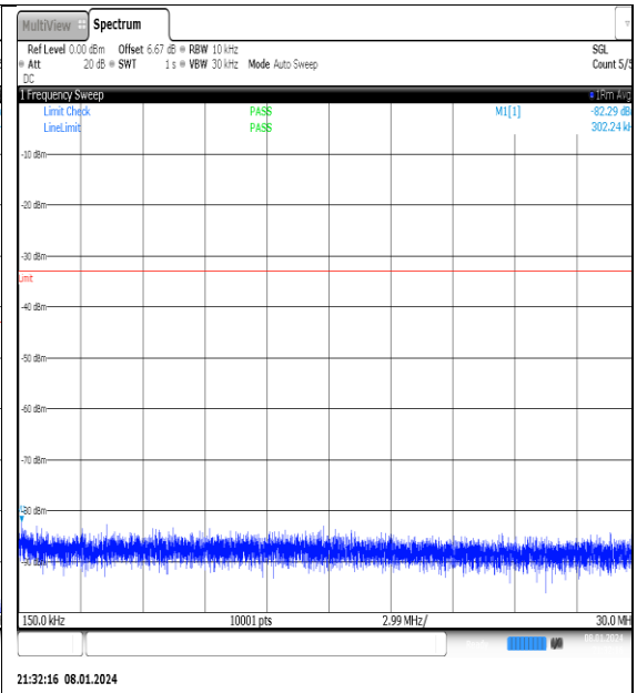
NTN_V_N77-3700- 3980_PC2_30_40_M_TID15_NS_01_0.15_30_#1
