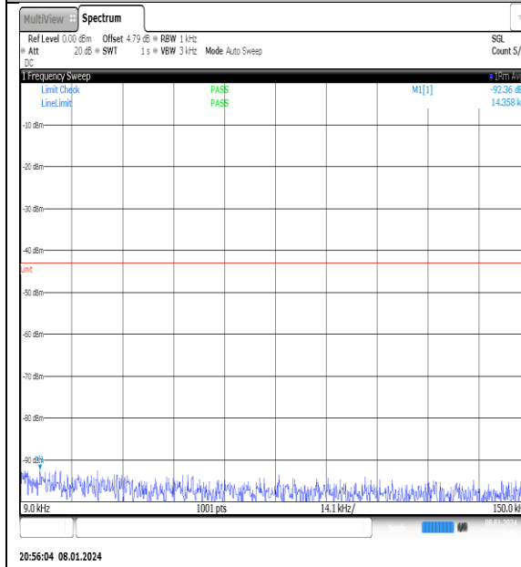
NTNV_N77-3700- 3980_PC2_30_40_M_TID2_NS_01_0.009_0.15_#1
