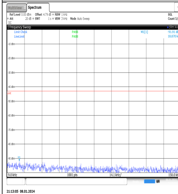
NTNV_N77-3700- 3980_PC2_30_40_M_TID8_NS_01_0.009_0.15_#1
