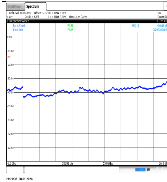
NTNV_N77-3700- 3980_PC2_30_40_M_TID13_NS_01_6000_26000 _#1
