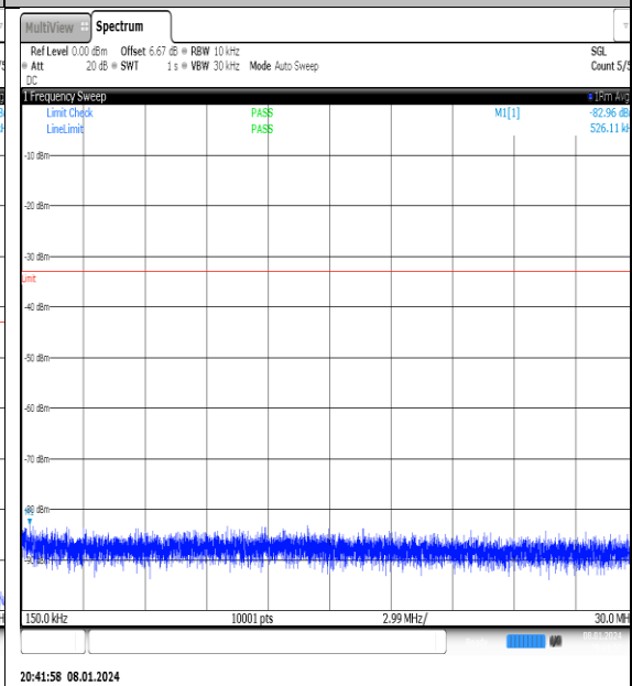
NTNV_N77-3700- 3980_PC2_30_40_L_TID13_NS_01_0.15_30_#1
