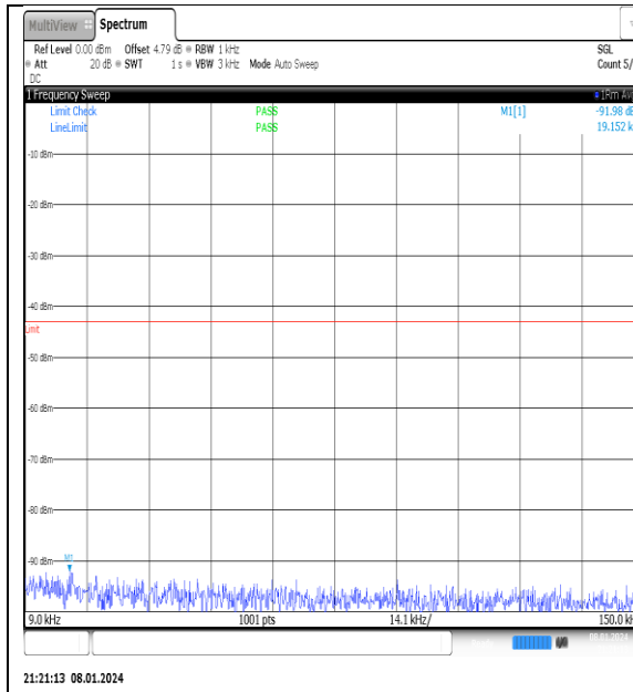
NTN_V_N77-3700- 3980_PC2_30_40_M_TID11_NS_01_0.009_0.15_ #1
