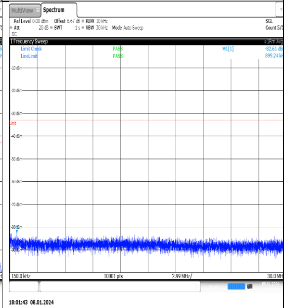
NTNV_N77-3700- 3980_PC2_30_30_L_TID10_NS_01_0.15_30_#1
