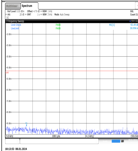
NTNV_N77-3700- 3980_PC2_30_30_L_TID14_NS_01_0.009_0.15_#1
