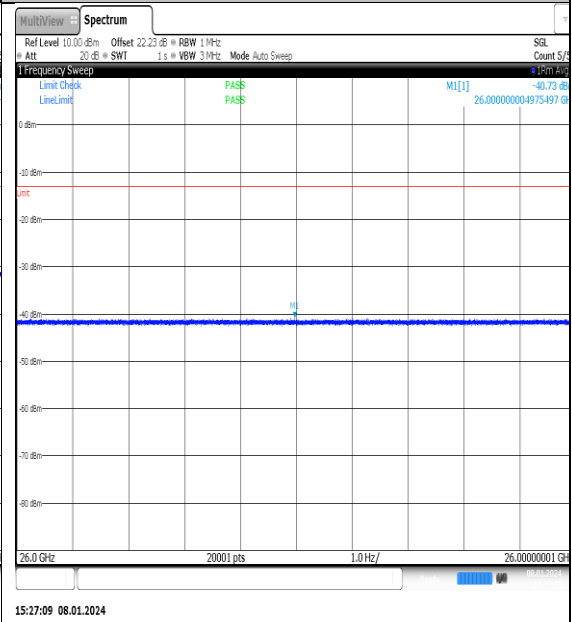
NTNV_N77-3700- 3980_PC2_30_25_H_TID13_NS_01_26000_4000_0_#1
