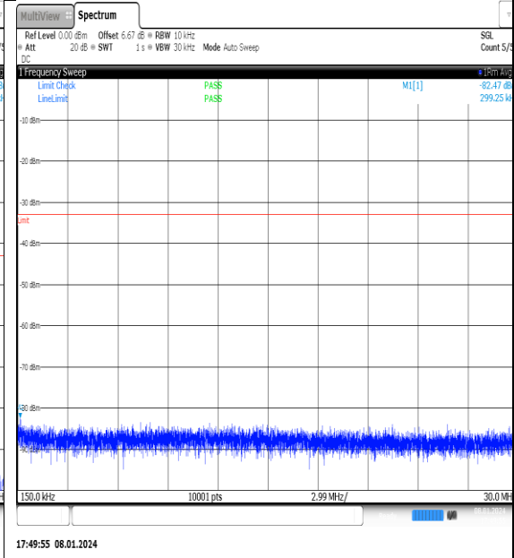
NTNV_N77-3700- 3980_PC2_30_30_L_TID6_NS_01_0.15_30_#1
