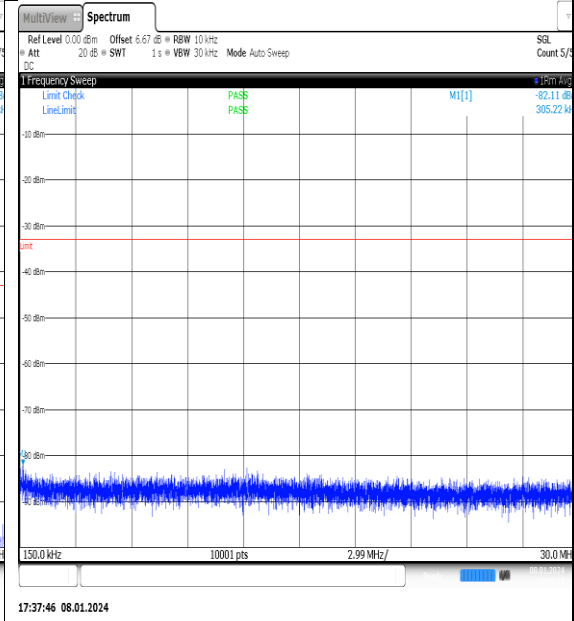
NTNV_N77-3700- 3980_PC2_30_30_L_TID2_NS_01_0.15_30_#1
