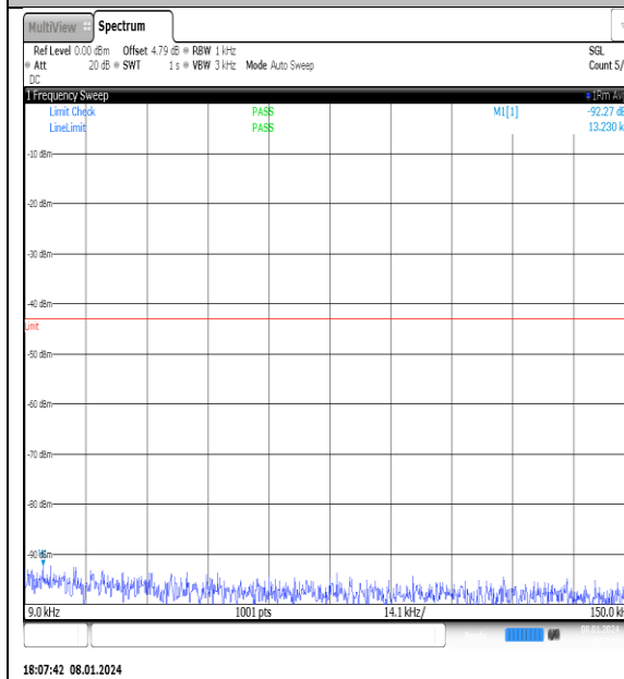
NTNV_N77-3700- 3980_PC2_30_30_L_TID12_NS_01_0.009_0.15_#1
