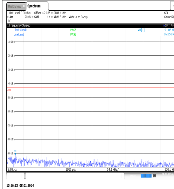
NTNV_N77-3700- 3980_PC2_30_25_H_TID13_NS_01_0.009_0.15_#1
