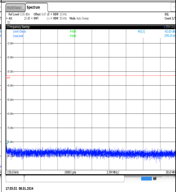
NTNV_N77-3700- 3980_PC2_30_30_L_TID8_NS_01_0.15_30_#1
