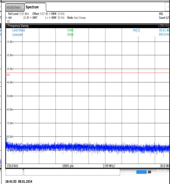
NTNV_N77-3700- 3980_PC2_30_30_M_TID7_NS_01_0.15_30_#1
