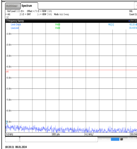
NTNV_N77-3700- 3980_PC2_30_30_M_TID1_NS_01_0.009_0.15_# 1
