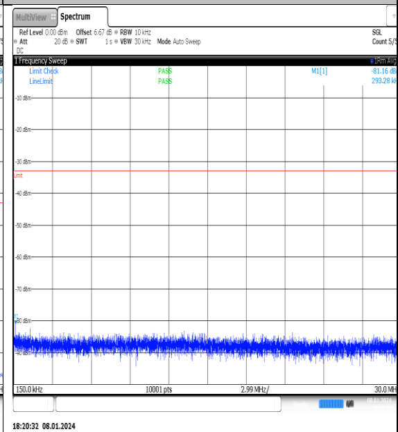
NTNV_N77-3700- 3980_PC2_30_30_M_TID1_NS_01_0.15_30_#1
