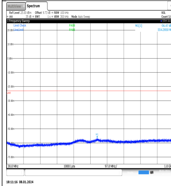
NTN_V_N77-3700- 3980_PC2_30_30_L_TID13_NS_01_30_1000_#1
