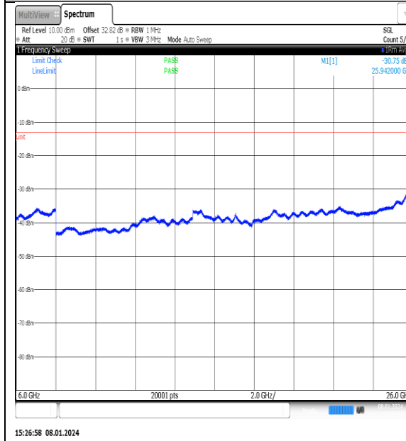
NTNV_N77-3700- 3980_PC2_30_25_H_TID13_NS_01_6000_26000_#1
