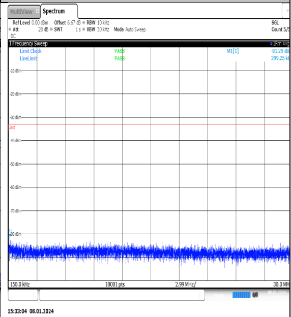
NTNV_N77-3700- 3980_PC2_30_25_H_TID15_NS_01_0.15_30_#1
