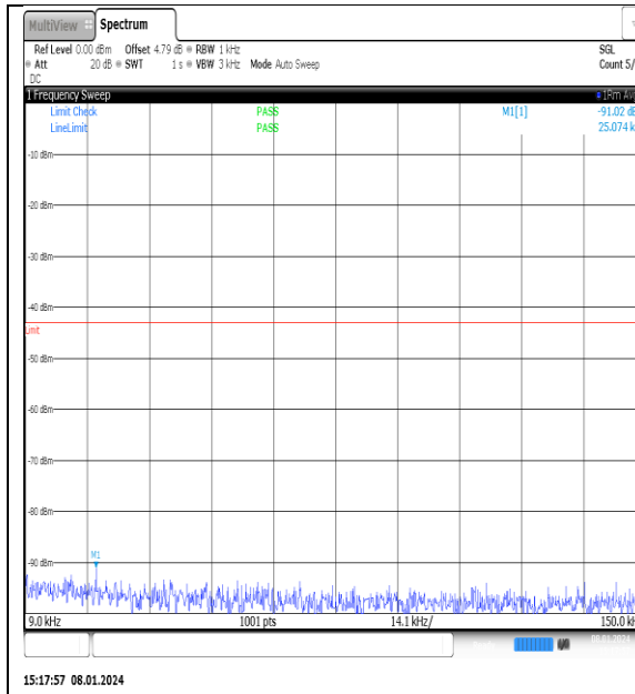
NTNV_N77-3700- 3980_PC2_30_25_H_TID12_NS_01_0.009_0.15_ #1
