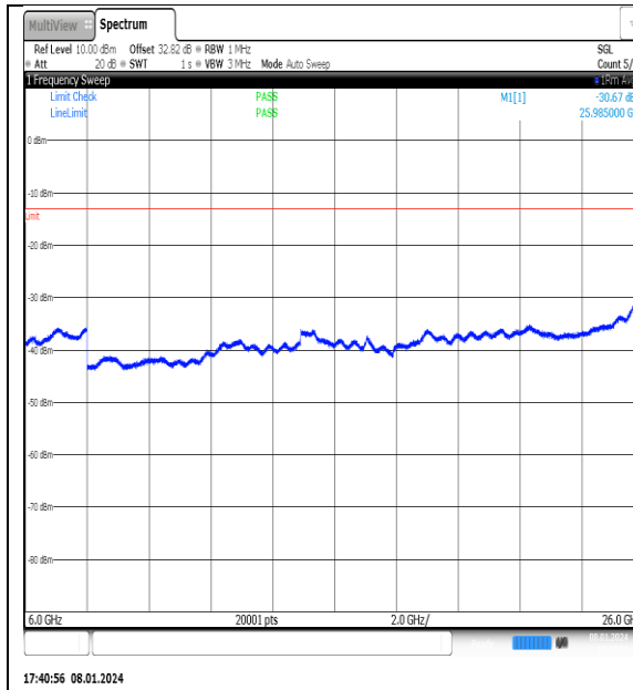
NTNV_N77-3700- 3980_PC2_30_30_L_TID3_NS_01_6000_26000_ #1
