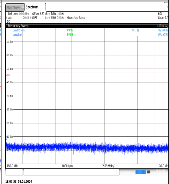
NTNV_N77-3700- 3980_PC2_30_30_L_TID12_NS_01_0.15_30_#1
