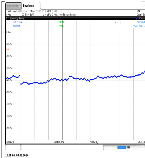
NTNV_N77-3700- 3980_PC2_30_30_L_TID1_NS_01_6000_26000_ #1
