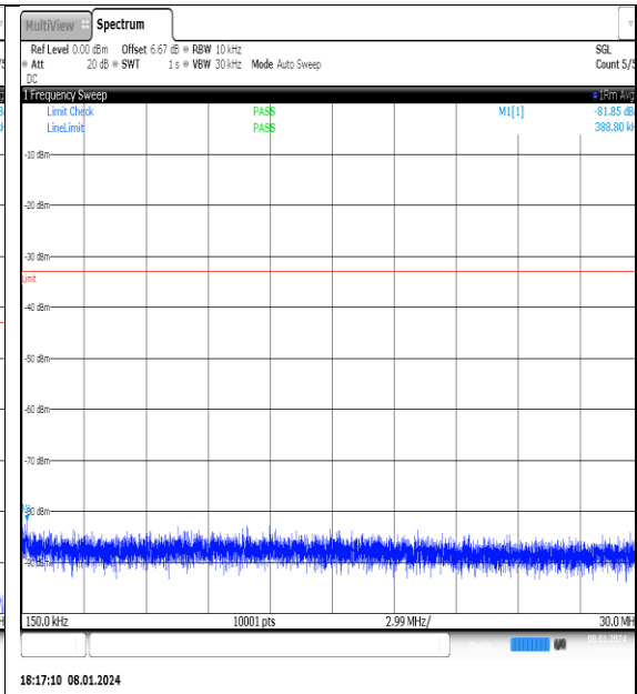
NTN_V_N77-3700- 3980_PC2_30_30_L_TID15_NS_01_0.15_30_#1
