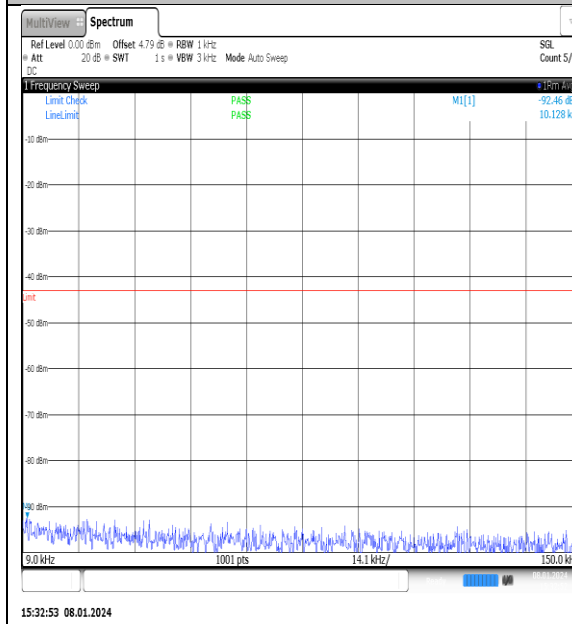
NTNV_N77-3700- 3980_PC2_30_25_H_TID15_NS_01_0.009_0.15_#1
