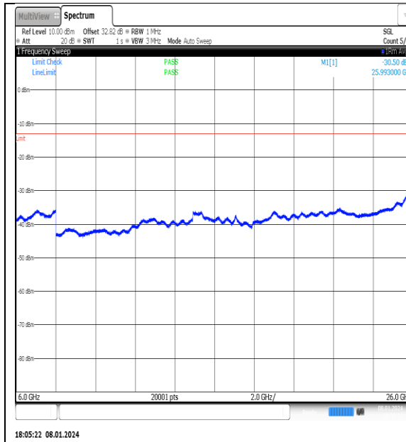
NTNV_N77-3700- 3980_PC2_30_30_L_TID11_NS_01_6000_26000 _#1
