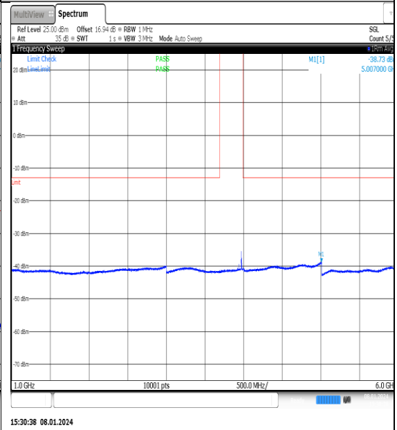
NTNV_N77-3700- 3980_PC2_30_25_H_TID14_NS_01_1000_6000_ #1
