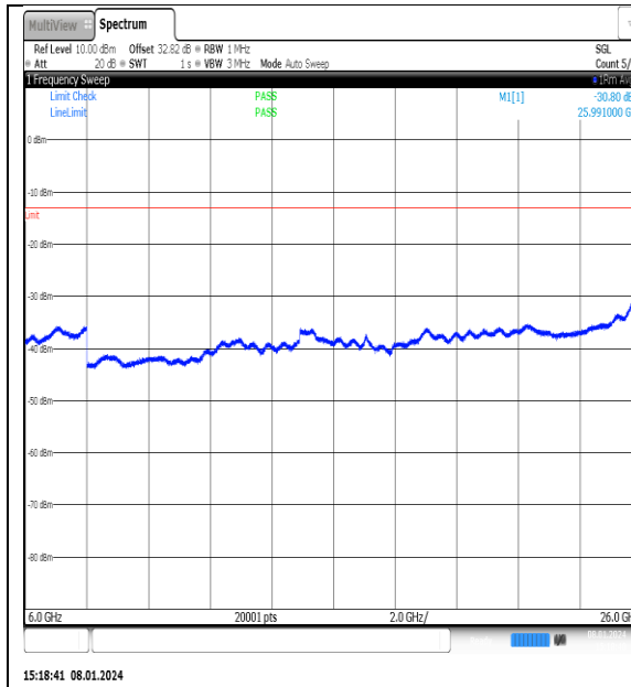
NTNV_N77-3700- 3980_PC2_30_25_H_TID12_NS_01_6000_26000 _#1
