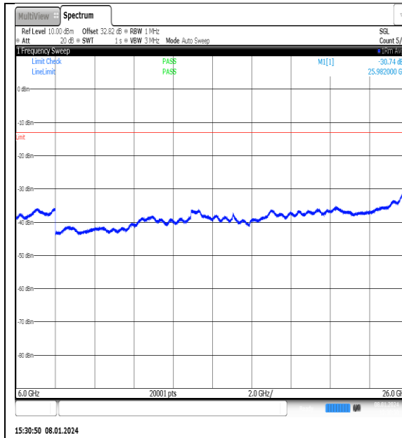
NTNV_N77-3700- 3980_PC2_30_25_H_TID14_NS_01_6000_26000 _#1
