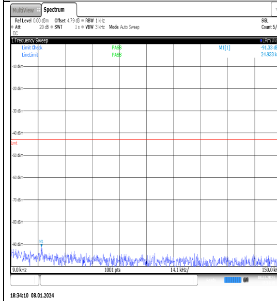
NTNV_N77-3700- 3980_PC2_30_30_M_TID5_NS_01_0.009_0.15_# 1
