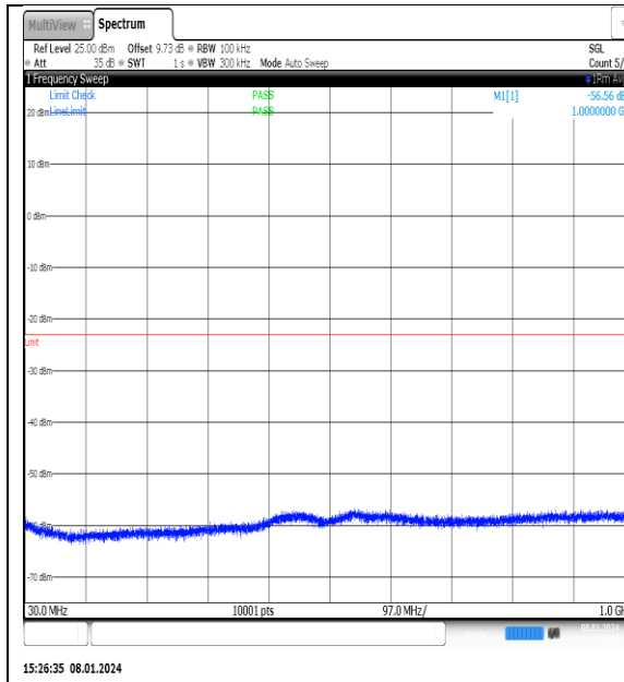
NTNV_N77-3700- 3980_PC2_30_25_H_TID13_NS_01_30_1000_#1
