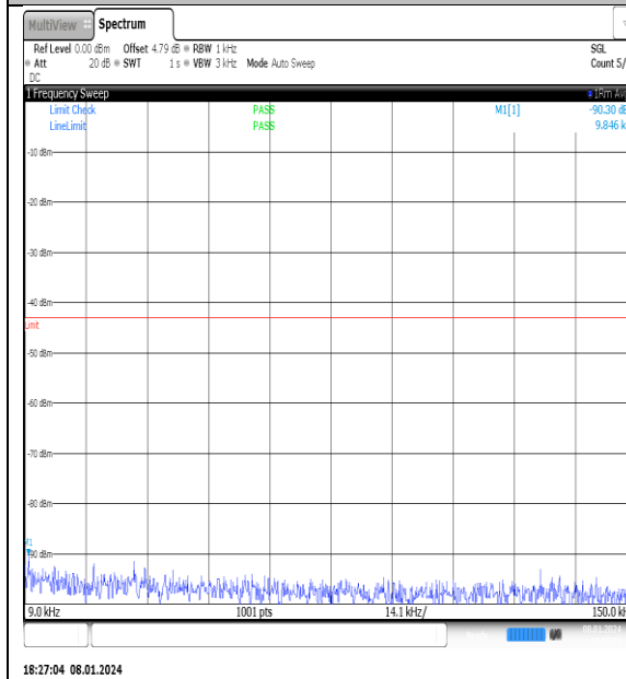
NTNV_N77-3700- 3980_PC2_30_30_M_TID3_NS_01_0.009_0.15_# 1
