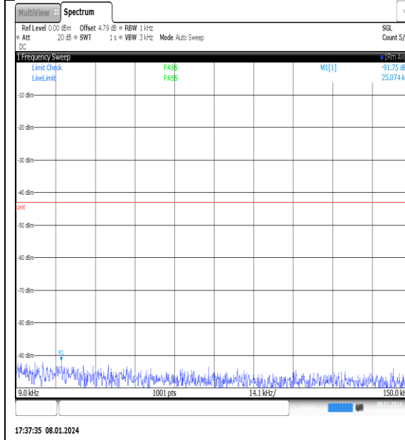
NTNV_N77-3700- 3980_PC2_30_30_L_TID2_NS_01_0.009_0.15_# 1
