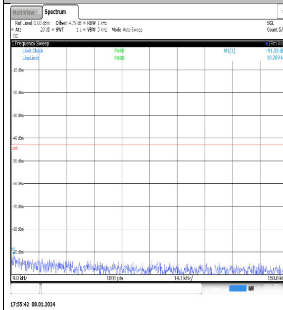
NTNV_N77-3700- 3980_PC2_30_30_L_TID8_NS_01_0.009_0.15_# 1
