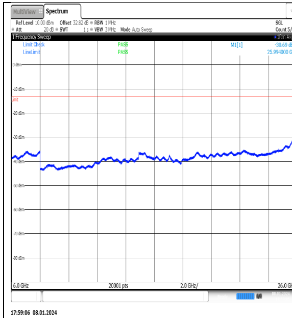
NTNV_N77-3700- 3980_PC2_30_30_L_TID9_NS_01_6000_26000_ #1
