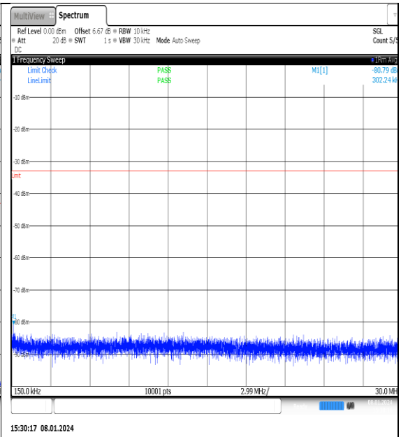
NTNV_N77-3700- 3980_PC2_30_25_H_TID14_NS_01_0.15_30_#1
