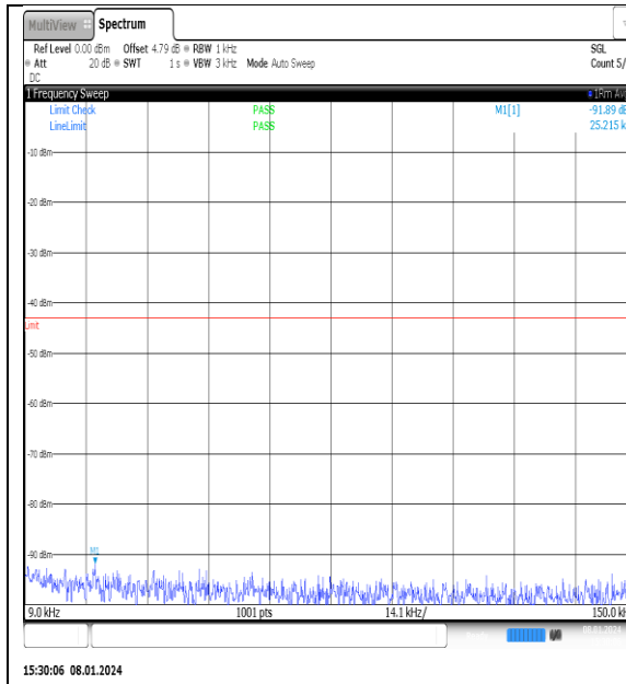
NTNV_N77-3700- 3980_PC2_30_25_H_TID14_NS_01_0.009_0.15_ #1
