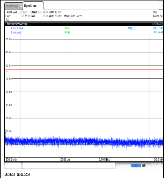
NTNV_N77-3700- 3980_PC2_30_25_H_TID13_NS_01_0.15_30_#1
