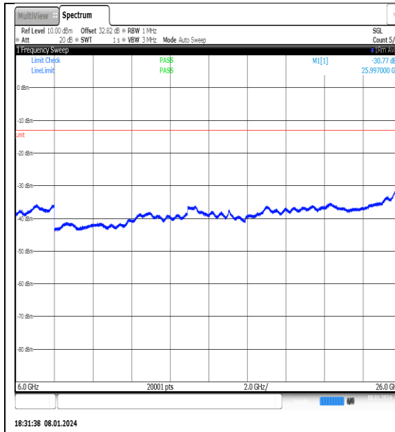
NTNV_N77-3700- 3980_PC2_30_30_M_TID4_NS_01_6000_26000_ #1
