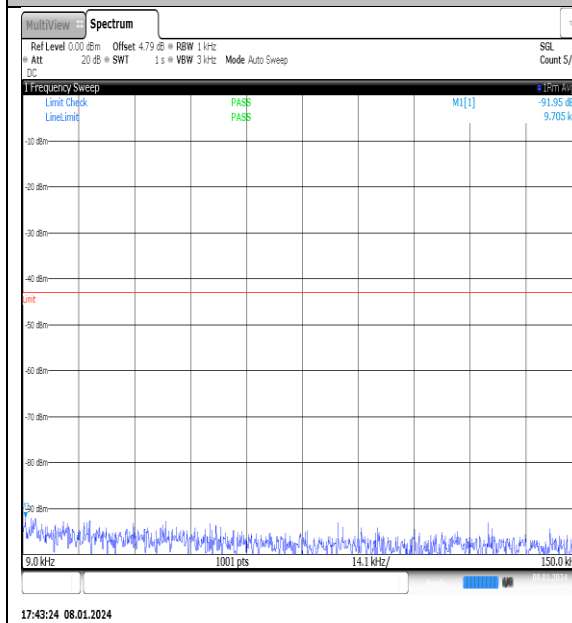
NTNV_N77-3700- 3980_PC2_30_30_L_TID4_NS_01_0.009_0.15_# 1
