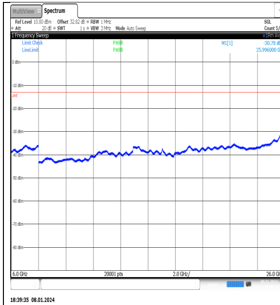
NTNV_N77-3700- 3980_PC2_30_30_M_TID6_NS_01_6000_26000_#1
