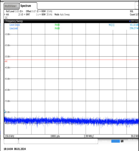
NTNV_N77-3700- 3980_PC2_30_30_L_TID14_NS_01_0.15_30_#1
