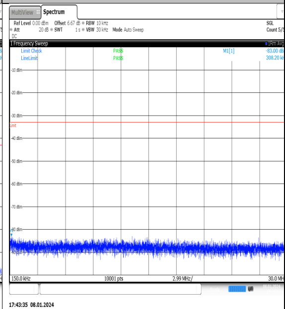
NTNV_N77-3700- 3980_PC2_30_30_L_TID4_NS_01_0.15_30_#1
