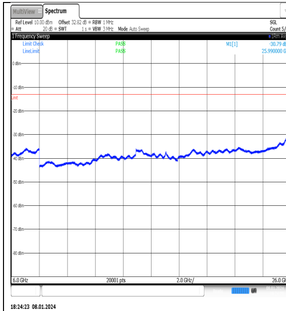
NTNV_N77-3700- 3980_PC2_30_30_M_TID2_NS_01_6000_26000_ #1
