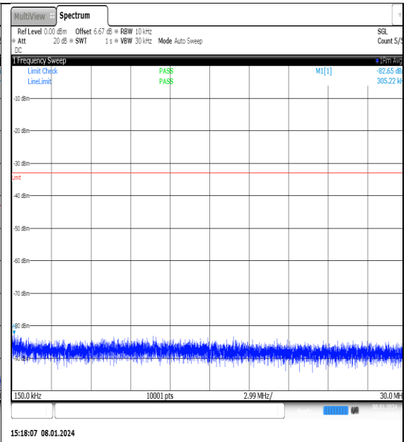
NTNV_N77-3700- 3980_PC2_30_25_H_TID12_NS_01_0.15_30_#1
