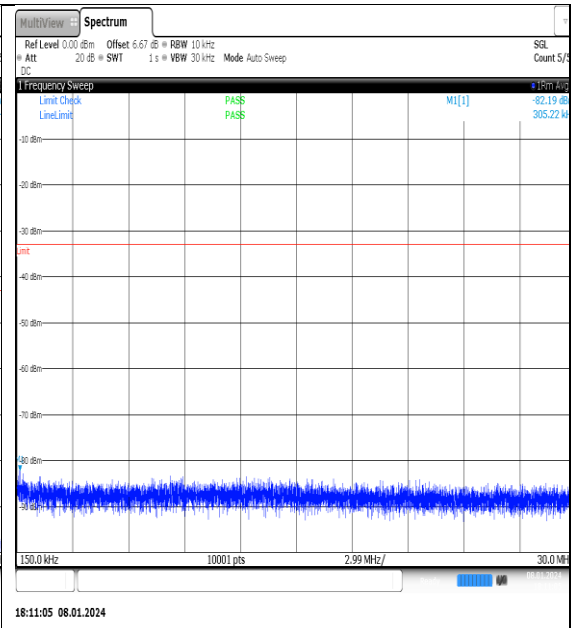
NTN_V_N77-3700- 3980_PC2_30_30_L_TID13_NS_01_0.15_30_#1
