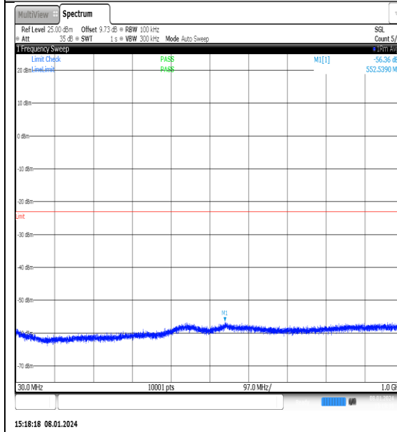
NTNV_N77-3700- 3980_PC2_30_25_H_TID12_NS_01_30_1000_#1
