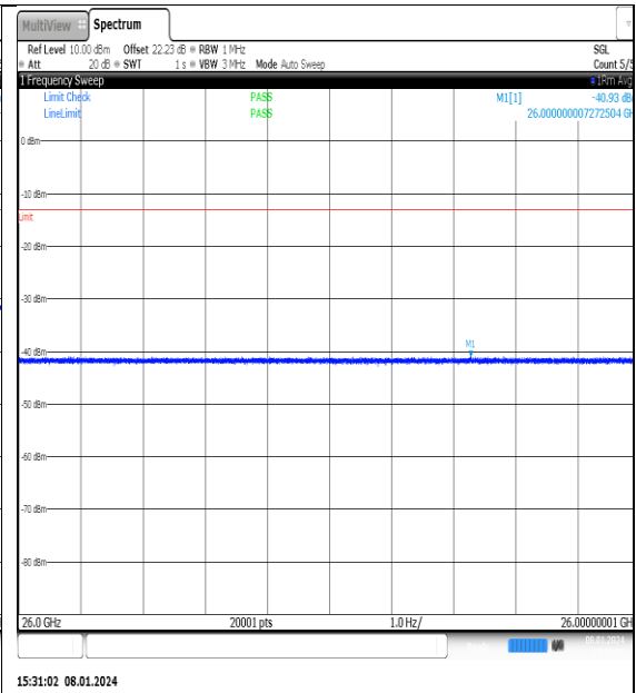
NTNV_N77-3700- 3980_PC2_30_25_H_TID14_NS_01_26000_4000 0_#1
