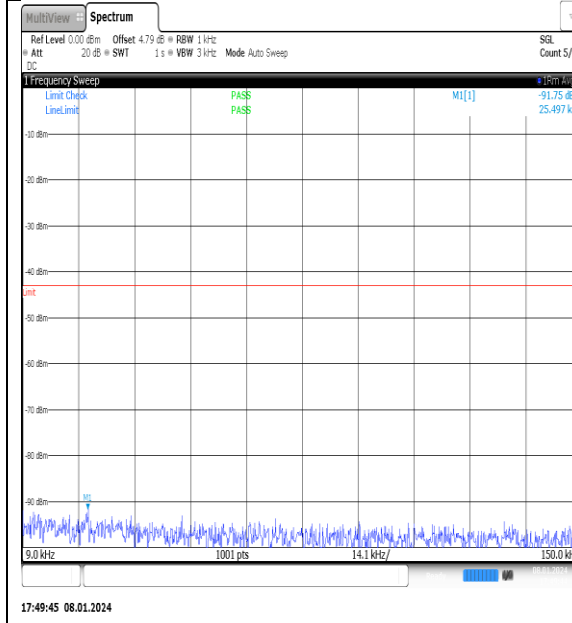
NTNV_N77-3700- 3980_PC2_30_30_L_TID6_NS_01_0.009_0.15_# 1
