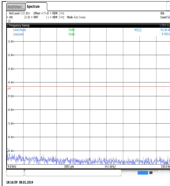
NTN_V_N77-3700- 3980_PC2_30_30_L_TID15_NS_01_0.009_0.15_ #1
