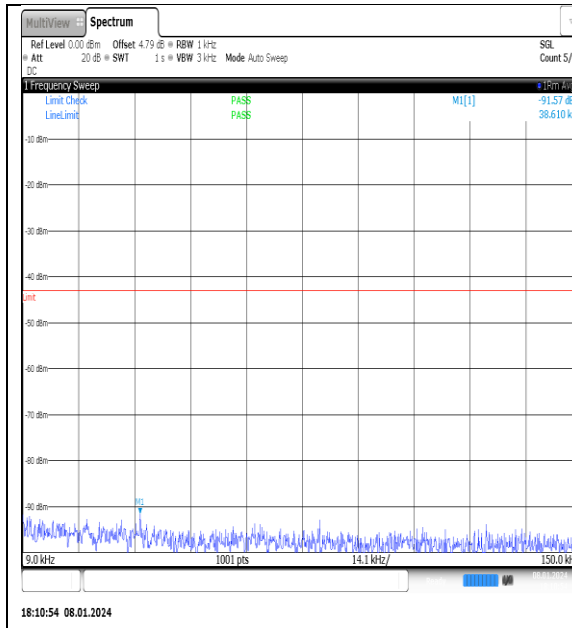
NTN_V_N77-3700- 3980_PC2_30_30_L_TID13_NS_01_0.009_0.15_ #1
