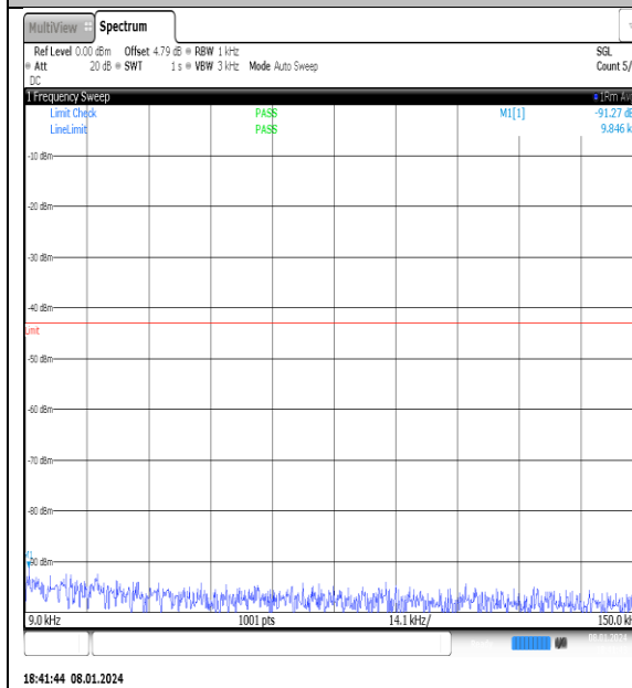
NTNV_N77-3700- 3980_PC2_30_30_M_TID7_NS_01_0.009_0.15_#1
