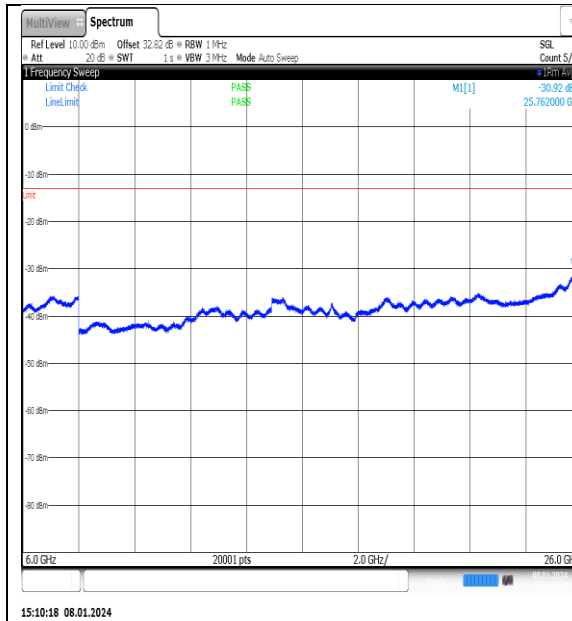
NTNV_N77-3700- 3980_PC2_30_25_H_TID10_NS_01_6000_26000 _#1
