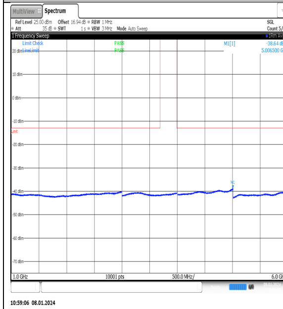
NTNV_N77-3700- 3980_PC2_30_25_M_TID2_NS_01_1000_6000_#1
