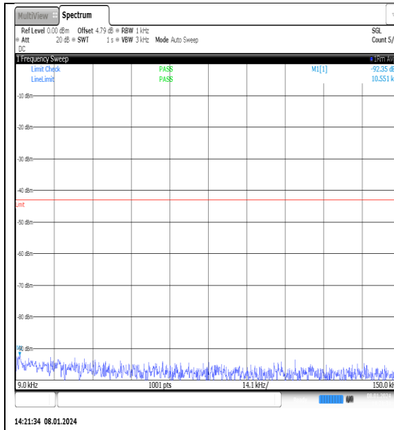
NTNV_N77-3700- 3980_PC2_30_25_M_TID15_NS_01_0.009_0.15_ #1
