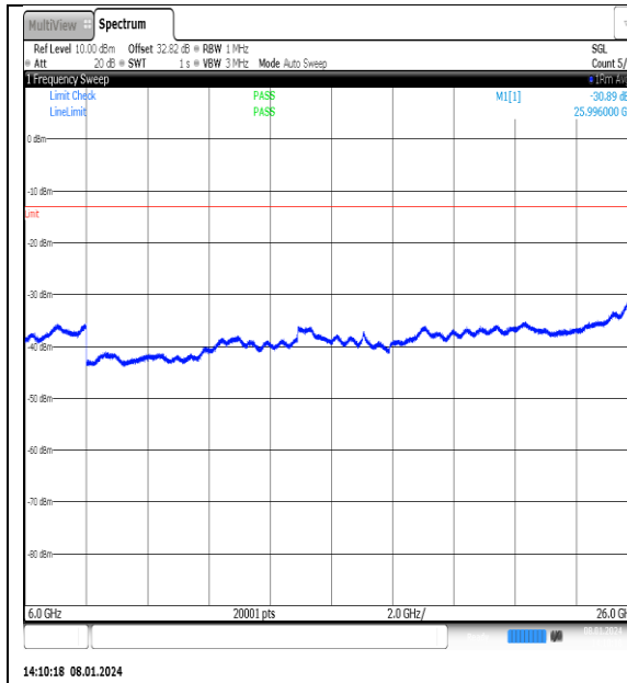
NTNV_N77-3700- 3980_PC2_30_25_M_TID11_NS_01_6000_26000 _#1
