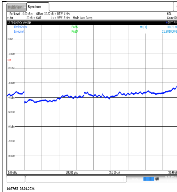
NTNV_N77-3700- 3980_PC2_30_25_H_TID4_NS_01_6000_26000_#1
