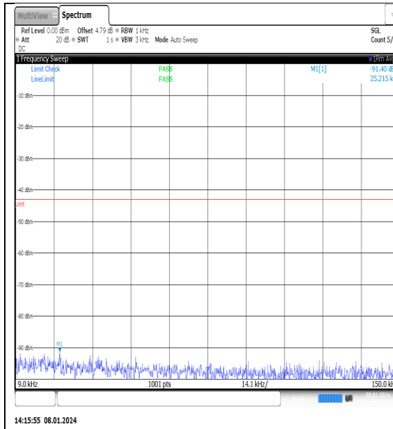
NTN_V_N77-3700- 3980_PC2_30_25_M_TID13_NS_01_0.009_0.15_ #1
