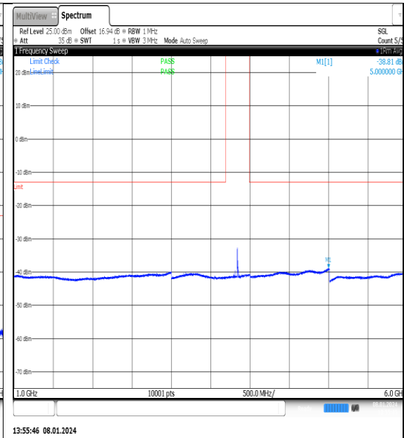
NTNV_N77-3700- 3980_PC2_30_25_M_TID8_NS_01_1000_6000_#1
