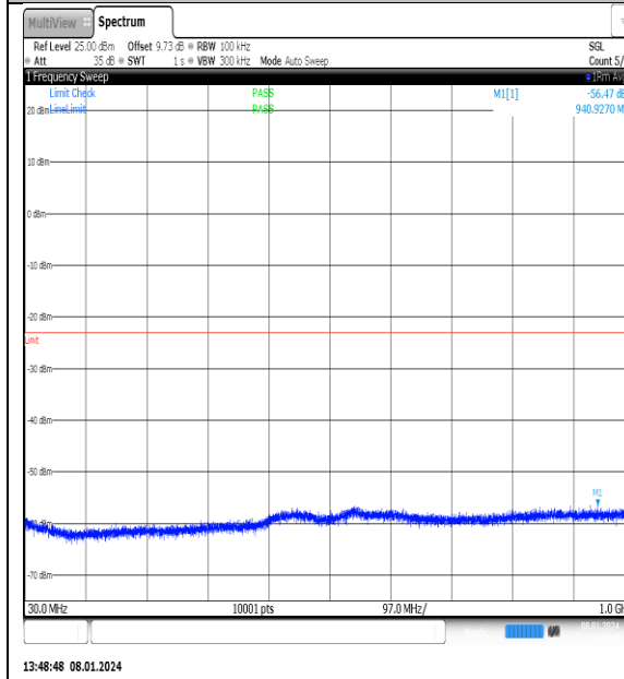
NTNV_N77-3700- 3980_PC2_30_25_M_TID6_NS_01_26000_40000 _#1
