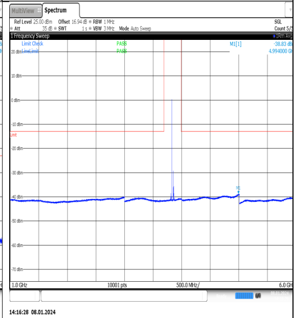
NTN_V_N77-3700- 3980_PC2_30_25_M_TID13_NS_01_1000_6000_ #1
