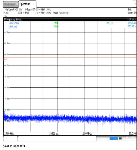
NTNV_N77-3700- 3980_PC2_30_25_H_TID7_NS_01_0.15_30_#1
