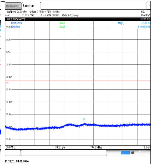
NTNV_N77-3700-3980_PC2_30_25_M_TID6_NS_01_30_1000_#1
