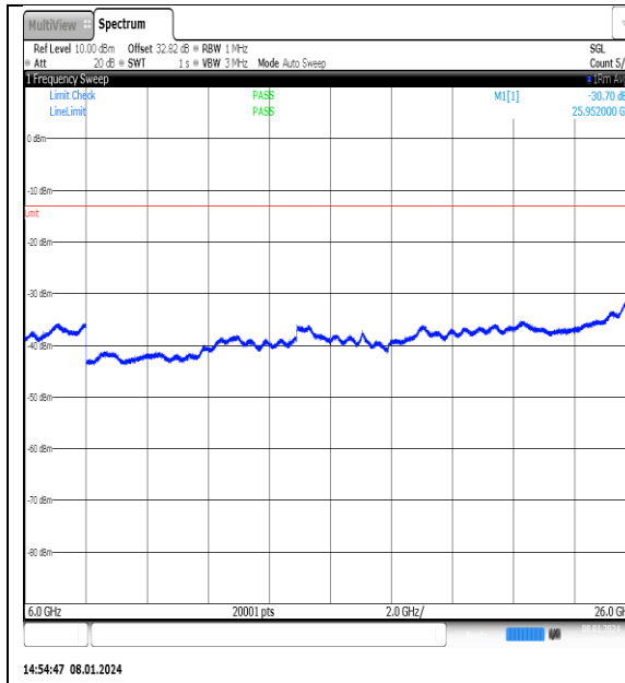
NTNV_N77-3700- 3980_PC2_30_25_H_TID8_NS_01_6000_26000_#1
