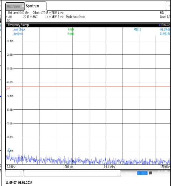
NTN_V_N77-3700- 3980_PC2_30_25_M_TID4_NS_01_0.009_0.15_# 1
