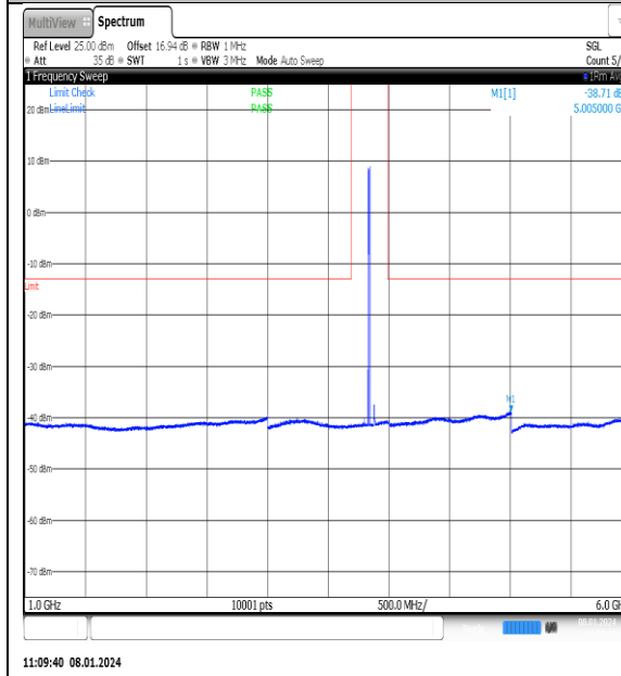
NTNV_N77-3700- 3980_PC2_30_25_M_TID4_NS_01_1000_6000_#1
