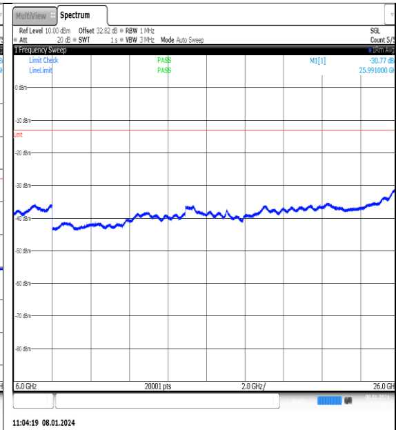
NTN_V_N77-3700- 3980_PC2_30_25_M_TID3_NS_01_6000_26000_# #1
