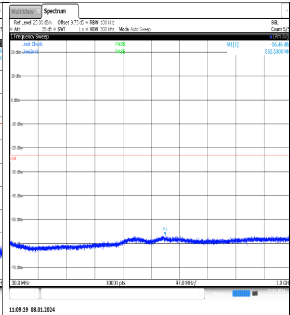
NTNV_N77-3700- 3980_PC2_30_25_M_TID4_NS_01_30_1000_#1
