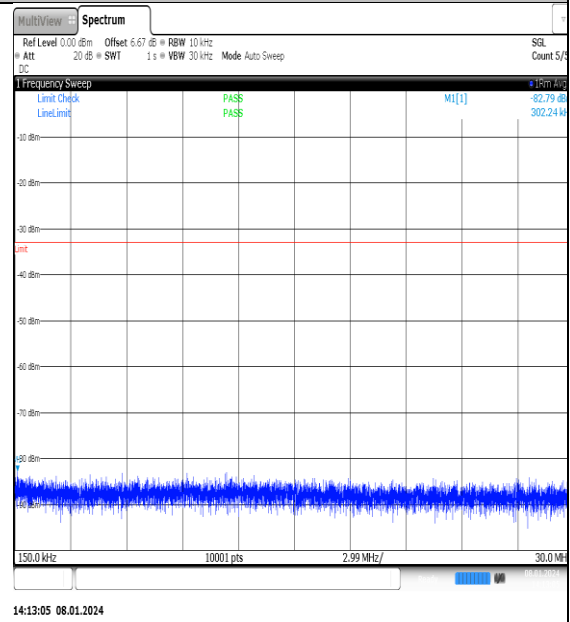
NTNV_N77-3700- 3980_PC2_30_25_M_TID12_NS_01_0.15_30_#1
