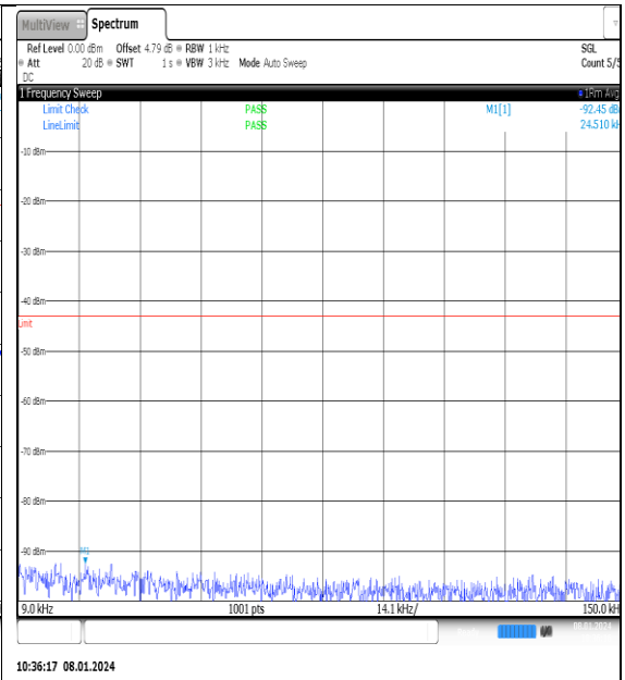
NTNV_N77-3700- 3980_PC2_30_25_L_TID14_NS_01_0.009_0.15_#1
