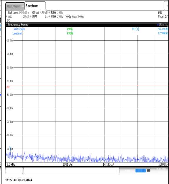
NTNV_N77-3700- 3980_PC2_30_25_M_TID6_NS_01_0.009_0.15_# 1
