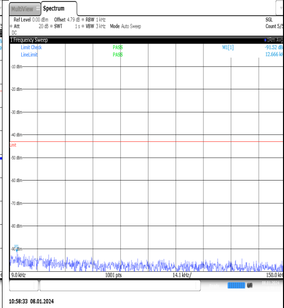
NTN_V_N77-3700- 3980_PC2_30_25_M_TID2_NS_01_0.009_0.15_# 1
