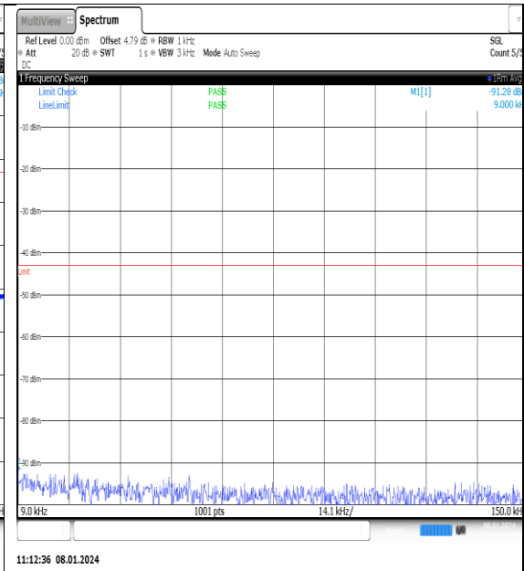
NTNV_N77-3700- 3980_PC2_30_25_M_TID5_NS_01_0.009_0.15_# 1
