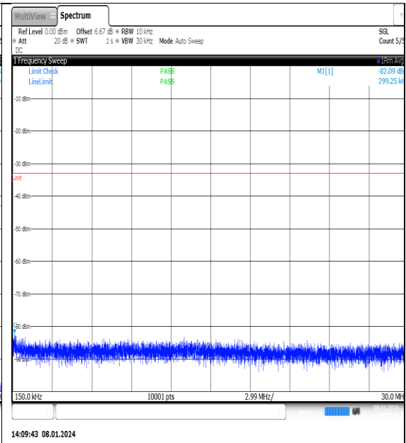
NTNV_N77-3700- 3980_PC2_30_25_M_TID11_NS_01_0.15_30_#1
