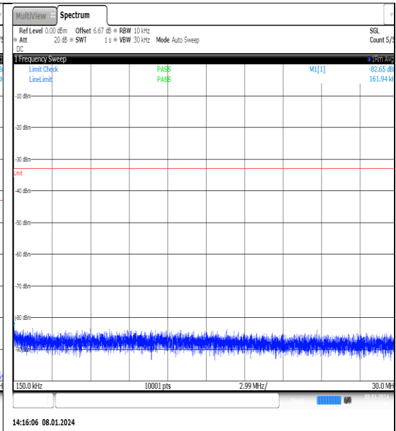
NTN_V_N77-3700- 3980_PC2_30_25_M_TID13_NS_01_0.15_30_#1
