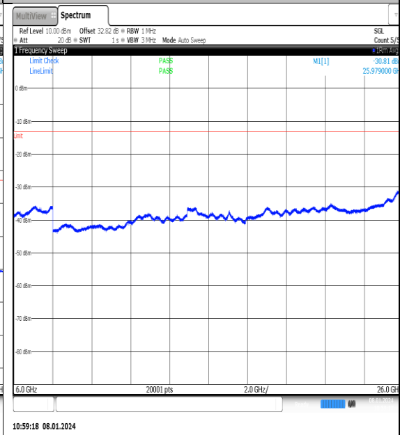
NTNV_N77-3700- 3980_PC2_30_25_M_TID2_NS_01_6000_26000_#1
