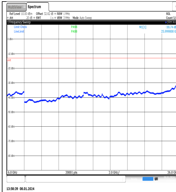
NTNV_N77-3700- 3980_PC2_30_25_M_TID9_NS_01_6000_26000_#1
