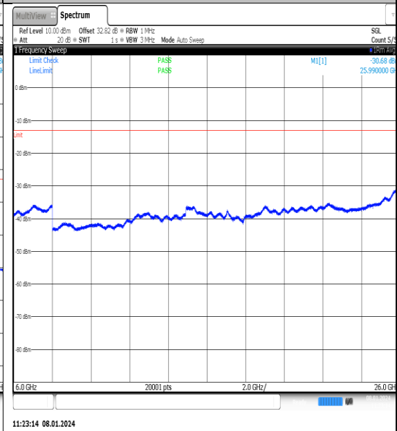
NTNV_N77-3700-3980_PC2_30_25_M_TID6_NS_01_6000_26000_#1
