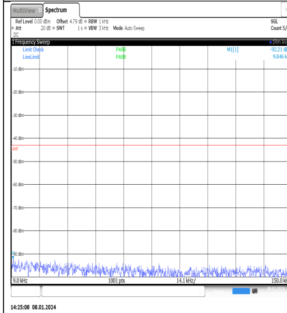
NTNV_N77-3700- 3980_PC2_30_25_H_TID1_NS_01_0.009_0.15_# 1
