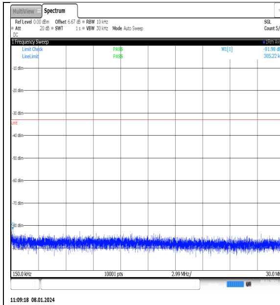
NTNV_N77-3700- 3980_PC2_30_25_M_TID4_NS_01_0.15_30_#1
