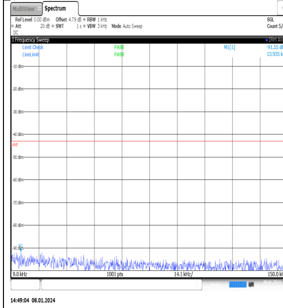
NTNV_N77-3700- 3980_PC2_30_25_H_TID7_NS_01_0.009_0.15_#1
