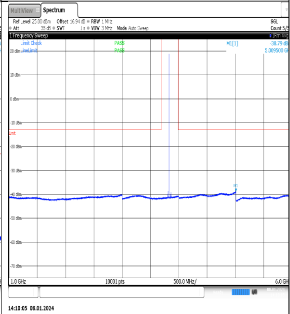
NTNV_N77-3700- 3980_PC2_30_25_M_TID11_NS_01_1000_6000_ #1
