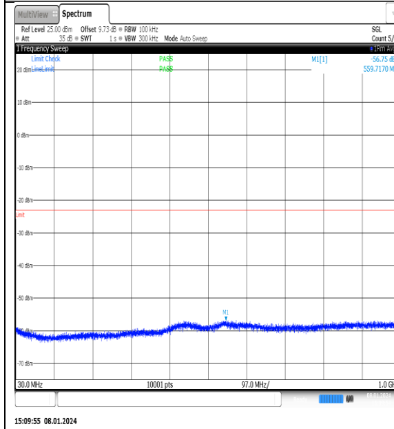
NTN_V_N77-3700- 3980_PC2_30_25_H_TID10_NS_01_30_1000_#1
