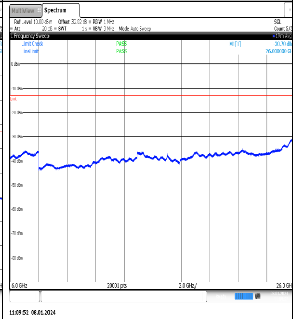
NTNV_N77-3700- 3980_PC2_30_25_M_TID4_NS_01_6000_26000_#1
