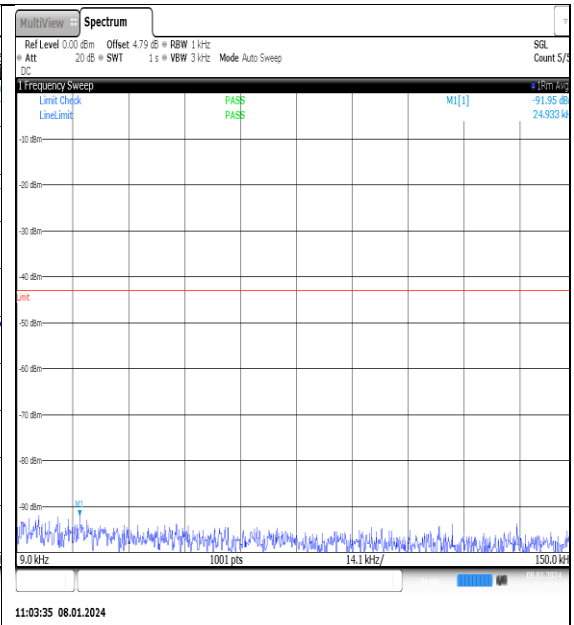
NTNV_N77-3700- 3980_PC2_30_25_M_TID3_NS_01_0.009_0.15_# 1
