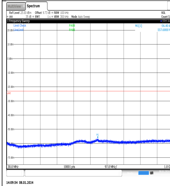
NTNV_N77-3700- 3980_PC2_30_25_M_TID11_NS_01_30_1000_#1
