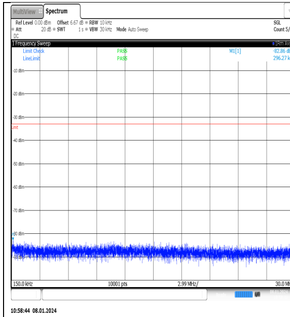
NTNV_N77-3700- 3980_PC2_30_25_M_TID2_NS_01_0.15_30_#1
