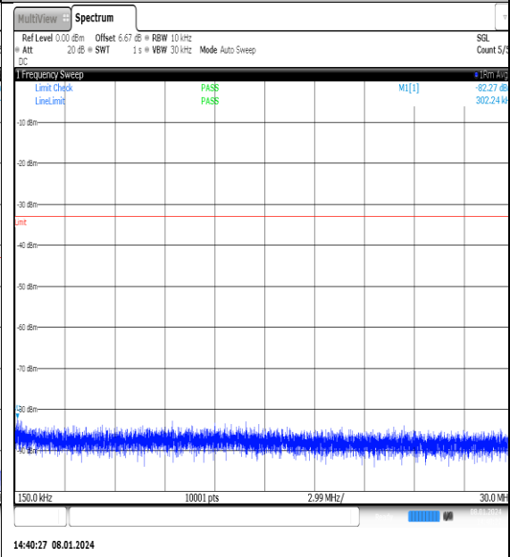
NTNV_N77-3700- 3980_PC2_30_25_H_TID5_NS_01_0.15_30_#1
