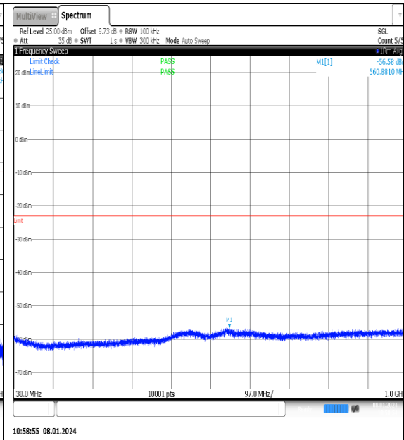
NTNV_N77-3700- 3980_PC2_30_25_M_TID2_NS_01_30_1000_#1
