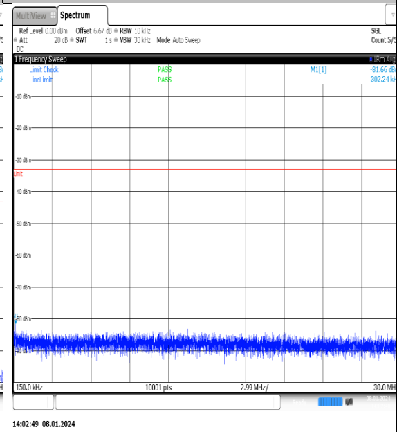
NTNV_N77-3700- 3980_PC2_30_25_M_TID10_NS_01_0.15_30_#1
