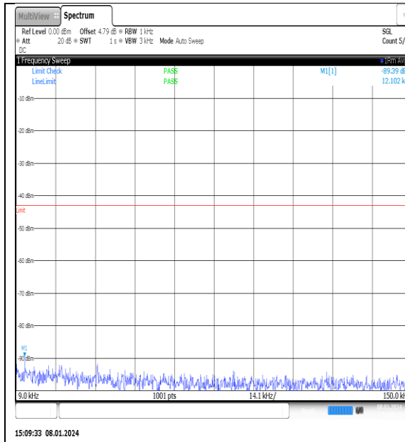
NTN_V_N77-3700- 3980_PC2_30_25_H_TID10_NS_01_0.009_0.15_ #1
