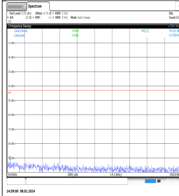
NTNV_N77-3700- 3980_PC2_30_25_H_TID9_NS_01_0.009_0.15_#1
