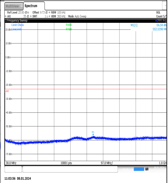
NTNV_N77-3700- 3980_PC2_30_25_M_TID3_NS_01_30_1000_#1
