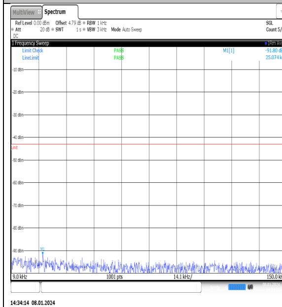
NTNV_N77-3700- 3980_PC2_30_25_H_TID3_NS_01_0.009_0.15_#1
