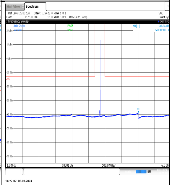
NTNV_N77-3700- 3980_PC2_30_25_M_TID15_NS_01_1000_6000_ #1
