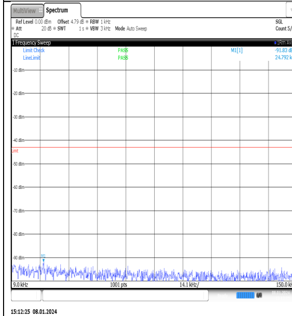
NTNV_N77-3700- 3980_PC2_30_25_H_TID11_NS_01_0.009_0.15_#1
