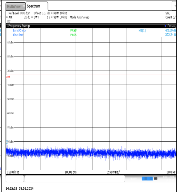
NTNV_N77-3700- 3980_PC2_30_25_H_TID1_NS_01_0.15_30_#1
