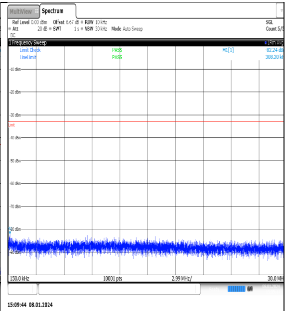
NTN_V_N77-3700- 3980_PC2_30_25_H_TID10_NS_01_0.15_30_#1
