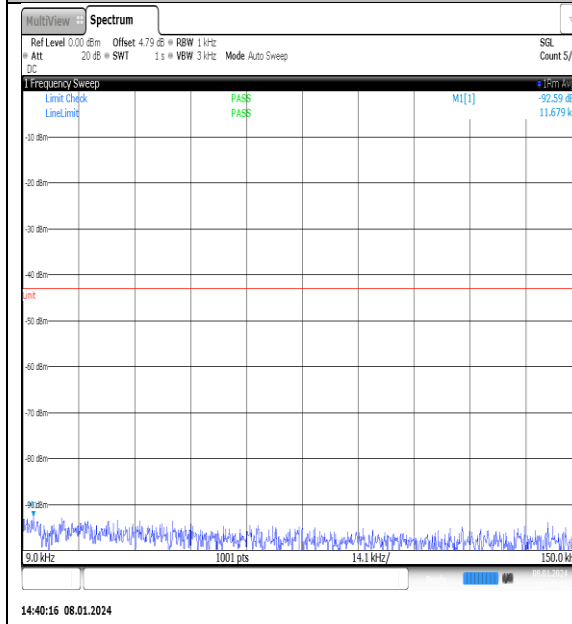
NTNV_N77-3700- 3980_PC2_30_25_H_TID5_NS_01_0.009_0.15_#1
