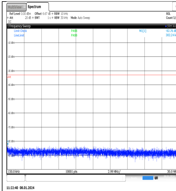
NTNV_N77-3700-3980_PC2_30_25_M_TID6_NS_01_0.15_30_#1
