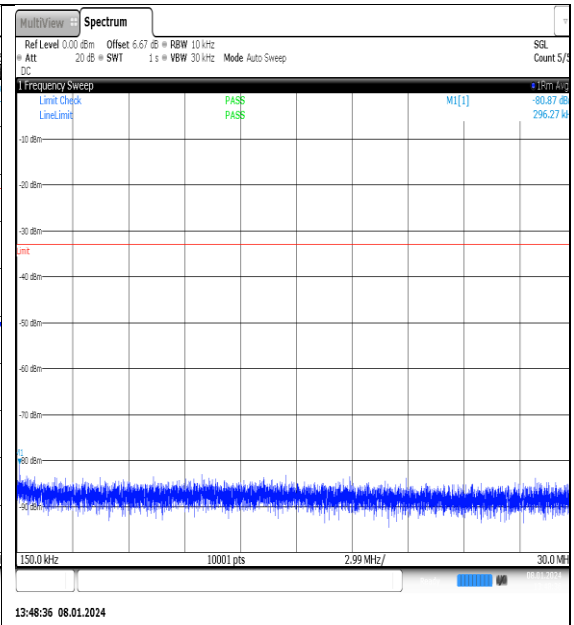
NTNV_N77-3700- 3980_PC2_30_25_M_TID7_NS_01_0.15_30_#1
