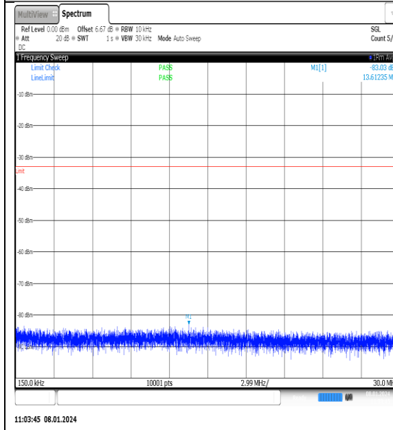
NTNV_N77-3700- 3980_PC2_30_25_M_TID3_NS_01_0.15_30_#1
