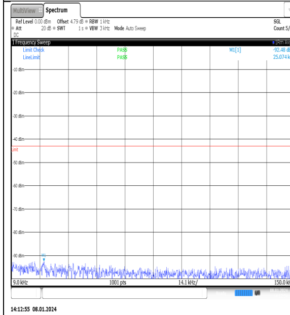
NTNV_N77-3700- 3980_PC2_30_25_M_TID12_NS_01_0.009_0.15_#1
