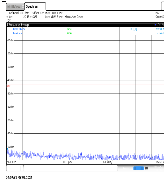
NTNV_N77-3700- 3980_PC2_30_25_M_TID11_NS_01_0.009_0.15_ #1
