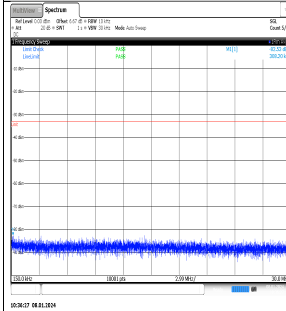
NTNV_N77-3700- 3980_PC2_30_25_L_TID14_NS_01_0.15_30_#1
