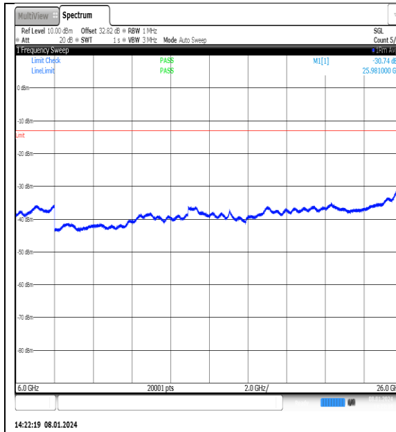
NTNV_N77-3700- 3980_PC2_30_25_M_TID15_NS_01_6000_26000 _#1
