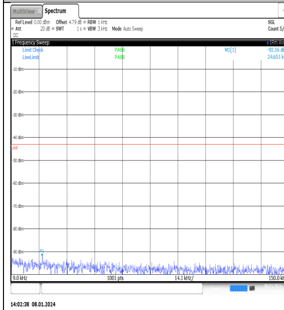
NTNV_N77-3700- 3980_PC2_30_25_M_TID10_NS_01_0.009_0.15_#1
