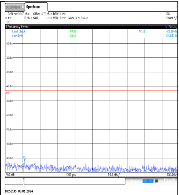
NTNV_N77-3700- 3980_PC2_30_25_M_TID1_NS_01_0.009_0.15_# 1
