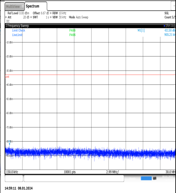
NTNV_N77-3700- 3980_PC2_30_25_H_TID9_NS_01_0.15_30_#1
