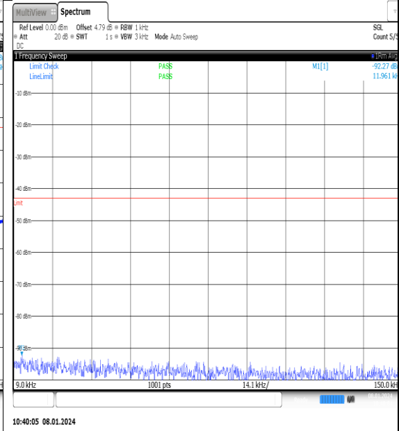
NTN_V_N77-3700- 3980_PC2_30_25_L_TID15_NS_01_0.009_0.15_ #1
