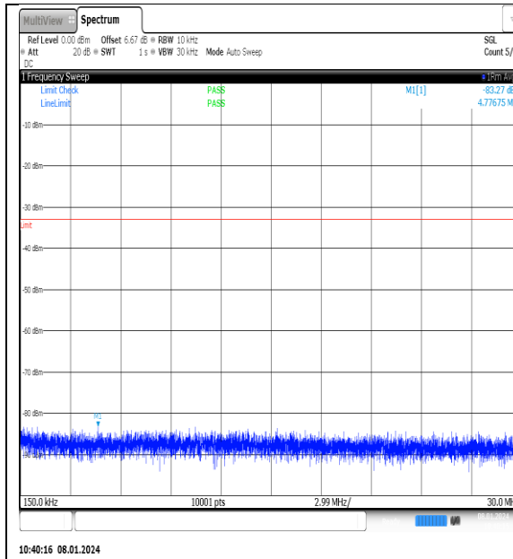
NTNV_N77-3700- 3980_PC2_30_25_L_TID15_NS_01_0.15_30_#1
