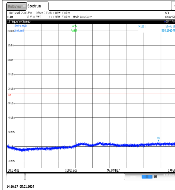
NTN_V_N77-3700- 3980_PC2_30_25_M_TID13_NS_01_30_1000_#1
