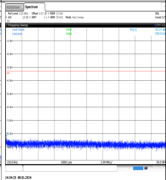
NTNV_N77-3700- 3980_PC2_30_25_H_TID3_NS_01_0.15_30_#1
