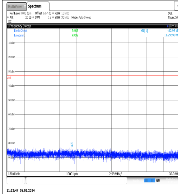
NTNV_N77-3700- 3980_PC2_30_25_M_TID5_NS_01_0.15_30_#1
