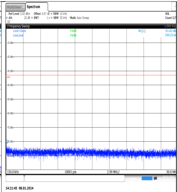
NTNV_N77-3700- 3980_PC2_30_25_M_TID15_NS_01_0.15_30_#1
