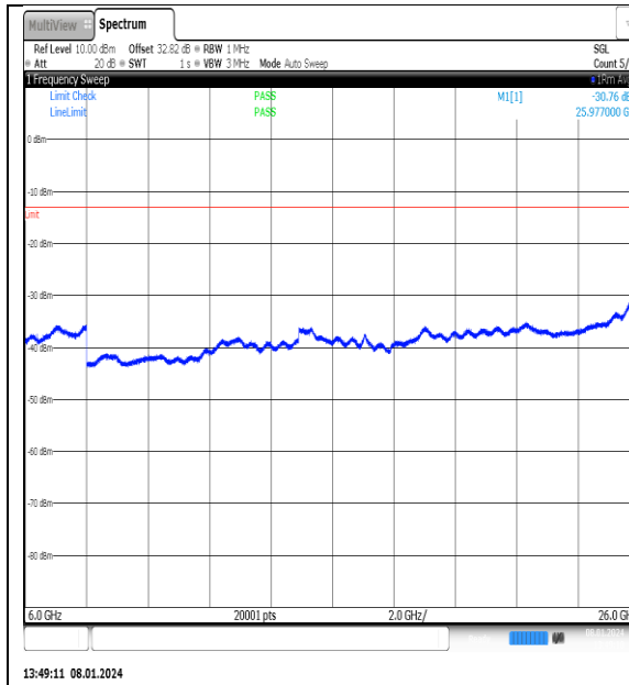
NTNV_N77-3700- 3980_PC2_30_25_M_TID7_NS_01_6000_26000_#1
