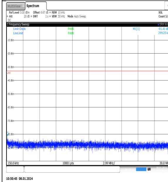
NTNV_N77-3700- 3980_PC2_30_25_M_TID1_NS_01_0.15_30_#1
