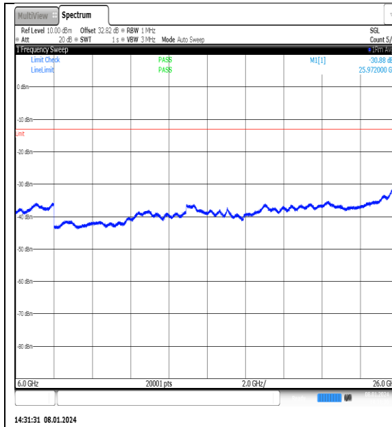
NTNV_N77-3700- 3980_PC2_30_25_H_TID2_NS_01_6000_26000_#1
