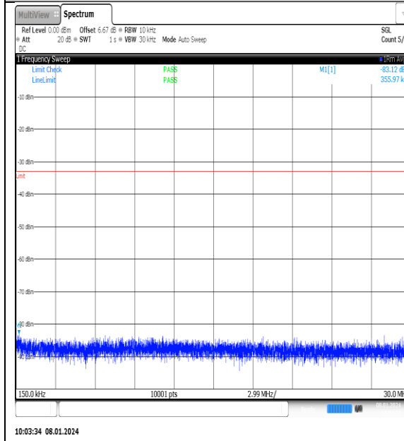
NTNV_N77-3700- 3980_PC2_30_25_L_TID6_NS_01_0.15_30_#1
