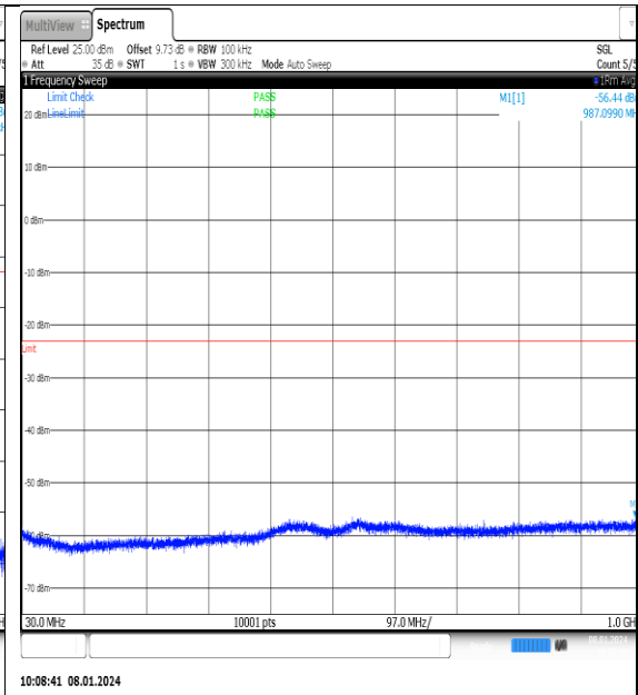
NTNV_N77-3700- 3980_PC2_30_25_L_TID7_NS_01_30_1000_#1
