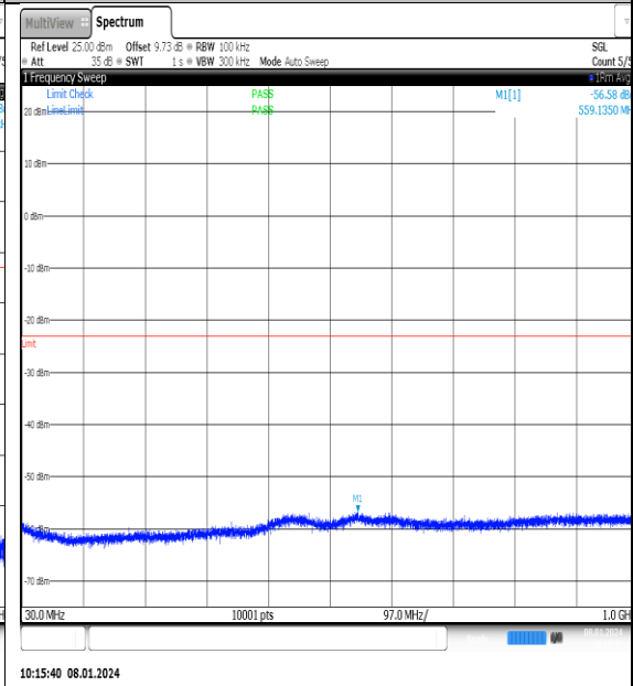
NTNV_N77-3700- 3980_PC2_30_25_L_TID8_NS_01_30_1000_#1
