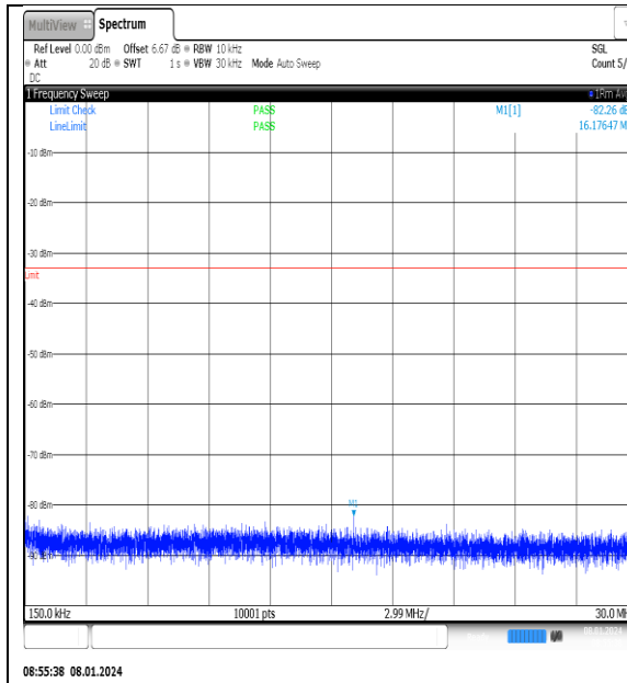
NTNV_N77-3700- 3980_PC2_30_20_H_TID2_NS_01_0.15_30_#1
