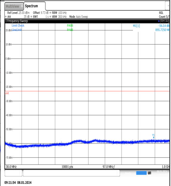
NTNV_N77-3700- 3980_PC2_30_20_H_TID11_NS_01_30_1000_#1
