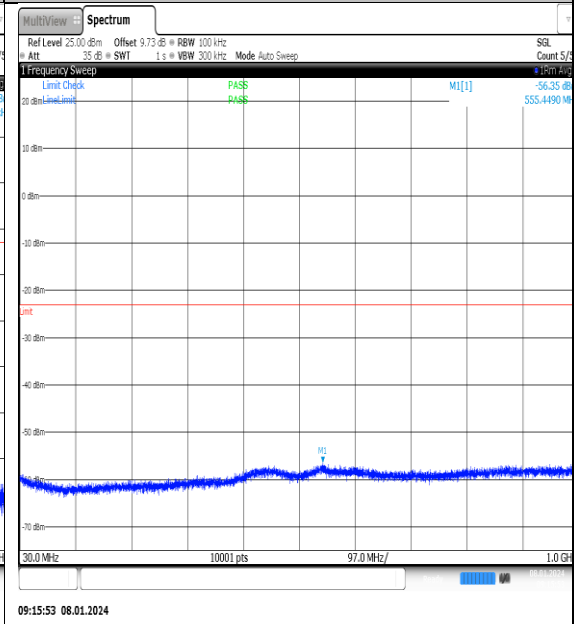
NTNV_N77-3700- 3980_PC2_30_20_H_TID9_NS_01_30_1000_#1
