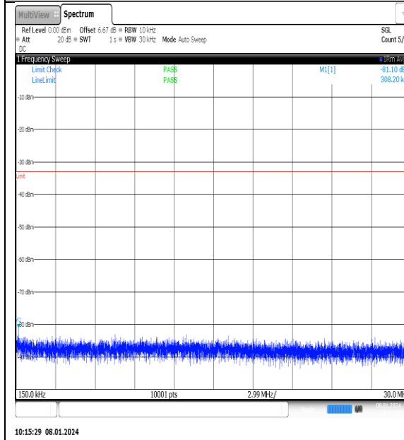
NTNV_N77-3700- 3980_PC2_30_25_L_TID8_NS_01_0.15_30_#1
