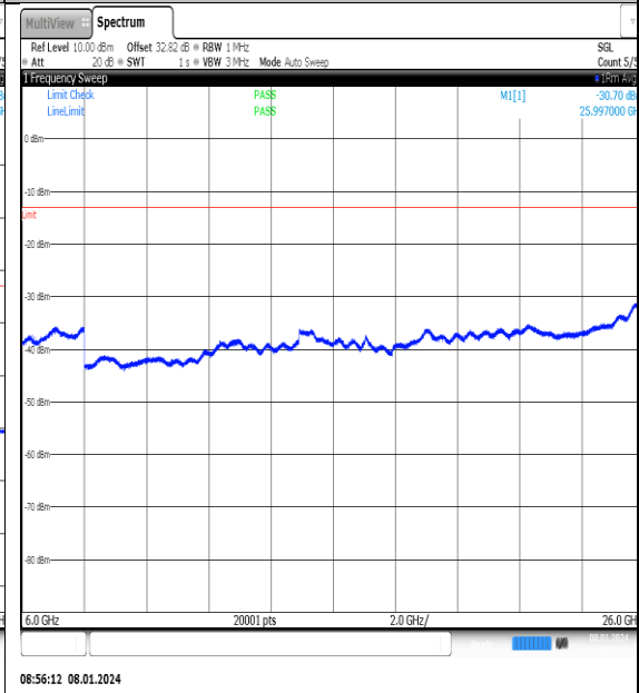
NTNV_N77-3700- 3980_PC2_30_20_H_TID2_NS_01_6000_26000_#1
