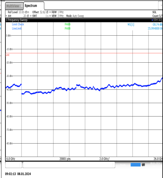
NTNV_N77-3700- 3980_PC2_30_20_H_TID4_NS_01_6000_26000_#1
