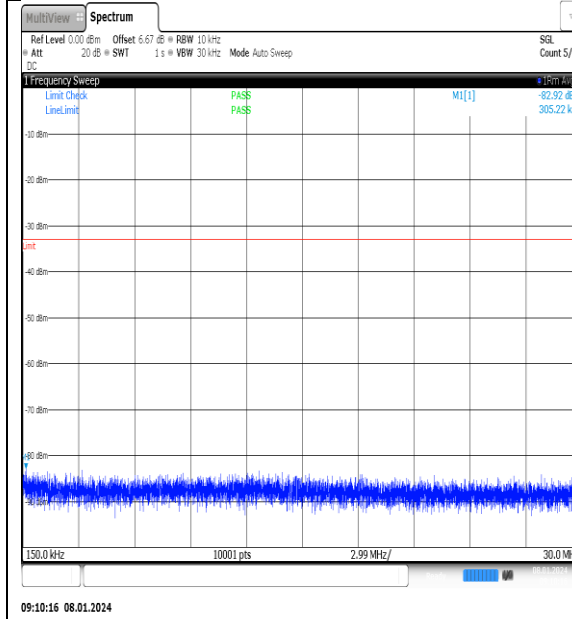
NTNV_N77-3700- 3980_PC2_30_20_H_TID7_NS_01_0.15_30_#1
