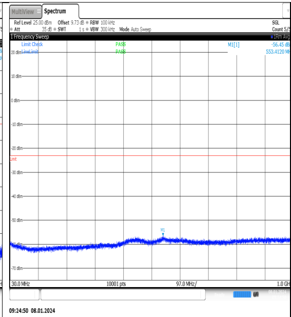
NTNV_N77-3700- 3980_PC2_30_20_H_TID12_NS_01_30_1000_#1
