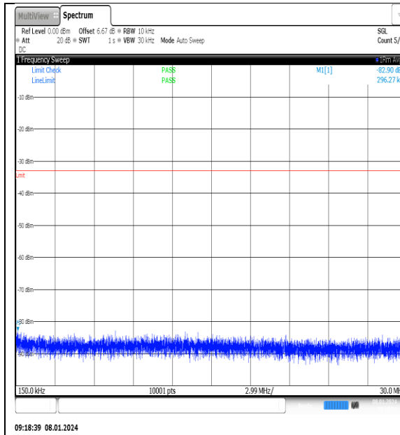
NTN_V_N77-3700- 3980_PC2_30_20_H_TID10_NS_01_0.15_30_#1
