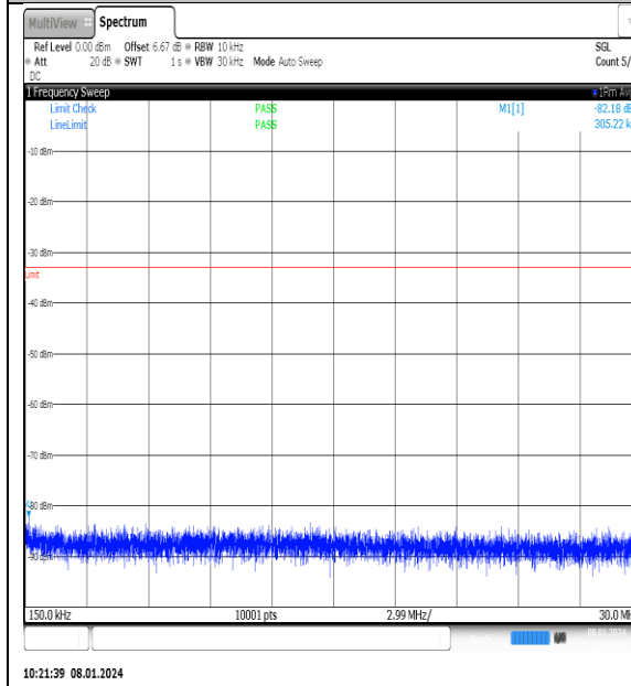
NTNV_N77-3700- 3980_PC2_30_25_L_TID10_NS_01_0.15_30_#1
