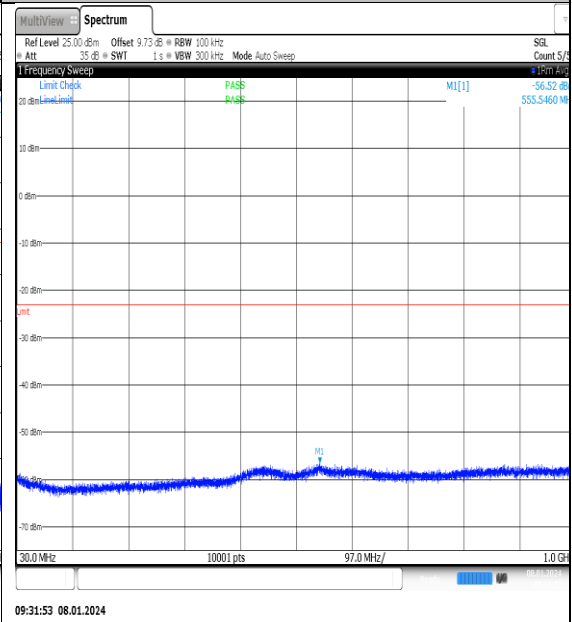
NTNV_N77-3700- 3980_PC2_30_20_H_TID13_NS_01_30_1000_#1
