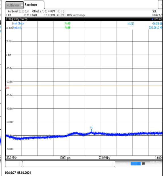
NTNV_N77-3700- 3980_PC2_30_20_H_TID7_NS_01_30_1000_#1
