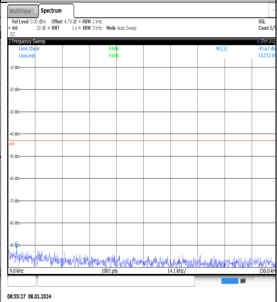
NTN_V_N77-3700- 3980_PC2_30_20_H_TID2_NS_01_0.009_0.15_# 1
