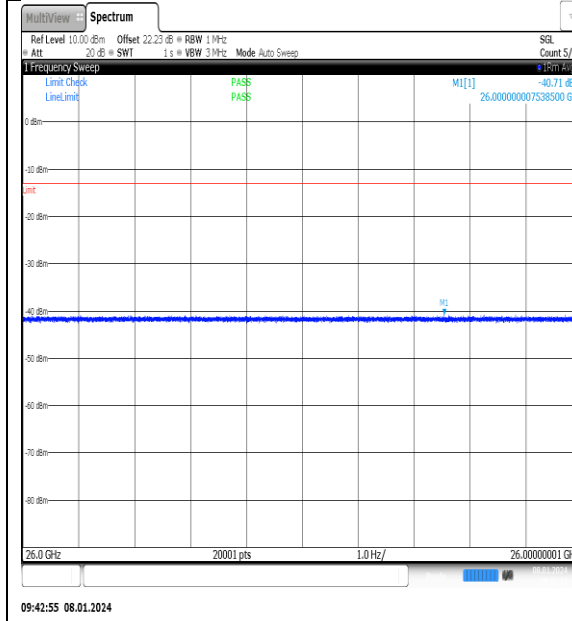
NTNV_N77-3700- 3980_PC2_30_20_H_TID15_NS_01_26000_4000_0_#1
