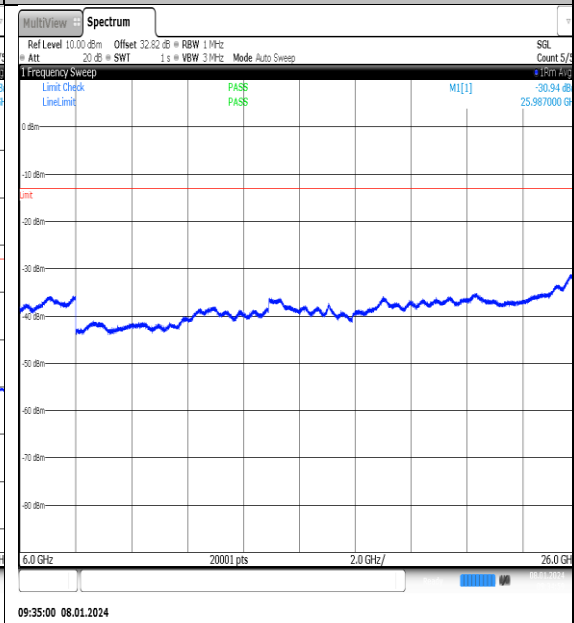
NTNV_N77-3700-3980_PC2_30_20_H_TID14_NS_01_6000_26000_#1
