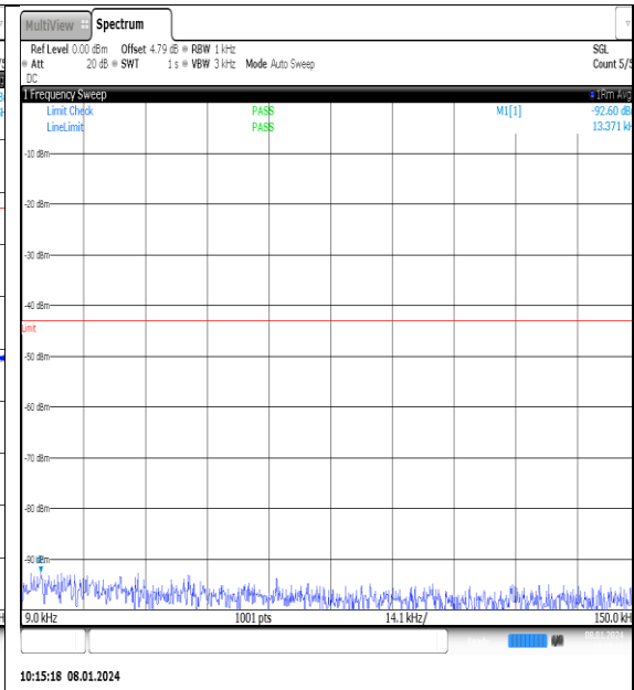
NTNV_N77-3700- 3980_PC2_30_25_L_TID8_NS_01_0.009_0.15_# 1
