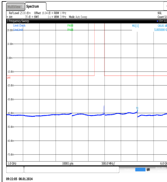
NTN_V_N77-3700- 3980_PC2_30_20_H_TID11_NS_01_1000_6000_#1
