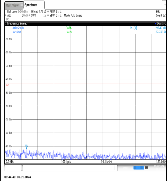
NTNV_N77-3700- 3980_PC2_30_25_L_TID1_NS_01_0.009_0.15_#1
