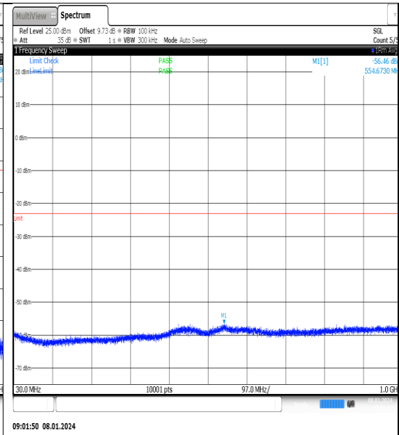
NTNV_N77-3700- 3980_PC2_30_20_H_TID4_NS_01_30_1000_#1
