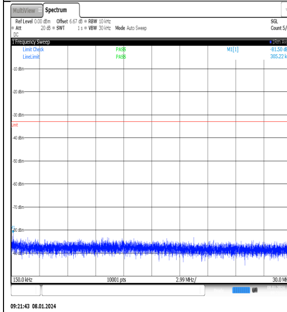
NTNV_N77-3700- 3980_PC2_30_20_H_TID11_NS_01_0.15_30_#1
