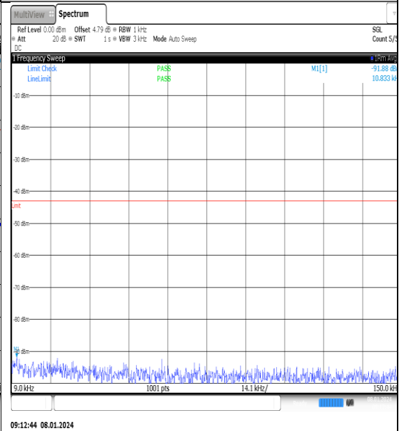
NTN_V_N77-3700- 3980_PC2_30_20_H_TID8_NS_01_0.009_0.15_# 1
