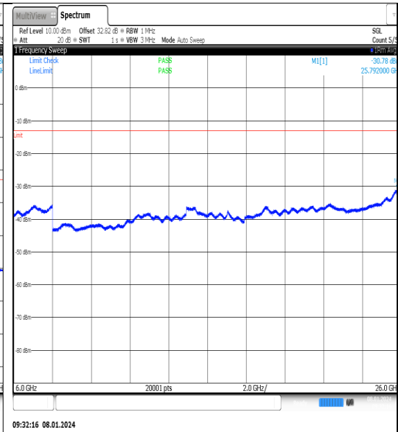
NTN_V_N77-3700- 3980_PC2_30_20_H_TID13_NS_01_6000_26000 #1
