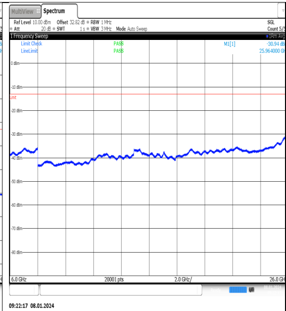
NTN_V_N77-3700- 3980_PC2_30_20_H_TID11_NS_01_6000_26000_#1
