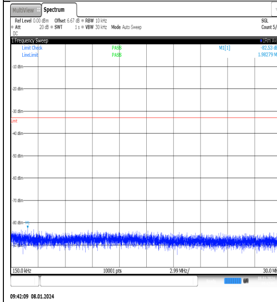
NTNV_N77-3700- 3980_PC2_30_20_H_TID15_NS_01_0.15_30_#1
