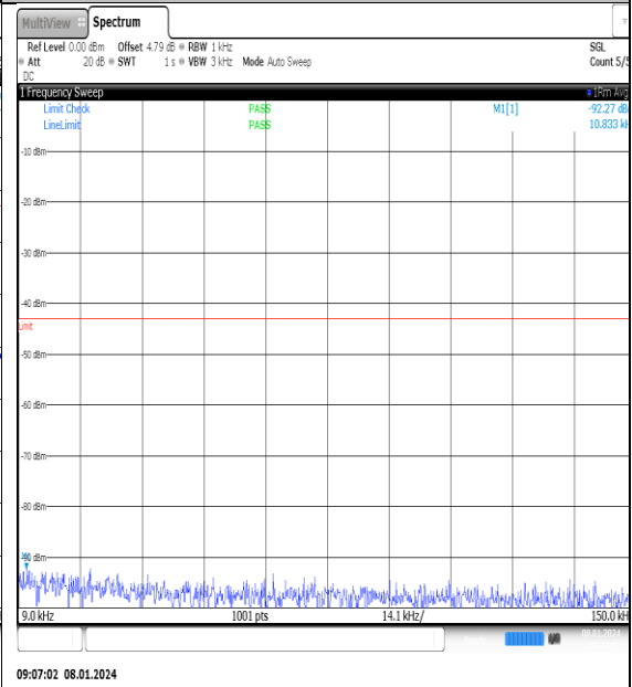
NTNV_N77-3700- 3980_PC2_30_20_H_TID6_NS_01_0.009_0.15_# 1
