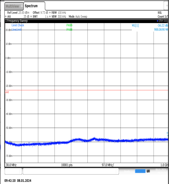
NTNV_N77-3700- 3980_PC2_30_20_H_TID15_NS_01_30_1000_#1
