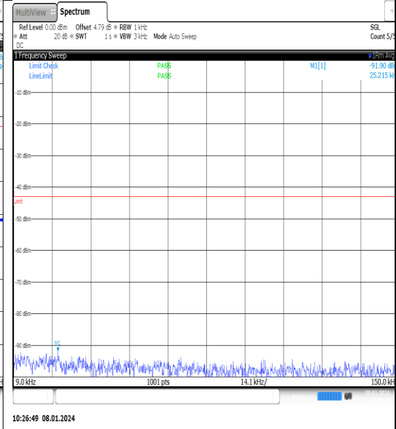
NTN_V_N77-3700- 3980_PC2_30_25_L_TID11_NS_01_0.009_0.15_ #1
