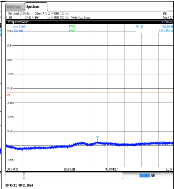
NTNV_N77-3700- 3980_PC2_30_25_L_TID1_NS_01_30_1000_#1
