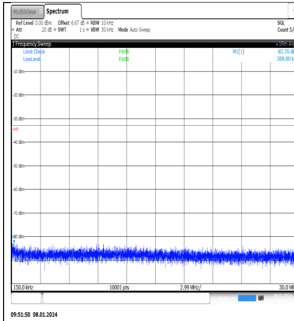
NTNV_N77-3700- 3980_PC2_30_25_L_TID3_NS_01_0.15_30_#1
