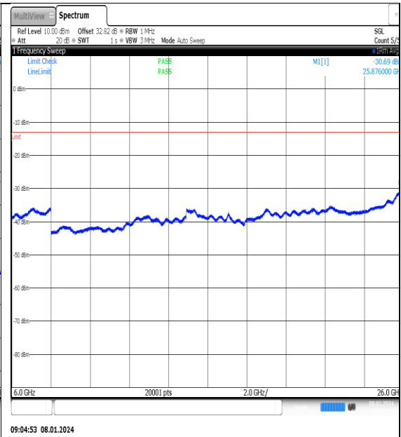
NTNV_N77-3700- 3980_PC2_30_20_H_TID5_NS_01_6000_26000_# #1
