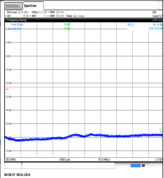
NTNV_N77-3700- 3980_PC2_30_20_H_TID3_NS_01_30_1000_#1
