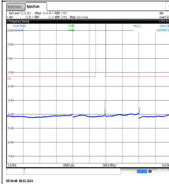
NTNV_N77-3700-3980_PC2_30_20_H_TID14_NS_01_1000_6000_#1
