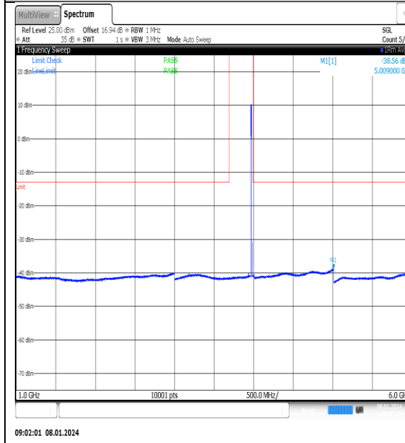
NTNV_N77-3700- 3980_PC2_30_20_H_TID4_NS_01_1000_6000_#1
