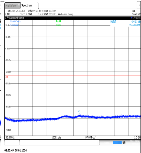
NTNV_N77-3700- 3980_PC2_30_20_H_TID2_NS_01_30_1000_#1
