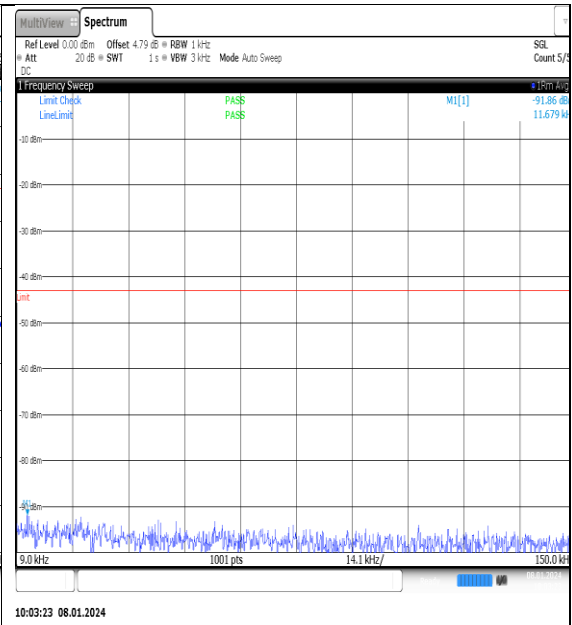
NTNV_N77-3700- 3980_PC2_30_25_L_TID6_NS_01_0.009_0.15_# 1
