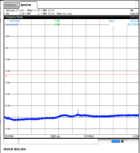
NTNV_N77-3700- 3980_PC2_30_20_H_TID5_NS_01_30_1000_#1
