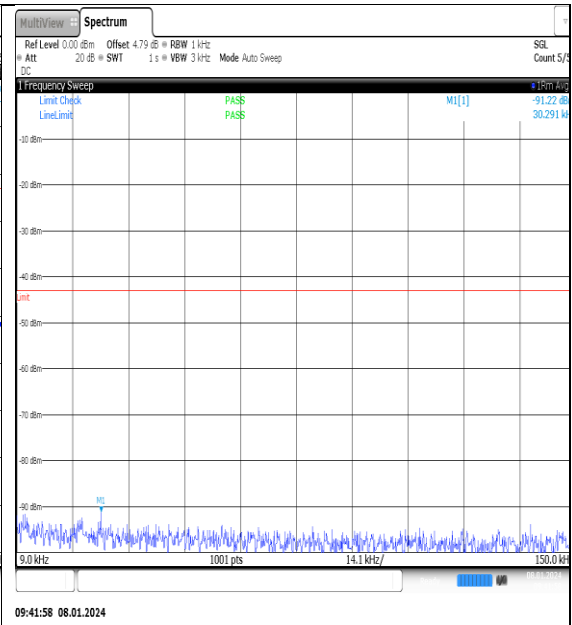
NTNV_N77-3700- 3980_PC2_30_20_H_TID15_NS_01_0.009_0.15_ #1
