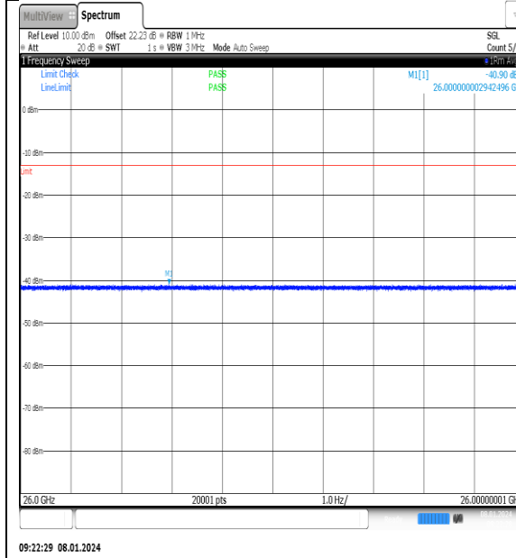
NTN_V_N77-3700- 3980_PC2_30_20_H_TID11_NS_01_26000_4000_0_#1
