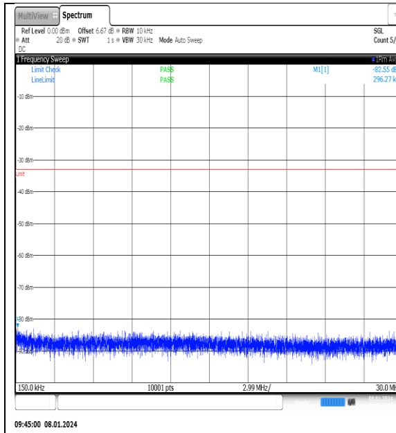
NTNV_N77-3700- 3980_PC2_30_25_L_TID1_NS_01_0.15_30_#1
