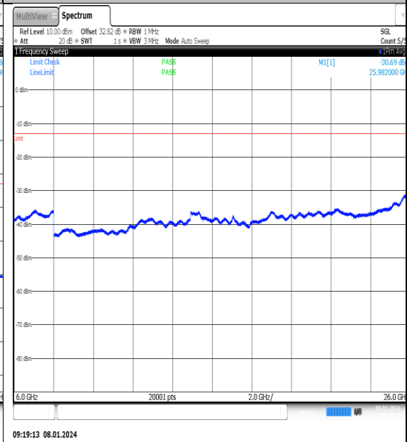
NTN_V_N77-3700- 3980_PC2_30_20_H_TID10_NS_01_6000_26000_#1
