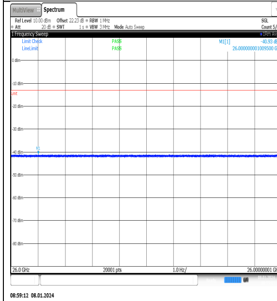
NTN_V_N77-3700- 3980_PC2_30_20_H_TID3_NS_01_26000_40000_# #1
