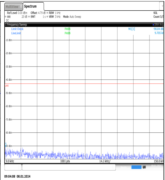
NTNV_N77-3700- 3980_PC2_30_20_H_TID5_NS_01_0.009_0.15_# 1
