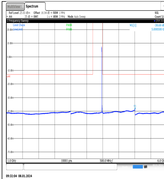
NTN_V_N77-3700- 3980_PC2_30_20_H_TID13_NS_01_1000_6000_ #1
