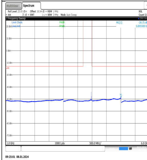
NTNV_N77-3700- 3980_PC2_30_20_H_TID12_NS_01_1000_6000_#1
