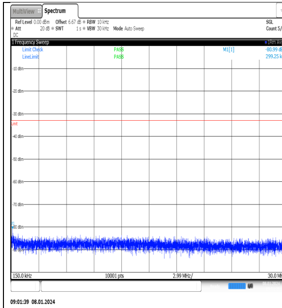
NTNV_N77-3700- 3980_PC2_30_20_H_TID4_NS_01_0.15_30_#1
