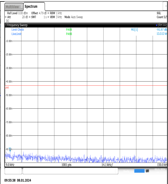
NTNV_N77-3700- 3980_PC2_30_25_L_TID4_NS_01_0.009_0.15_# 1
