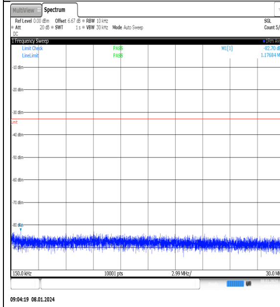
NTNV_N77-3700- 3980_PC2_30_20_H_TID5_NS_01_0.15_30_#1
