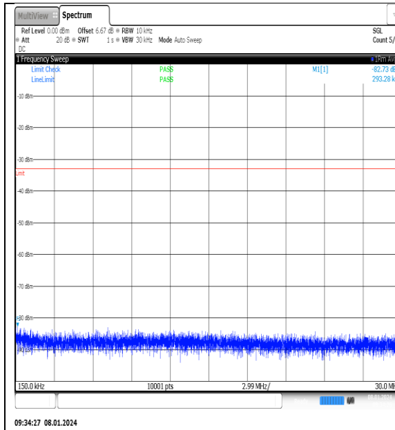
NTNV_N77-3700-3980_PC2_30_20_H_TID14_NS_01_0.15_30_#1
