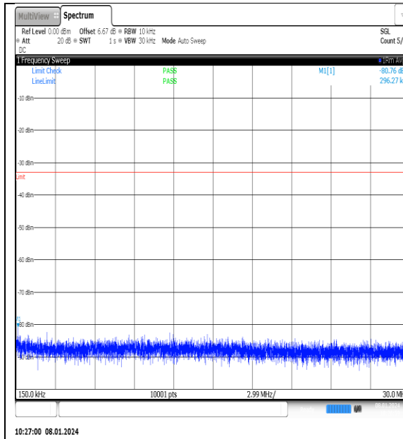
NTNV_N77-3700- 3980_PC2_30_25_L_TID11_NS_01_0.15_30_#1
