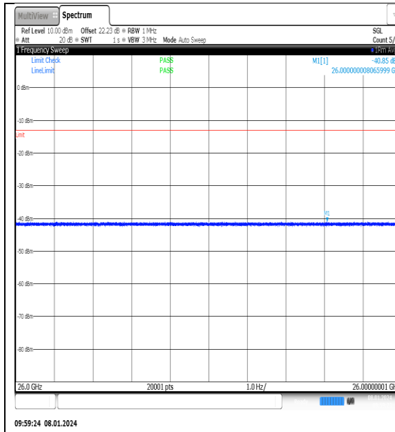
NTNV_N77-3700- 3980_PC2_30_25_L_TID5_NS_01_26000_40000 #1
