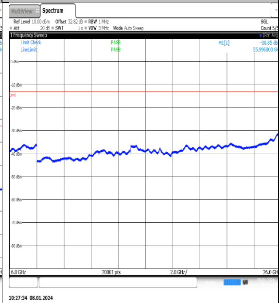
NTNV_N77-3700- 3980_PC2_30_25_L_TID11_NS_01_6000_26000_#1
