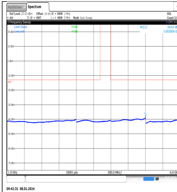
NTNV_N77-3700- 3980_PC2_30_20_H_TID15_NS_01_1000_6000_#1
