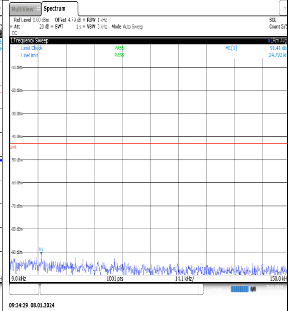
NTN_V_N77-3700- 3980_PC2_30_20_H_TID12_NS_01_0.009_0.15_#1
