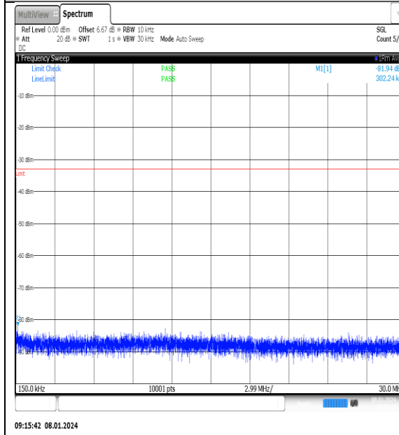
NTNV_N77-3700- 3980_PC2_30_20_H_TID9_NS_01_0.15_30_#1
