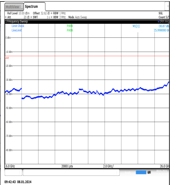
NTNV_N77-3700- 3980_PC2_30_20_H_TID15_NS_01_6000_26000_#1
