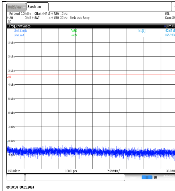
NTNV_N77-3700- 3980_PC2_30_25_L_TID5_NS_01_0.15_30_#1
