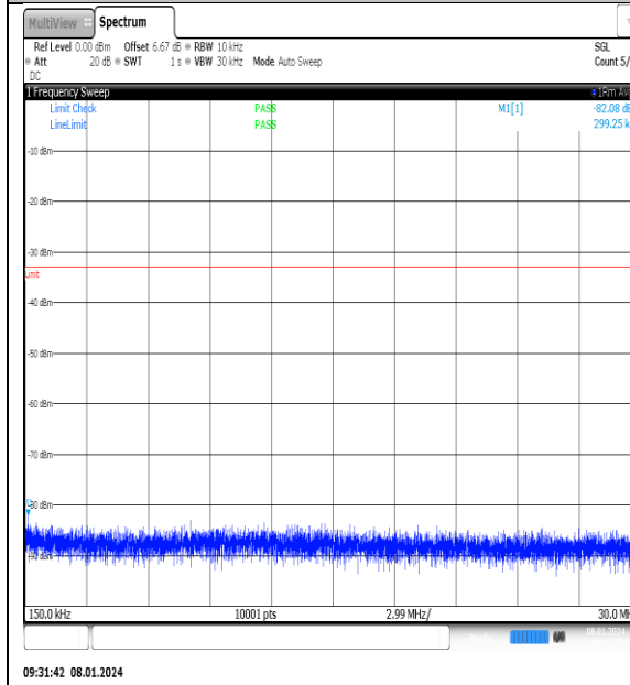
NTNV_N77-3700- 3980_PC2_30_20_H_TID13_NS_01_0.15_30_#1
