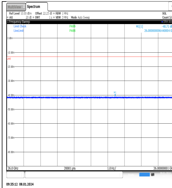
NTNV_N77-3700- 3980_PC2_30_20_H_TID14_NS_01_26000_4000 0_#1
