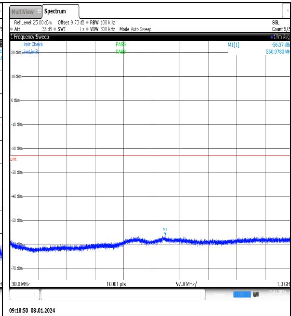
NTN_V_N77-3700- 3980_PC2_30_20_H_TID10_NS_01_30_1000_#1
