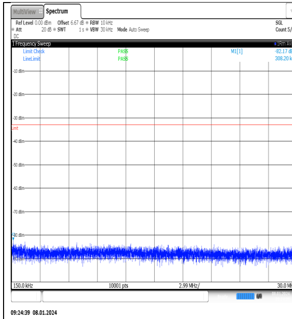
NTNV_N77-3700- 3980_PC2_30_20_H_TID12_NS_01_0.15_30_#1
