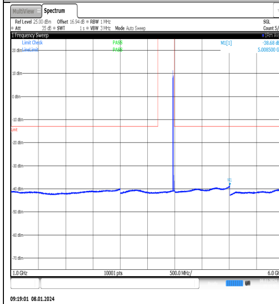
NTN_V_N77-3700- 3980_PC2_30_20_H_TID10_NS_01_1000_6000_#1
