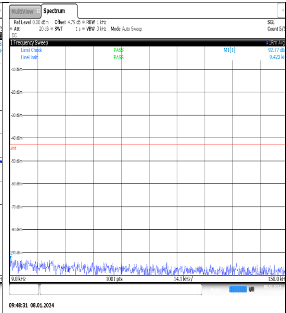
NTNV_N77-3700- 3980_PC2_30_25_L_TID2_NS_01_0.009_0.15_# 1
