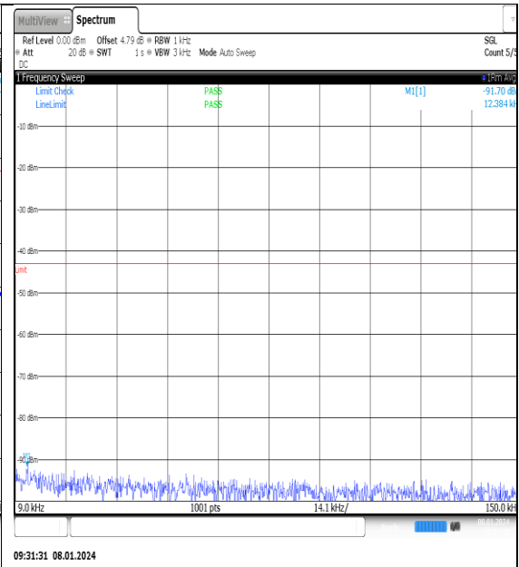
NTNV_N77-3700- 3980_PC2_30_20_H_TID13_NS_01_0.009_0.15_ #1
