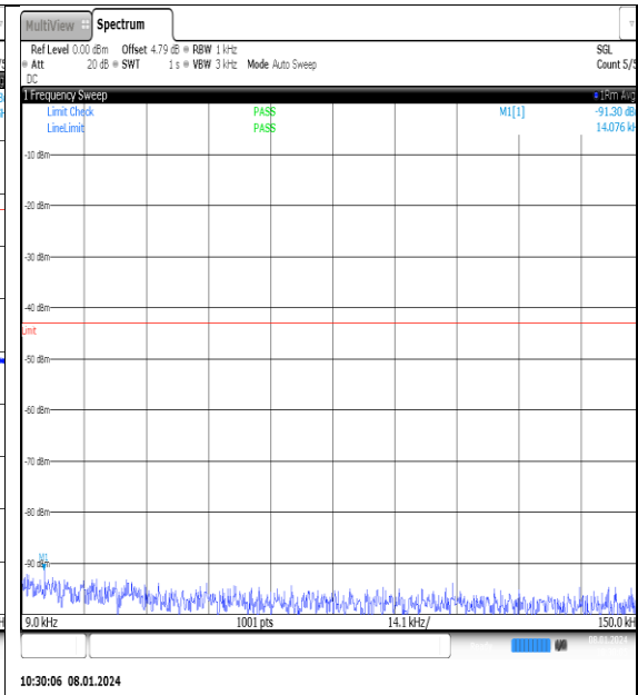
NTNV_N77-3700- 3980_PC2_30_25_L_TID12_NS_01_0.009_0.15_ #1
