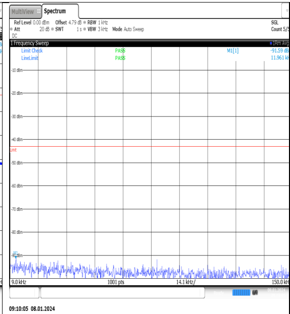
NTNV_N77-3700- 3980_PC2_30_20_H_TID7_NS_01_0.009_0.15_# 1
