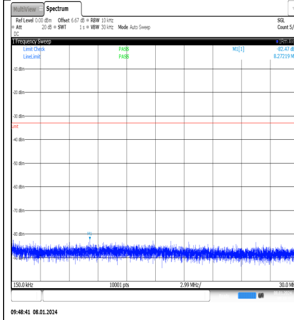
NTNV_N77-3700- 3980_PC2_30_25_L_TID2_NS_01_0.15_30_#1
