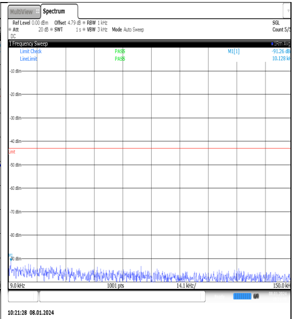
NTNV_N77-3700- 3980_PC2_30_25_L_TID10_NS_01_0.009_0.15_ #1
