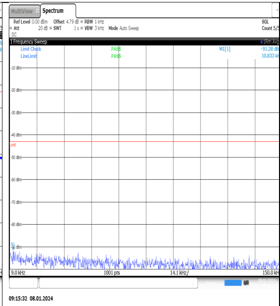
NTNV_N77-3700- 3980_PC2_30_20_H_TID9_NS_01_0.009_0.15_# 1
