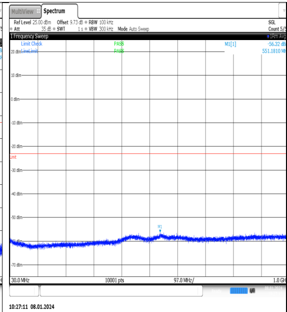
NTNV_N77-3700- 3980_PC2_30_25_L_TID11_NS_01_30_1000_#1
