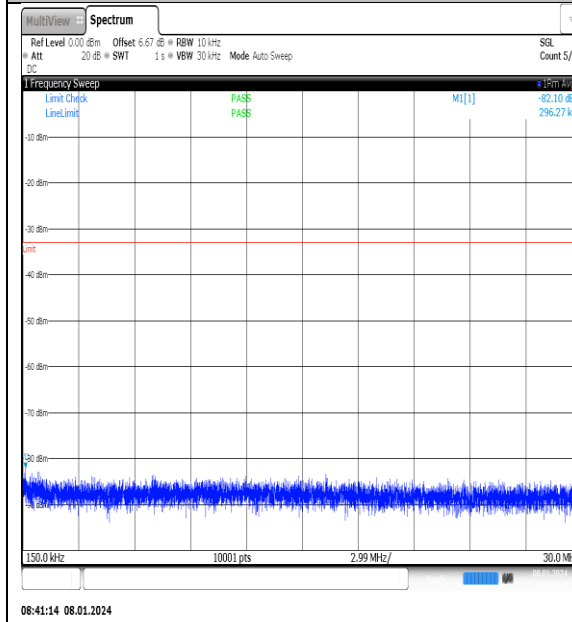
NTNV_N77-3700- 3980_PC2_30_20_M_TID12_NS_01_0.15_30_#1
