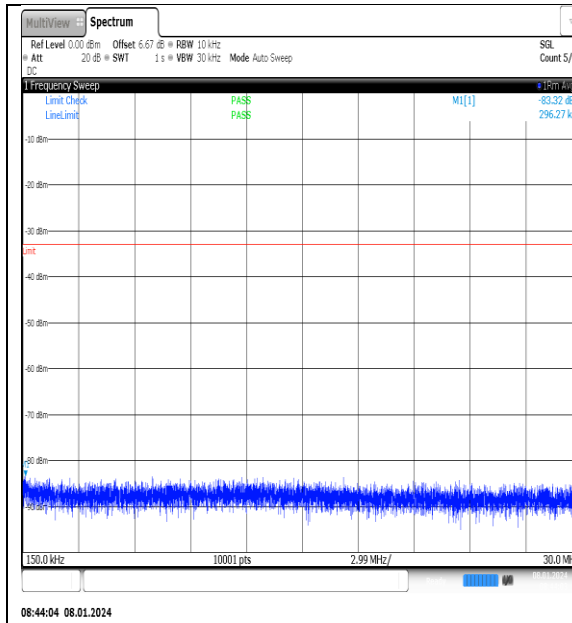
NTNV_N77-3700- 3980_PC2_30_20_M_TID13_NS_01_0.15_30_#1
