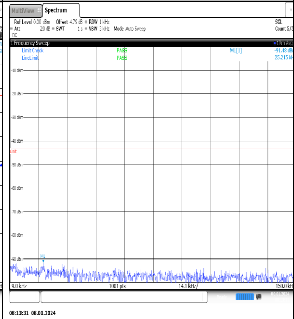
NTN_V_N77-3700- 3980_PC2_30_20_M_TID5_NS_01_0.009_0.15_# 1
