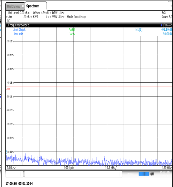
NTN_V_N77-3700- 3980_PC2_30_20_L_TID10_NS_01_0.009_0.15_# #1
