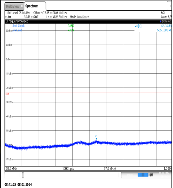
NTNV_N77-3700- 3980_PC2_30_20_M_TID12_NS_01_30_1000_#1
