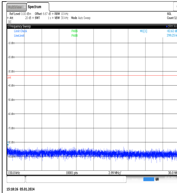
NTNV_N77-3700-3980_PC2_30_20_L_TID8_NS_01_0.15_30_#1
