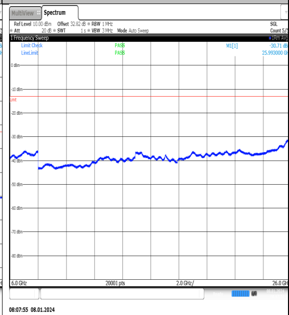
NTNV_N77-3700- 3980_PC2_30_20_M_TID3_NS_01_6000_26000_# #1
