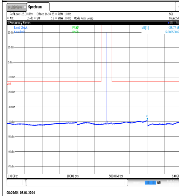
NTNV_N77-3700- 3980_PC2_30_20_M_TID9_NS_01_1000_6000_#1
