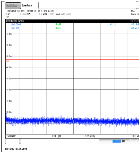
NTNV_N77-3700- 3980_PC2_30_20_M_TID5_NS_01_0.15_30_#1
