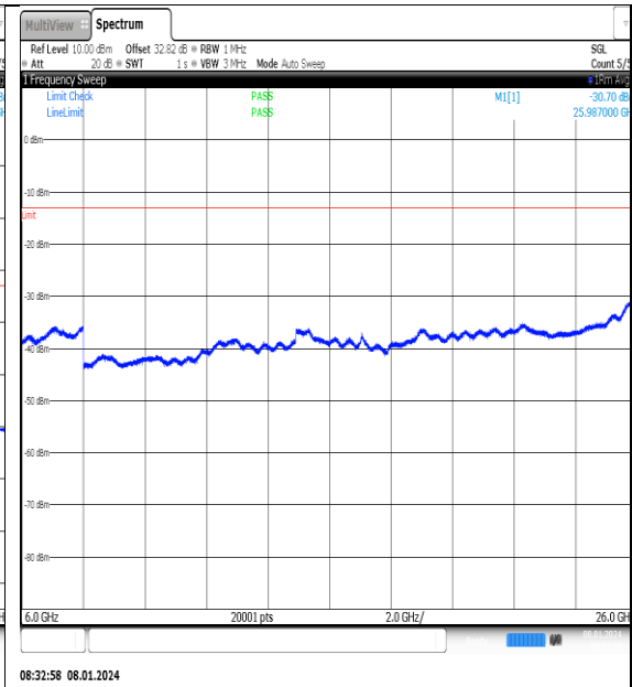
NTN_V_N77-3700- 3980_PC2_30_20_M_TID10_NS_01_6000_26000 #1
