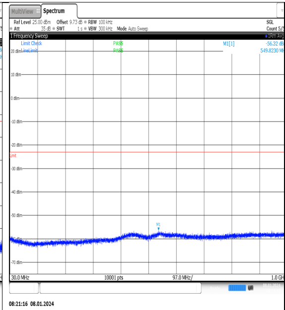
NTNV_N77-3700- 3980_PC2_30_20_M_TID7_NS_01_30_1000_#1
