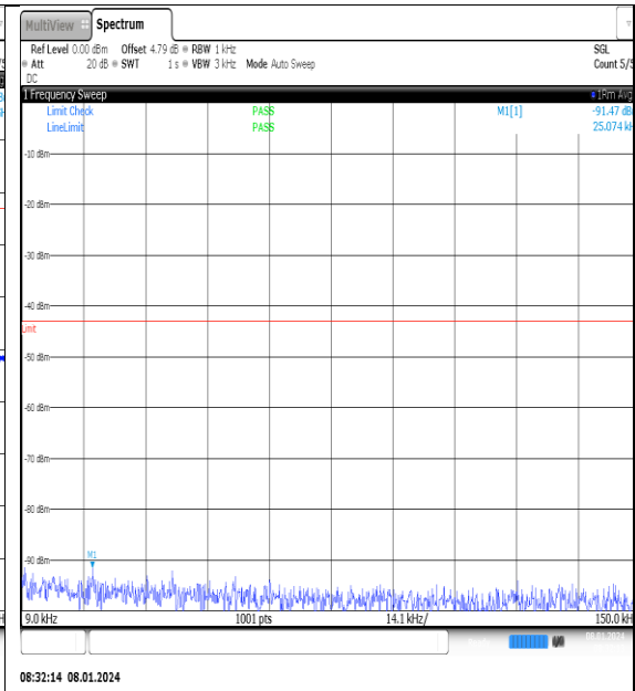
NTNV_N77-3700- 3980_PC2_30_20_M_TID10_NS_01_0.009_0.15_ #1
