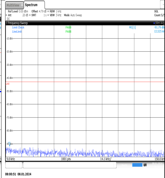
NTN_V_N77-3700- 3980_PC2_30_20_M_TID1_NS_01_0.009_0.15_# 1
