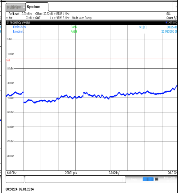
NTNV_N77-3700- 3980_PC2_30_20_M_TID15_NS_01_6000_26000_#1
