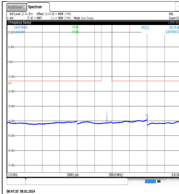
NTN_V_N77-3700- 3980_PC2_30_20_M_TID14_NS_01_1000_6000_ #1
