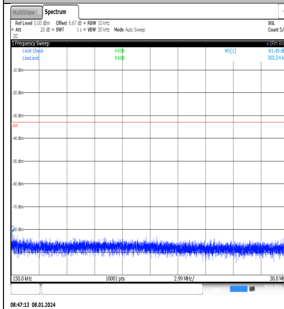
NTNV_N77-3700- 3980_PC2_30_20_M_TID14_NS_01_0.15_30_#1
