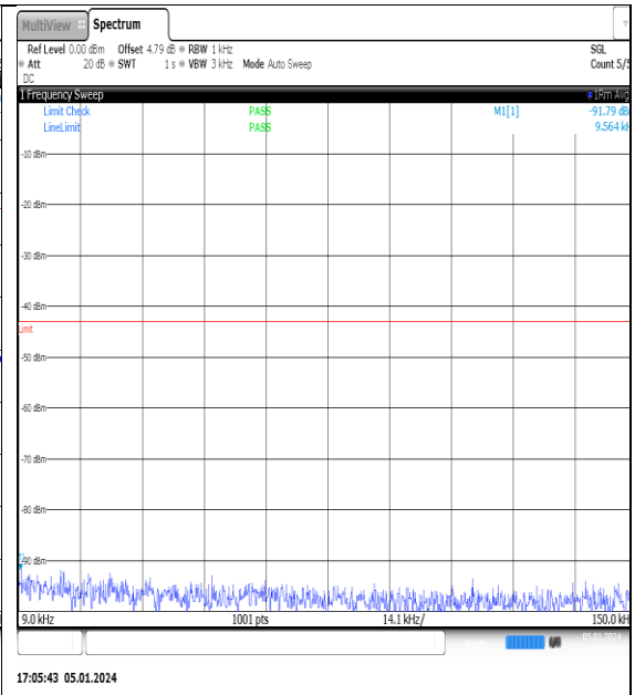
NTNV_N77-3700- 3980_PC2_30_20_L_TID11_NS_01_0.009_0.15_#1
