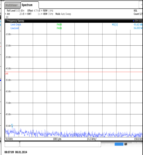
NTN_V_N77-3700- 3980_PC2_30_20_M_TID3_NS_01_0.009_0.15_# 1
