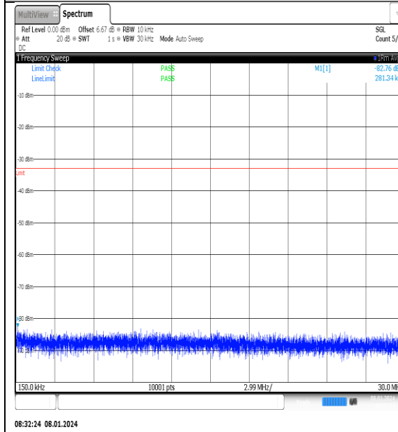
NTNV_N77-3700- 3980_PC2_30_20_M_TID10_NS_01_0.15_30_#1
