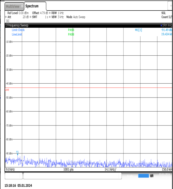
NTN V _N77-3700- 3980_PC2_30_20_L_TID8_NS_01_0.009_0.15_# 1
