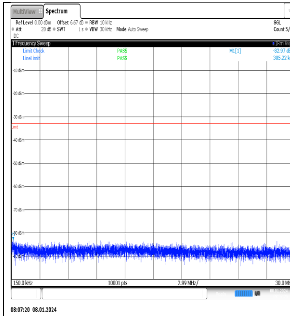
NTNV_N77-3700- 3980_PC2_30_20_M_TID3_NS_01_0.15_30_#1
