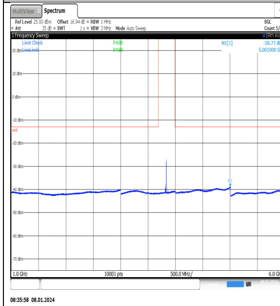
NTNV_N77-3700- 3980_PC2_30_20_M_TID11_NS_01_1000_6000_#1
