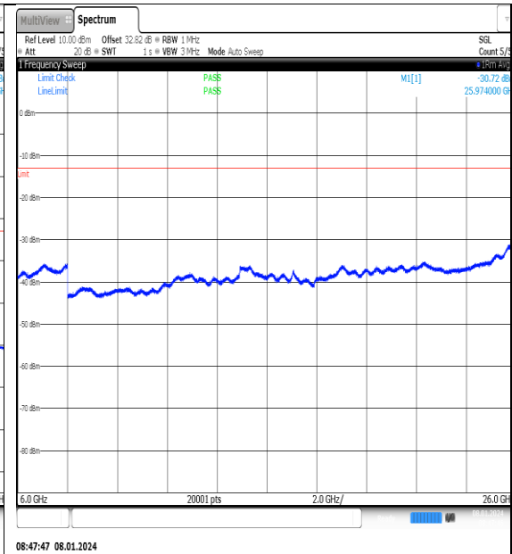
NTN_V_N77-3700- 3980_PC2_30_20_M_TID14_NS_01_6000_26000 #1
