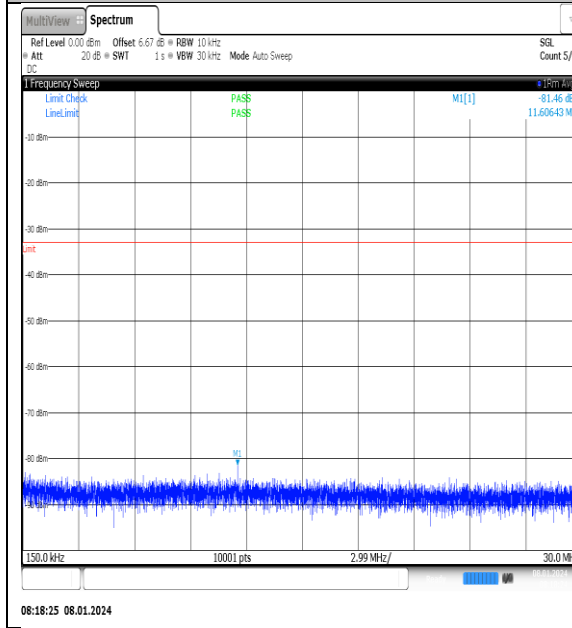
NTNV_N77-3700- 3980_PC2_30_20_M_TID6_NS_01_0.15_30_#1
