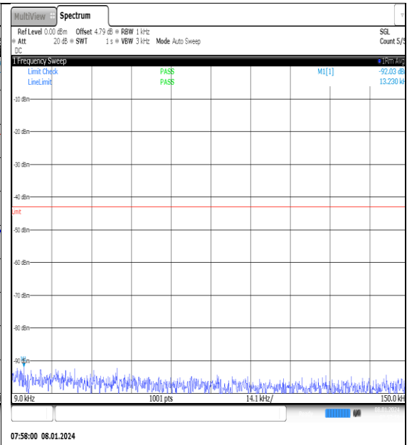
NTNV_N77-3700- 3980_PC2_30_20_L_TID15_NS_01_0.009_0.15_#1
