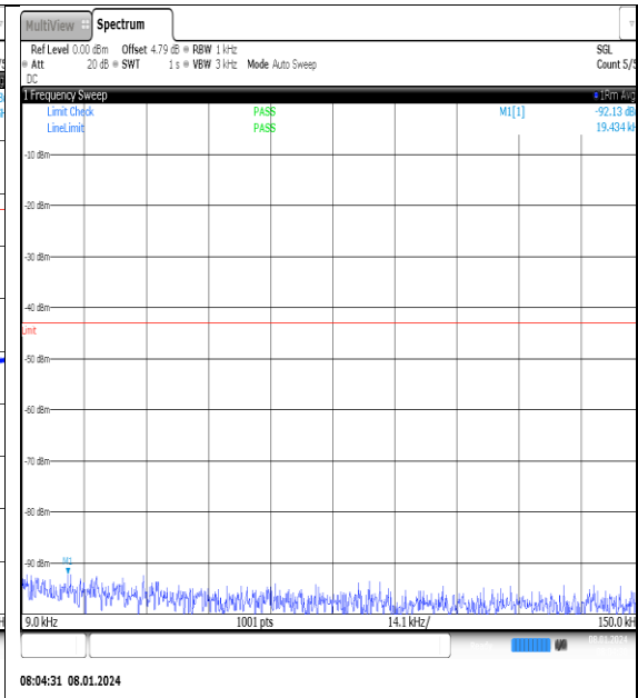
NTNV_N77-3700- 3980_PC2_30_20_M_TID2_NS_01_0.009_0.15_# 1
