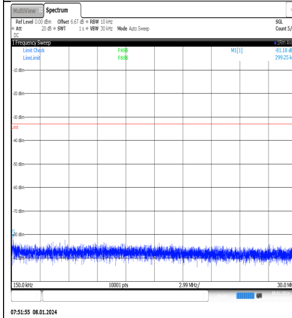
NTNV_N77-3700- 3980_PC2_30_20_L_TID13_NS_01_0.15_30_#1
