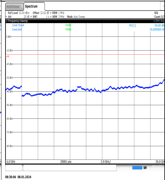
NTNV_N77-3700- 3980_PC2_30_20_M_TID9_NS_01_6000_26000_#1
