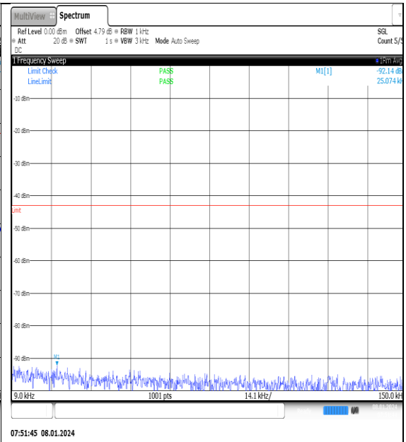
NTNV_N77-3700- 3980_PC2_30_20_L_TID13_NS_01_0.009_0.15_ #1
