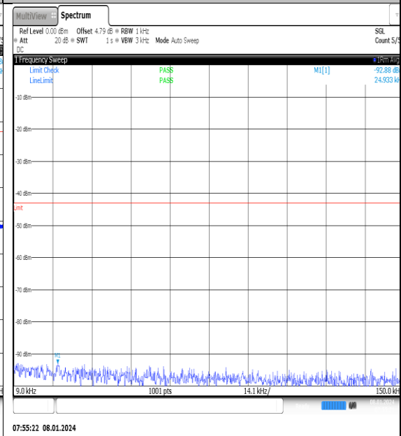
NTN_V_N77-3700- 3980_PC2_30_20_L_TID14_NS_01_0.009_0.15_ #1
