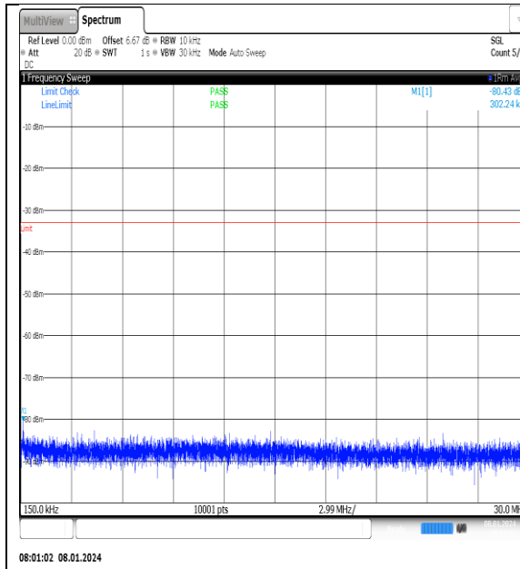
NTNV_N77-3700- 3980_PC2_30_20_M_TID1_NS_01_0.15_30_#1
