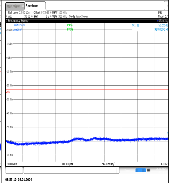
NTNV_N77-3700- 3980_PC2_30_20_H_TID1_NS_01_30_1000_#1
