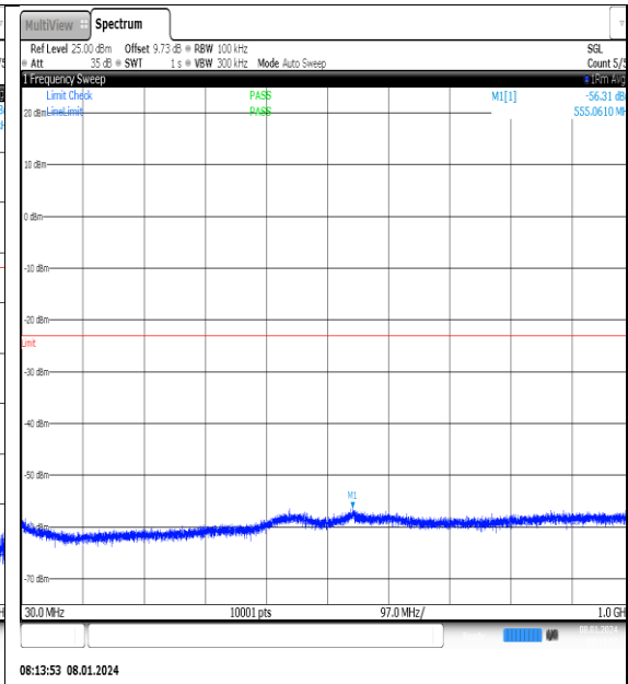
NTNV_N77-3700- 3980_PC2_30_20_M_TID5_NS_01_30_1000_#1
