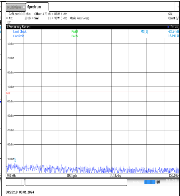
NTNV_N77-3700- 3980_PC2_30_20_M_TID8_NS_01_0.009_0.15_# 1
