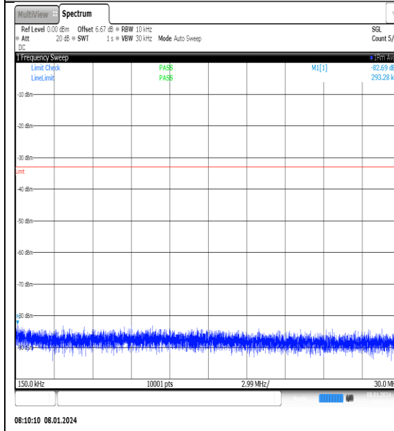
NTNV_N77-3700- 3980_PC2_30_20_M_TID4_NS_01_0.15_30_#1
