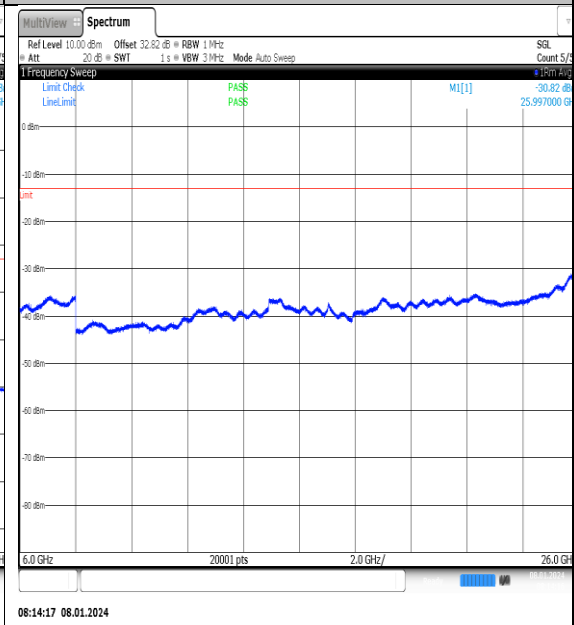
NTNV_N77-3700- 3980_PC2_30_20_M_TID5_NS_01_6000_26000_#1
