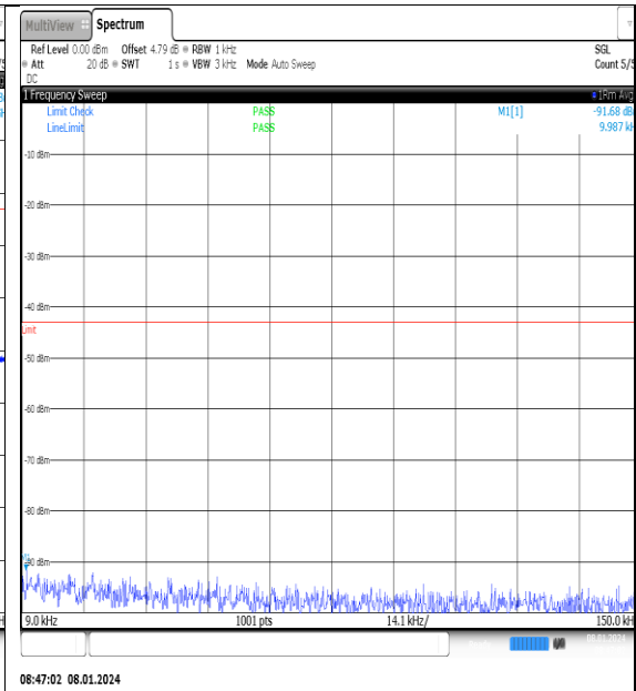
NTNV_N77-3700- 3980_PC2_30_20_M_TID14_NS_01_0.009_0.15_#1
