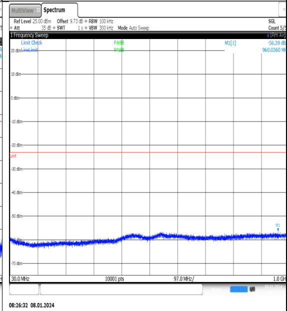
NTNV_N77-3700- 3980_PC2_30_20_M_TID8_NS_01_30_1000_#1
