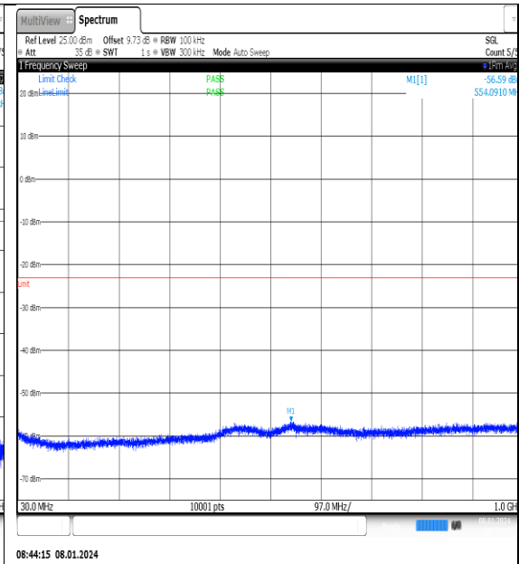
NTNV_N77-3700- 3980_PC2_30_20_M_TID13_NS_01_30_1000_#1
