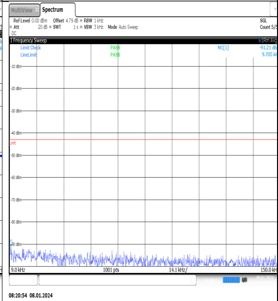
NTNV_N77-3700- 3980_PC2_30_20_M_TID7_NS_01_0.009_0.15_# 1
