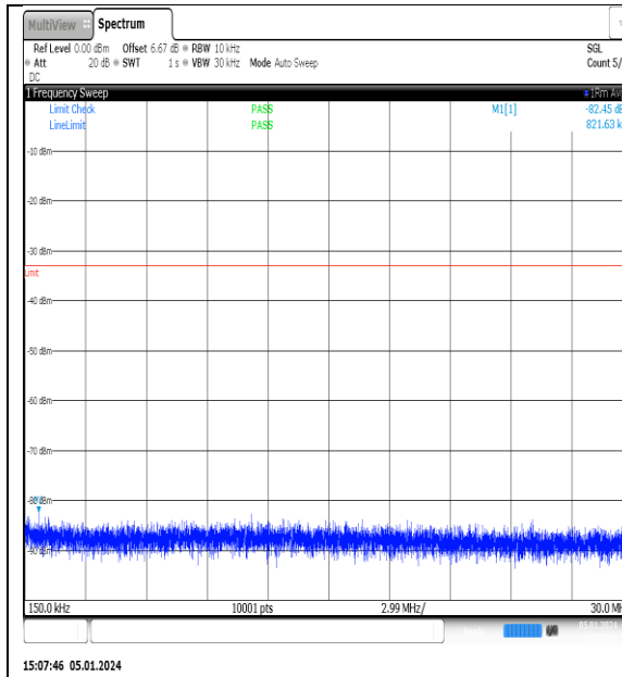
NTNV_N77-3700- 3980_PC2_30_20_L_TID4_NS_01_0.15_30_#1
