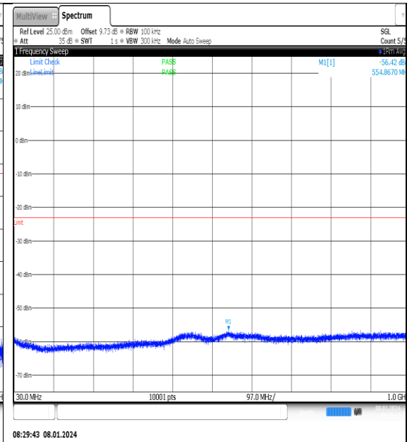
NTNV_N77-3700- 3980_PC2_30_20_M_TID9_NS_01_30_1000_#1
