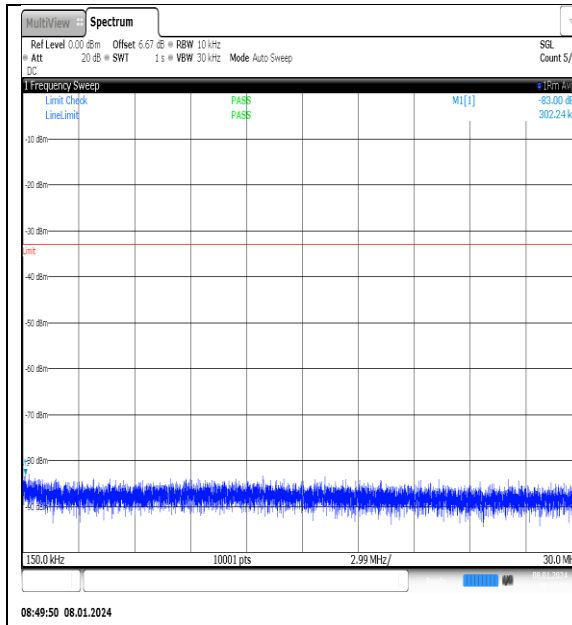
NTNV_N77-3700- 3980_PC2_30_20_M_TID15_NS_01_0.15_30_#1
