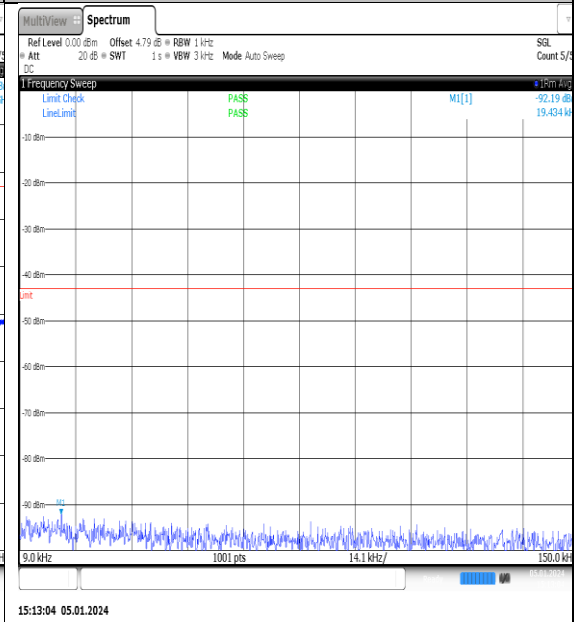
NTNV_N77-3700- 3980_PC2_30_20_L_TID6_NS_01_0.009_0.15_# 1
