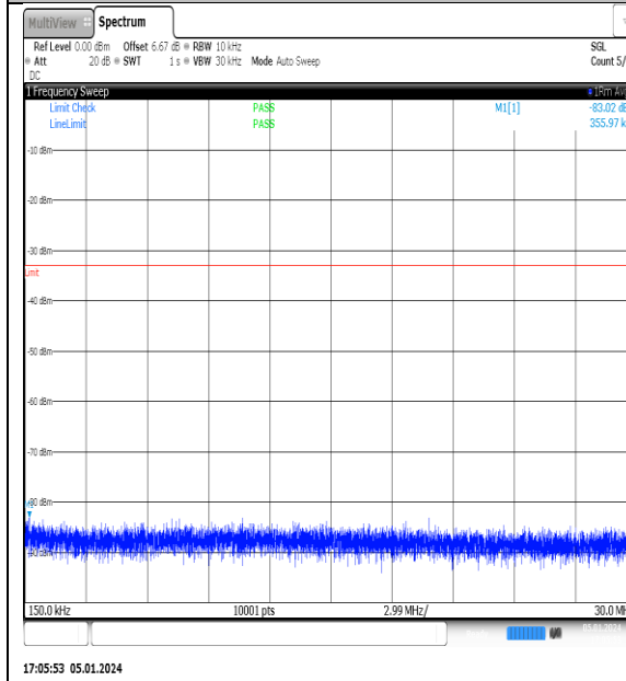
NTNV_N77-3700- 3980_PC2_30_20_L_TID11_NS_01_0.15_30_#1
