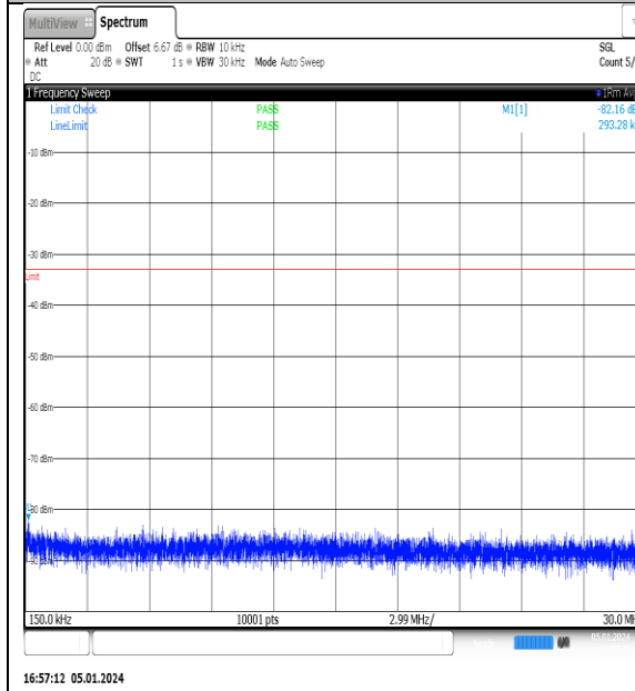
NTNV_N77-3700- 3980_PC2_30_20_L_TID9_NS_01_0.15_30_#1
