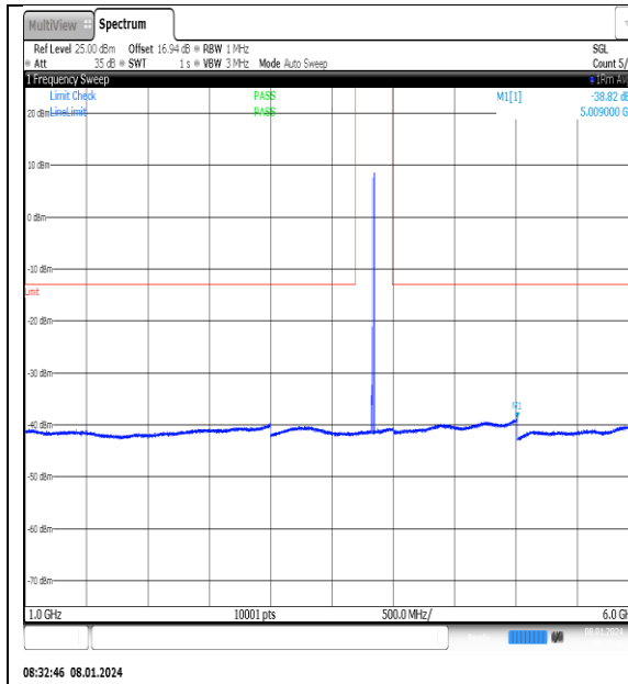
NTN_V_N77-3700- 3980_PC2_30_20_M_TID10_NS_01_1000_6000_ #1
