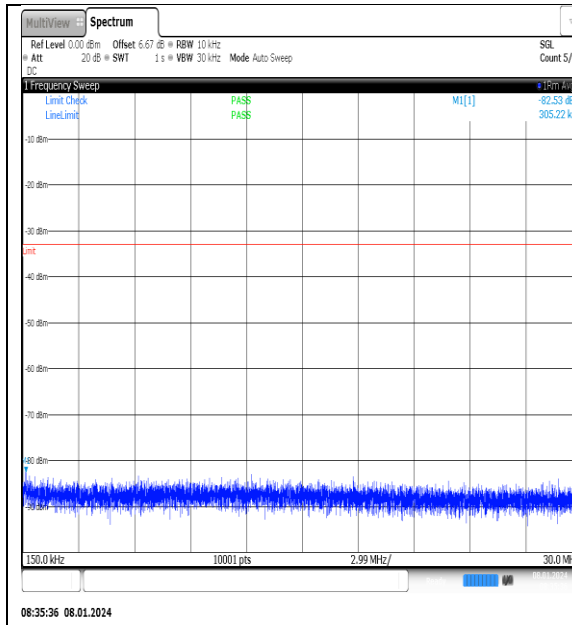
NTNV_N77-3700- 3980_PC2_30_20_M_TID11_NS_01_0.15_30_#1
