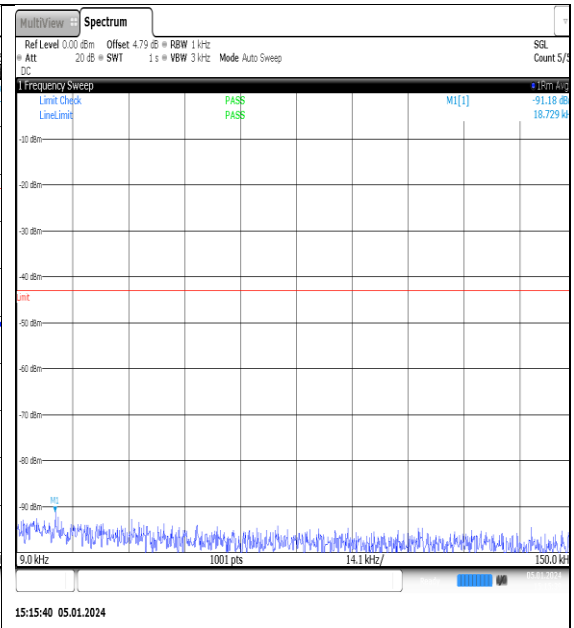
NTNV_N77-3700- 3980_PC2_30_20_L_TID7_NS_01_0.009_0.15_# 1
