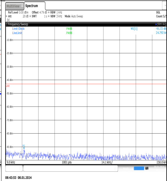
NTN_V_N77-3700- 3980_PC2_30_20_M_TID13_NS_01_0.009_0.15_ #1
