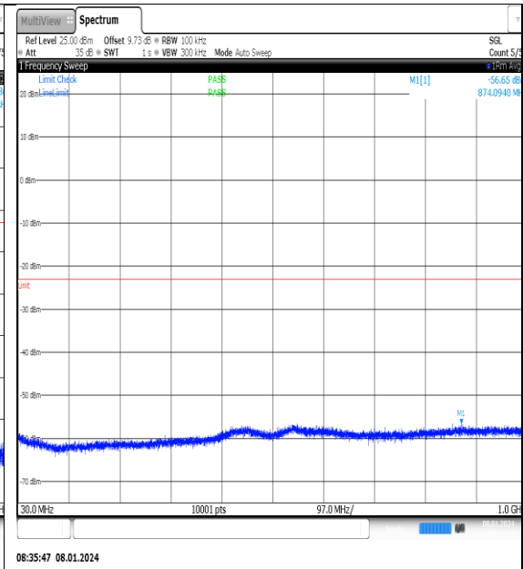
NTNV_N77-3700- 3980_PC2_30_20_M_TID11_NS_01_30_1000_#1
