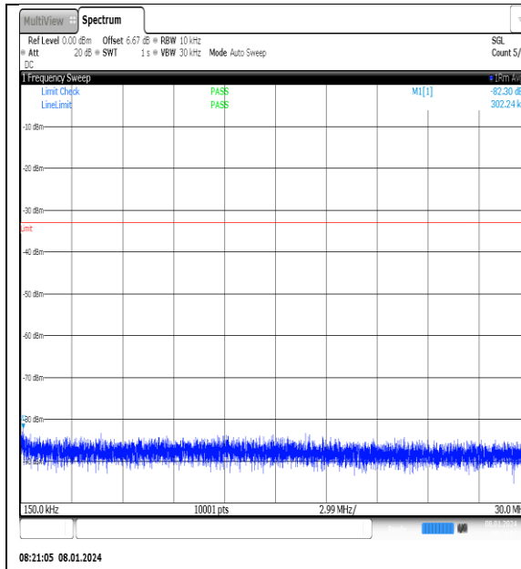
NTNV_N77-3700- 3980_PC2_30_20_M_TID7_NS_01_0.15_30_#1
