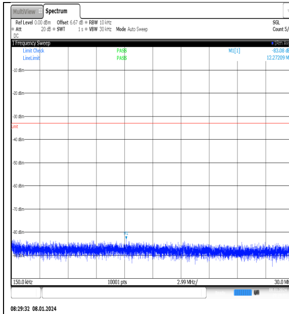
NTNV_N77-3700- 3980_PC2_30_20_M_TID9_NS_01_0.15_30_#1
