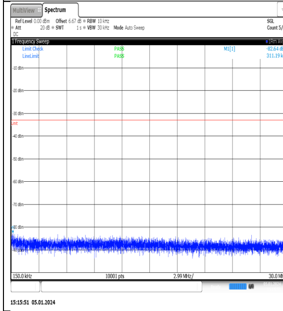
NTNV_N77-3700- 3980_PC2_30_20_L_TID7_NS_01_0.15_30_#1
