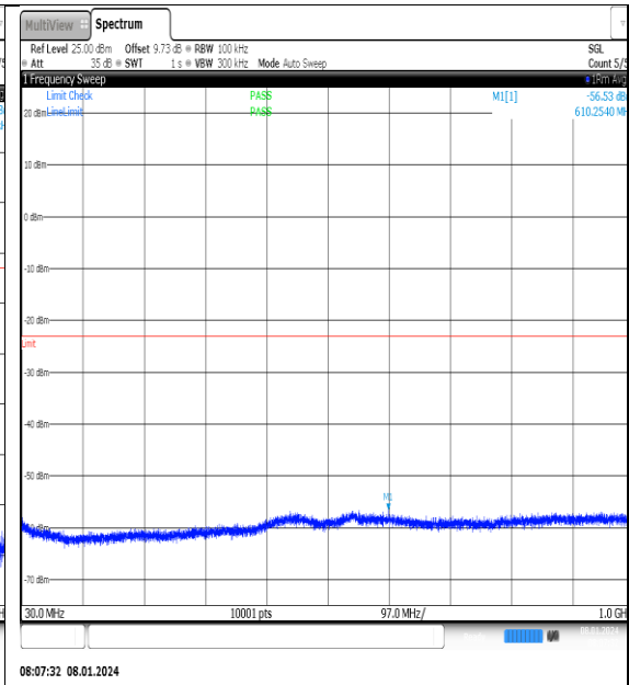
NTNV_N77-3700- 3980_PC2_30_20_M_TID3_NS_01_30_1000_#1
