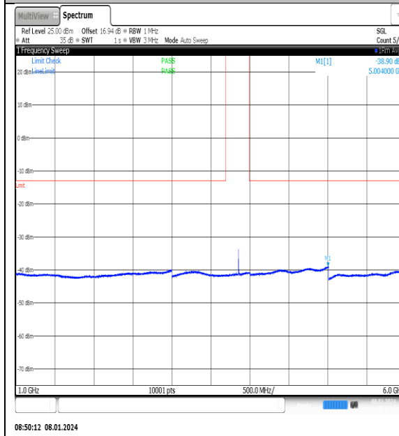
NTNV_N77-3700- 3980_PC2_30_20_M_TID15_NS_01_1000_6000_#1
