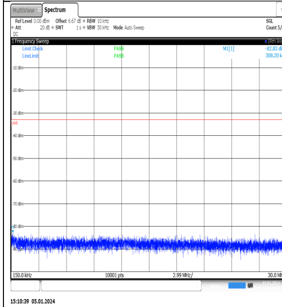
NTNV_N77-3700- 3980_PC2_30_20_L_TID5_NS_01_0.15_30_#1
