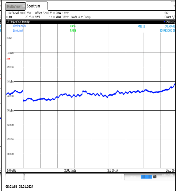
NTNV_N77-3700- 3980_PC2_30_20_M_TID1_NS_01_6000_26000_#1
