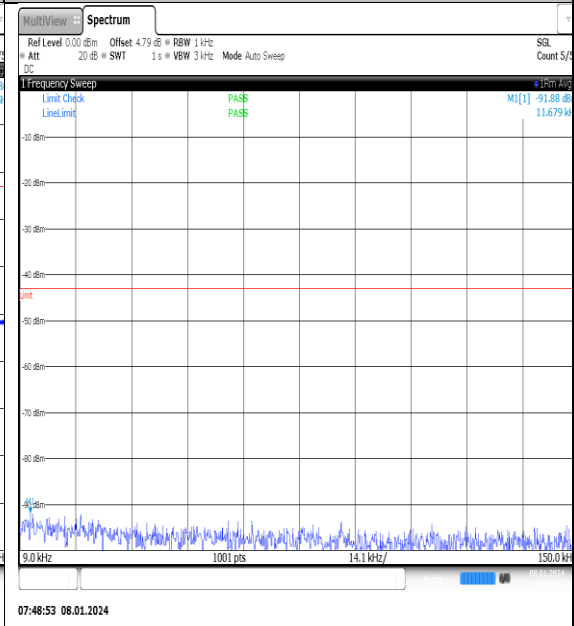
NTN_V_N77-3700- 3980_PC2_30_20_L_TID12_NS_01_0.009_0.15_ #1
