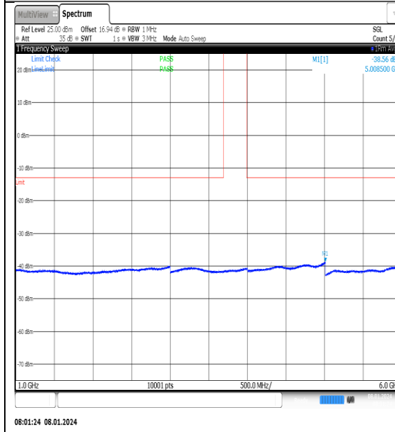
NTNV_N77-3700- 3980_PC2_30_20_M_TID1_NS_01_1000_6000_#1
