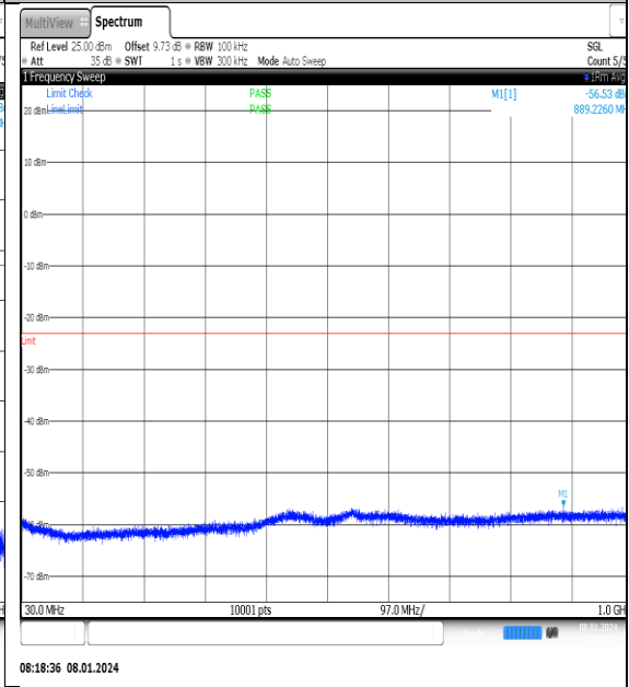
NTNV_N77-3700- 3980_PC2_30_20_M_TID6_NS_01_30_1000_#1
