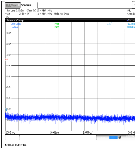
NTNV_N77-3700-3980_PC2_30_20_L_TID10_NS_01_0.15_30_#1
