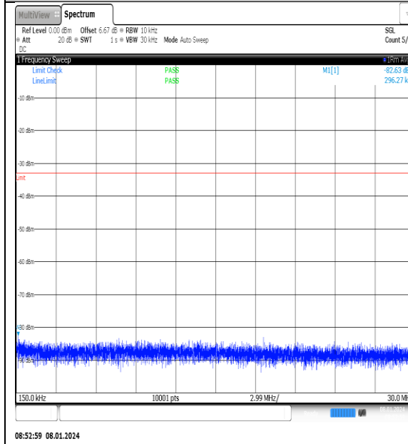
NTNV_N77-3700- 3980_PC2_30_20_H_TID1_NS_01_0.15_30_#1
