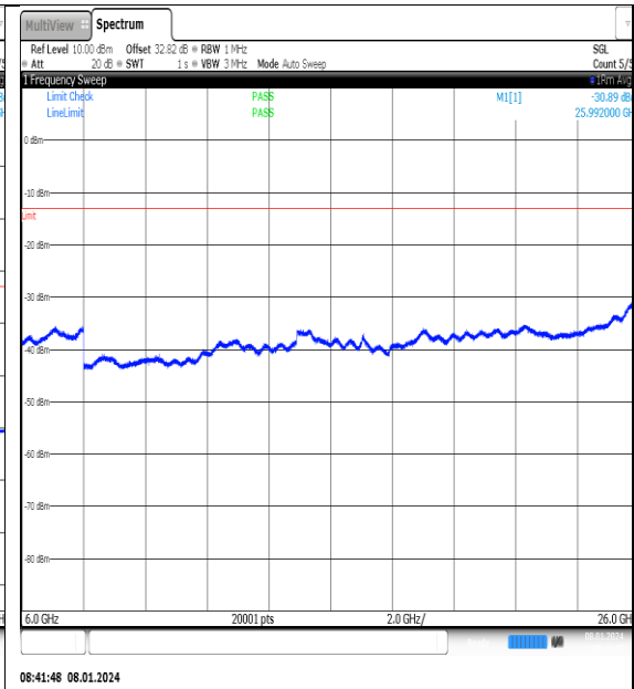
NTN_V_N77-3700- 3980_PC2_30_20_M_TID12_NS_01_6000_26000 #1
