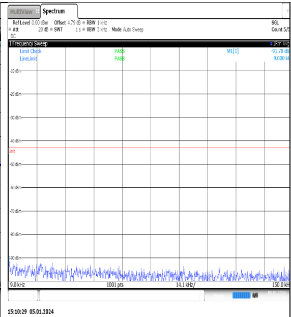
NTNV_N77-3700- 3980_PC2_30_20_L_TID5_NS_01_0.009_0.15_# 1
