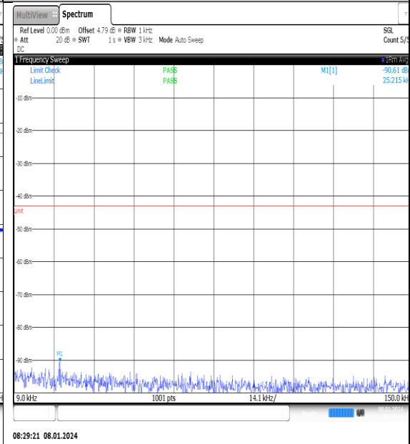
NTN_V_N77-3700- 3980_PC2_30_20_M_TID9_NS_01_0.009_0.15_# 1
