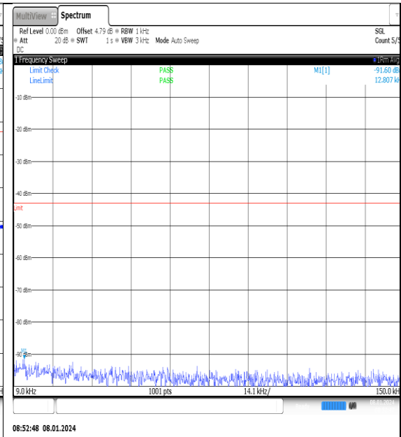
NTNV_N77-3700- 3980_PC2_30_20_H_TID1_NS_01_0.009_0.15_# 1
