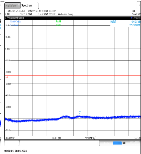
NTNV_N77-3700- 3980_PC2_30_20_M_TID15_NS_01_30_1000_#1
