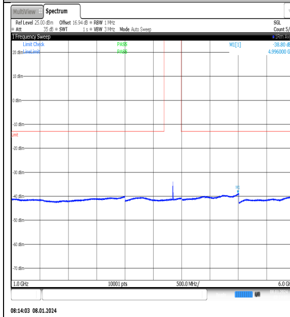
NTNV_N77-3700- 3980_PC2_30_20_M_TID5_NS_01_1000_6000_#1
