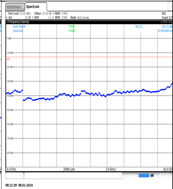
NTNV_N77-3700- 3980_PC2_30_20_M_TID7_NS_01_6000_26000_#1
