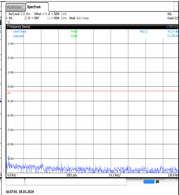
NTNV_N77-3700- 3980_PC2_30_20_L_TID9_NS_01_0.009_0.15_# 1
