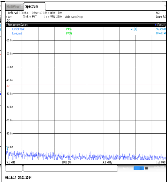
NTNV_N77-3700- 3980_PC2_30_20_M_TID6_NS_01_0.009_0.15_# 1
