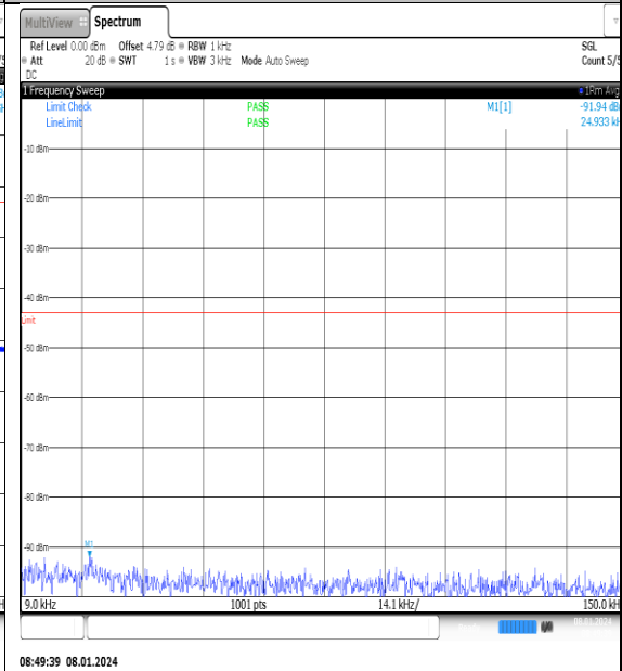
NTN_V_N77-3700- 3980_PC2_30_20_M_TID15_NS_01_0.009_0.15_ #1
