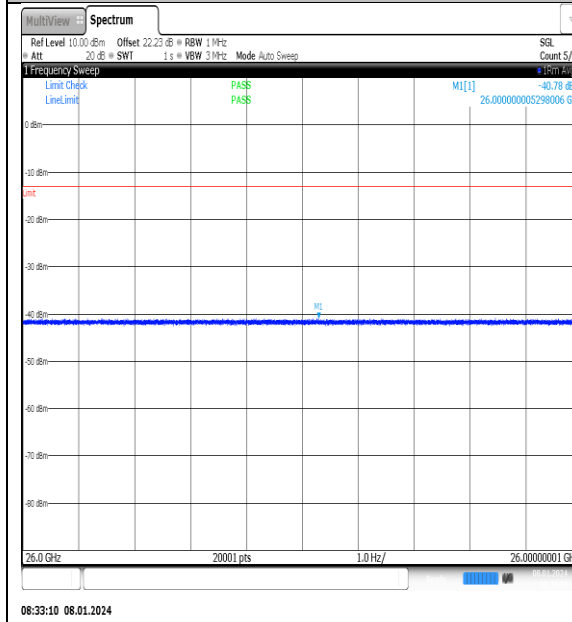
NTN_V_N77-3700- 3980_PC2_30_20_M_TID10_NS_01_26000_4000 0_#1
