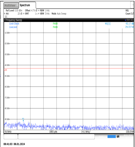
NTNV_N77-3700- 3980_PC2_30_20_M_TID12_NS_01_0.009_0.15_#1
