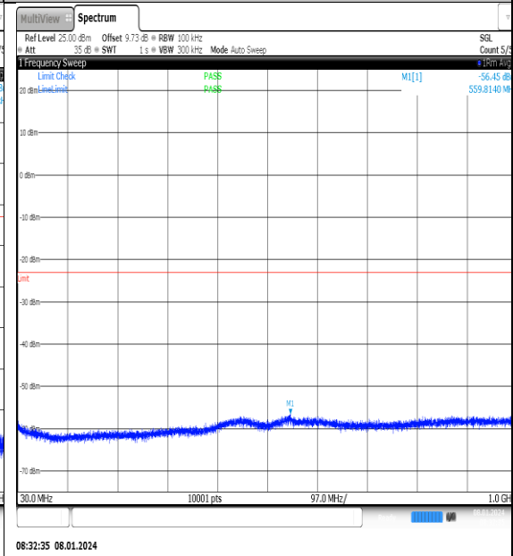
NTNV_N77-3700- 3980_PC2_30_20_M_TID10_NS_01_30_1000_#1
