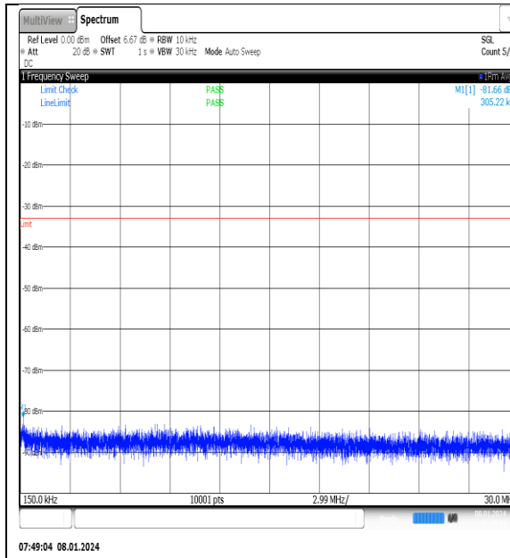
NTNV_N77-3700- 3980_PC2_30_20_L_TID12_NS_01_0.15_30_#1
