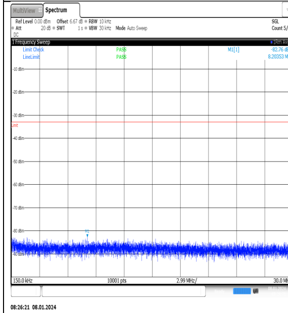
NTNV_N77-3700- 3980_PC2_30_20_M_TID8_NS_01_0.15_30_#1
