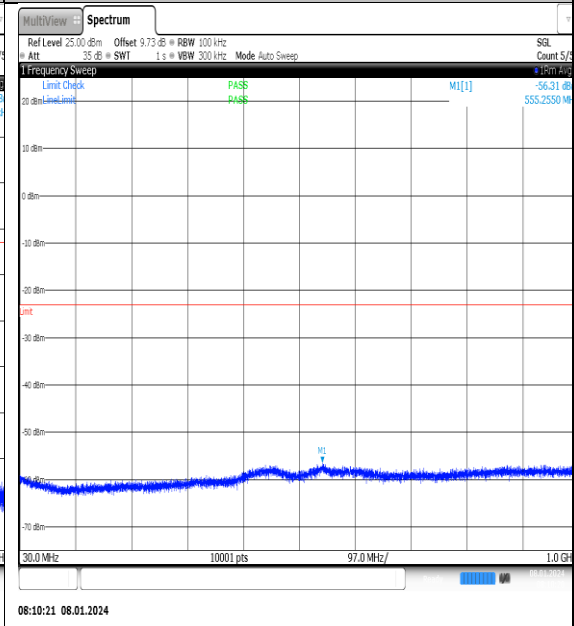
NTNV_N77-3700- 3980_PC2_30_20_M_TID4_NS_01_30_1000_#1
