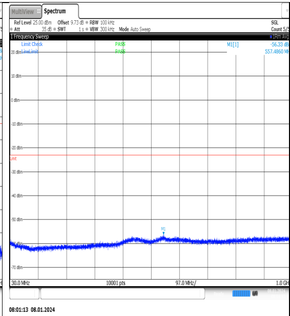
NTNV_N77-3700- 3980_PC2_30_20_M_TID1_NS_01_30_1000_#1
