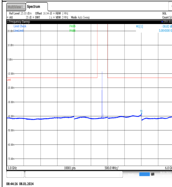
NTNV_N77-3700- 3980_PC2_30_20_M_TID13_NS_01_1000_6000_#1
