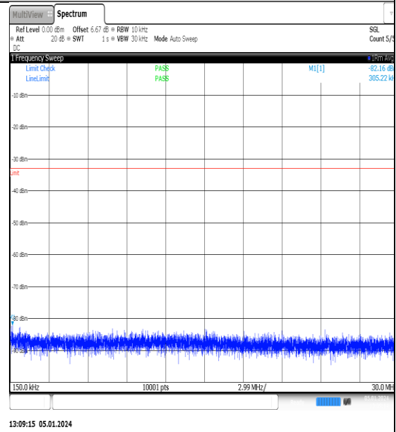
NTNV_N77-3700- 3980_PC2_30_15_H_TID4_NS_01_0.15_30_#1
