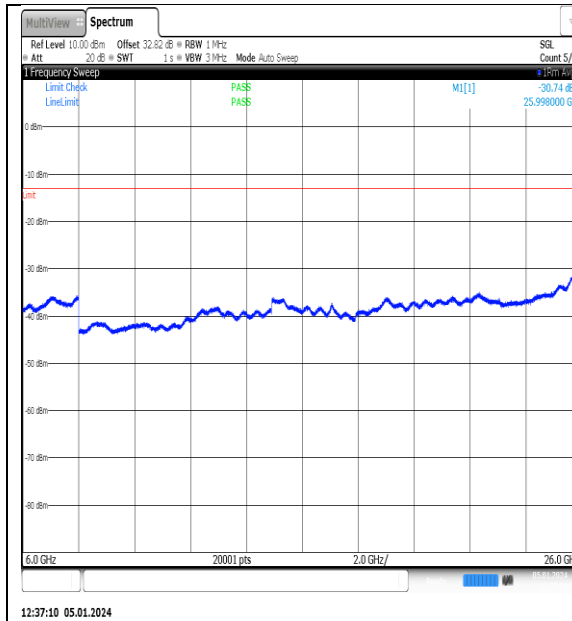
NTNV_N77-3700- 3980_PC2_30_15_M_TID12_NS_01_6000_26000 _#1
