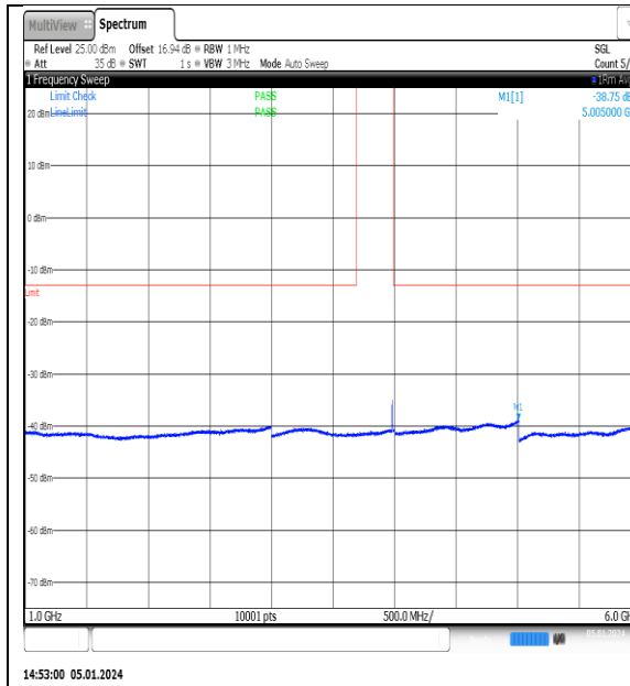
NTN_V_N77-3700- 3980_PC2_30_15_H_TID14_NS_01_1000_6000_ #1
