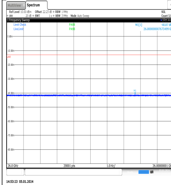
NTN_V_N77-3700- 3980_PC2_30_15_H_TID14_NS_01_26000_4000_ 0_#1
