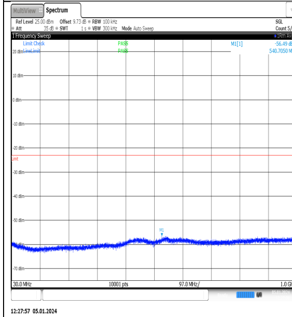
NTNV_N77-3700- 3980_PC2_30_15_M_TID10_NS_01_30_1000_#1
