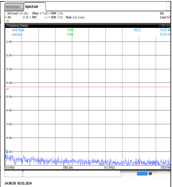
NTNV_N77-3700- 3980_PC2_30_20_L_TID1_NS_01_0.009_0.15_# 1
