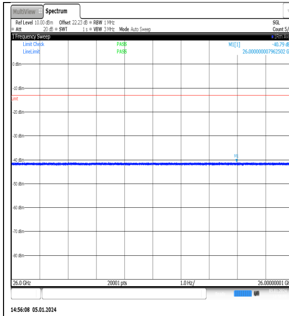
NTNV_N77-3700- 3980_PC2_30_15_H_TID15_NS_01_26000_4000 0_#1
