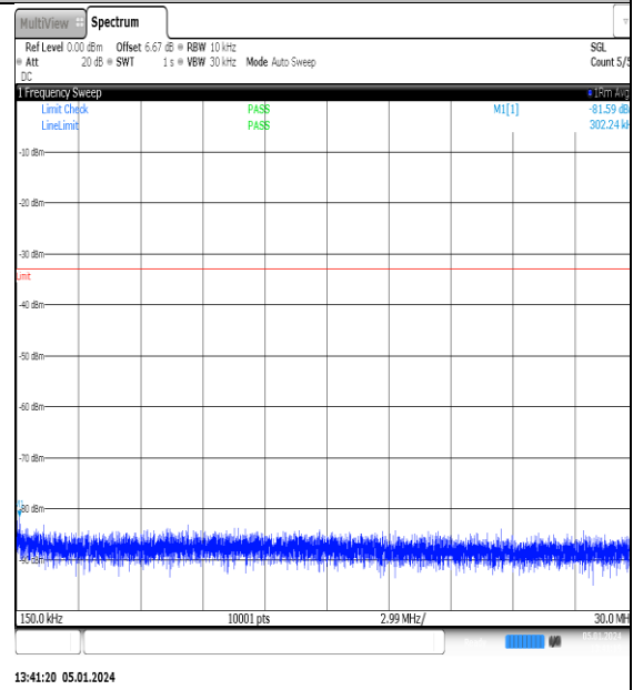
NTNV_N77-3700- 3980_PC2_30_15_H_TID6_NS_01_0.15_30_#1
