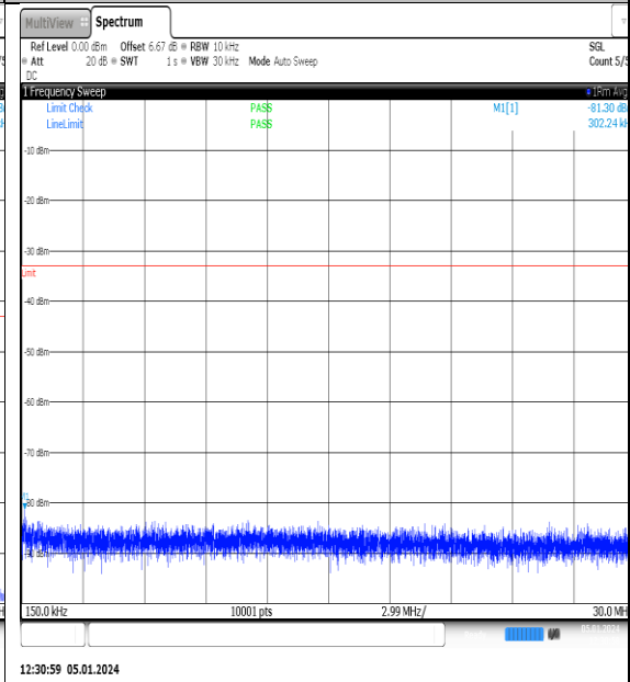
NTNV_N77-3700- 3980_PC2_30_15_M_TID11_NS_01_0.15_30_#1
