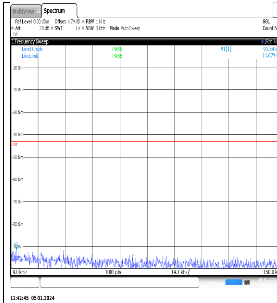
NTN_V_N77-3700- 3980_PC2_30_15_M_TID14_NS_01_0.009_0.15_ #1
