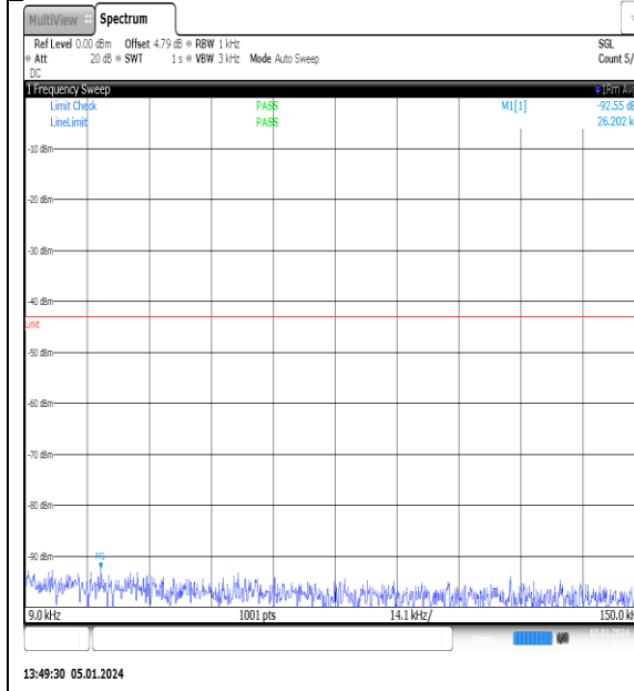
NTNV_N77-3700- 3980_PC2_30_15_H_TID8_NS_01_0.009_0.15_#1
