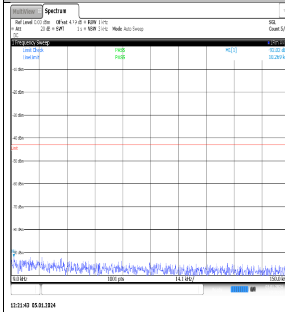
NTNV_N77-3700- 3980_PC2_30_15_M_TID9_NS_01_0.009_0.15_#1
