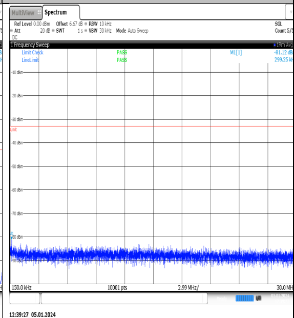
NTNV_N77-3700- 3980_PC2_30_15_M_TID13_NS_01_0.15_30_#1
