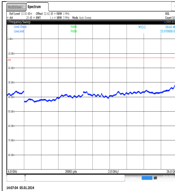
NTNV_N77-3700- 3980_PC2_30_15_H_TID11_NS_01_6000_26000 #1
