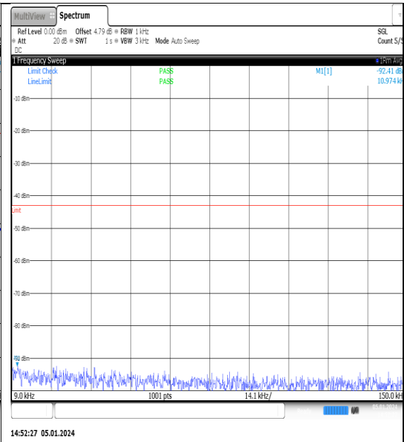
NTNV_N77-3700- 3980_PC2_30_15_H_TID14_NS_01_0.009_0.15_ #1
