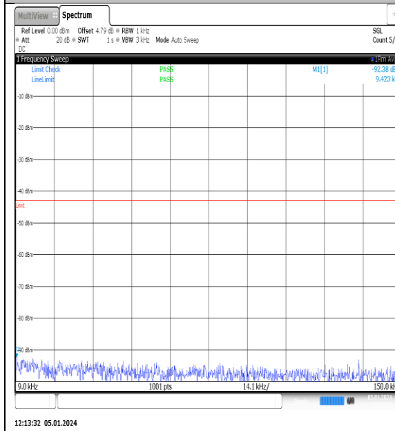
NTNV_N77-3700- 3980_PC2_30_15_M_TID7_NS_01_0.009_0.15_#1
