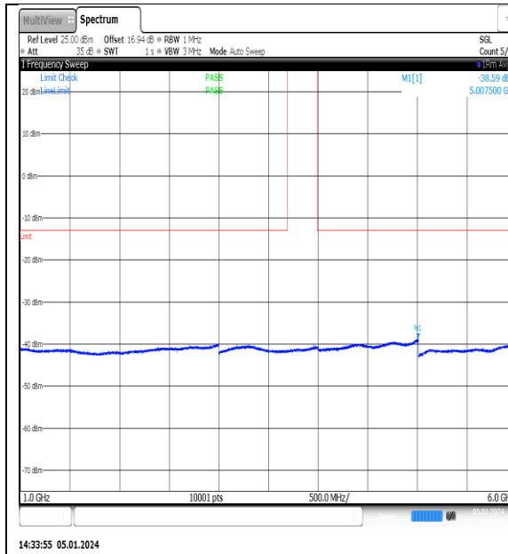
NTN_V_N77-3700- 3980_PC2_30_15_H_TID12_NS_01_1000_6000_ #1
