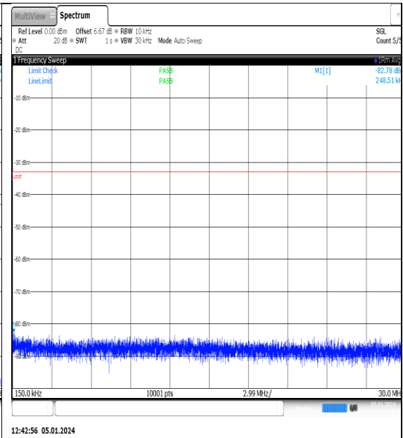
NTN_V_N77-3700- 3980_PC2_30_15_M_TID14_NS_01_0.15_30_#1
