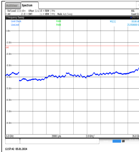
NTNV_N77-3700- 3980_PC2_30_15_H_TID1_NS_01_6000_26000_#1
