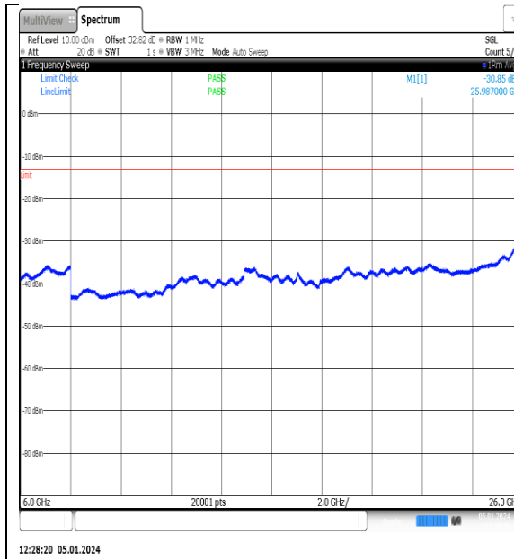
NTNV_N77-3700- 3980_PC2_30_15_M_TID10_NS_01_6000_26000 _#1
