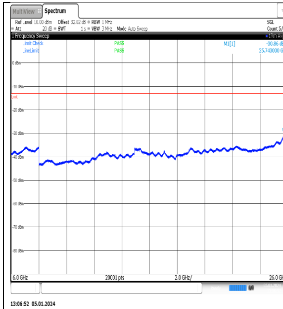
NTNV_N77-3700- 3980_PC2_30_15_H_TID3_NS_01_6000_26000_#1
