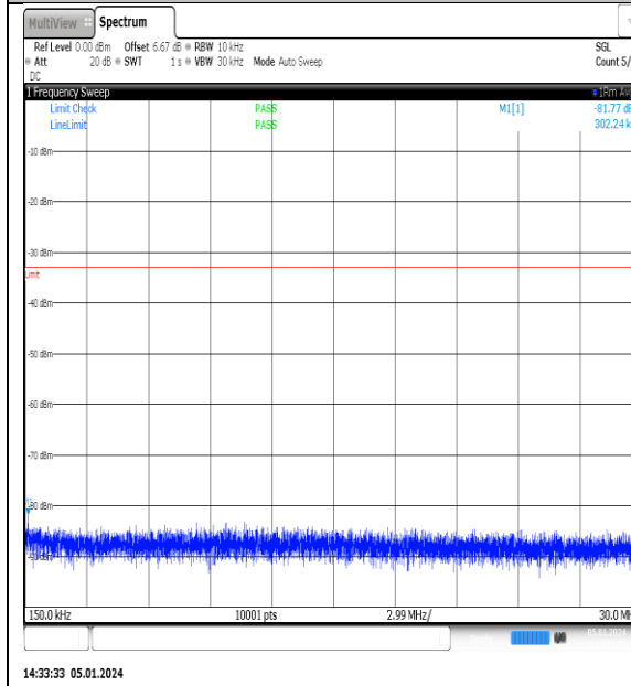
NTNV_N77-3700- 3980_PC2_30_15_H_TID12_NS_01_0.15_30_#1
