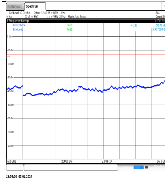
NTNV_N77-3700- 3980_PC2_30_15_H_TID9_NS_01_6000_26000_#1
