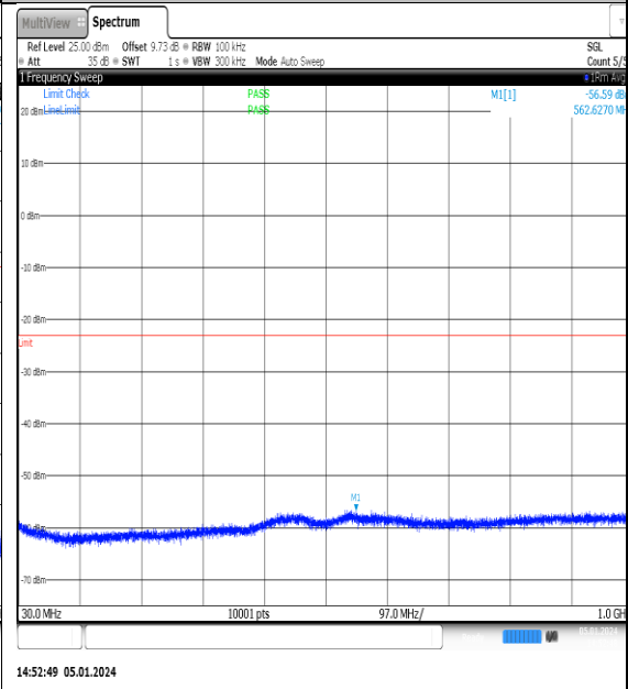
NTNV_N77-3700- 3980_PC2_30_15_H_TID14_NS_01_30_1000_#1
