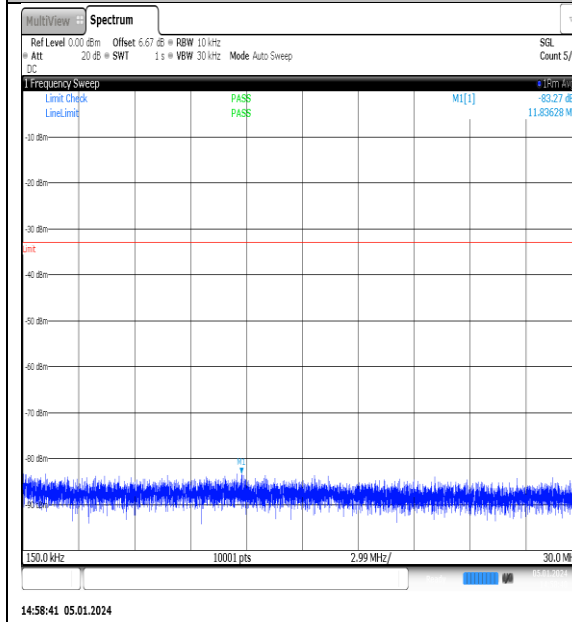
NTNV_N77-3700- 3980_PC2_30_20_L_TID1_NS_01_0.15_30_#1
