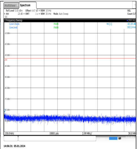
NTNV_N77-3700- 3980_PC2_30_15_H_TID11_NS_01_0.15_30_#1
