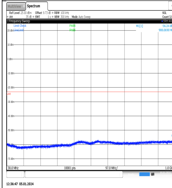
NTN_V_N77-3700- 3980_PC2_30_15_M_TID12_NS_01_30_1000_#1
