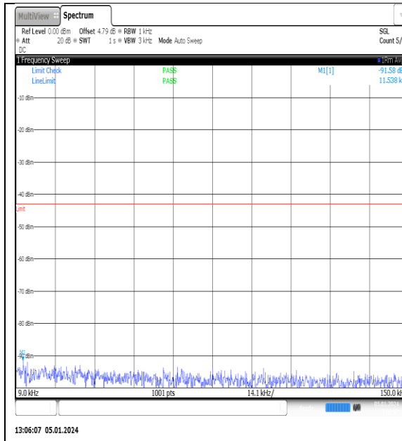
NTNV_N77-3700- 3980_PC2_30_15_H_TID3_NS_01_0.009_0.15_# 1
