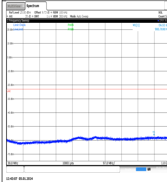
NTN_V_N77-3700- 3980_PC2_30_15_M_TID14_NS_01_30_1000_#1
