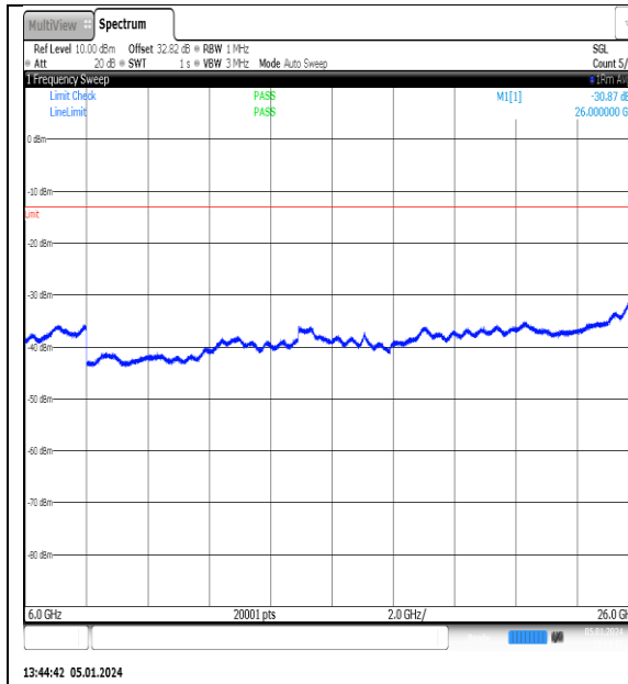
NTNV_N77-3700- 3980_PC2_30_15_H_TID7_NS_01_6000_26000_#1
