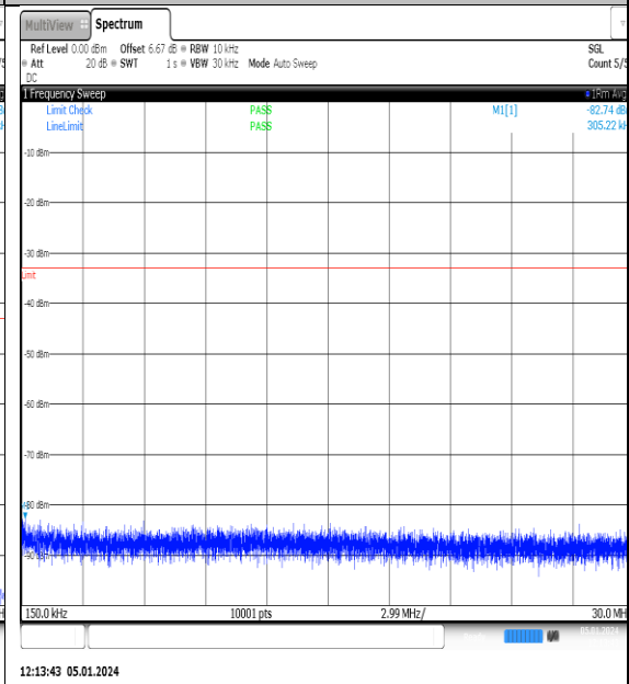
NTNV_N77-3700- 3980_PC2_30_15_M_TID7_NS_01_0.15_30_#1
