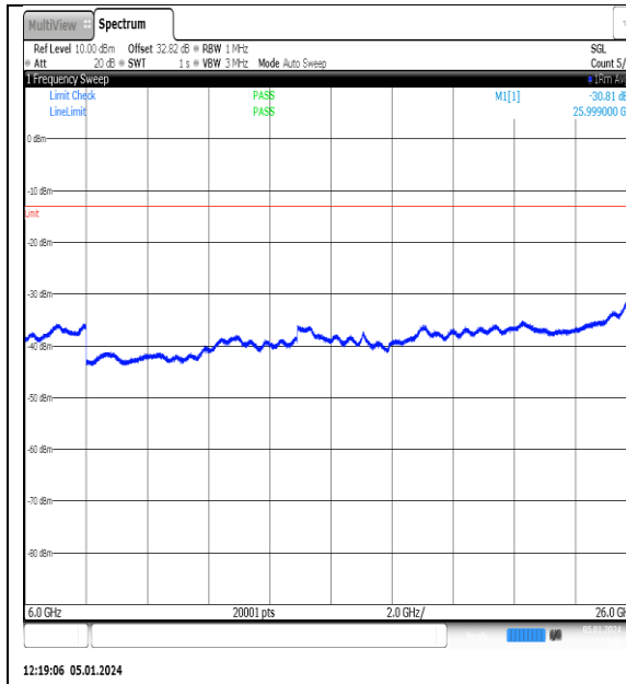
NTNV_N77-3700- 3980_PC2_30_15_M_TID8_NS_01_6000_26000_#1
