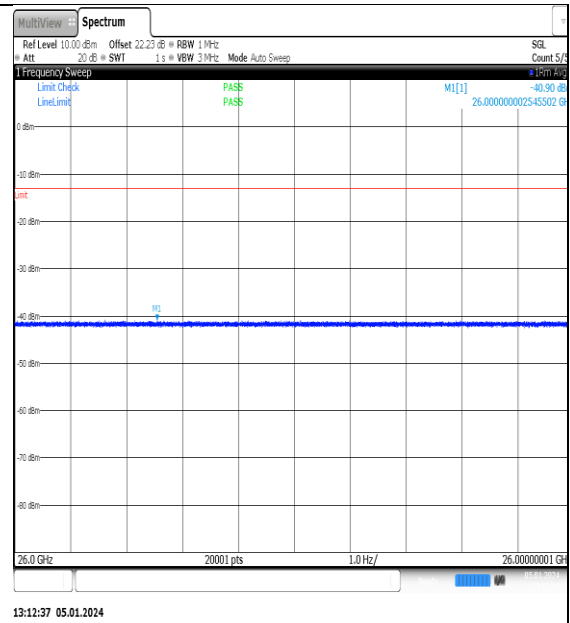
NTNV_N77-3700- 3980_PC2_30_15_H_TID5_NS_01_26000_40000_#1
