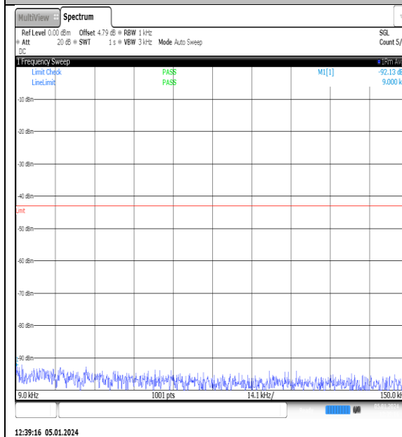
NTNV_N77-3700- 3980_PC2_30_15_M_TID13_NS_01_0.009_0.15_ _#1
