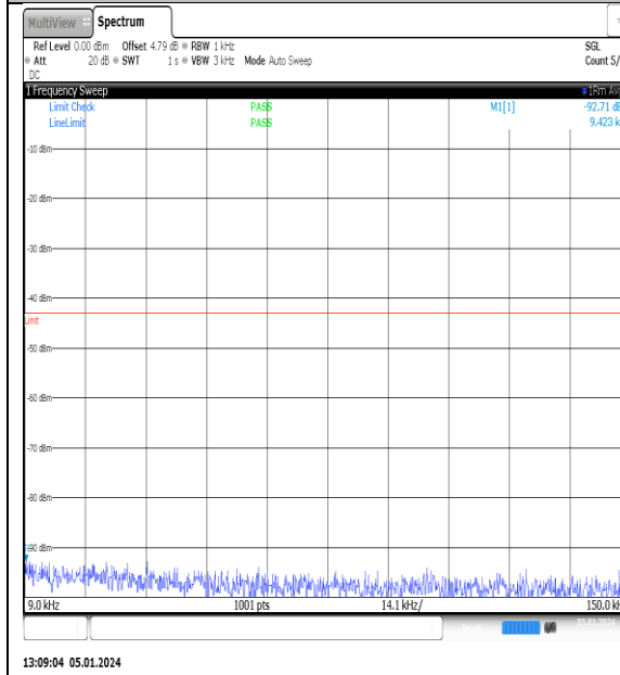
NTNV_N77-3700- 3980_PC2_30_15_H_TID4_NS_01_0.009_0.15_#1
