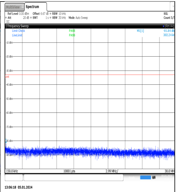
NTNV_N77-3700- 3980_PC2_30_15_H_TID3_NS_01_0.15_30_#1
