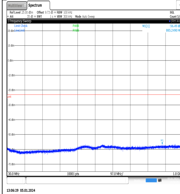
NTNV_N77-3700- 3980_PC2_30_15_H_TID3_NS_01_30_1000_#1
