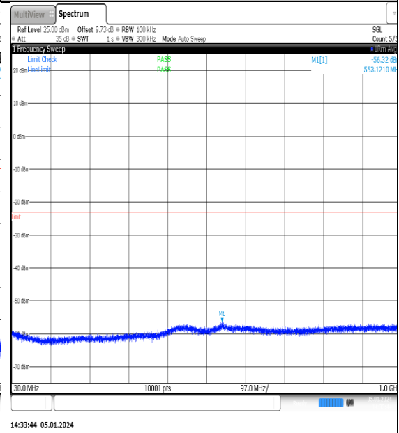
NTNV_N77-3700- 3980_PC2_30_15_H_TID12_NS_01_30_1000_#1
