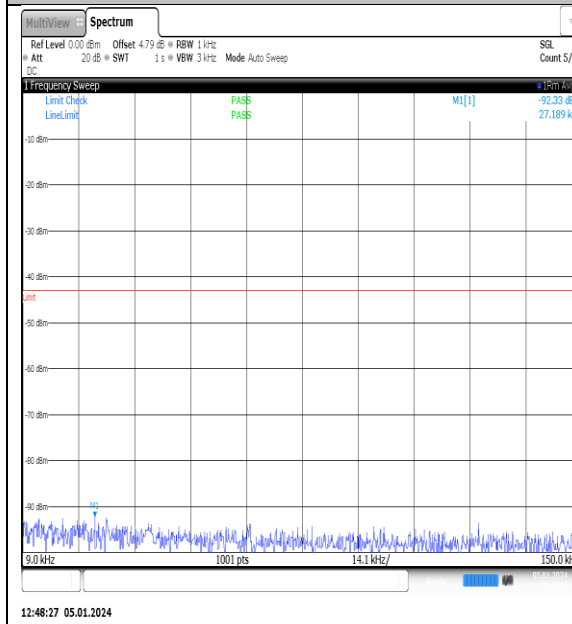
NTNV_N77-3700- 3980_PC2_30_15_M_TID15_NS_01_0.009_0.15_#1
