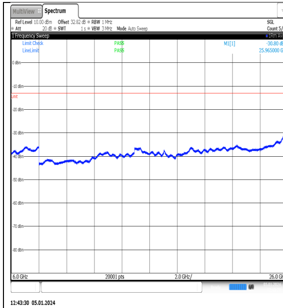
NTNV_N77-3700- 3980_PC2_30_15_M_TID14_NS_01_6000_26000 _#1
