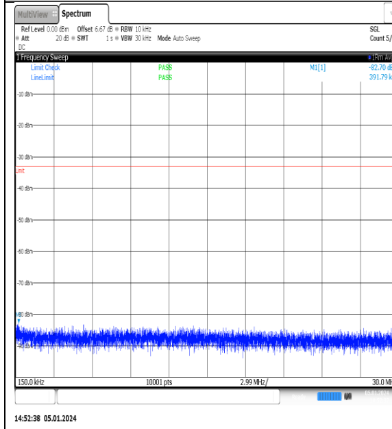
NTNV_N77-3700- 3980_PC2_30_15_H_TID14_NS_01_0.15_30_#1
