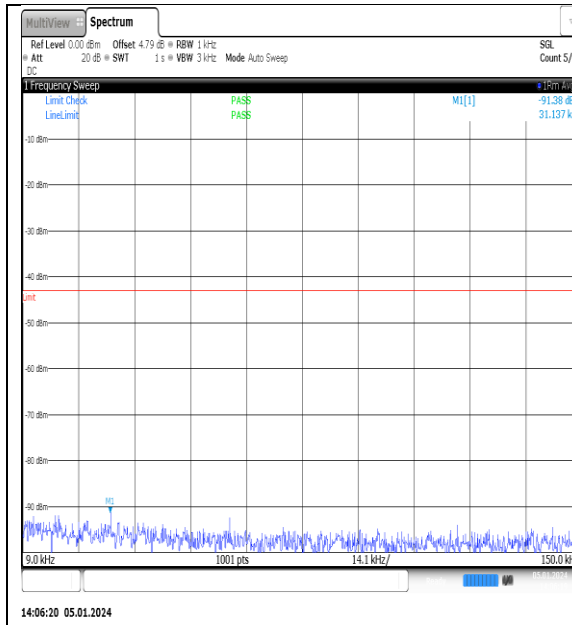
NTNV_N77-3700- 3980_PC2_30_15_H_TID11_NS_01_0.009_0.15_#1
