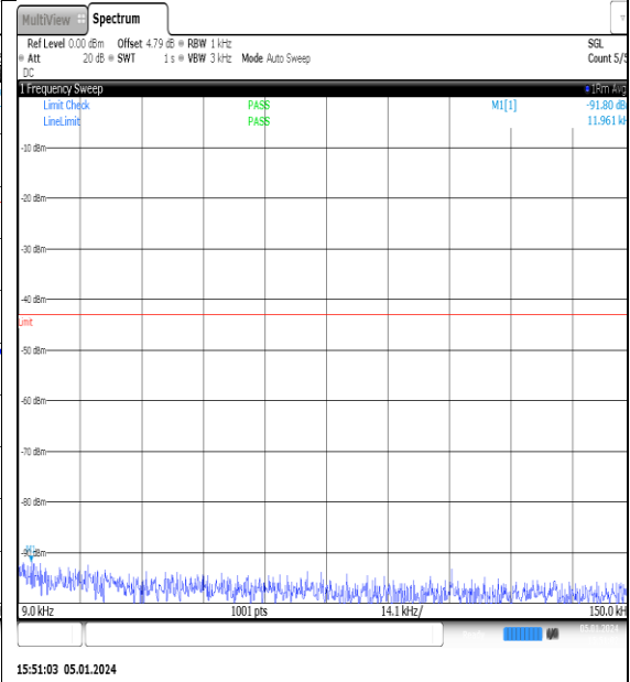
NTN_V_N77-3700- 3980_PC2_30_15_H_TID13_NS_01_0.009_0.15_ #1
