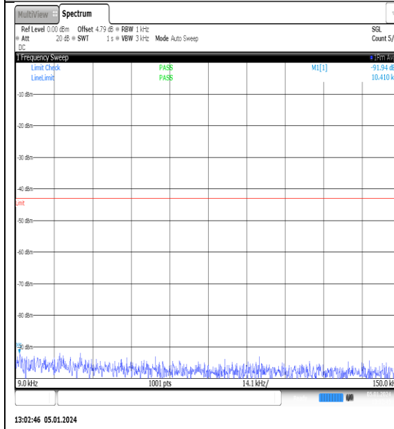
NTNV_N77-3700- 3980_PC2_30_15_H_TID2_NS_01_0.009_0.15_#1
