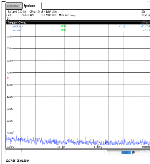
NTNV_N77-3700- 3980_PC2_30_15_M_TID10_NS_01_0.009_0.15_ #1
