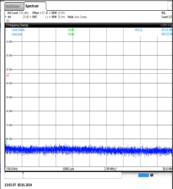
NTNV_N77-3700- 3980_PC2_30_15_H_TID2_NS_01_0.15_30_#1
