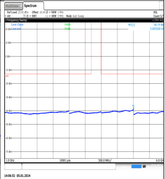
NTNV_N77-3700- 3980_PC2_30_15_H_TID11_NS_01_1000_6000_#1
