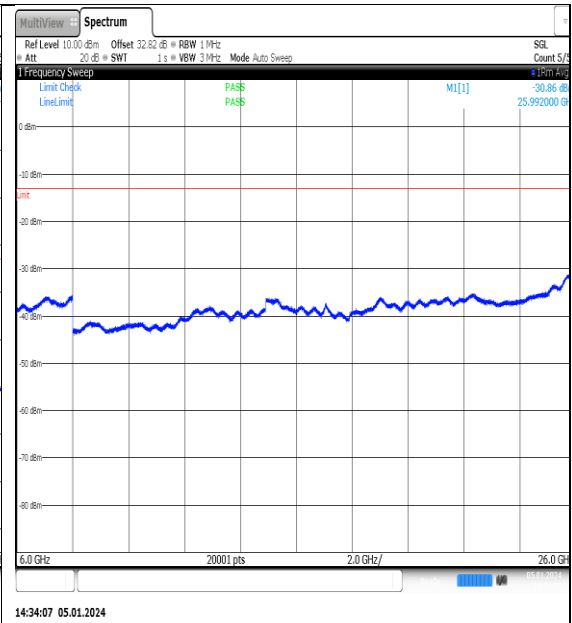
NTN_V_N77-3700- 3980_PC2_30_15_H_TID12_NS_01_6000_26000 #1
