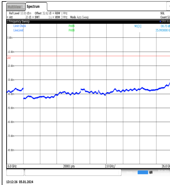
NTNV_N77-3700- 3980_PC2_30_15_H_TID5_NS_01_6000_26000_#1
