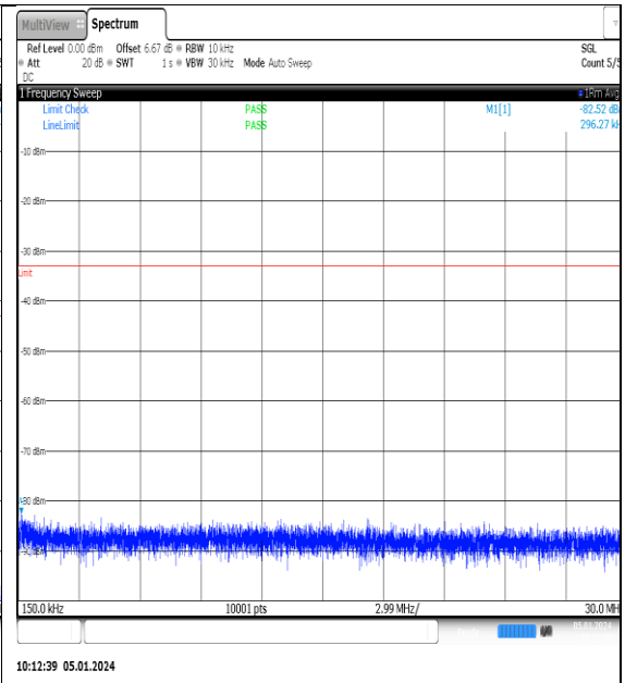
NTNV_N77-3700- 3980_PC2_30_10_H_TID10_NS_01_0.15_30_#1
