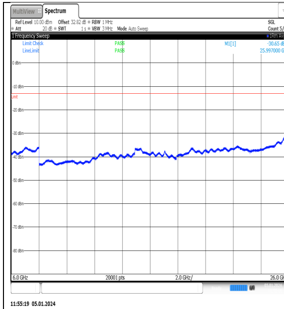
NTNV_N77-3700- 3980_PC2_30_15_M_TID2_NS_01_6000_26000_#1
