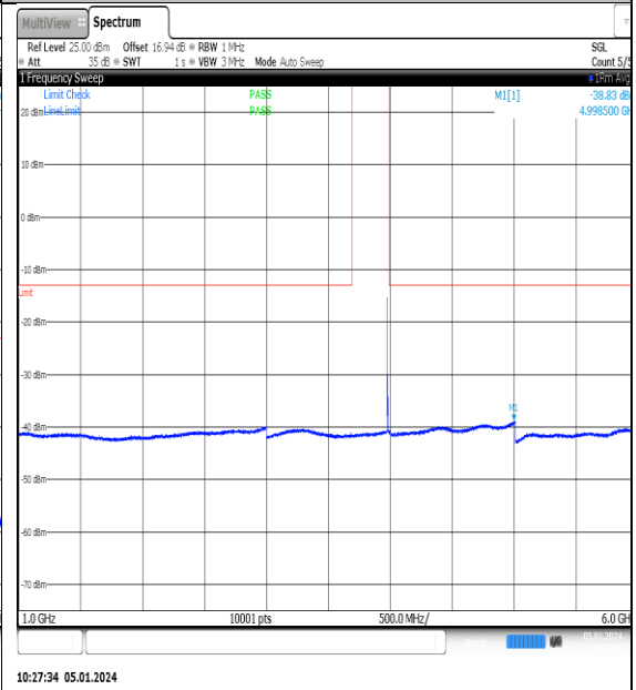
NTN_V_N77-3700- 3980_PC2_30_10_H_TID14_NS_01_1000_6000_ #1
