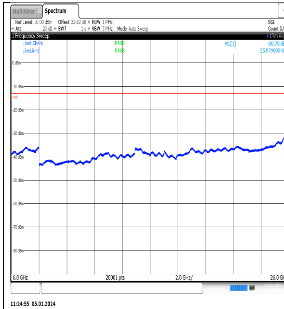
NTNV_N77-3700- 3980_PC2_30_15_L_TID7_NS_01_6000_26000_ #1
