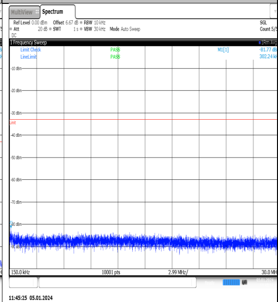
NTNV_N77-3700- 3980_PC2_30_15_L_TID14_NS_01_0.15_30_#1
