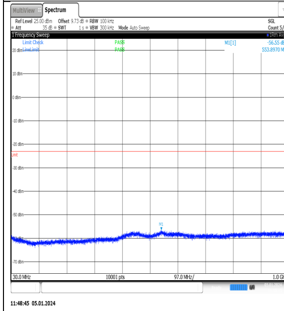
NTNV_N77-3700- 3980_PC2_30_15_L_TID15_NS_01_30_1000_#1
