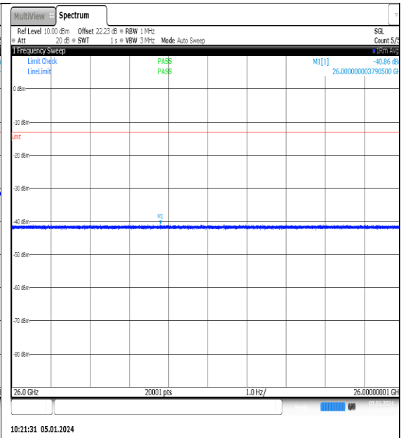
NTNV_N77-3700- 3980_PC2_30_10_H_TID12_NS_01_26000_4000 0_#1
