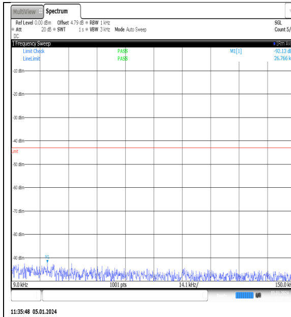
NTNV_N77-3700- 3980_PC2_30_15_L_TID11_NS_01_0.009_0.15_ #1
