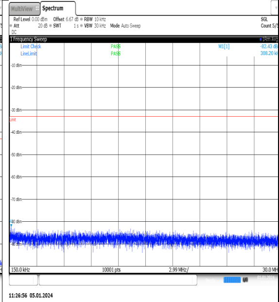
NTNV_N77-3700- 3980_PC2_30_15_L_TID8_NS_01_0.15_30_#1
