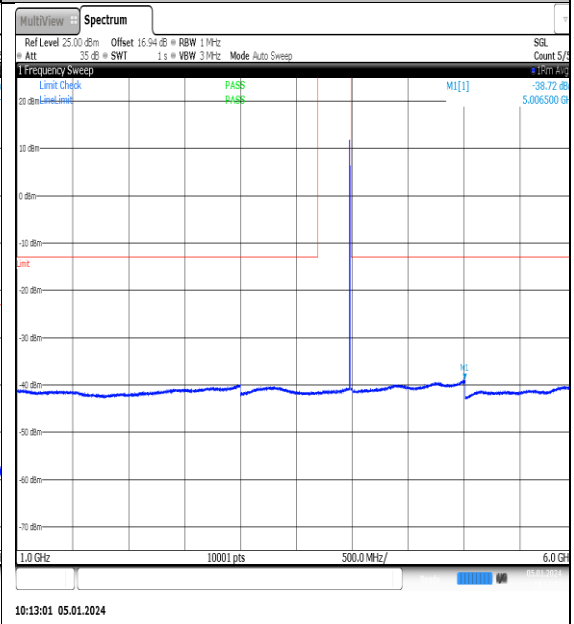
NTNV_N77-3700- 3980_PC2_30_10_H_TID10_NS_01_1000_6000_ #1
