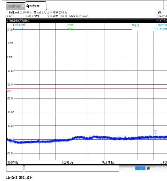
NTN_V_N77-3700- 3980_PC2_30_15_L_TID13_NS_01_30_1000_#1
