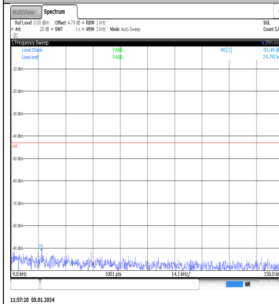
NTNV_N77-3700- 3980_PC2_30_15_M_TID3_NS_01_0.009_0.15_#1
