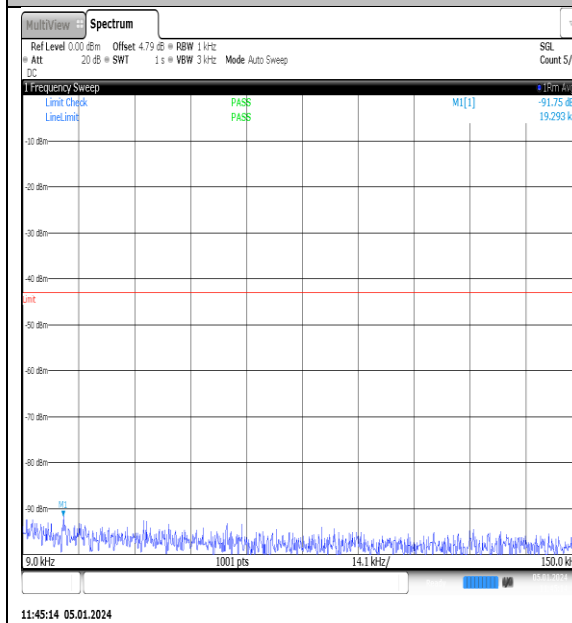
NTNV_N77-3700- 3980_PC2_30_15_L_TID14_NS_01_0.009_0.15_#1
