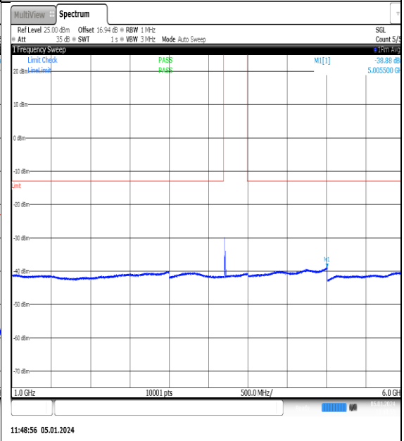
NTNV_N77-3700- 3980_PC2_30_15_L_TID15_NS_01_1000_6000_ #1
