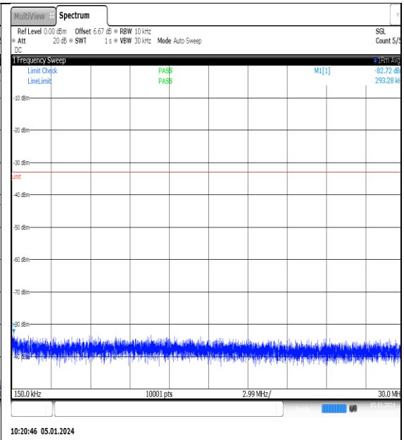
NTNV_N77-3700- 3980_PC2_30_10_H_TID12_NS_01_0.15_30_#1
