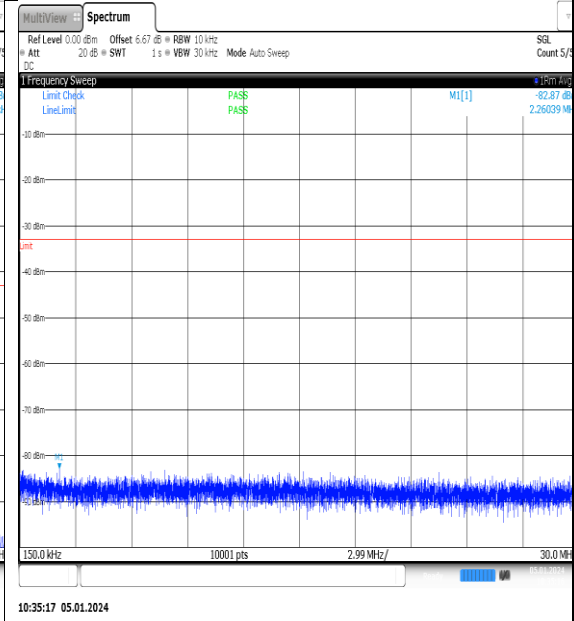
NTNV_N77-3700- 3980_PC2_30_15_L_TID2_NS_01_0.15_30_#1
