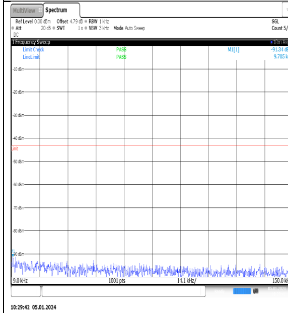
NTNV_N77-3700- 3980_PC2_30_10_H_TID15_NS_01_0.009_0.15_#1
